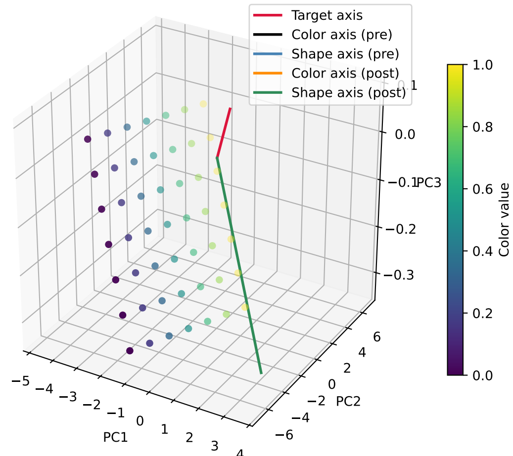
Shape-aligned (post)
