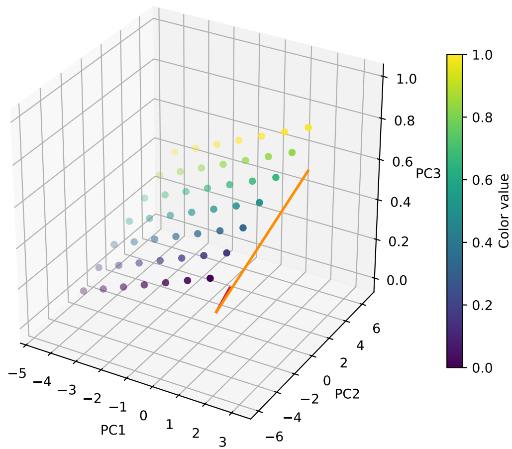
Color-aligned (post)
