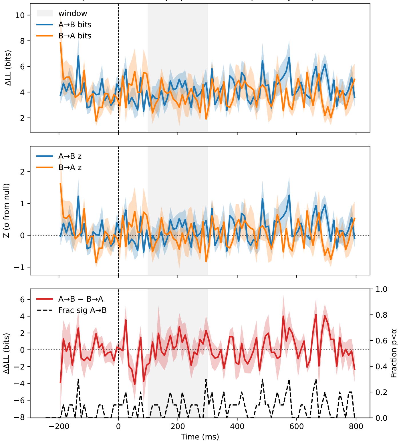
STIM | crnull-horizontal | C | MFEF vs MLIP | monkey=M | N=10
