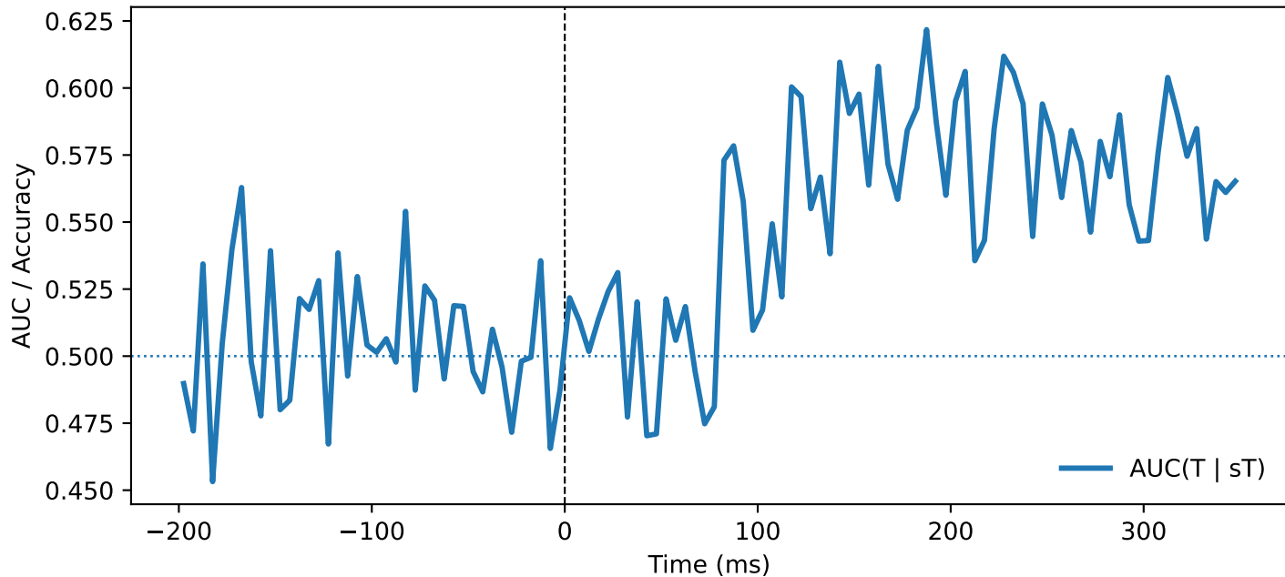
MFEF — QC (targ, ori=None, PT \geq 200.0)
