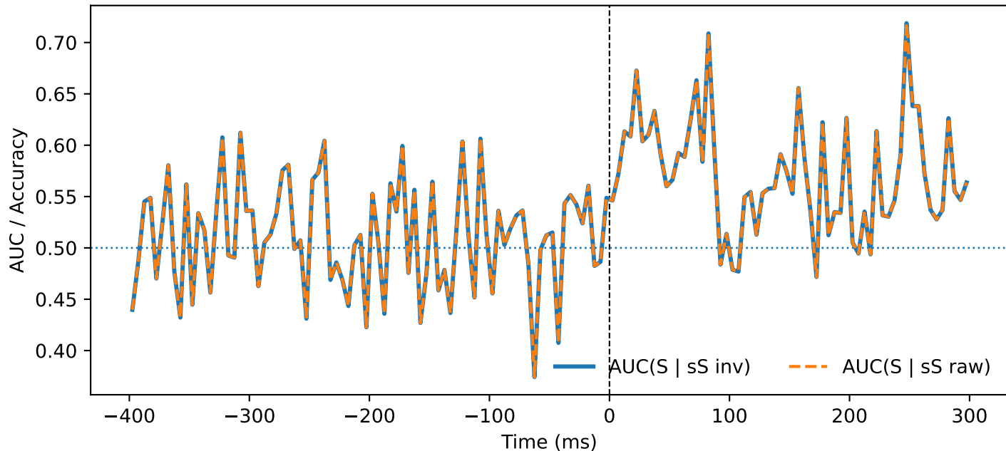
SLIP — QC (sacc, ori=vertical, PT \geq 200.0, norm=global)
