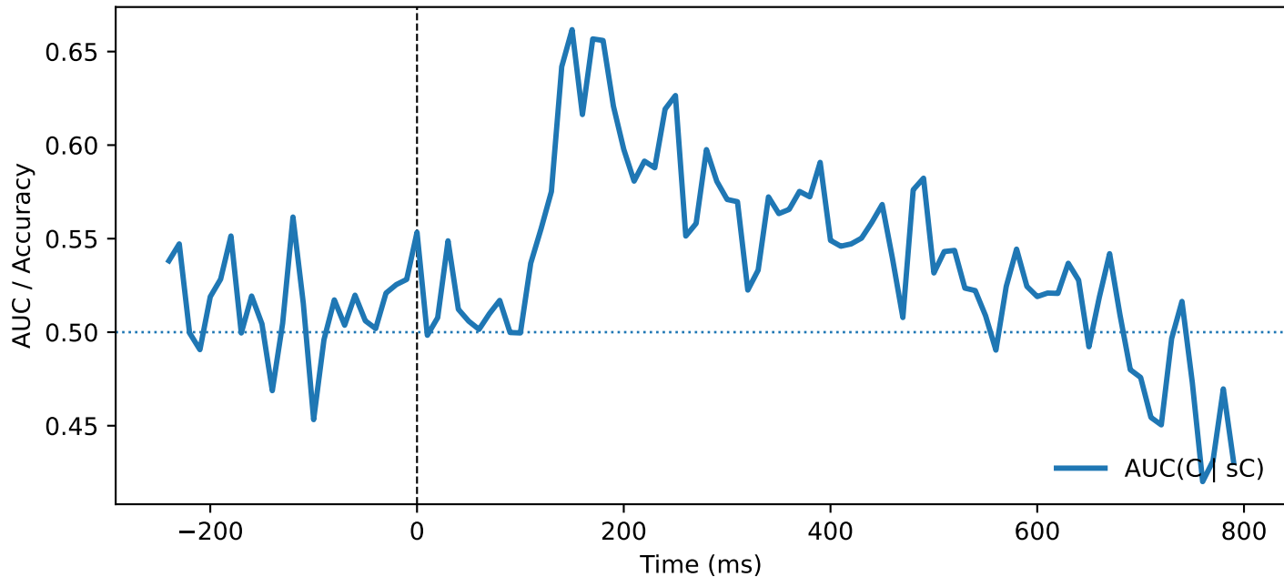
MSC — QC (stim, ori=None, PT \geq 200.0, norm=global)
