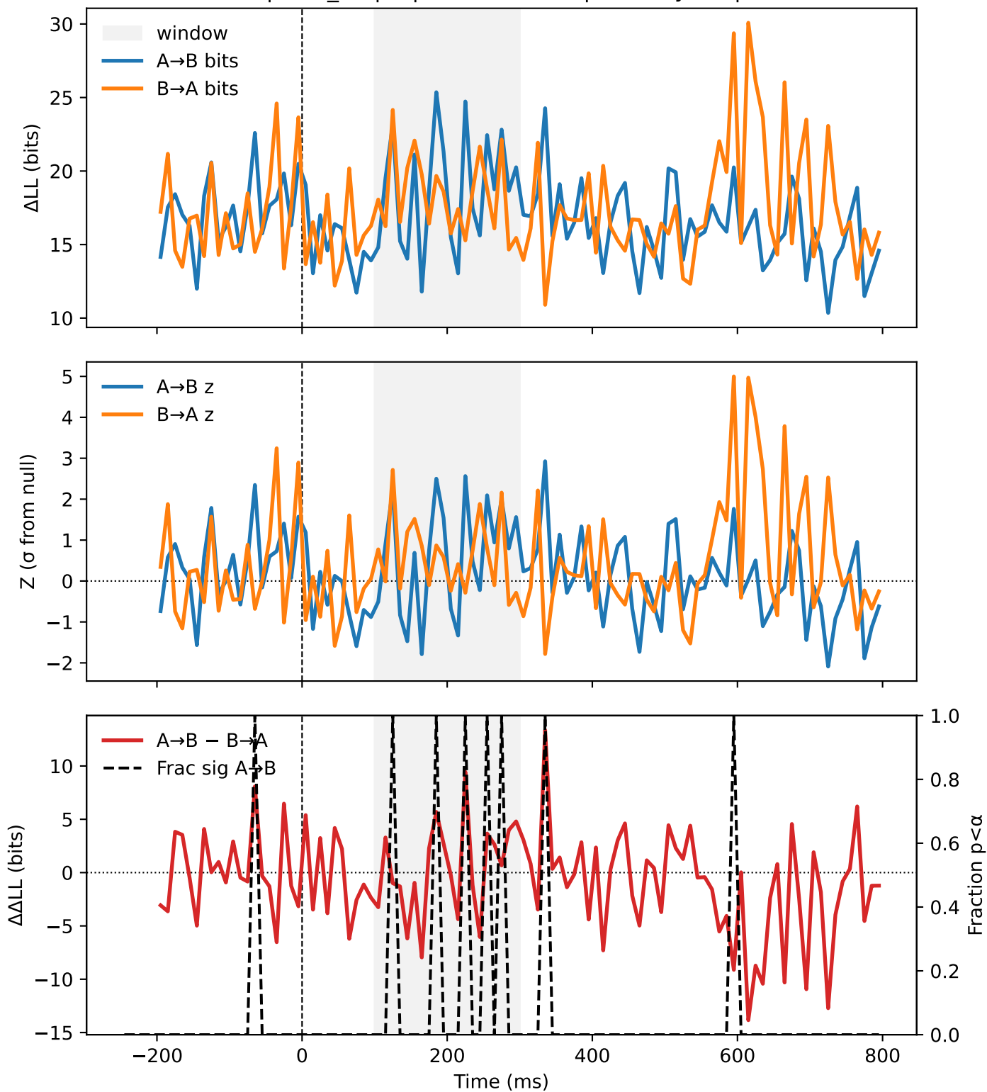
STIM | flow_v1 | R | MFEF vs MSC | monkey=M | N=1
