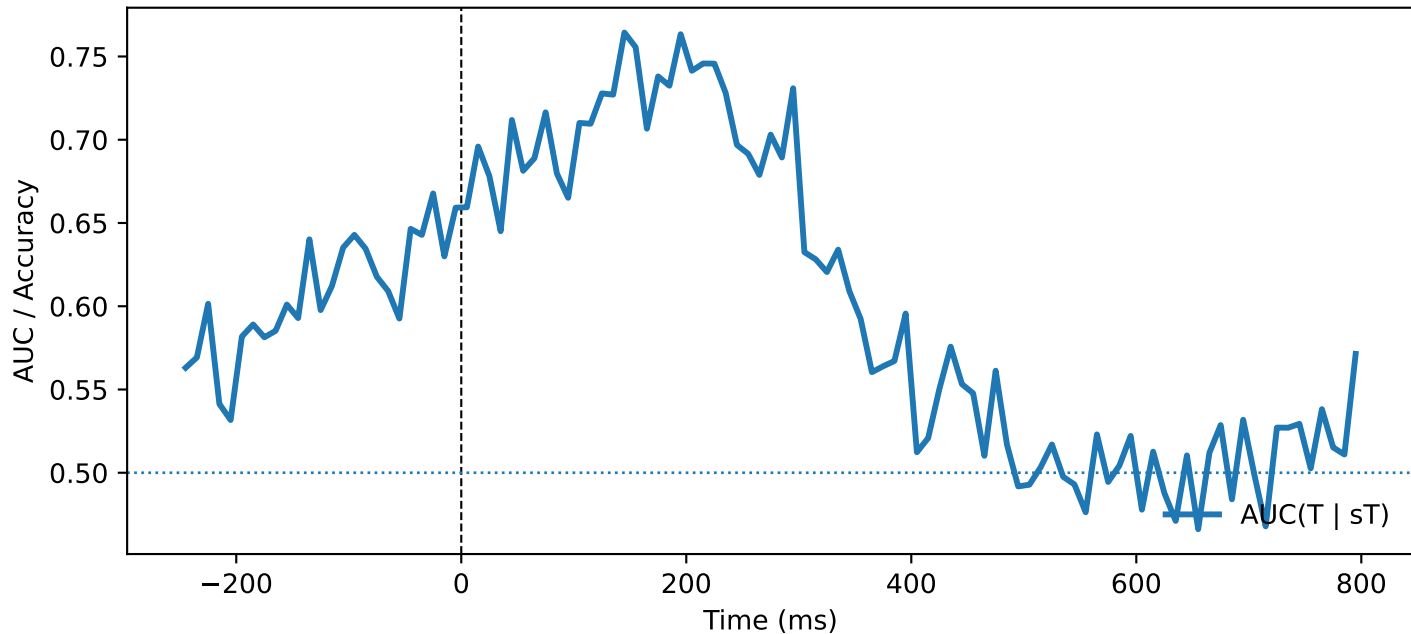
MSC — QC (stim, ori=None, PT \geq 200.0)
