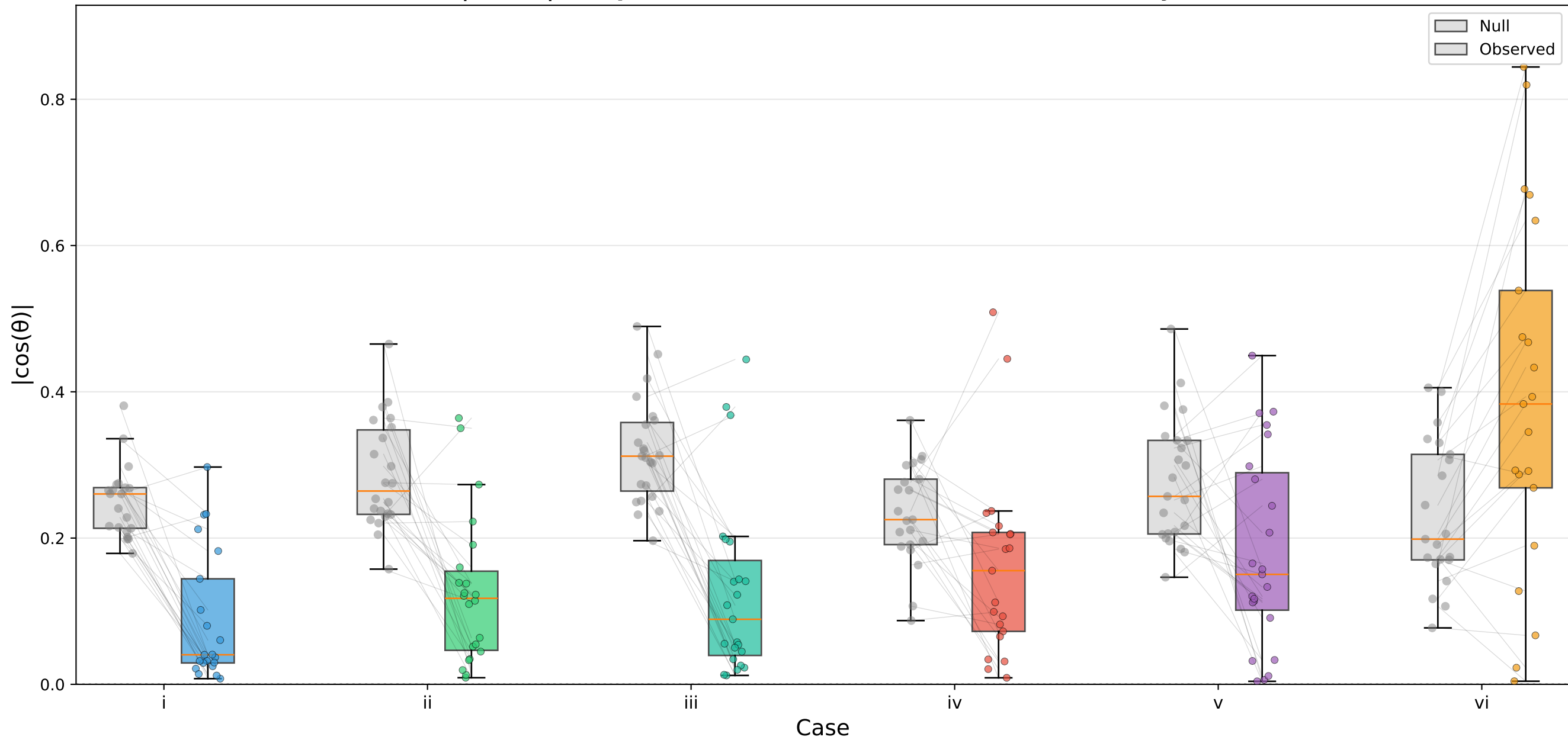
|\cos(\theta)| Comparison Across Six Cases (Correct Trials Only)
