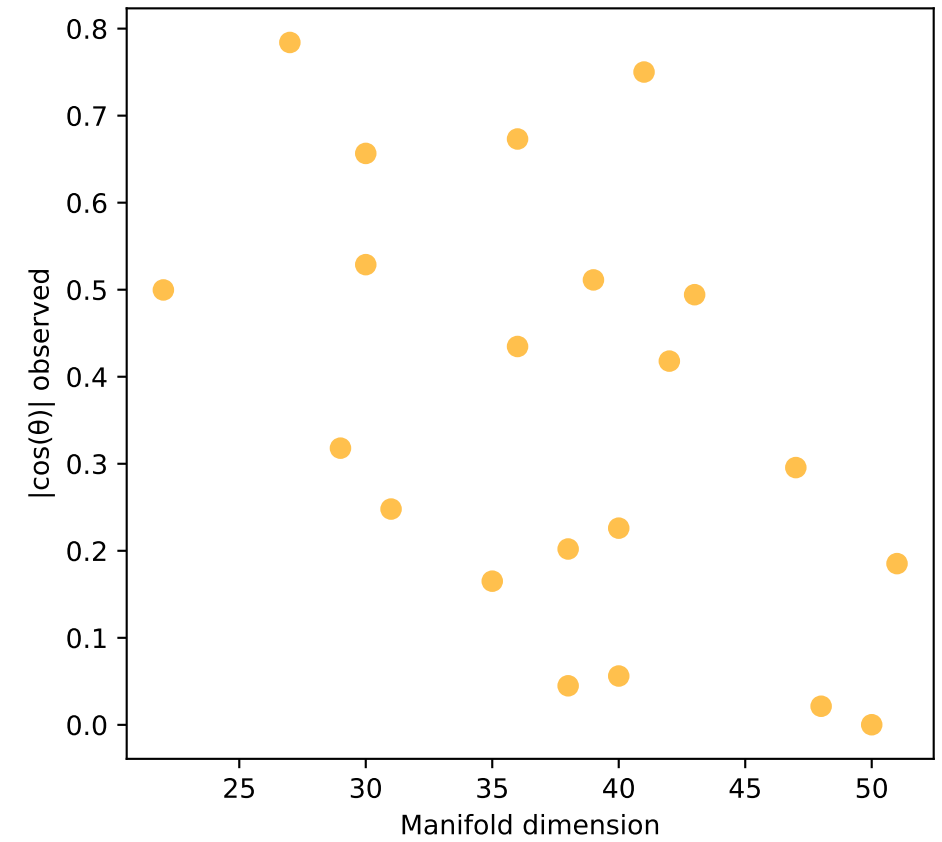
a_obs vs manifold_dim r=-0.500 , p=0.0209
