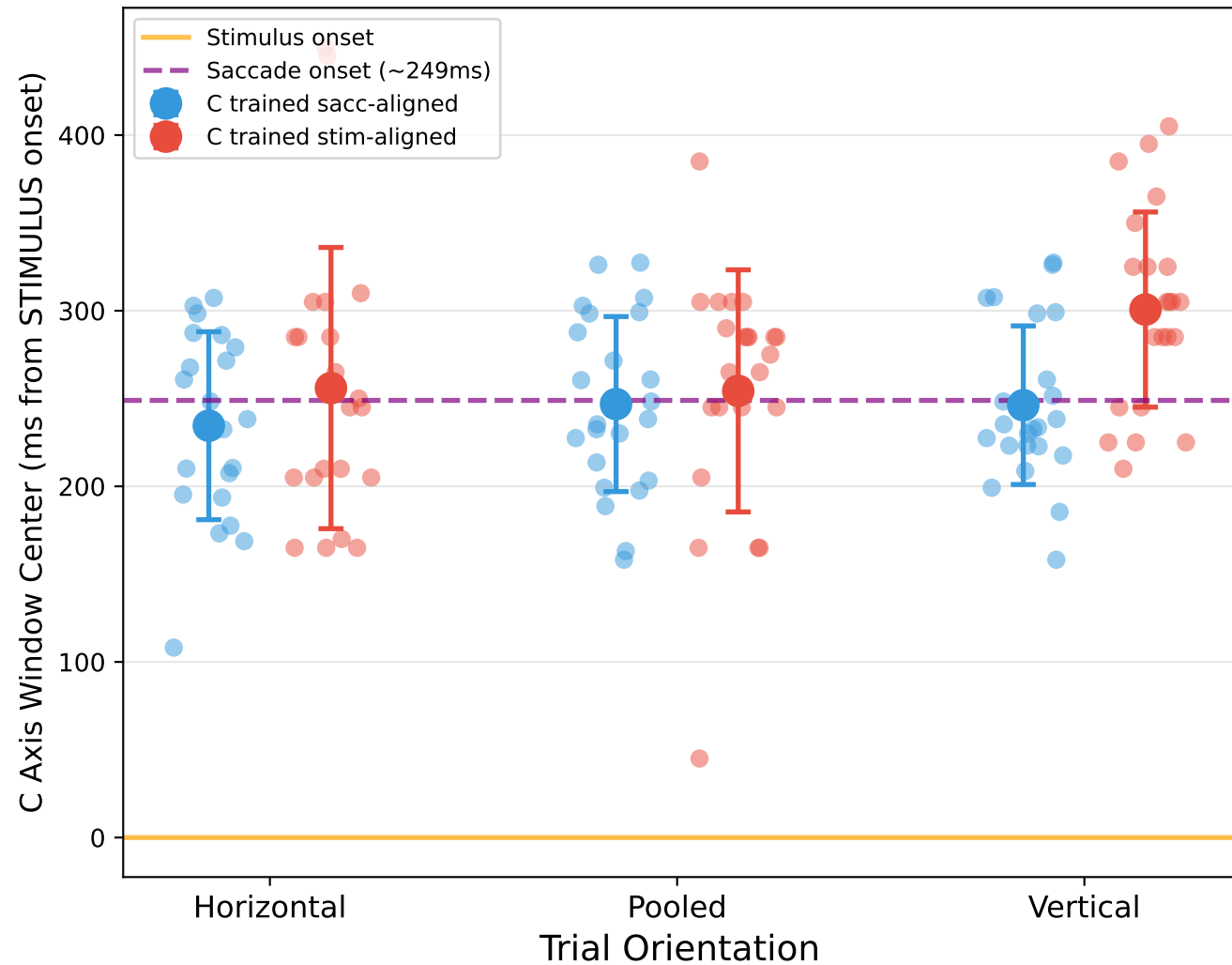
C Axis Window Center Comparison (all converted to stimulus-aligned timeline)
