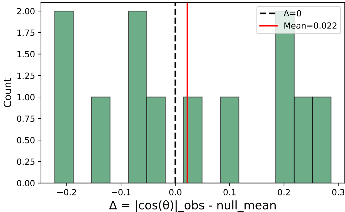
Case iv: Stim-C vs Sacc-S pooled (correct) - Monkey S
