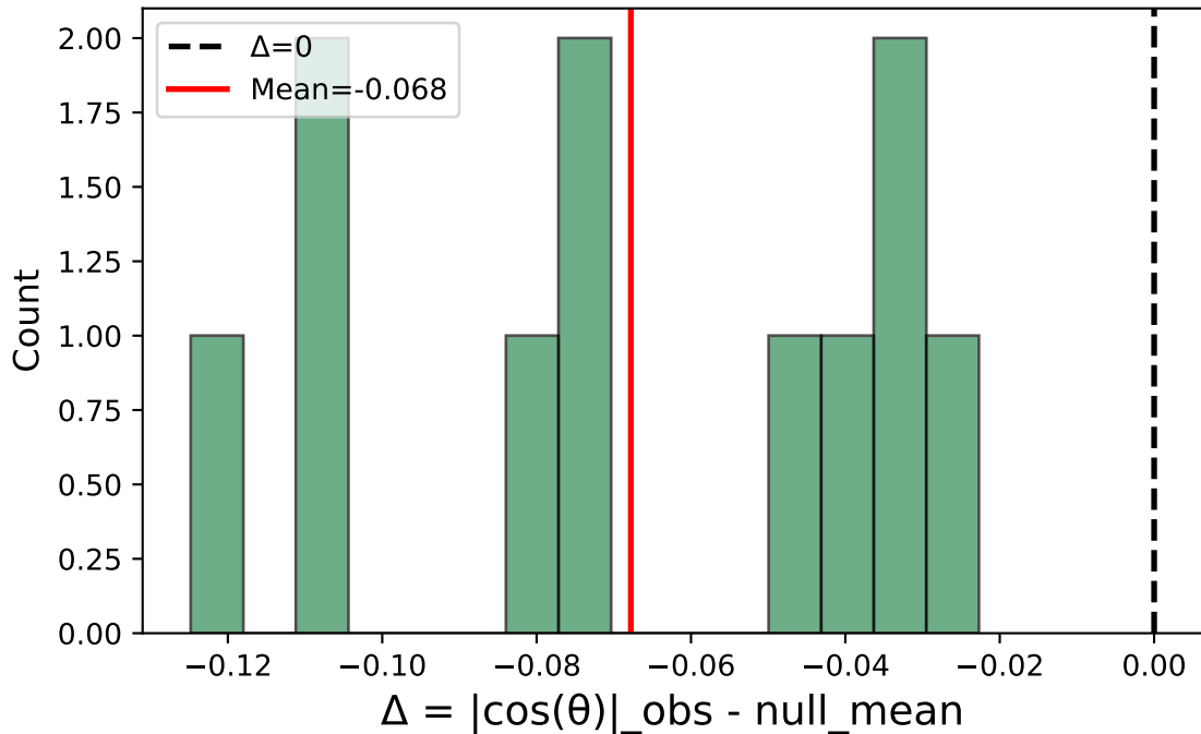
Monkey M: Axis Alignment \Delta (covariance null)
