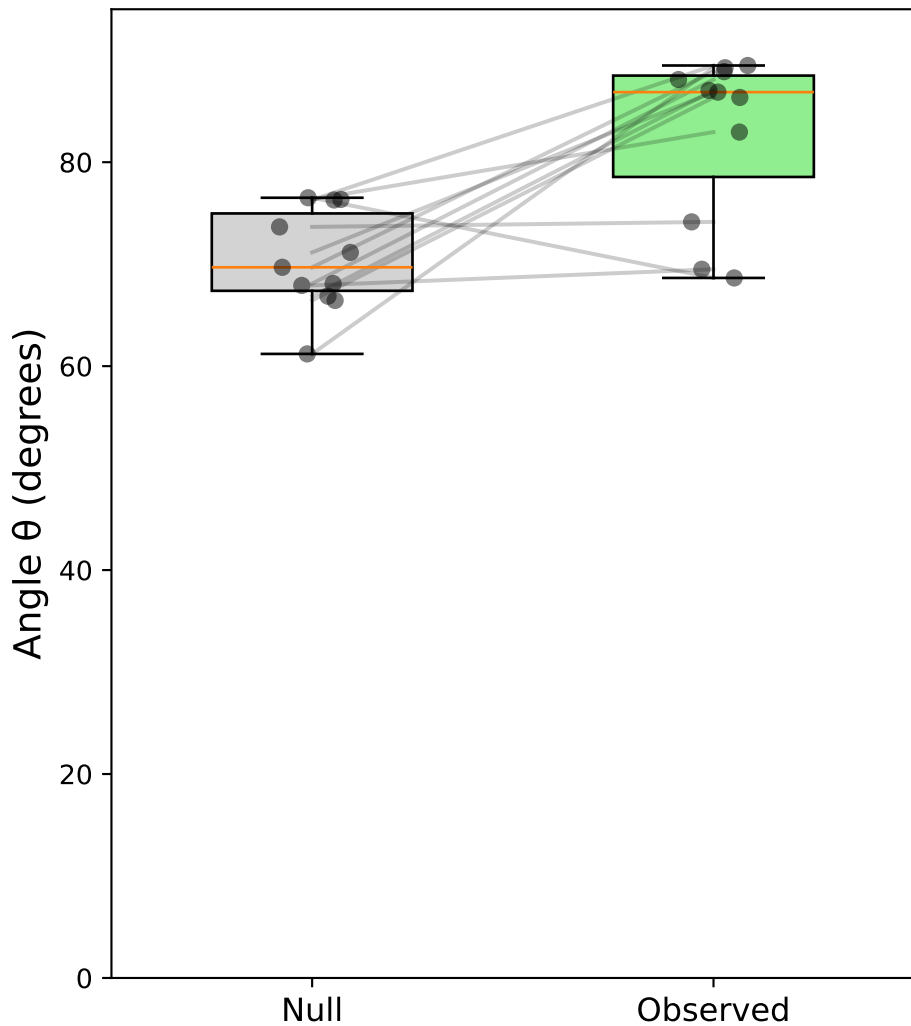
Case ii: Sacc C&S (pooled, correct) - Monkey S \Delta\theta = 12.5^\circ
