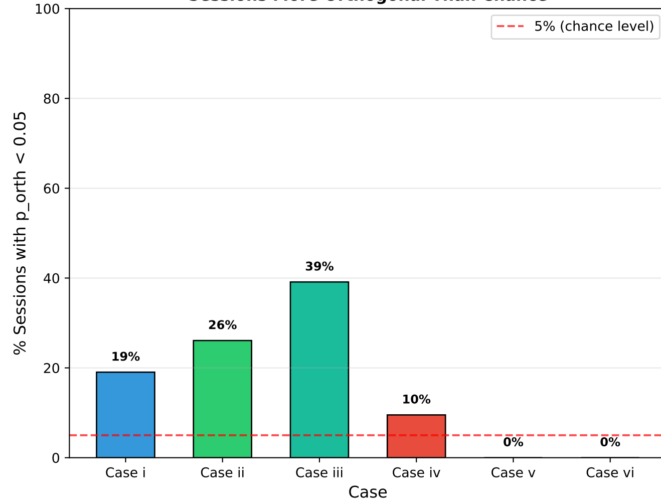
Sessions More Orthogonal Than Chance
