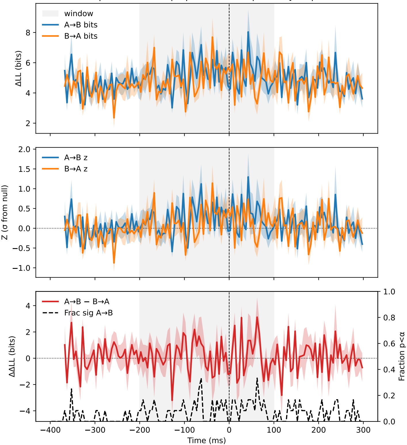
SACC | crnull-vertical | S | SFEF vs SLIP | monkey=S | N=12
