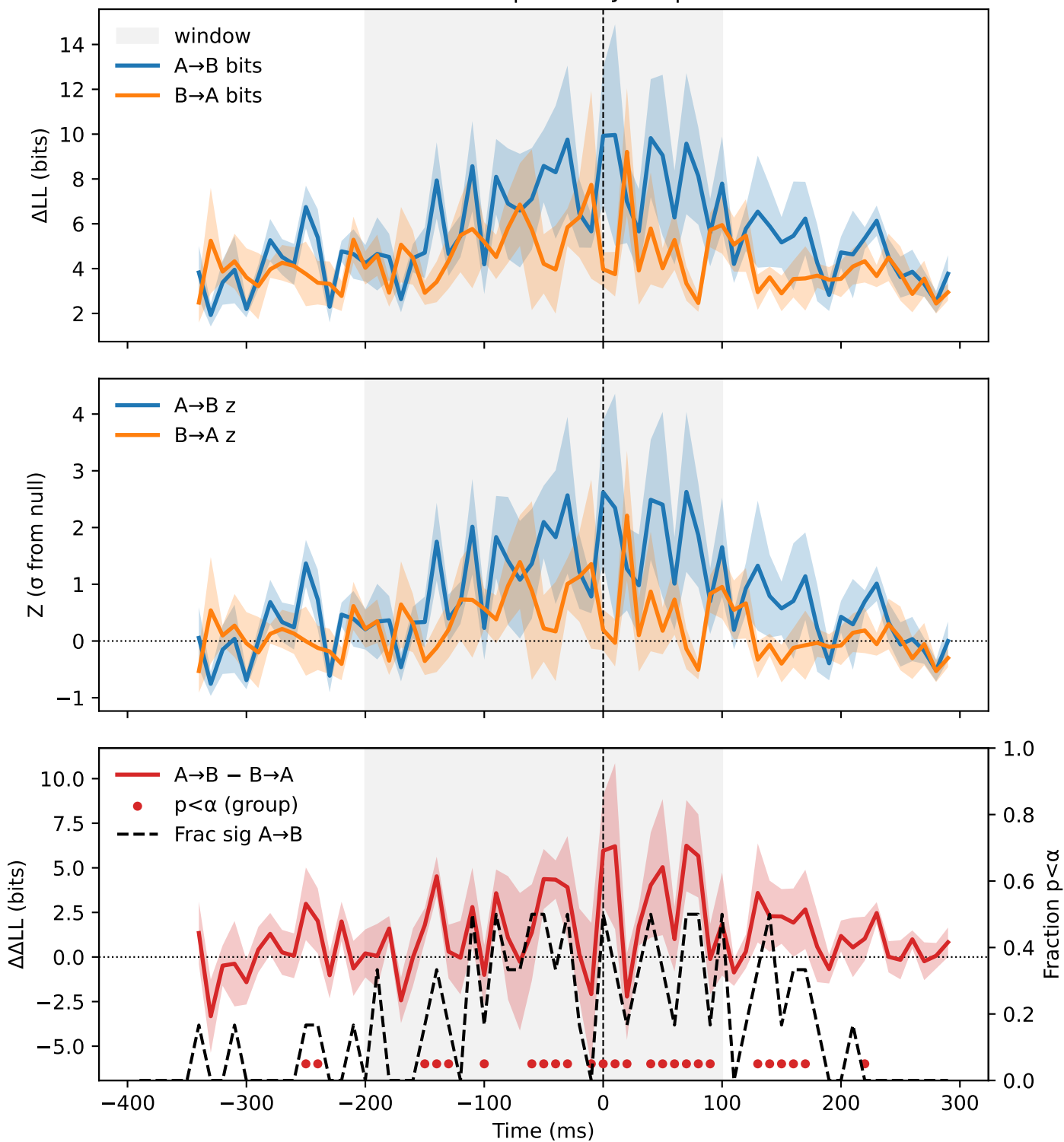
SACC | evoked_peakbin_saccS_horizontal_lag50ms_20mssw-none-trial | S MFEF vs MSC | monkey=M | N=6
