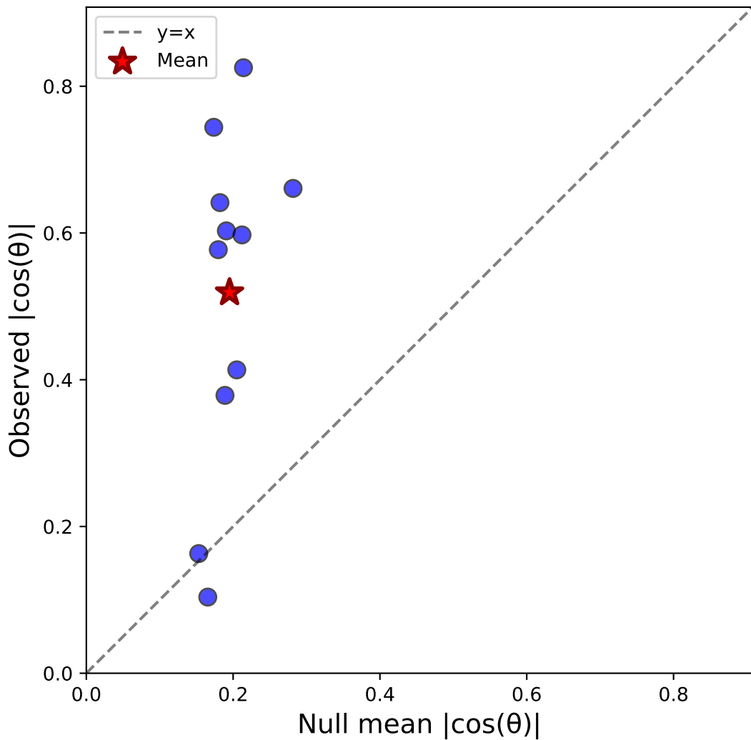
Case iii: Stim-C(ver) vs Sacc-S(horiz) (all) - Monkey M N=11, \Delta=0.324 , Sig=0/11
