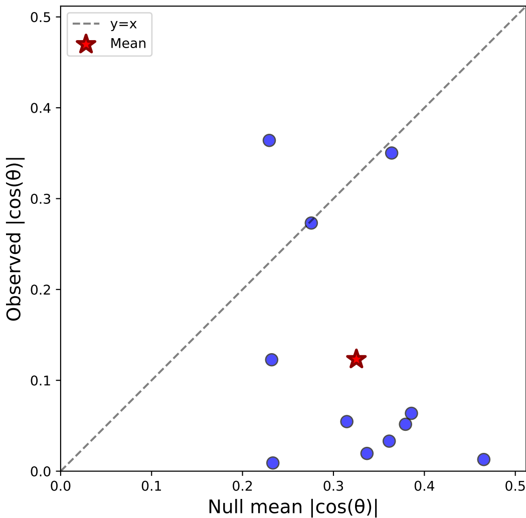
Case ii: Sacc C&S (pooled, correct) - Monkey S N=11, \Delta=-0.202
