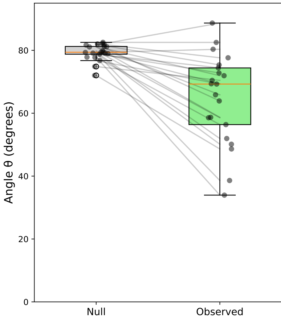
Case iii: Stim-C(ver) vs Sacc-S(horiz) (correct) - Monkey all \Delta\theta = -14.6^\circ
