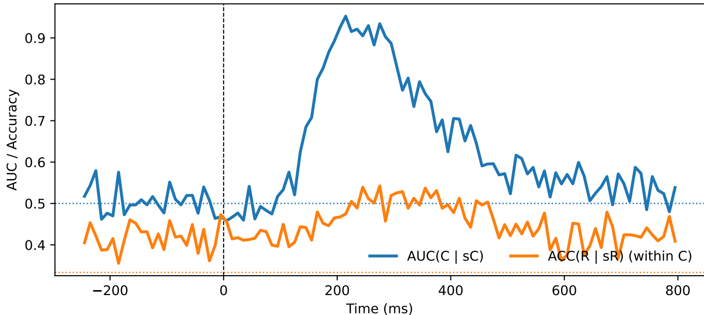
MFEF — QC (stim, ori=vertical, PT \geq 200.0, norm=global)
