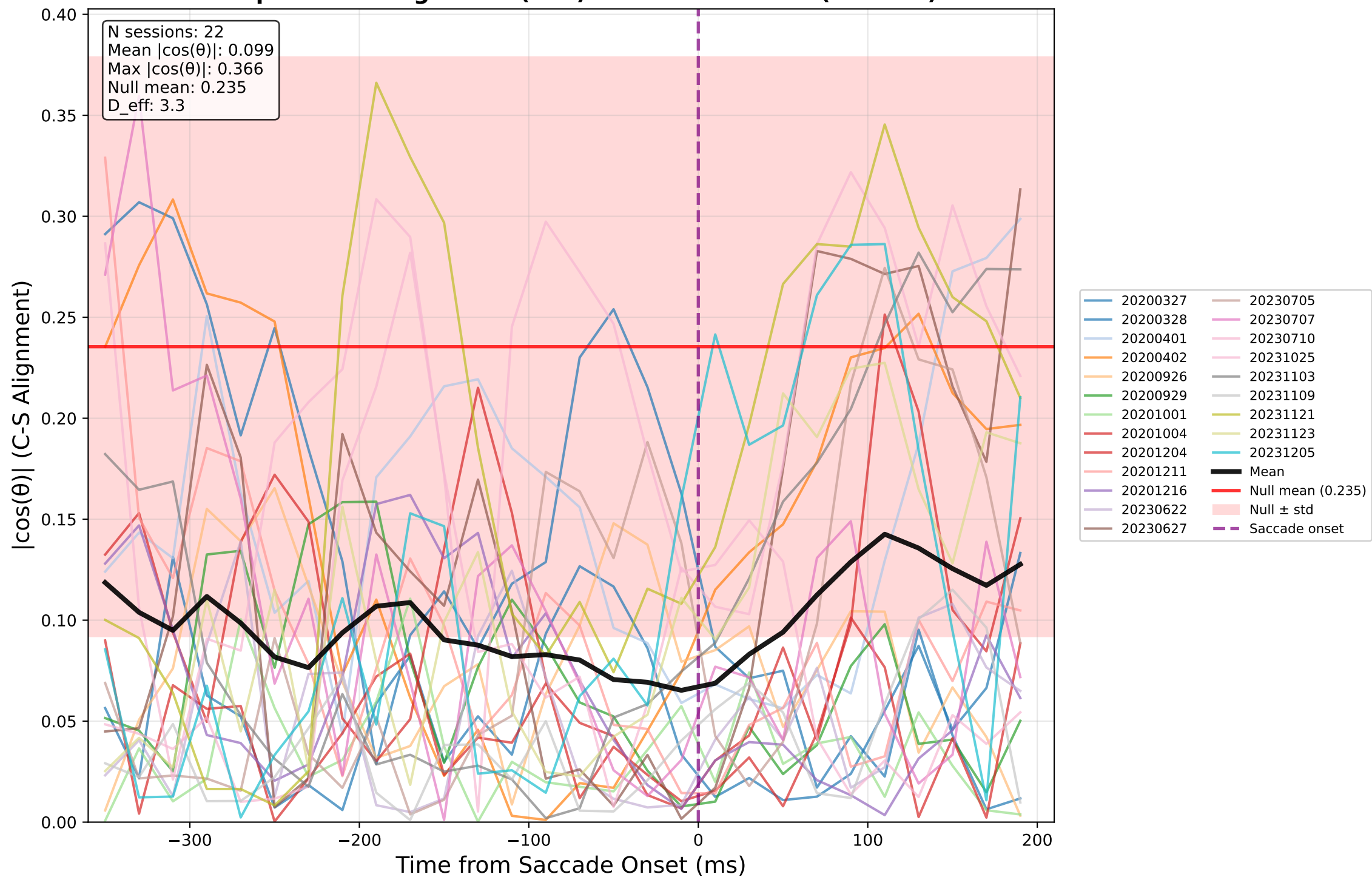
Temporal C-S Alignment (FEF): Horizontal Trials (alltrials)
