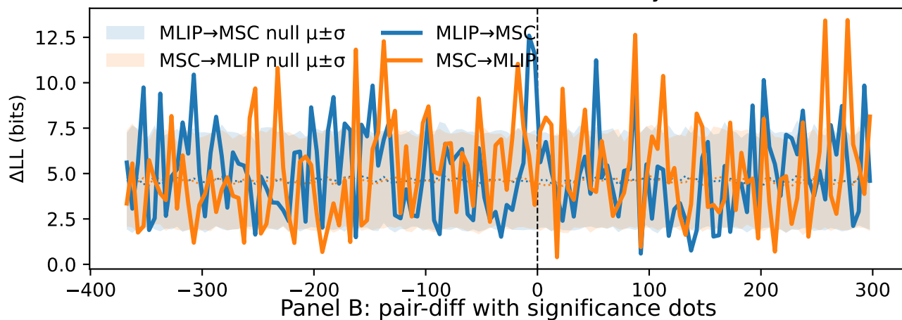
(MLIP vs MSC) — S-flow — Panel A: overlay + null bands
