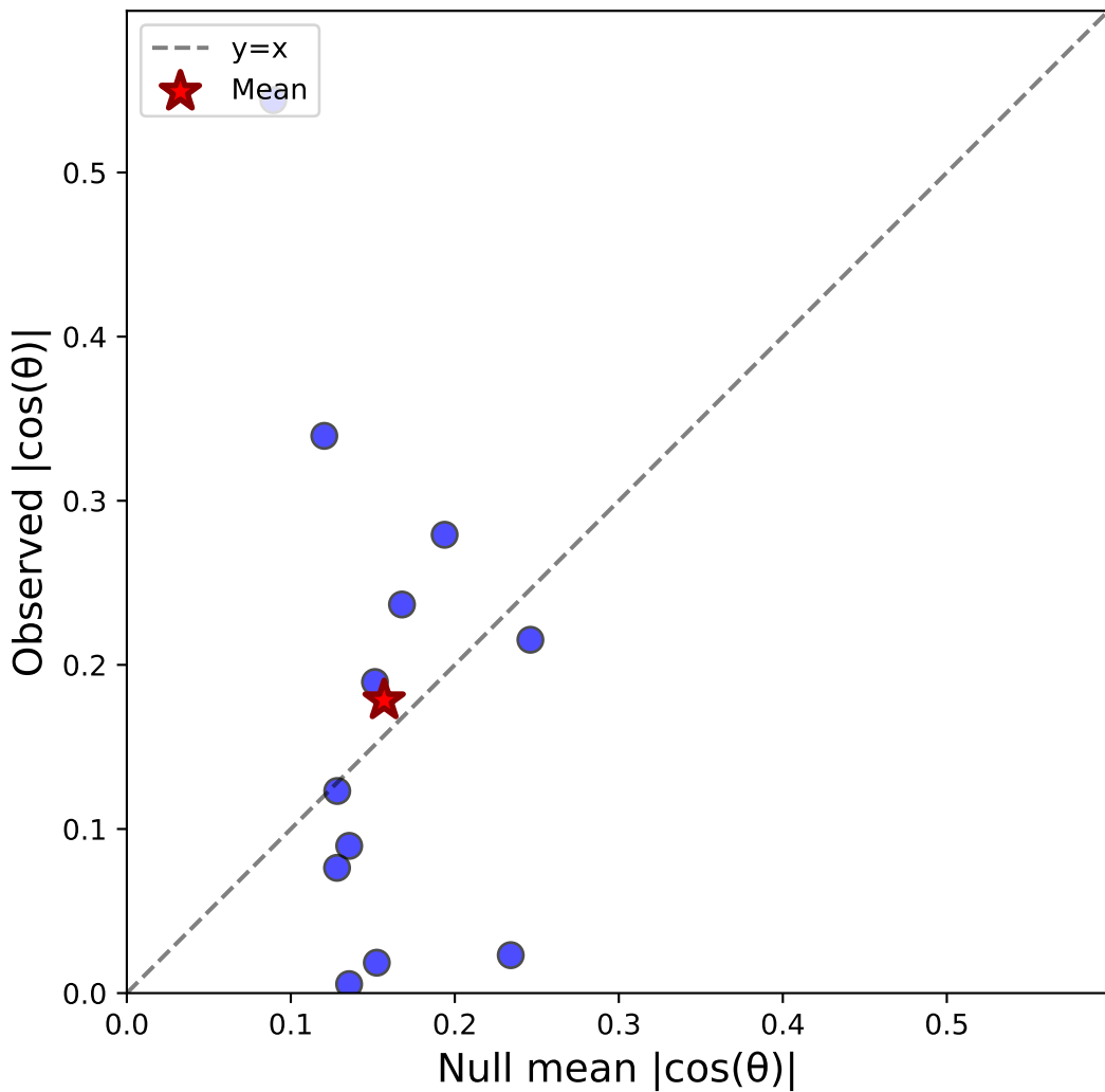
Case iv: Stim-C vs Sacc-S pooled (all) - Monkey S N=12 , \Delta=0.021\pm0.049
