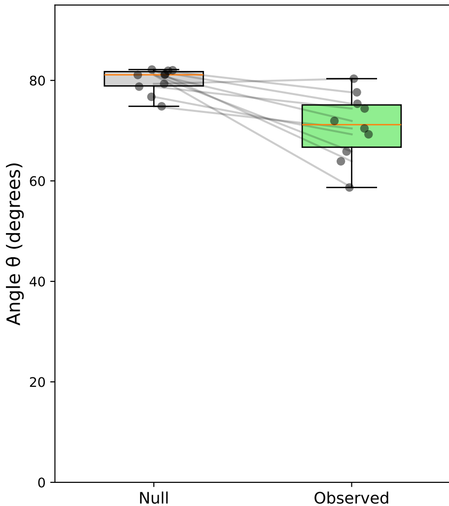
Case iii: Stim-C(vert) vs Sacc-S(horiz) (correct) - Monkey S \Delta\theta = -9.1^\circ
