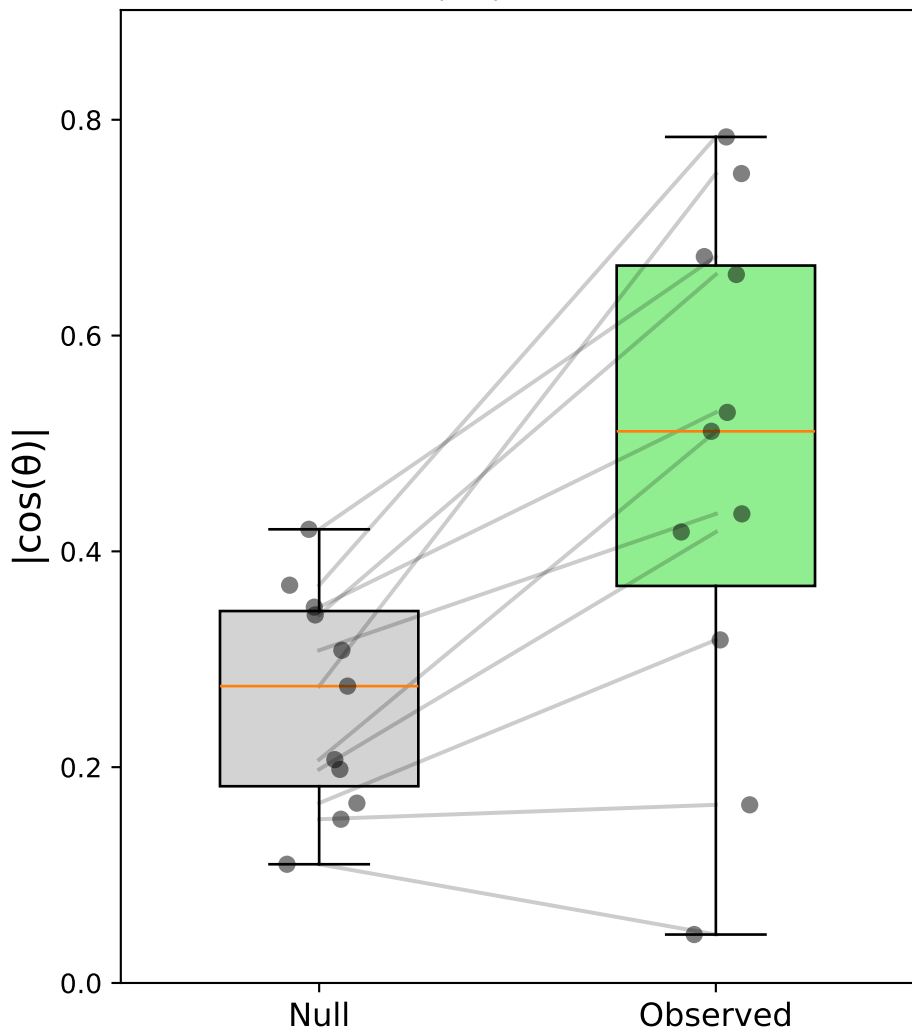
Case vi: Stim-C(ver) vs Sacc-S(horiz) - Monkey M \Delta|\cos| = 0.217
