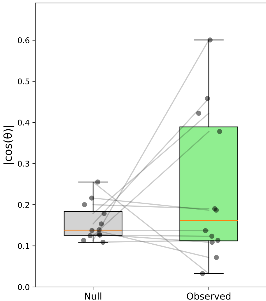
Case v: Stim-C(pool) vs Sacc-S(pool) - Monkey S \Delta|\cos| = 0.078
