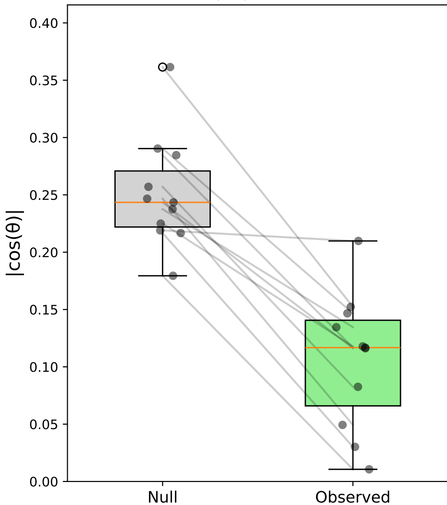
Case ii: Sacc C&S (pooled) - Monkey M \Delta|\cos| = -0.145
