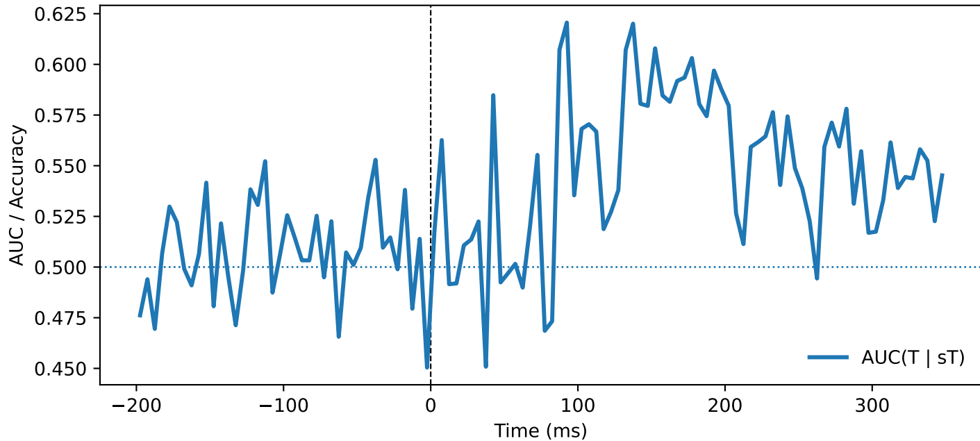
SLIP — QC (targ, ori=horizontal, PT \geq 200.0)
