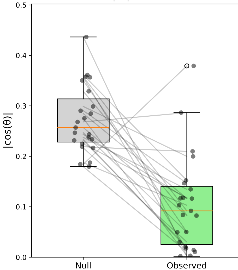
Case ii: Sacc C&S (pooled) - Monkey all \Delta|\cos| = -0.167
