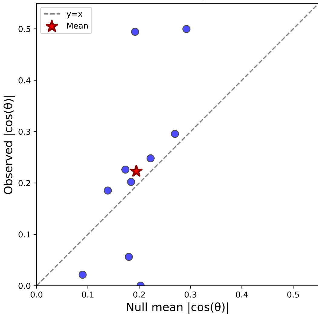
Case vi: Stim-C(vert) vs Sacc-S(horiz) - Monkey S N=10, \Delta=0.028 , Sig=1/10
