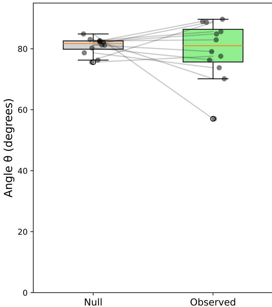
Case iv: Stim-C vs Sacc-S pooled (all) - Monkey S \Delta\theta = -1.3^\circ
