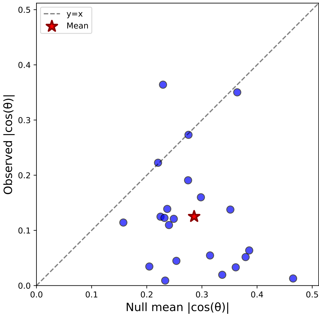
Case ii: Sacc C&S (pooled, correct) - Monkey all N=22, \Delta=-0.161
