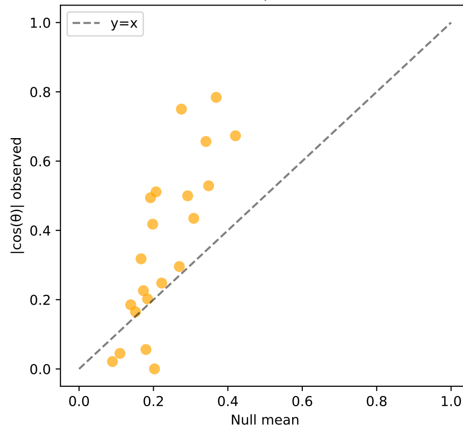
a_obs vs null_mean r=0.807 , p=0.0000
