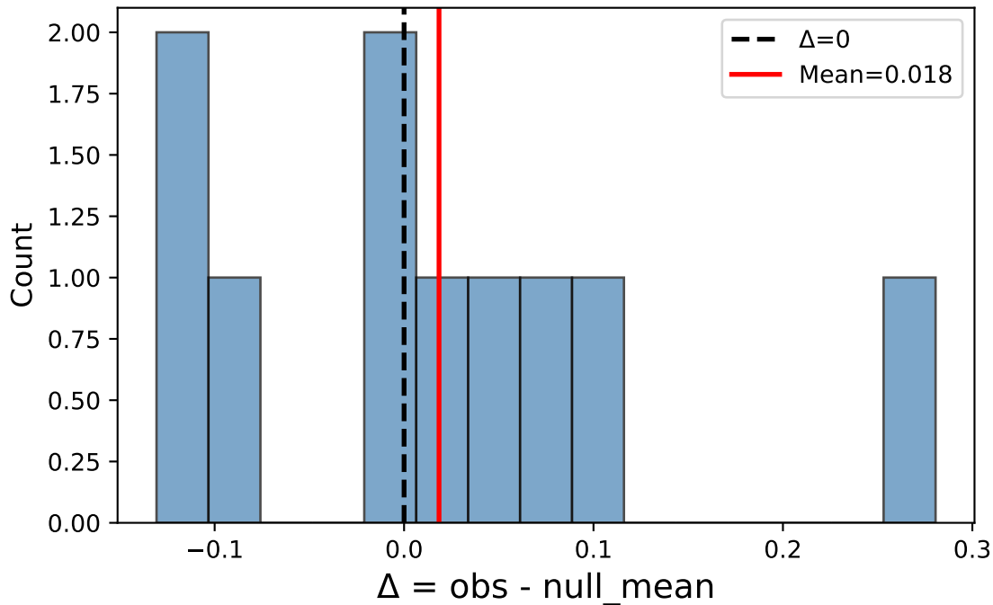
Monkey S: Effect Size Distribution
