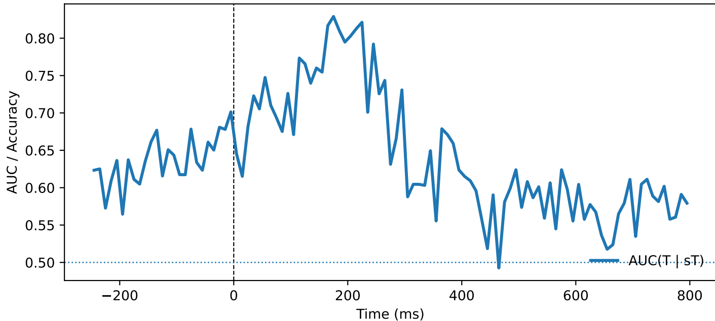
MLIP — QC (stim, ori=vertical, PT \geq 200.0)
