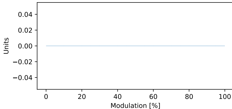
Target orientation modulation [%] (N=2020)
