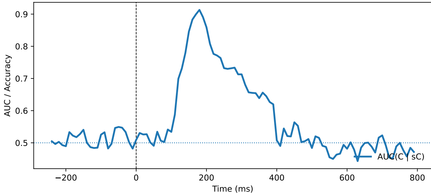
MFEF — QC (stim, ori=None, PT \geq 200.0, norm=global)
