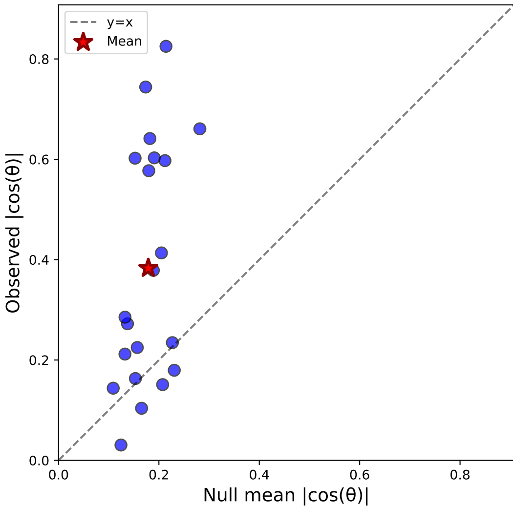
Case iii: Stim-C(ver) vs Sacc-S(horiz) (all) - Monkey all N=21, \Delta=0.204 , Sig=0/21
