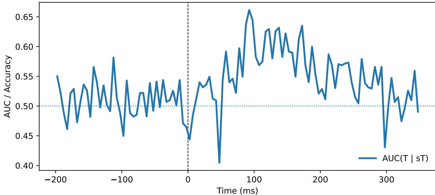
MSC — QC (targ, ori=vertical, PT \geq 200.0)
