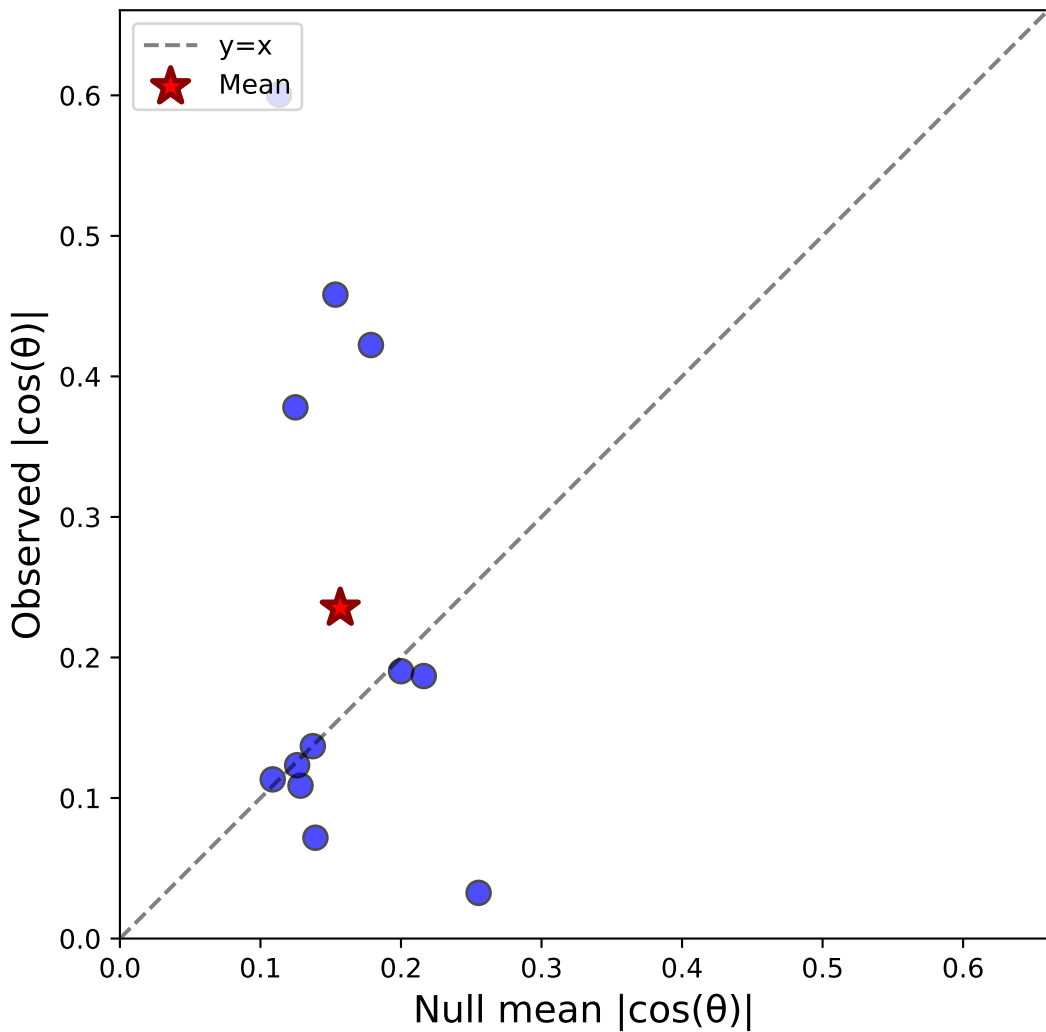
Case iv: Stim-C vs Sacc-S pooled (all) - Monkey S N=12, \Delta=0.078
