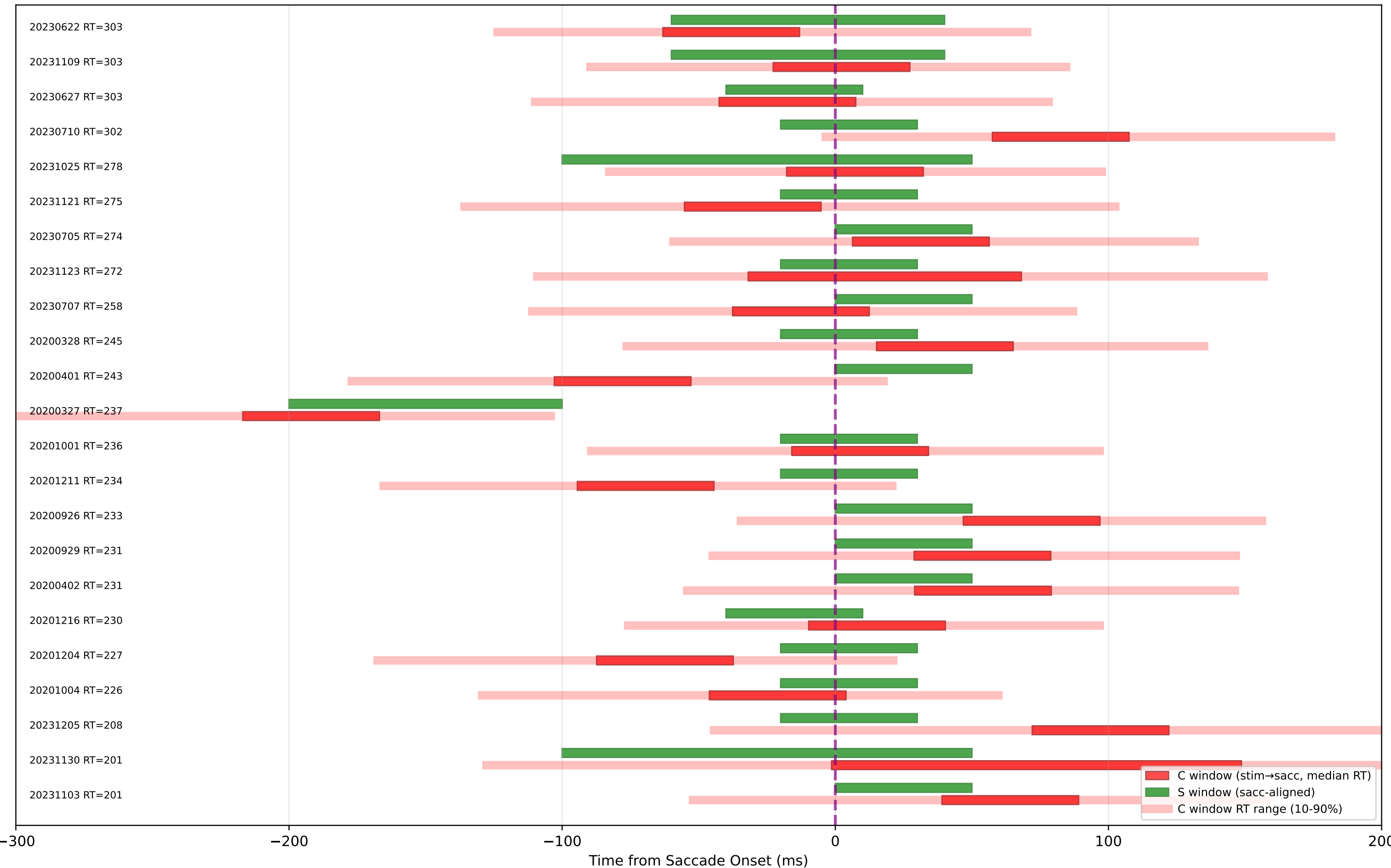
Case v: Stim-C & Sacc-S → Sacc Timeline (Pooled) (correctly)
