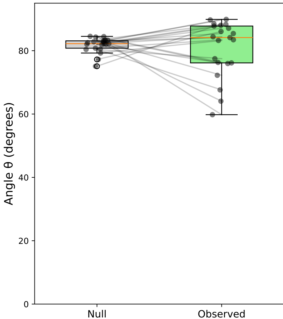
Case v: Stim-C(horiz) vs Sacc-S(horiz) (all) - Monkey all \Delta\theta = -1.1^\circ
