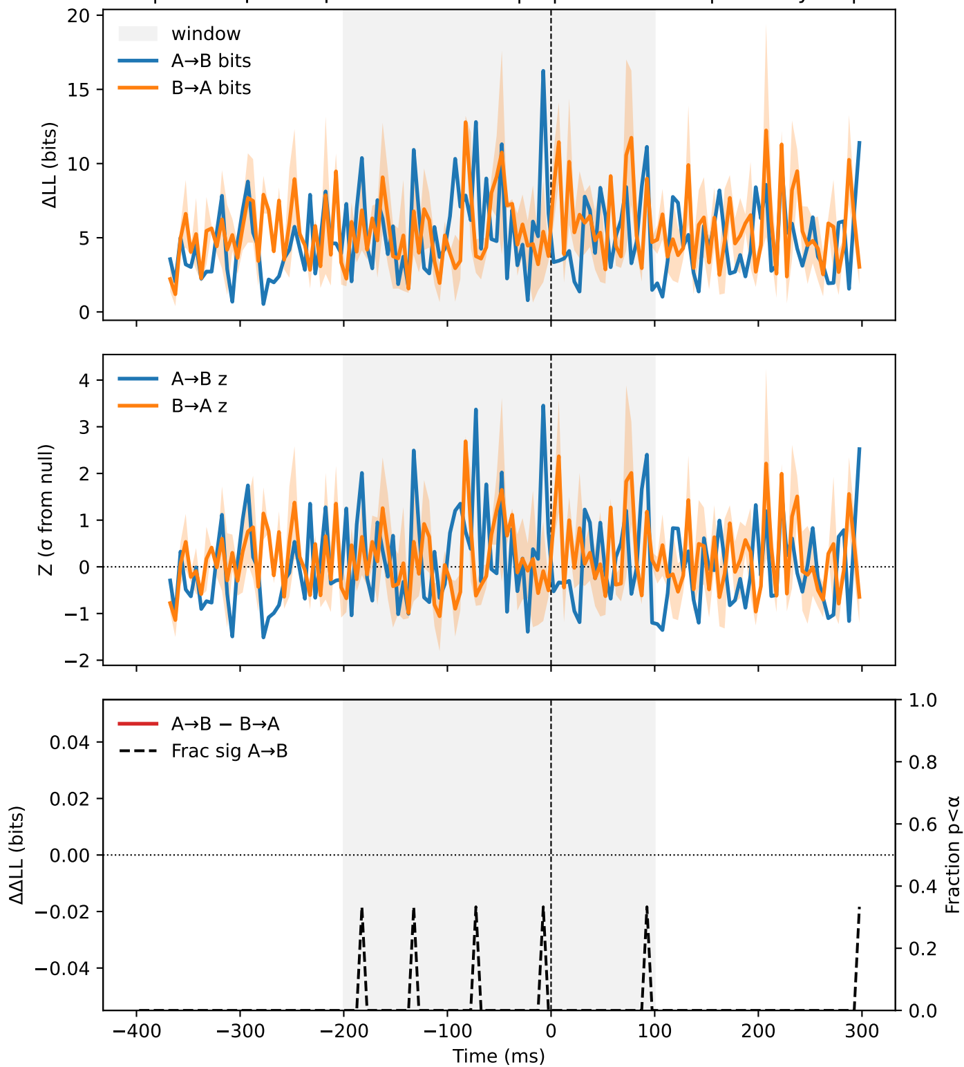
SACC | crsweep-sacc-pooled-none-circ | S | SFEF vs SSC | monkey=S | N=3
