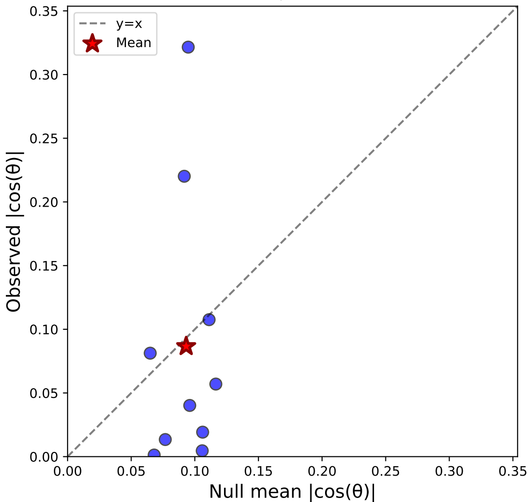
Monkey S: C-S Alignment in FEF N=10 sessions, \Delta = -0.007 \pm 0.032
