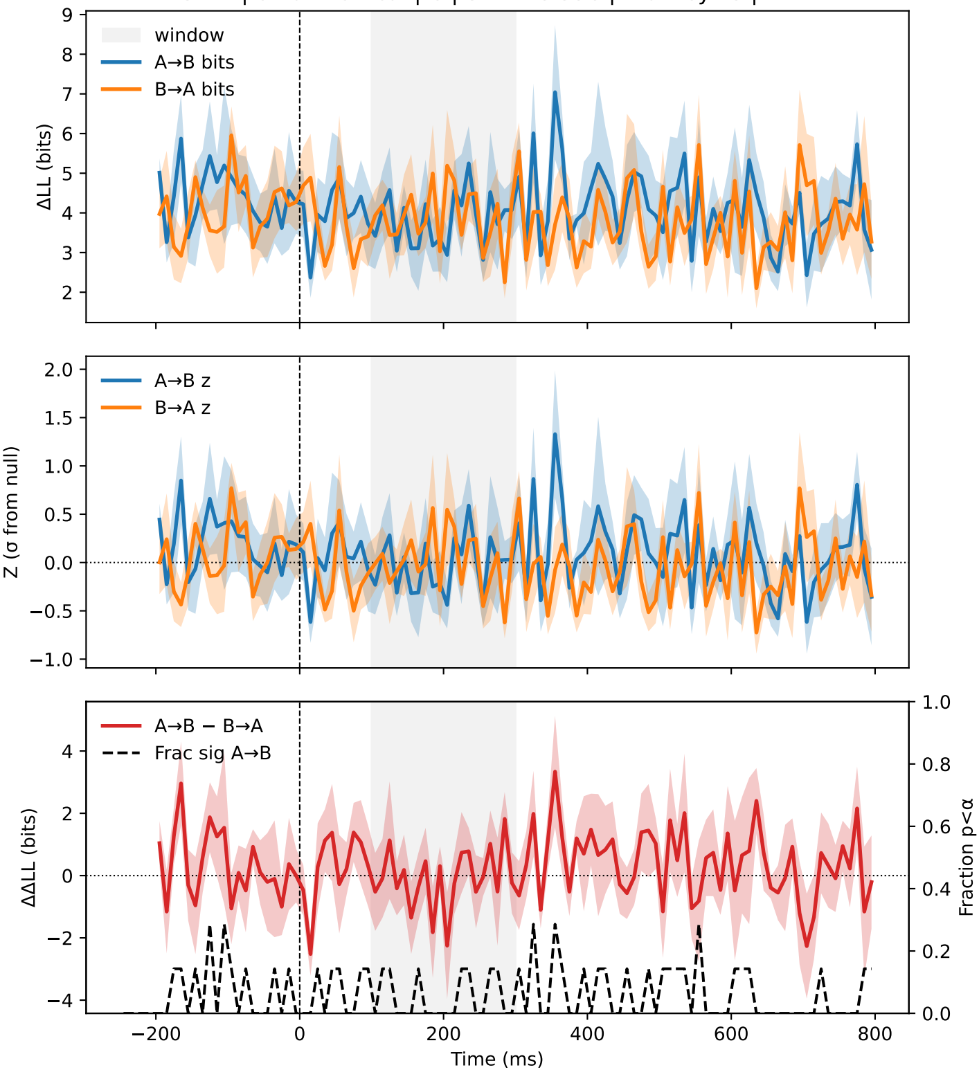
STIM | crnull-vertical | C | SFEF vs SSC | monkey=S | N=7
