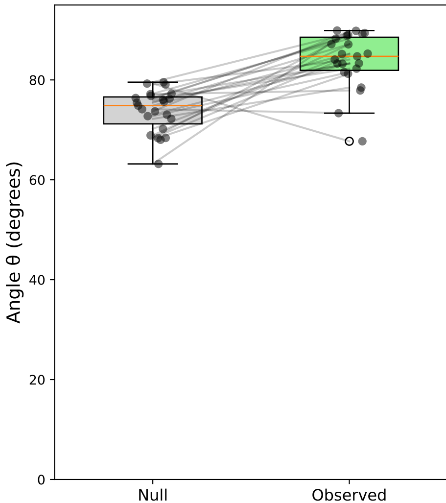
Case ii: Sacc C&S (pooled, all) - Monkey all \Delta\theta = 10.2^\circ
