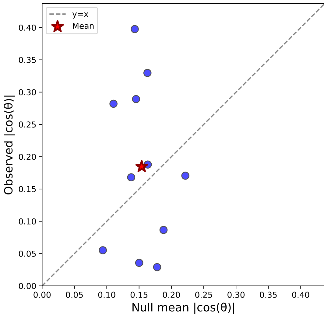
Case iv: Stim-C vs Sacc-S pooled (correct) - Monkey M N=11, \Delta=0.031
