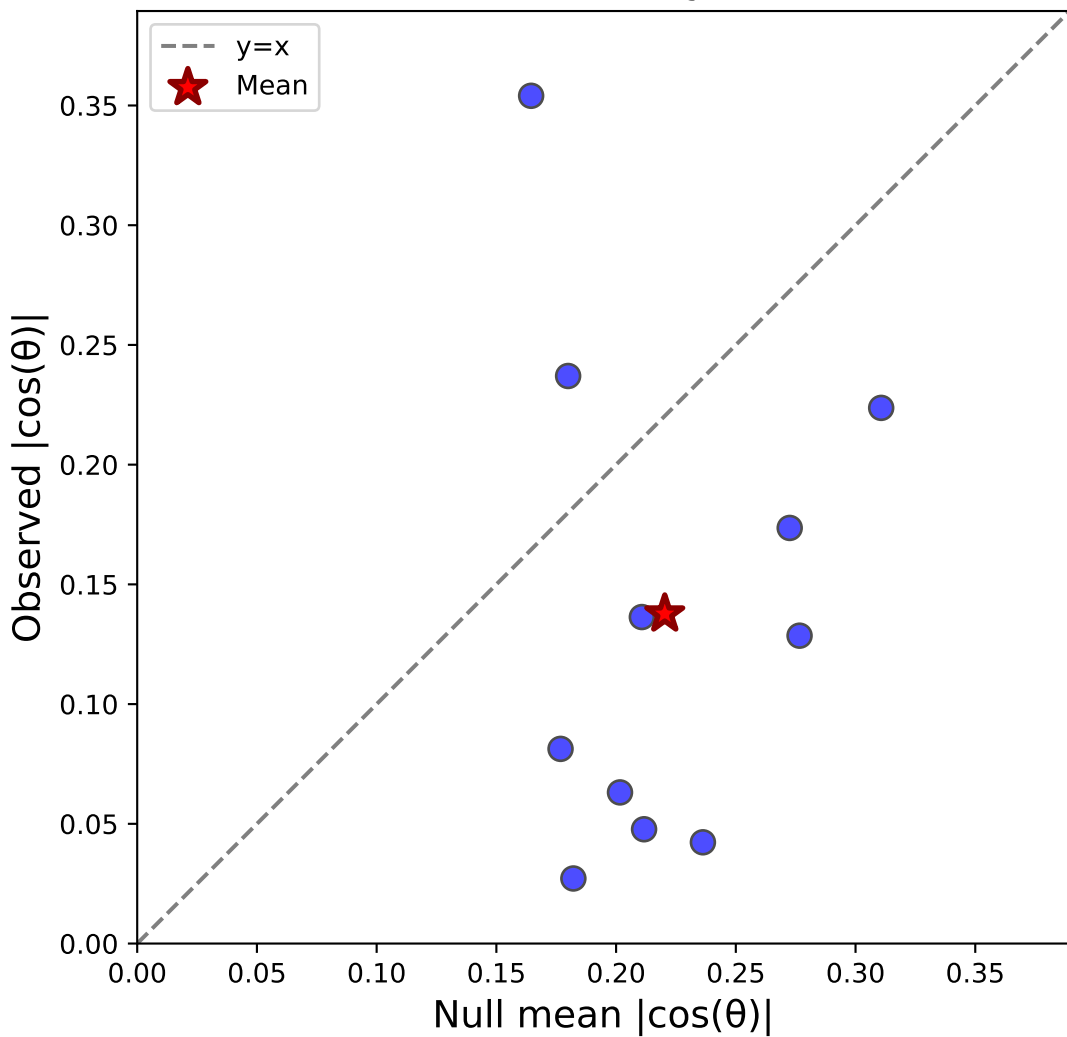
Case iv: Stim-C(horiz) vs Sacc-S(horiz) - Monkey M N=11, \Delta=-0.083 , Sig=0/11
