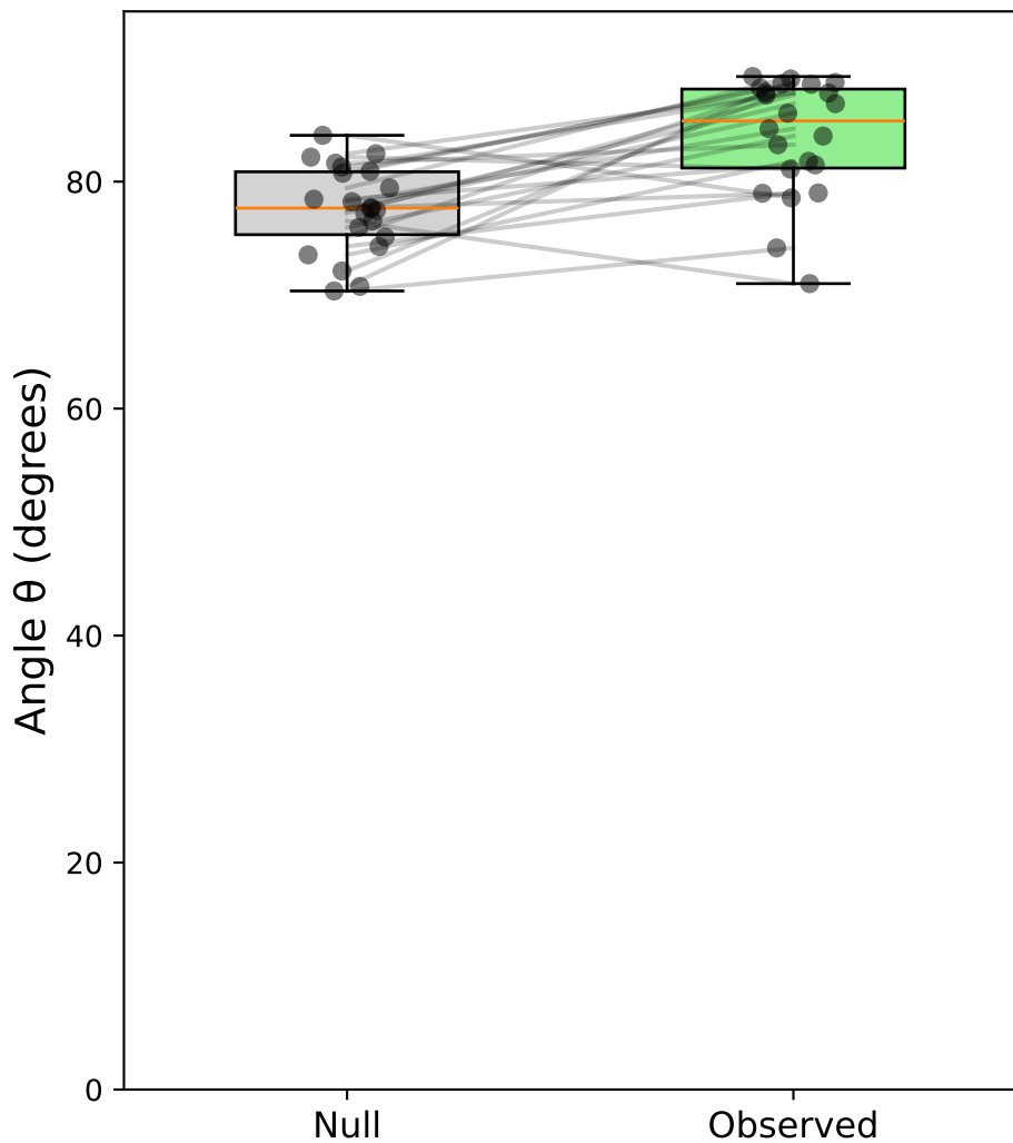
Case ii: Sacc C&S (pooled, correct) - Monkey all \Delta\theta = 6.3^\circ
