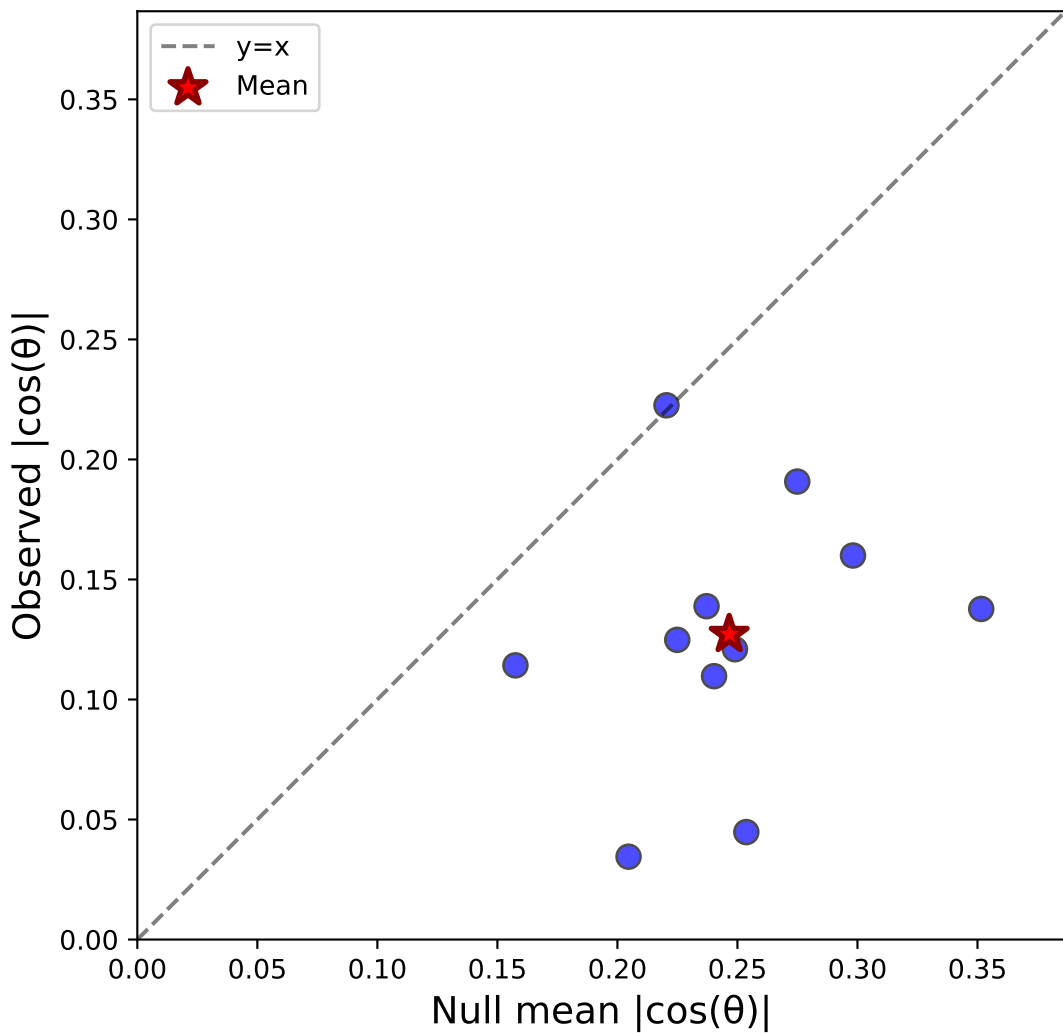
Case ii: Sacc C&S (pooled, correct) - Monkey M N=11, \Delta=-0.119
