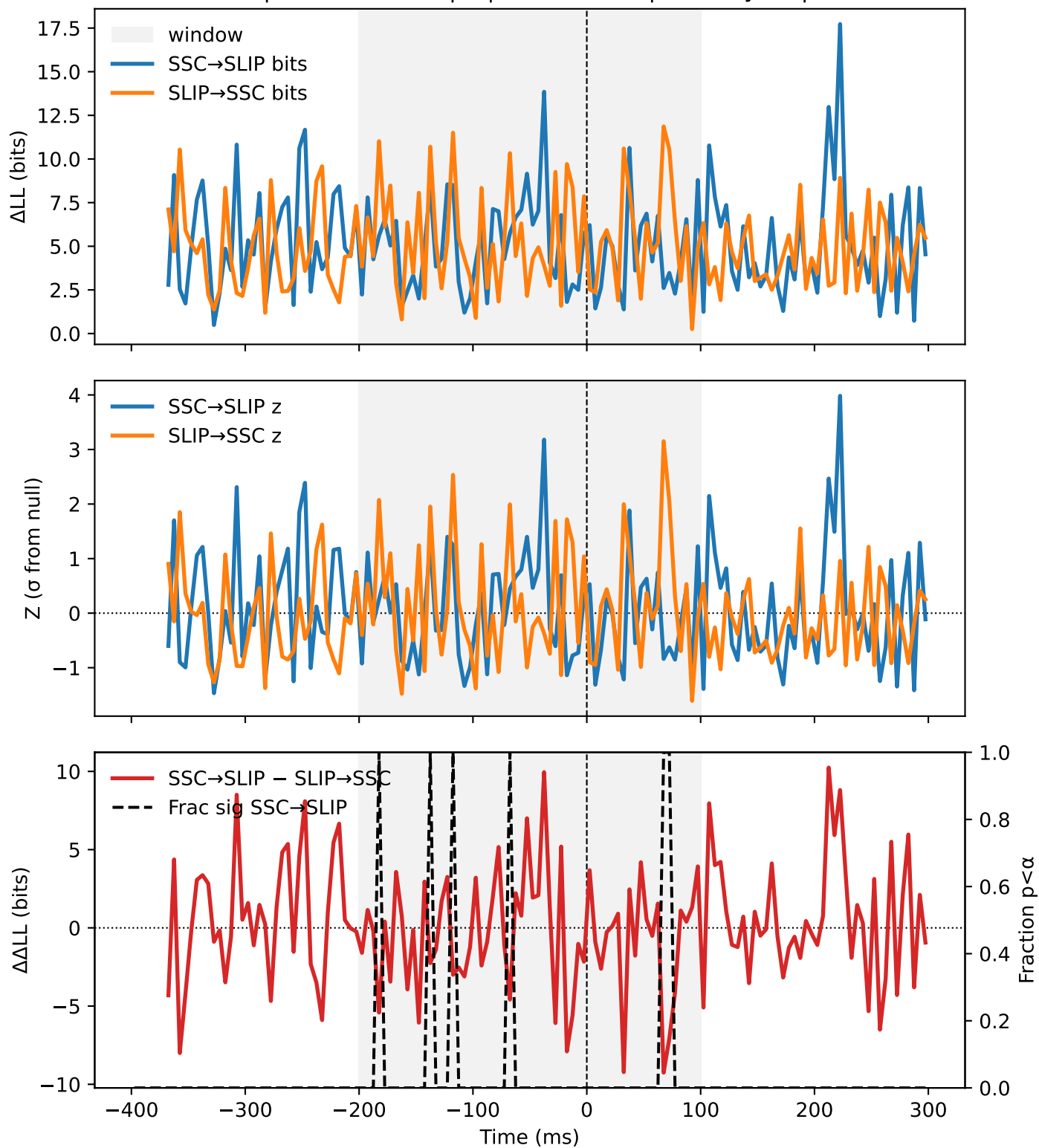
SACC | crnull-vertical | S | SSC vs SLIP | monkey=S | N=1
