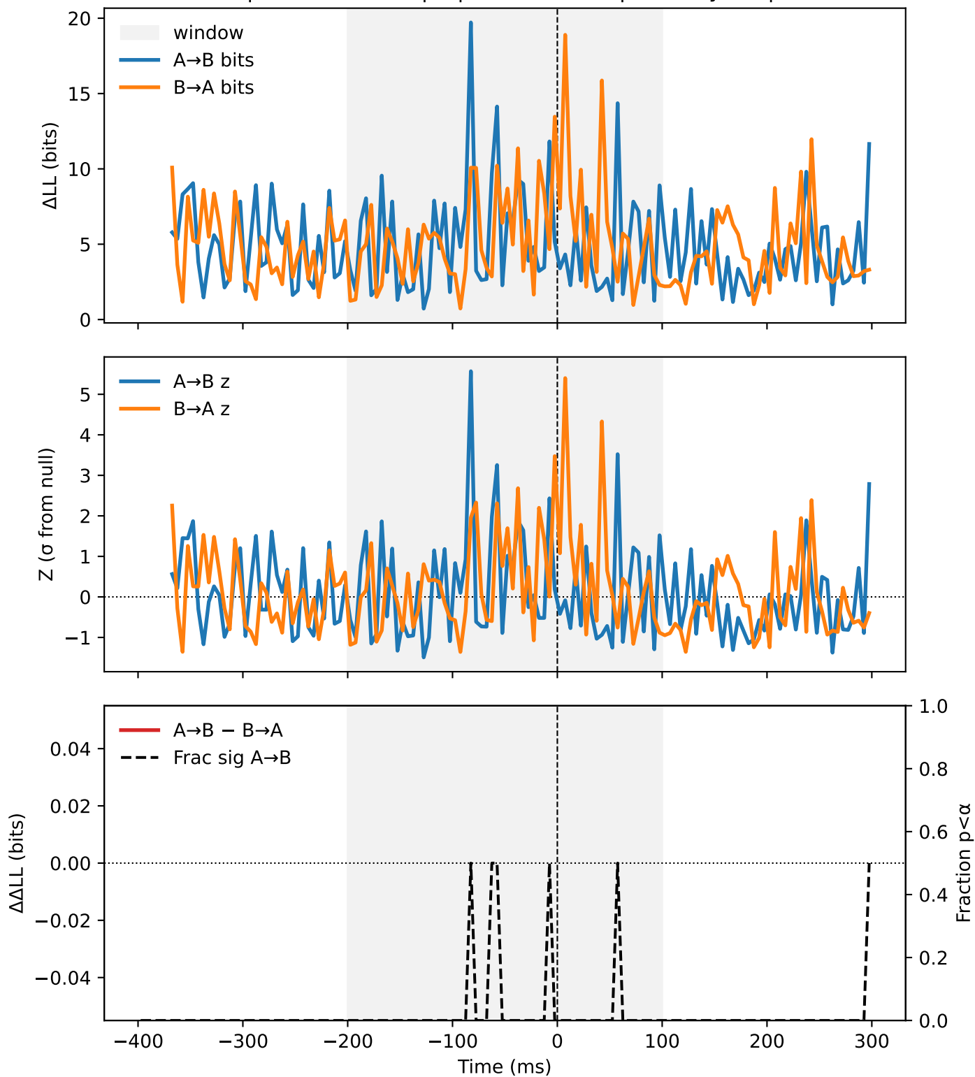
SACC | crnull-vertical | S | MLIP vs MSC | monkey=M | N=2
