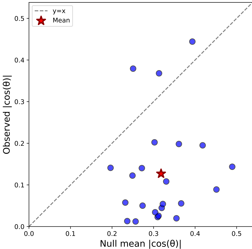
Case iii: Sacc C&S (vert) - Monkey all N=23, \Delta=-0.191 , Sig=4/23
