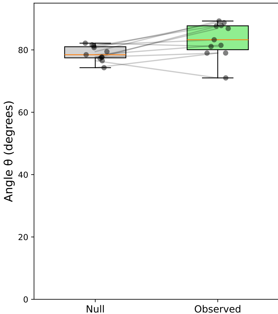
Case ii: Sacc C&S (pooled, correct) - Monkey M \Delta\theta = 4.4^\circ
