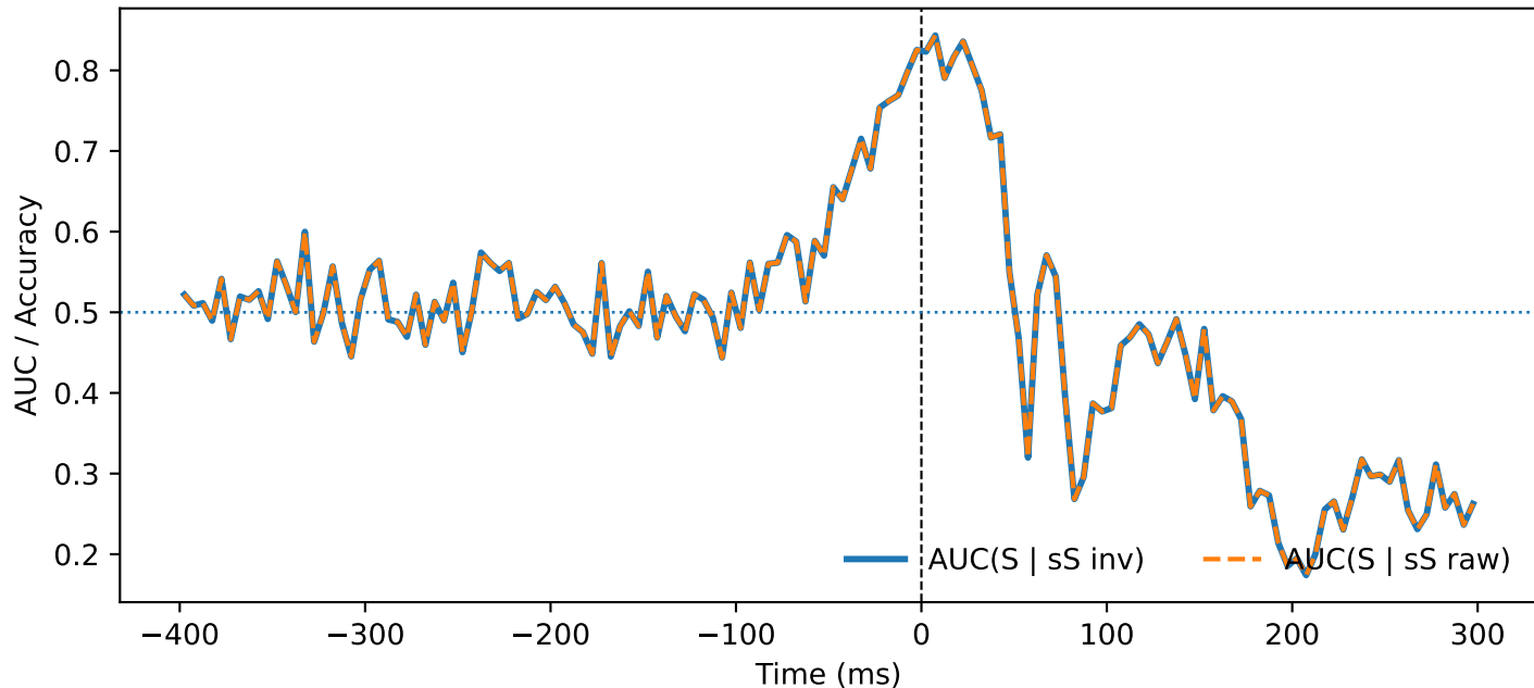
MLIP — QC (sacc, ori=vertical, PT \geq 200.0, norm=global)
