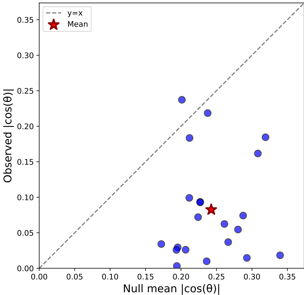
Case i: Sacc C&S (horiz, all) - Monkey all N=21, \Delta=-0.160
