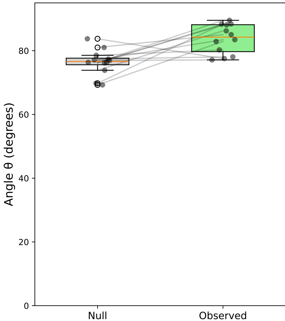
Case ii: Sacc C&S (pooled, all) - Monkey S \Delta\theta = 7.4^\circ
