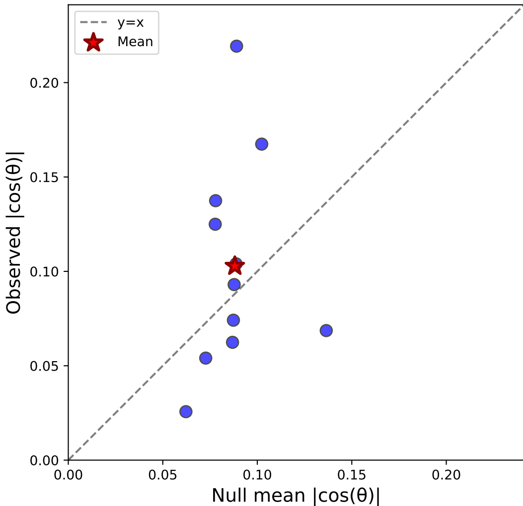
Monkey M: C-S Alignment in FEF N=11 sessions, \Delta=0.015\pm0.016
