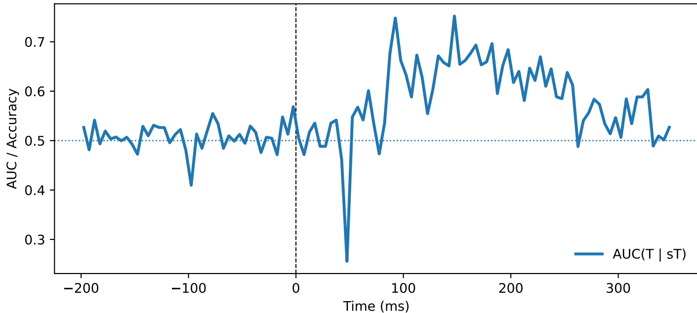
MLIP — QC (targ, ori=horizontal, PT \geq 200.0)
