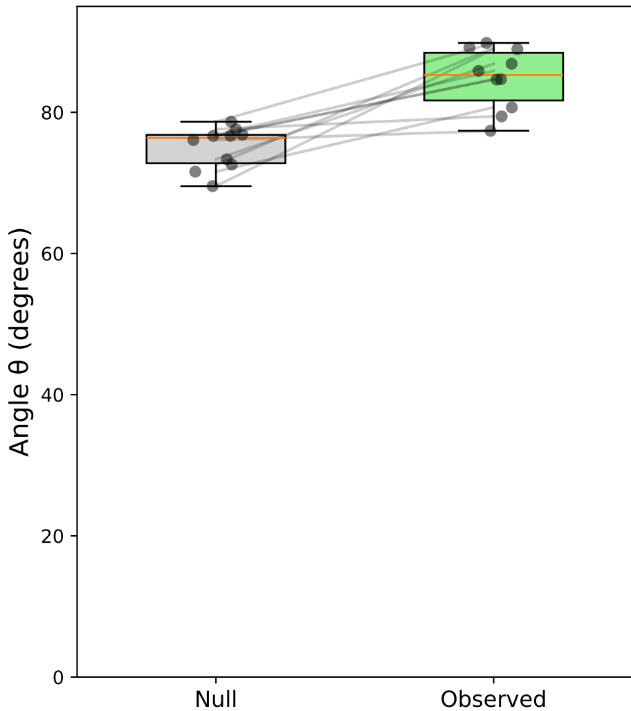
Case i: Sacc C&S (horiz, all) - Monkey S \Delta\theta = 9.8^\circ
