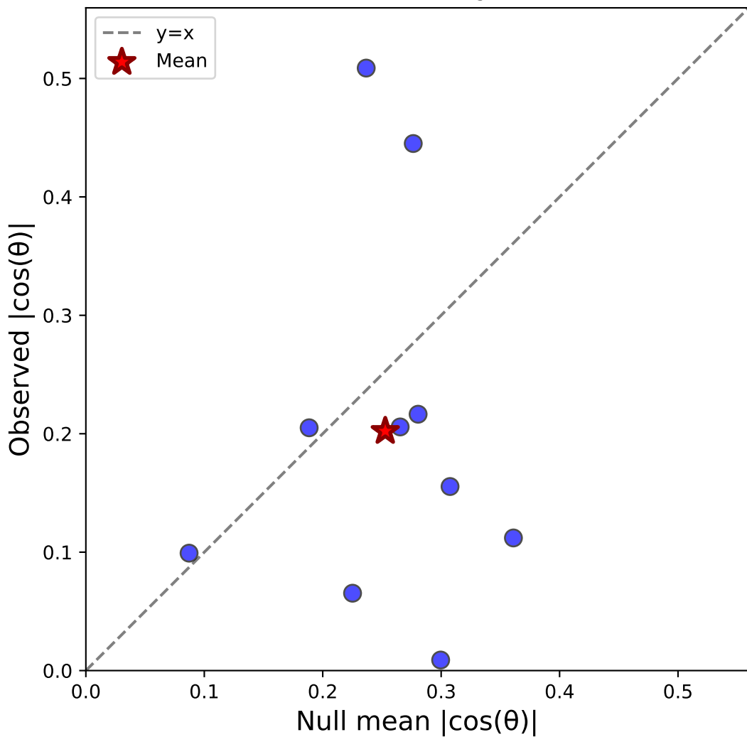
Case iv: Stim-C(horiz) vs Sacc-S(horiz) - Monkey S N=10, \Delta=-0.051 , Sig=1/10
