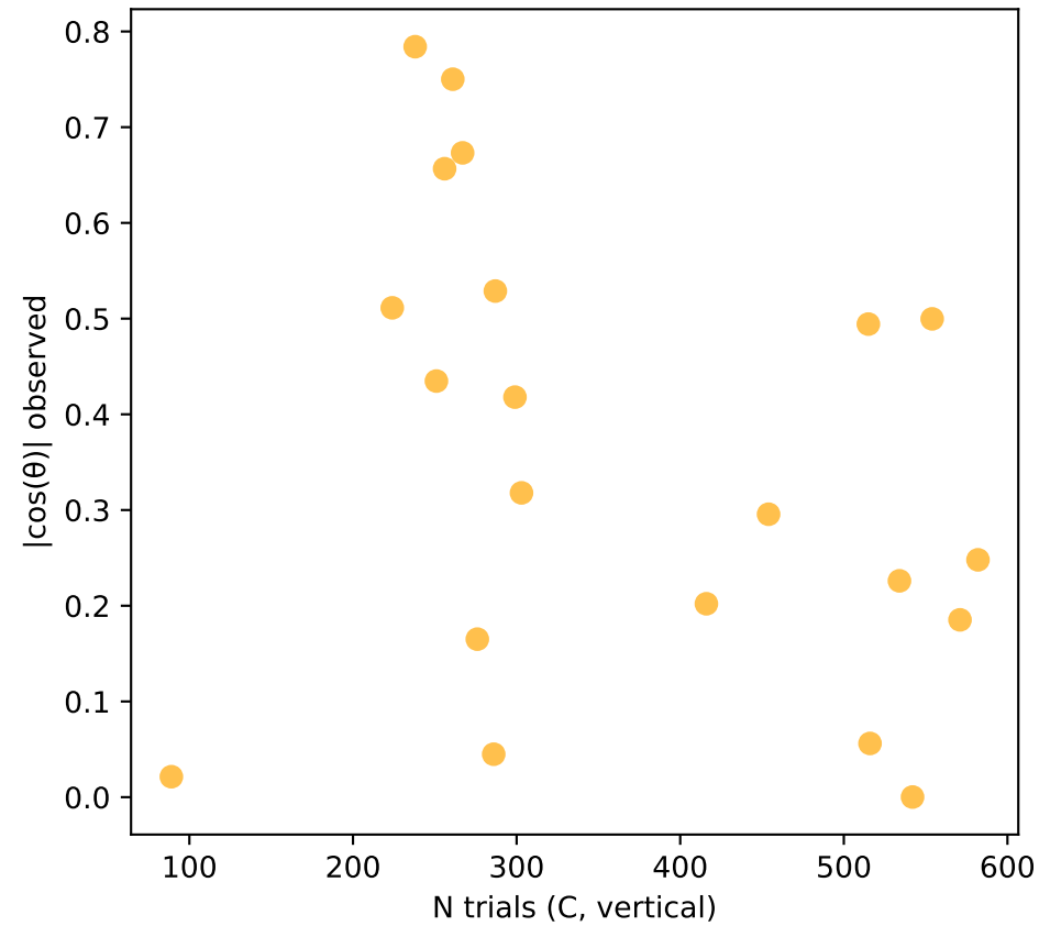
a_obs vs n_trials_C r=-0.318 , p=0.1604
