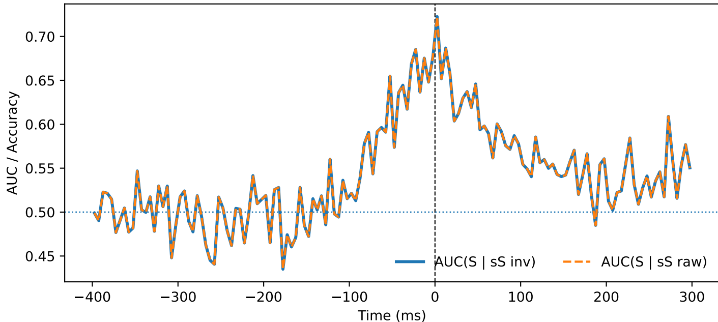
SFEF — QC (sacc, ori=vertical, PT \geq 200.0, norm=global)
