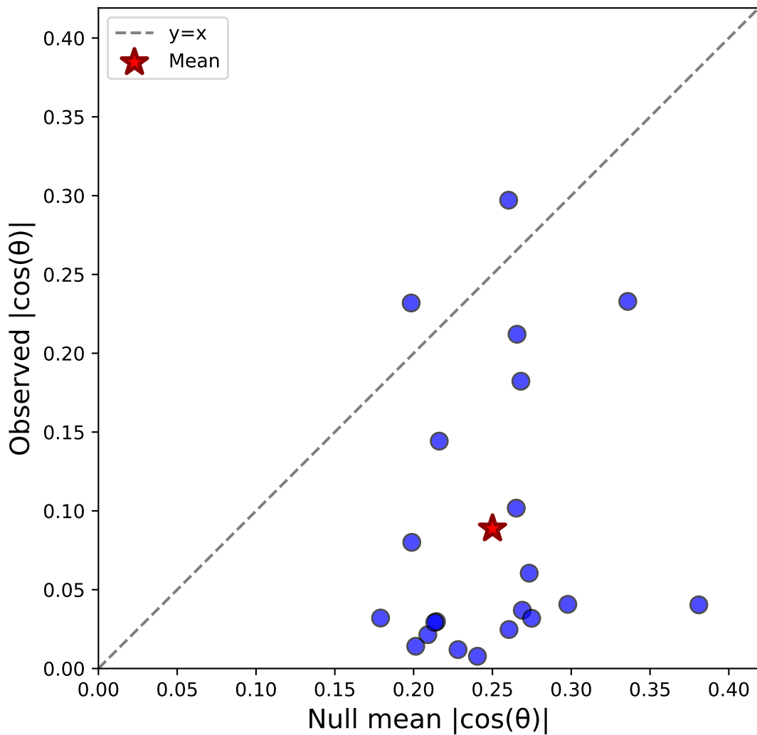
Case i: Sacc C&S (horiz, correct) - Monkey all N=21, \Delta=-0.161
