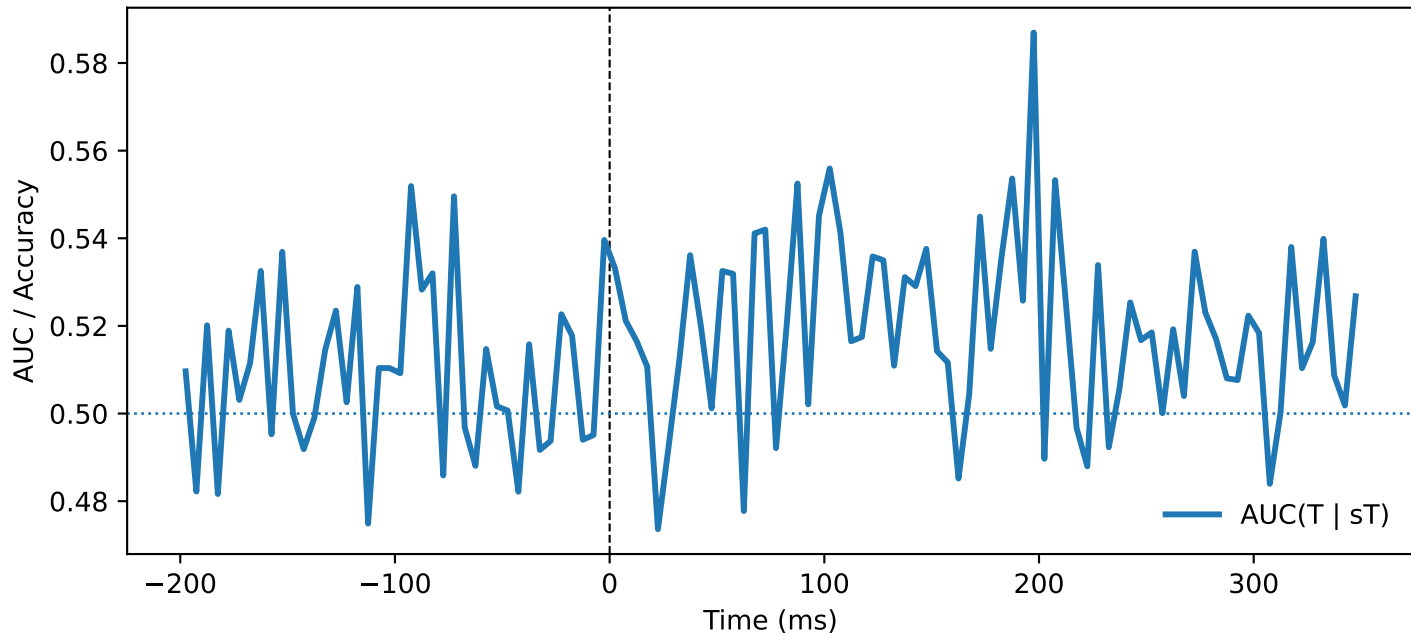
SFEF — QC (targ, ori=None, PT \geq 200.0)
