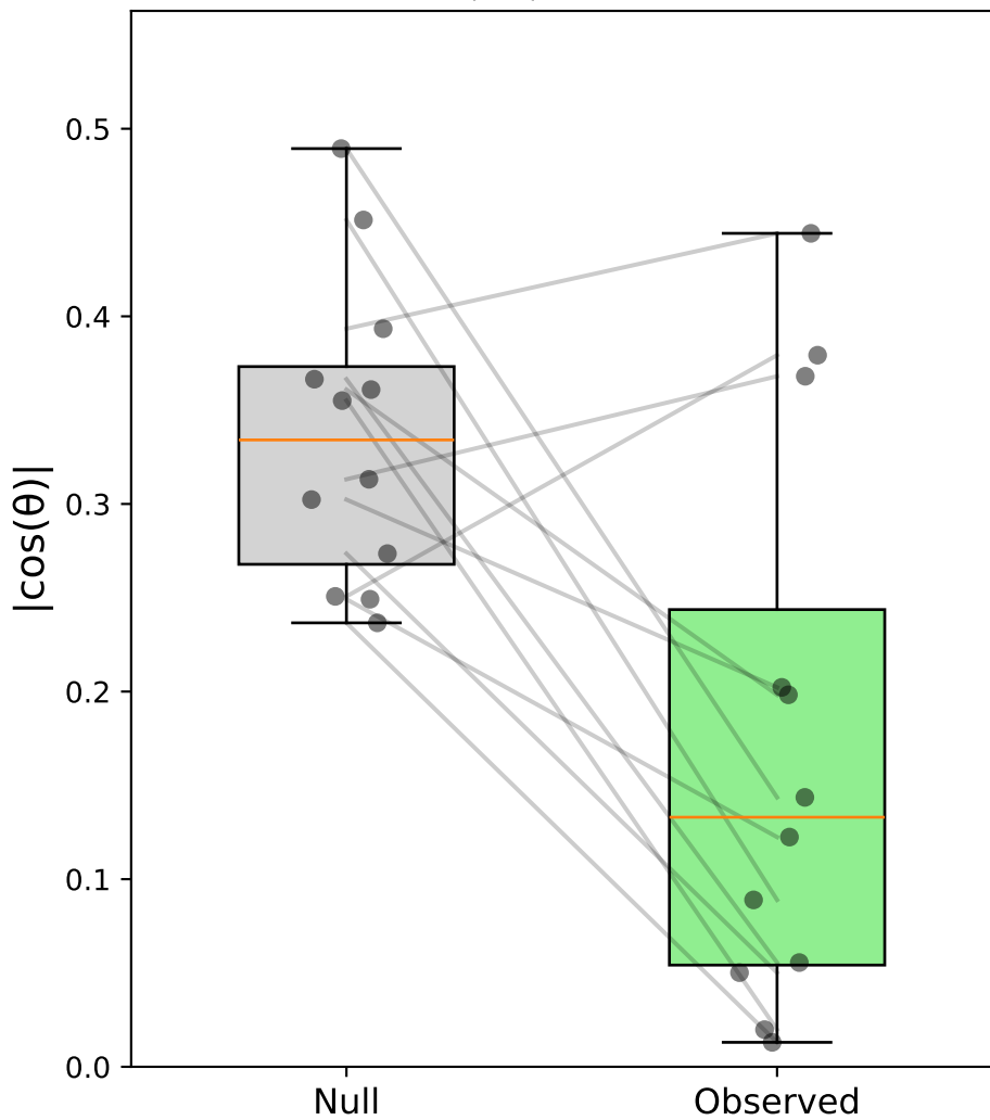
Case iii: Sacc C&S (vert) - Monkey S \Delta|\cos| = -0.163
