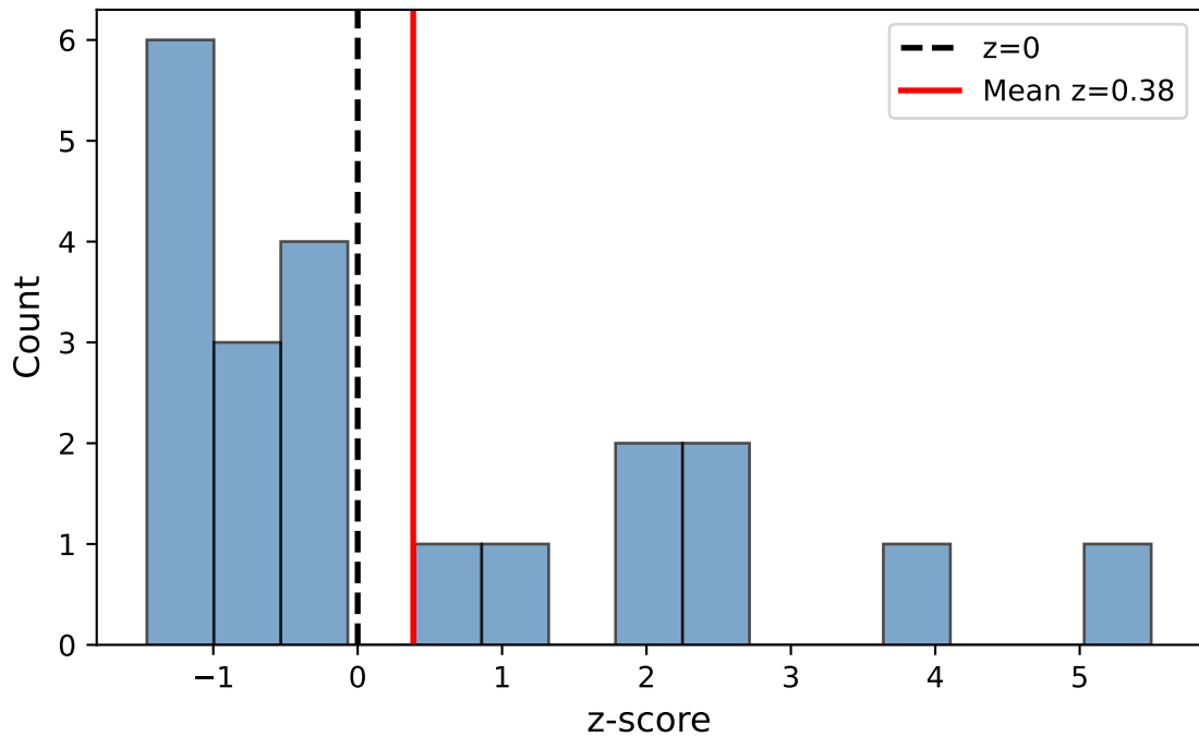
Case iv: Stim-C(horiz) vs Sacc-S(horiz) - Monkey all
