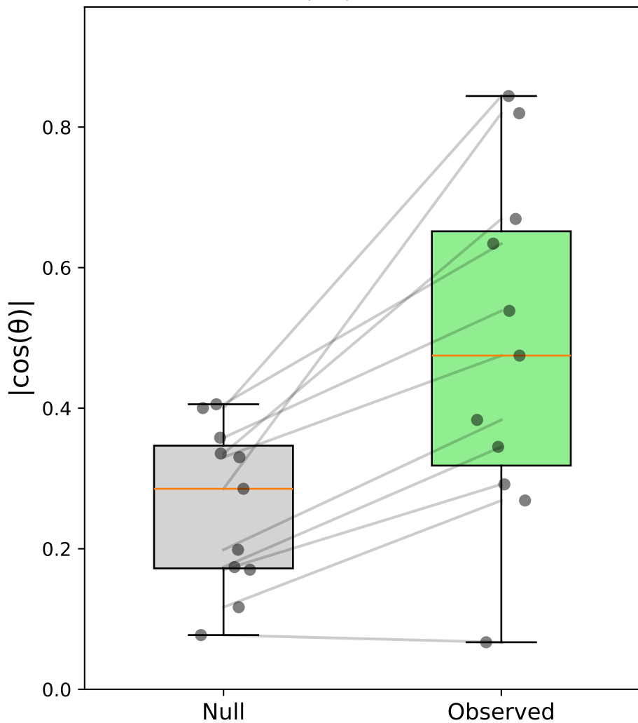
Case vi: Stim-C(ver) vs Sacc-S(horiz) - Monkey M \Delta|\cos| = 0.226
