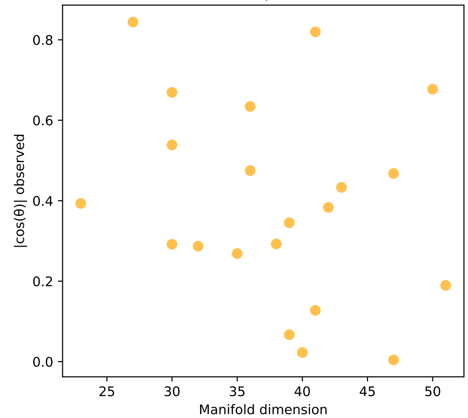
a_obs vs manifold_dim r=-0.264 , p=0.2473
