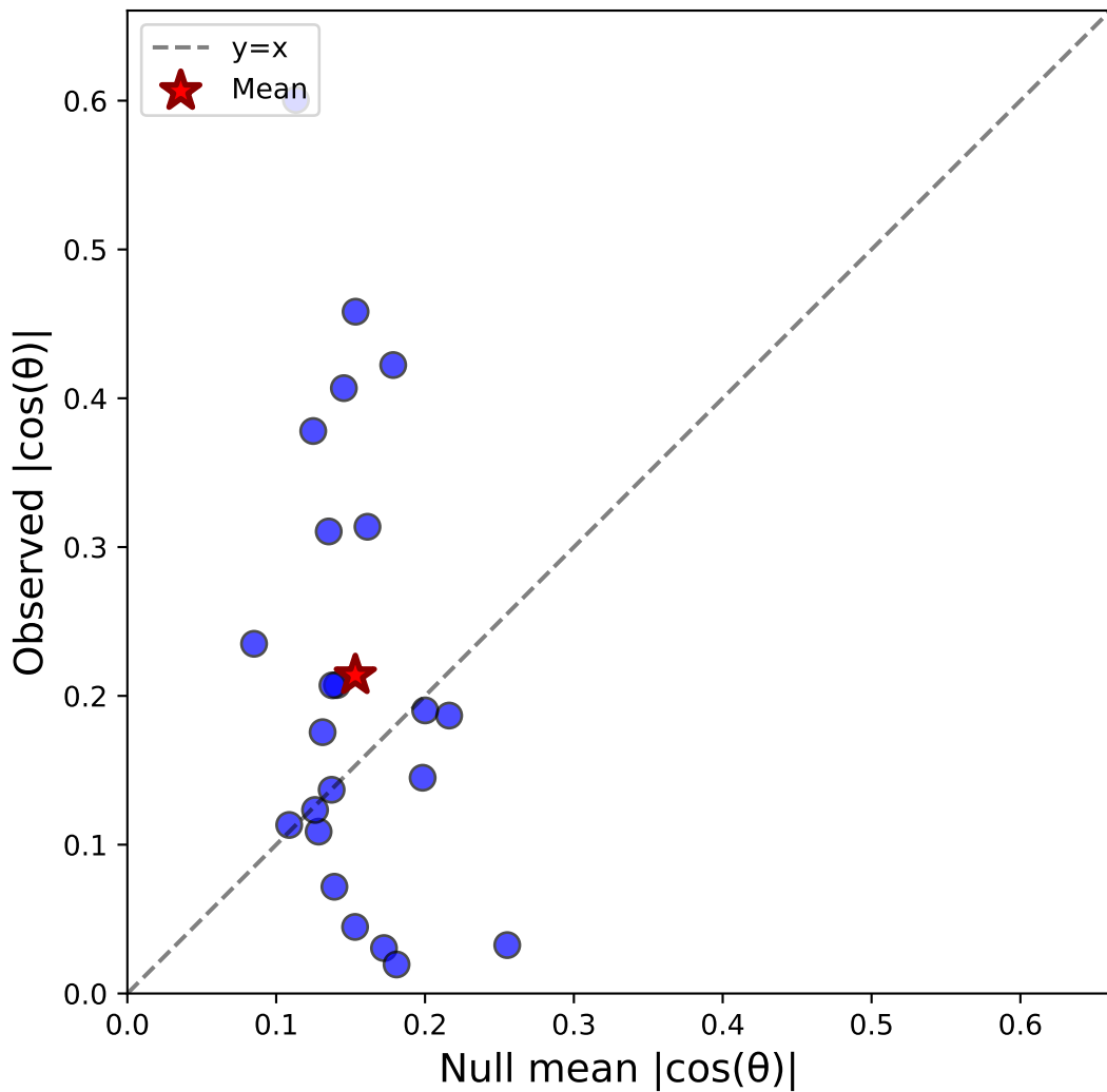
Case v: Stim-C(pool) vs Sacc-S(pool) - Monkey all N=23, \Delta=0.061 , Sig=0/23
