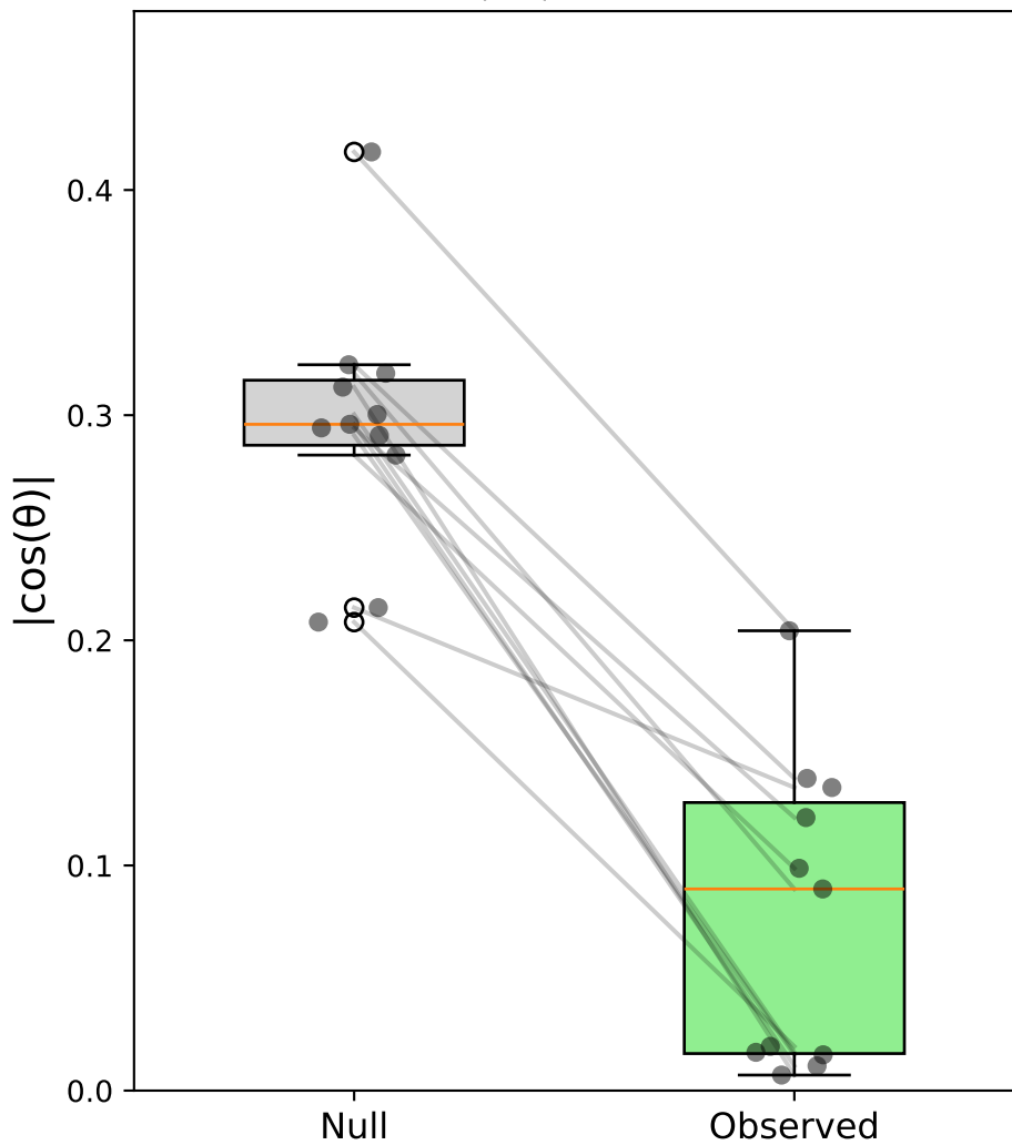
Case vi: Sacc C&S (vert, all) - Monkey M \Delta|\cos| = -0.218
