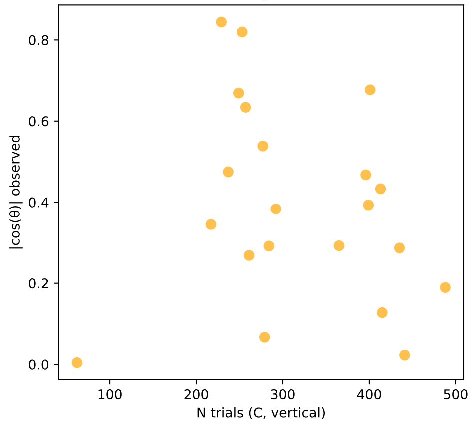
a_obs vs n_trials_C r=-0.153 , p=0.5089
