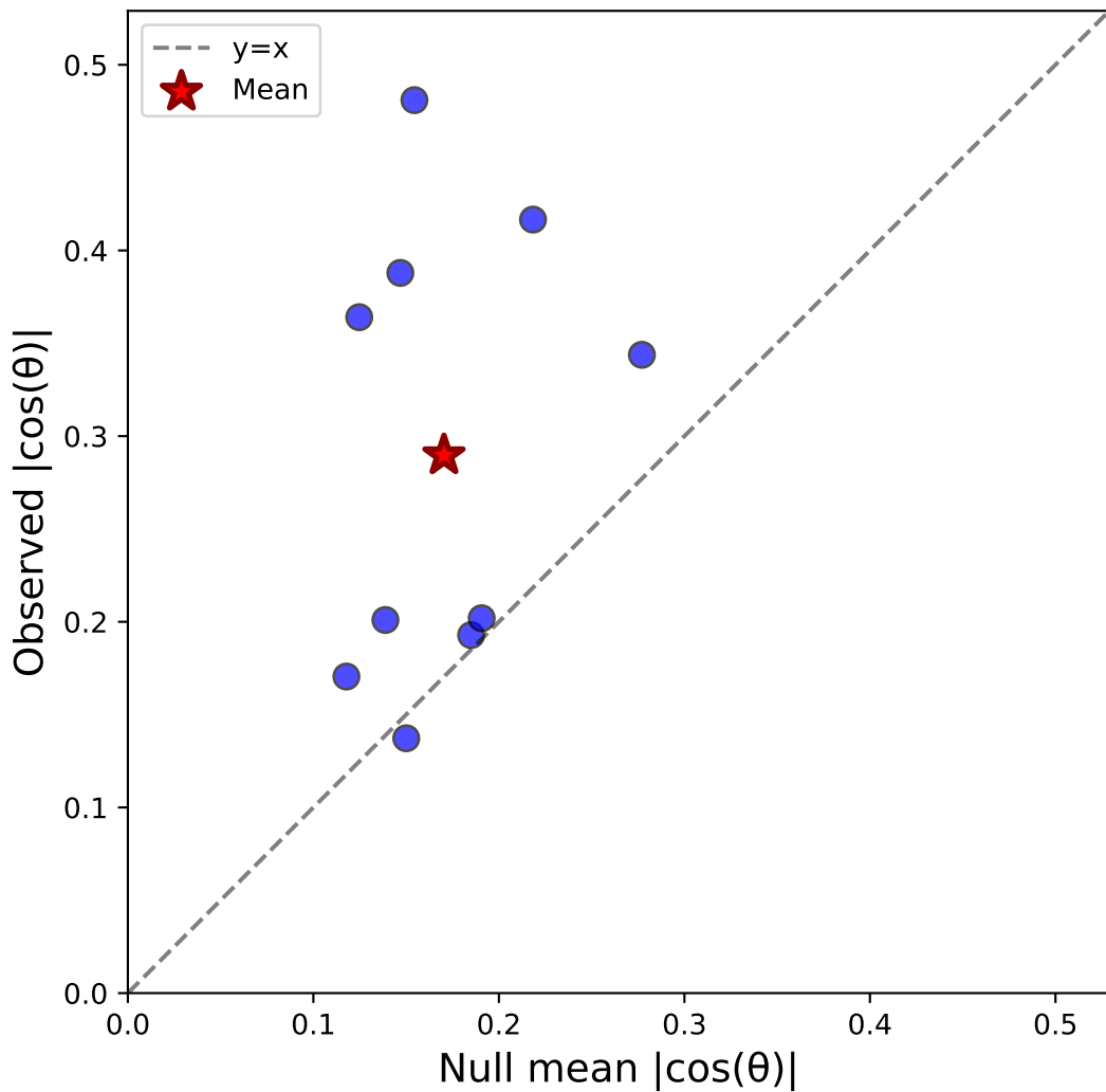
Case iii: Stim-C vs Sacc-S (correct) - Monkey S N=10 , \Delta=0.119\pm0.036
