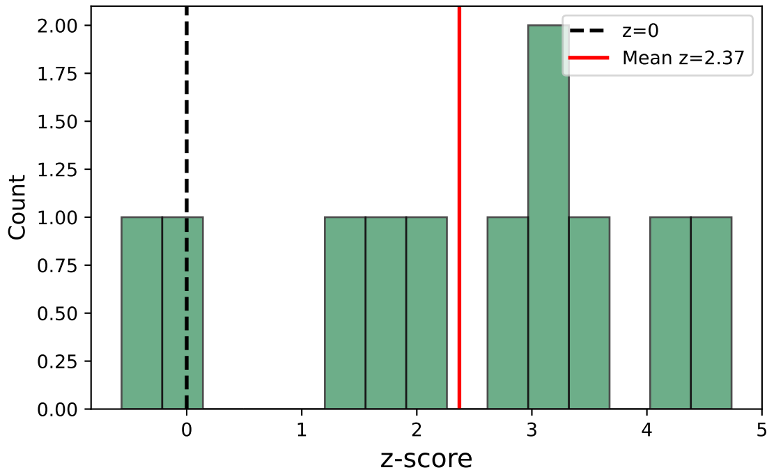
Case iii: Stim-C(ver) vs Sacc-S(horiz) (all) - Monkey M
