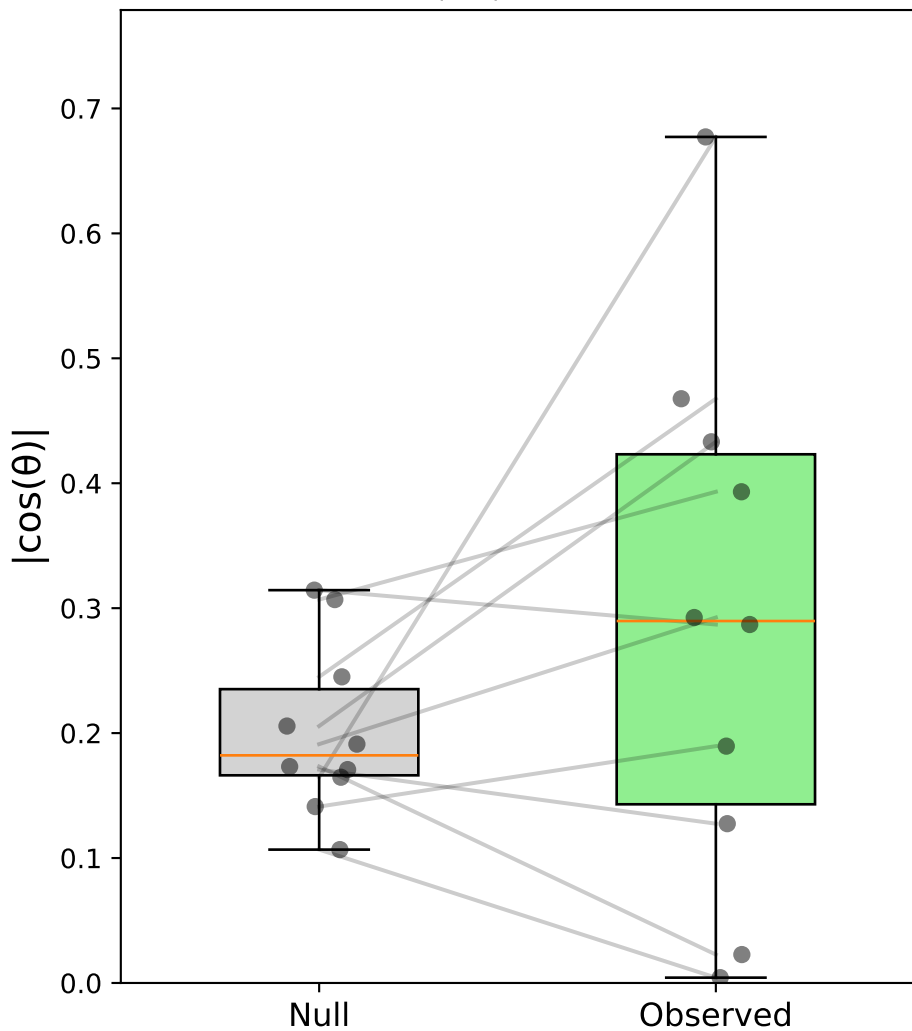
Case vi: Stim-C(ver) vs Sacc-S(horiz) - Monkey S \Delta|\cos| = 0.087
