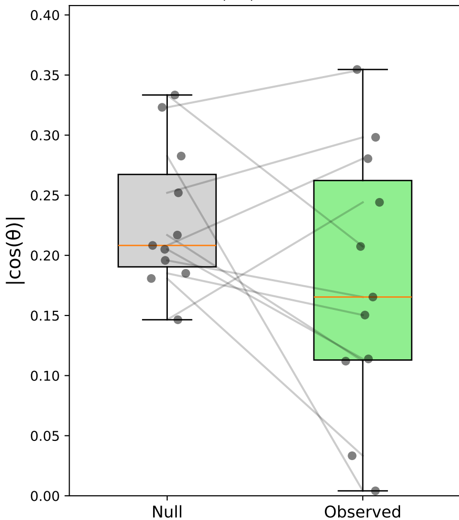
Case v: Stim-C(pool) vs Sacc-S(pool) - Monkey M \Delta|\cos| = -0.051
