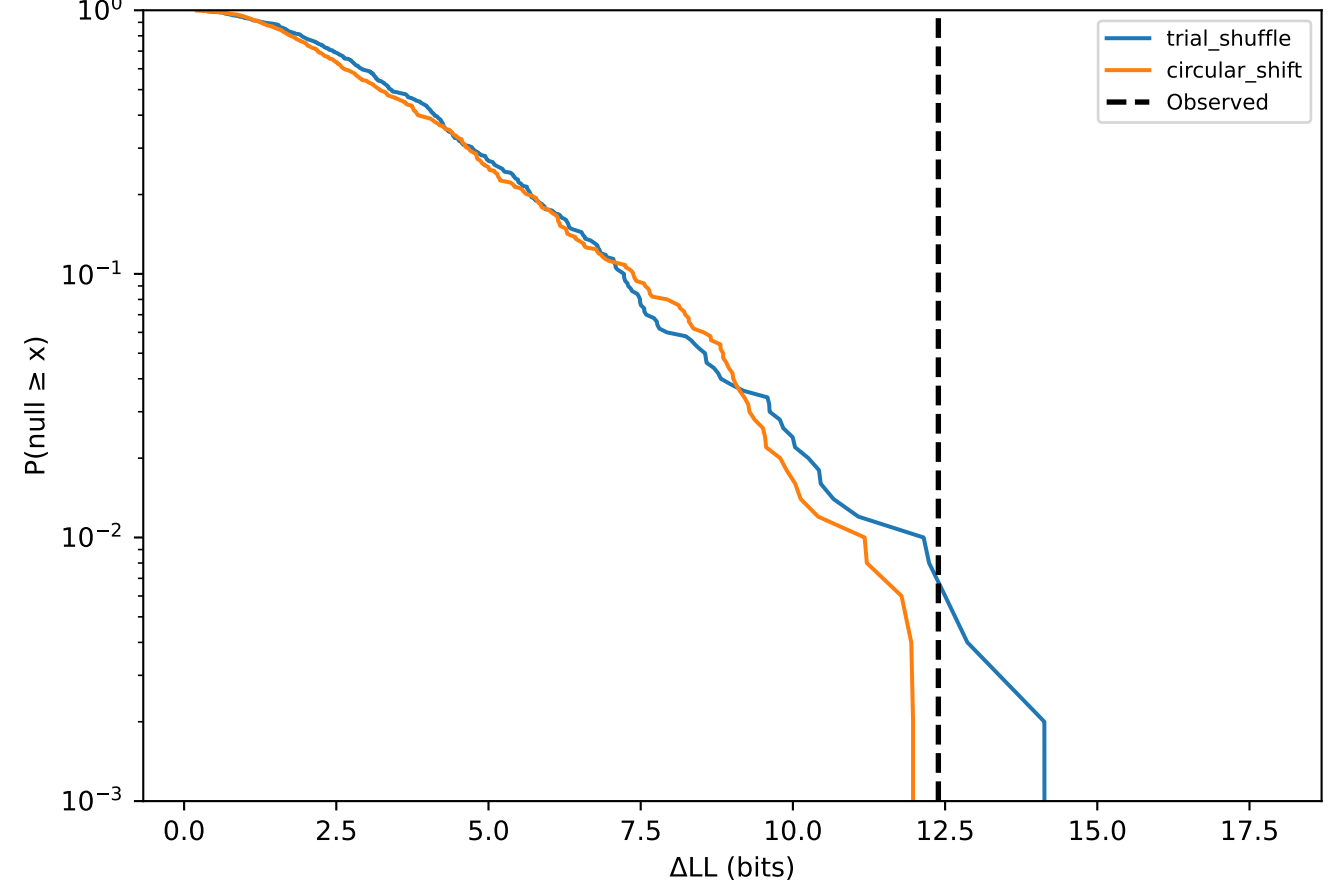
Tail Probabilities at Peak (t=65 ms)
