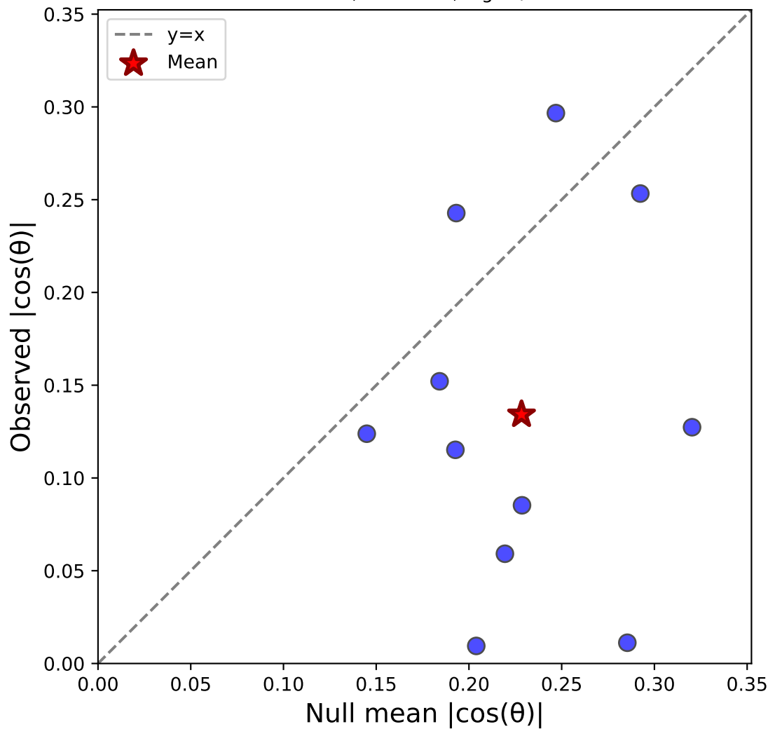
Case v: Stim-C(pool) vs Sacc-S(pool) - Monkey M N=11, \Delta=-0.094 , Sig=2/11
