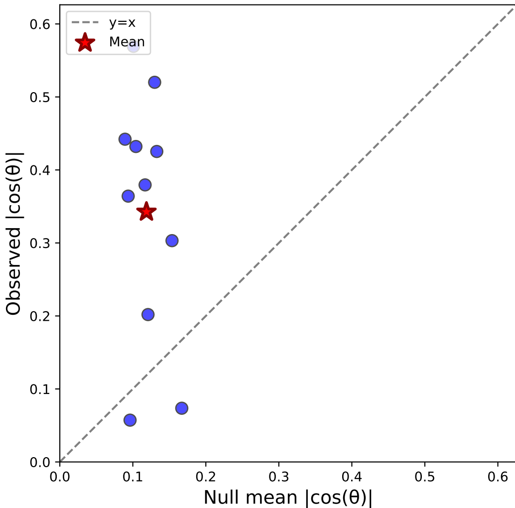
Monkey M: C-S Alignment in FEF N=11 sessions, \Delta=0.224\pm0.051
