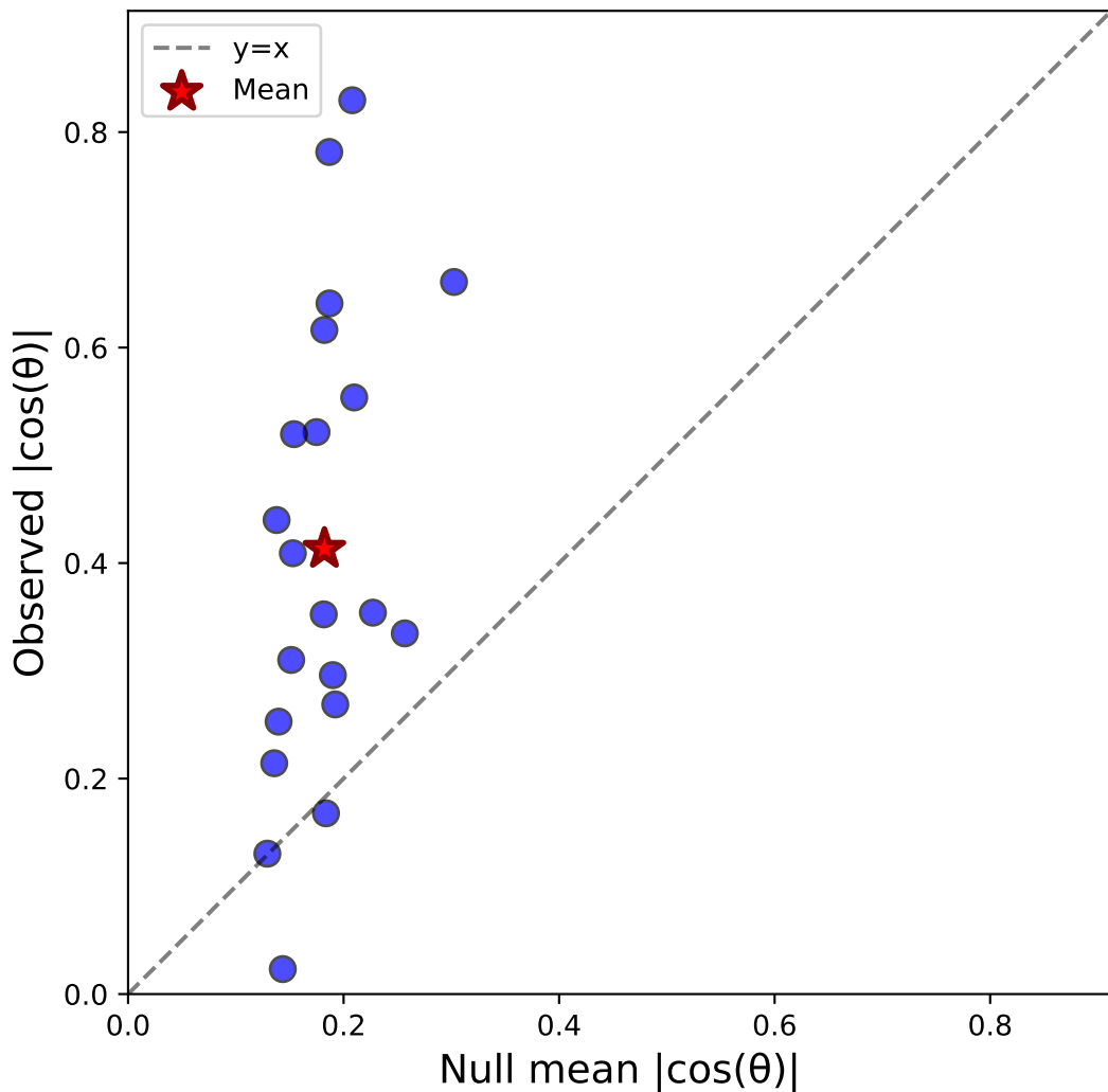
Case iii: Stim-C(vert) vs Sacc-S(horiz) (correct) - Monkey all N=21, \Delta=0.231
