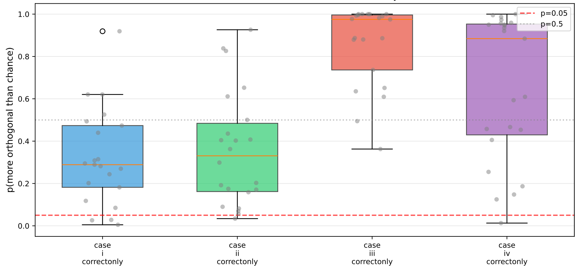
P-value Distribution (Correct Trials Only)
