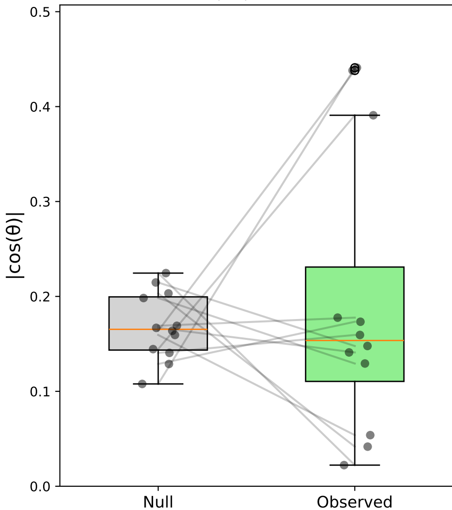
Case v: Stim-C(pool) vs Sacc-S(pool) - Monkey S \Delta|\cos| = 0.025
