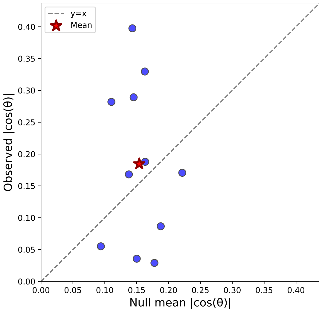
Case v: Stim-C(pool) vs Sacc-S(pool) - Monkey M N=11, \Delta=0.031 , Sig=0/11
