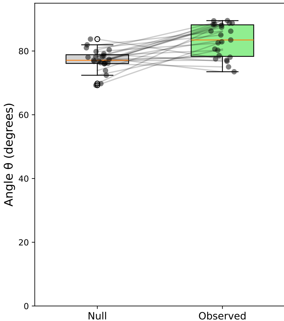
Case ii: Sacc C&S (pooled, all) - Monkey all \Delta\theta = 6.1^\circ
