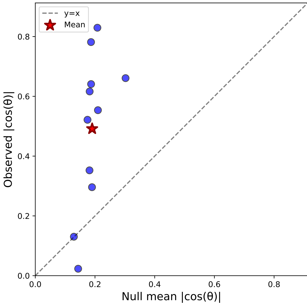
Case iii: Stim-C(ver) vs Sacc-S(horiz) (correct) - Monkey M N=11, \Delta=0.301 , Sig=0/11
