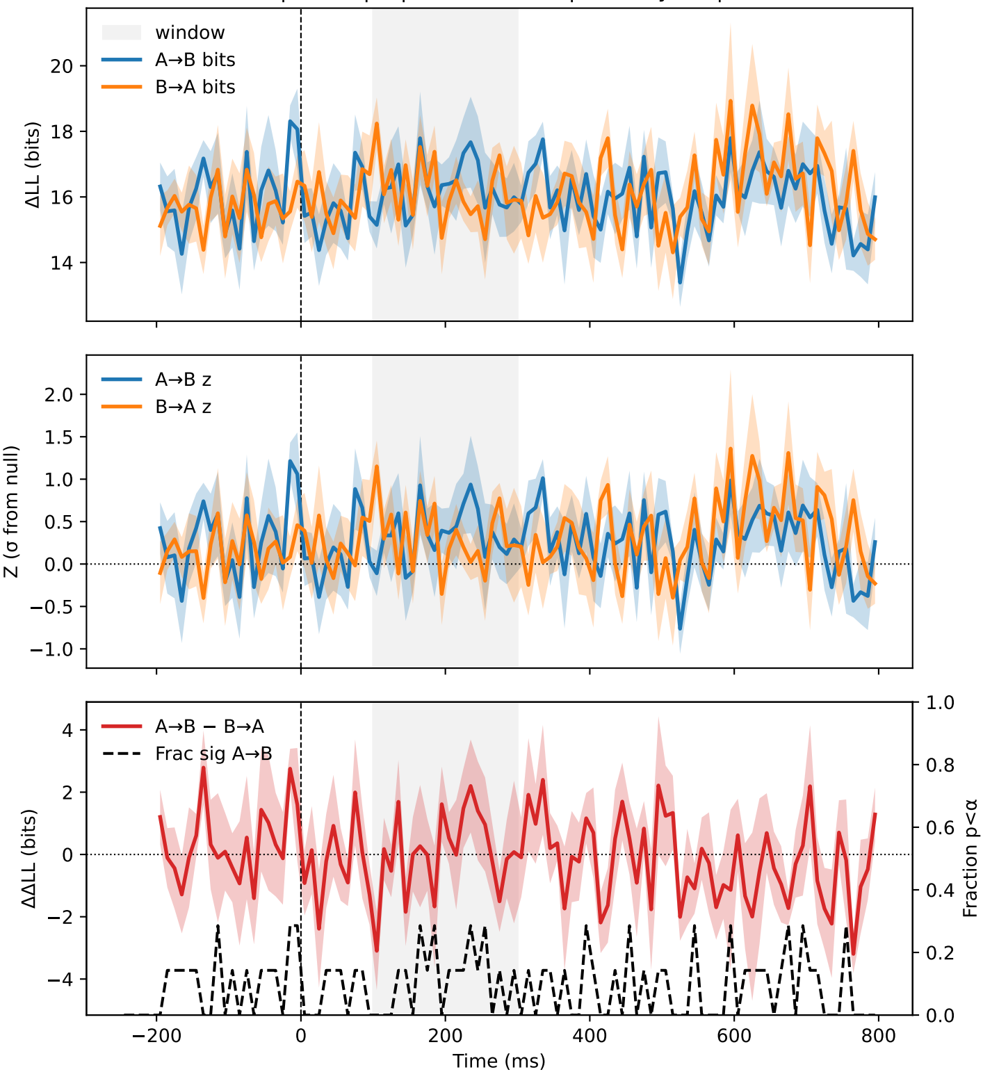
STIM | crnull | R | MFEF vs MSC | monkey=M | N=7
