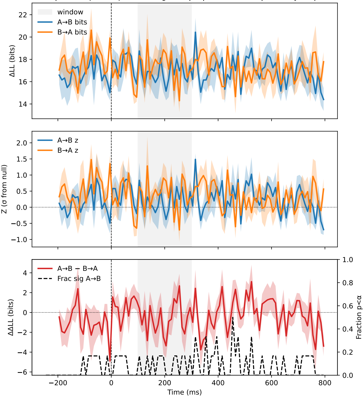
STIM | crsweep-stim-pooled-zreg-trial | R | SFEF vs SSC | monkey=S | N=6
