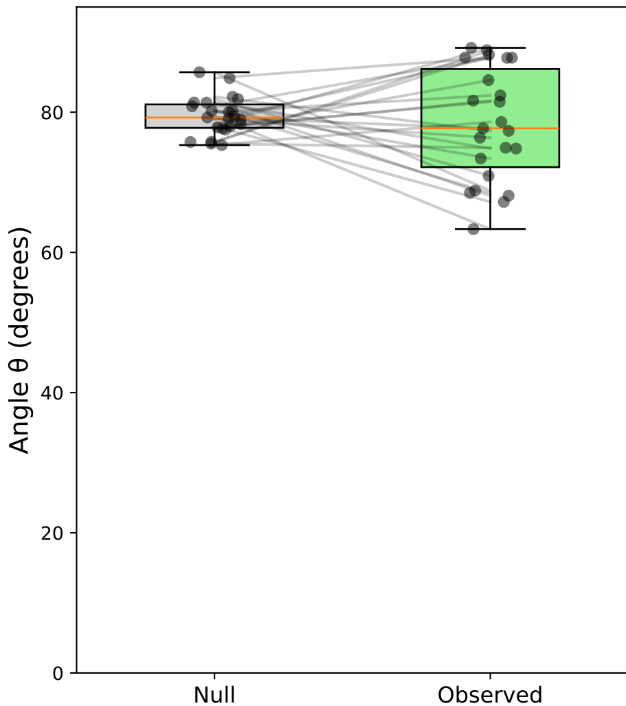
Case iv: Stim-C vs Sacc-S pooled (correct) - Monkey all \Delta\theta = -1.2^\circ
