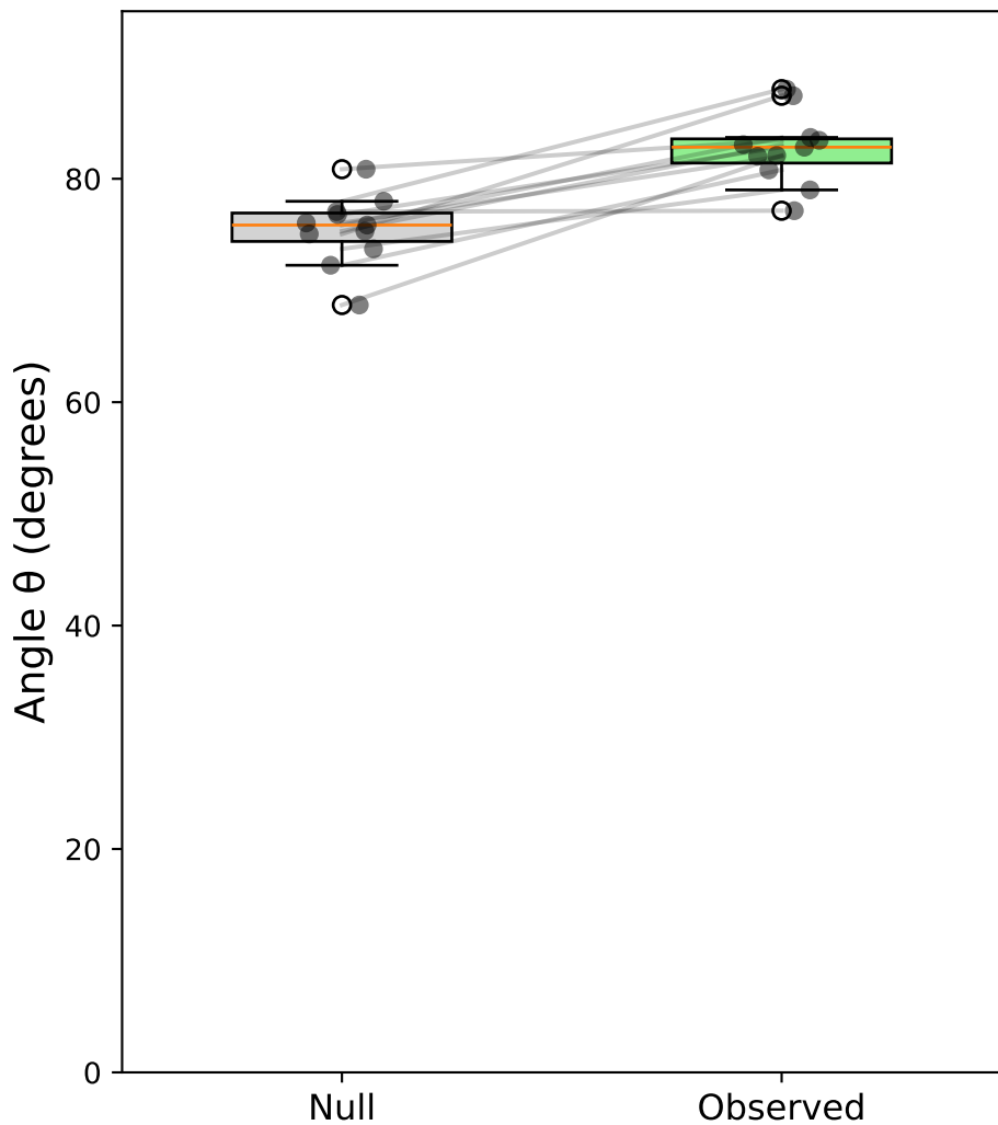
Case ii: Sacc C&S (pooled, correct) - Monkey M \Delta\theta = 7.3^\circ
