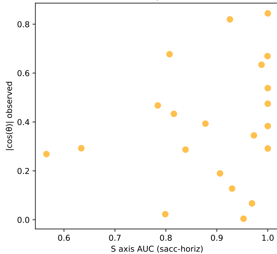
a_obs vs auc_S r=0.222 , p=0.3329
