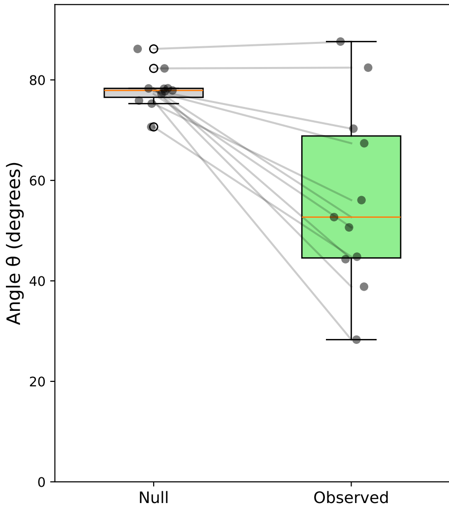
Case iii: Stim-C vs Sacc-S (correct) - Monkey M \Delta\theta = -21.3^\circ
