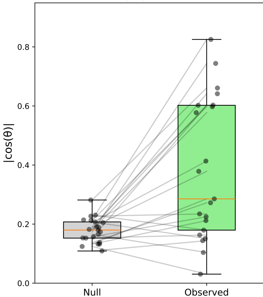
Case iii: Stim-C(ver) vs Sacc-S(horiz) (all) - Monkey all \Delta|\cos| = 0.204
