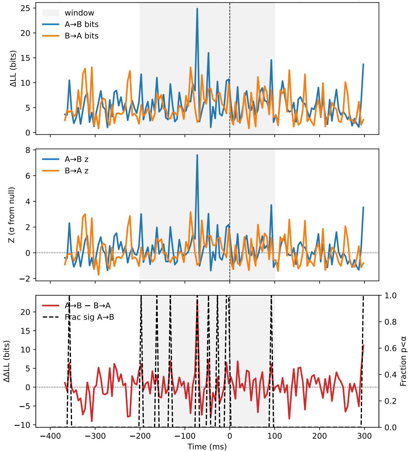
SACC | crsweep-sacc-vertical-none-circ | S | SFEF vs SSC | monkey=S | N=1
