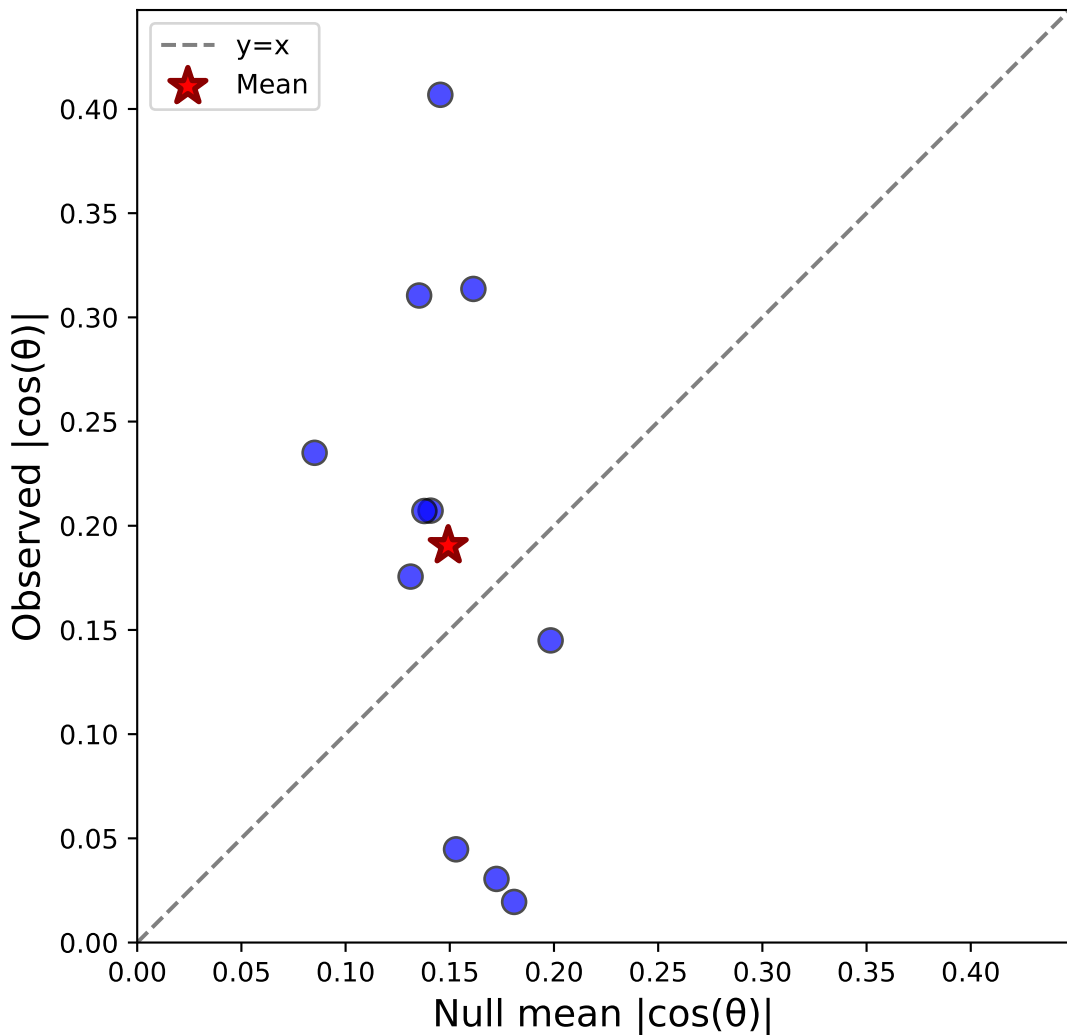
Case v: Stim-C(pool) vs Sacc-S(pool) - Monkey M N=11, \Delta=0.041 , Sig=0/11
