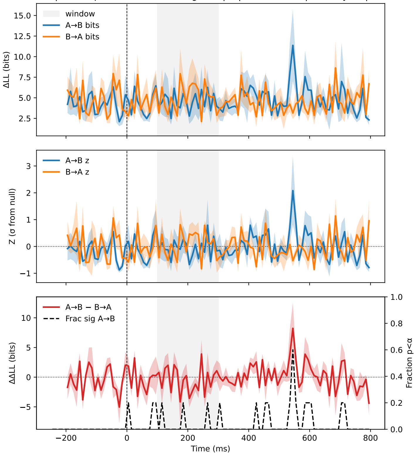
STIM | crsweep-stim-horizontal-zreg-trial | C | SFEF vs SSC | monkey=S | N=5
