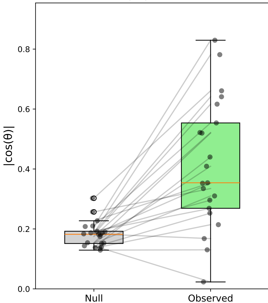
Case vi: Stim-C(ver) vs Sacc-S(horiz) - Monkey all \Delta|\cos| = 0.231
