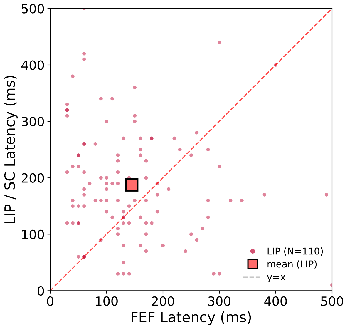
Monkey M - (LIP & SC) vs FEF - direction [stim] LIP-FEF: 3 sess, mean(LIP-FEF)=42.8ms
