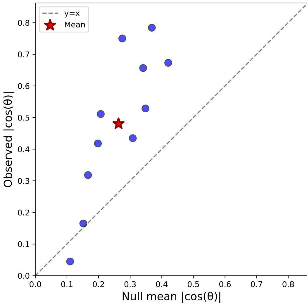
Case vi: Stim-C(ver) vs Sacc-S(horiz) - Monkey M N=11, \Delta=0.217 , Sig=0/11
