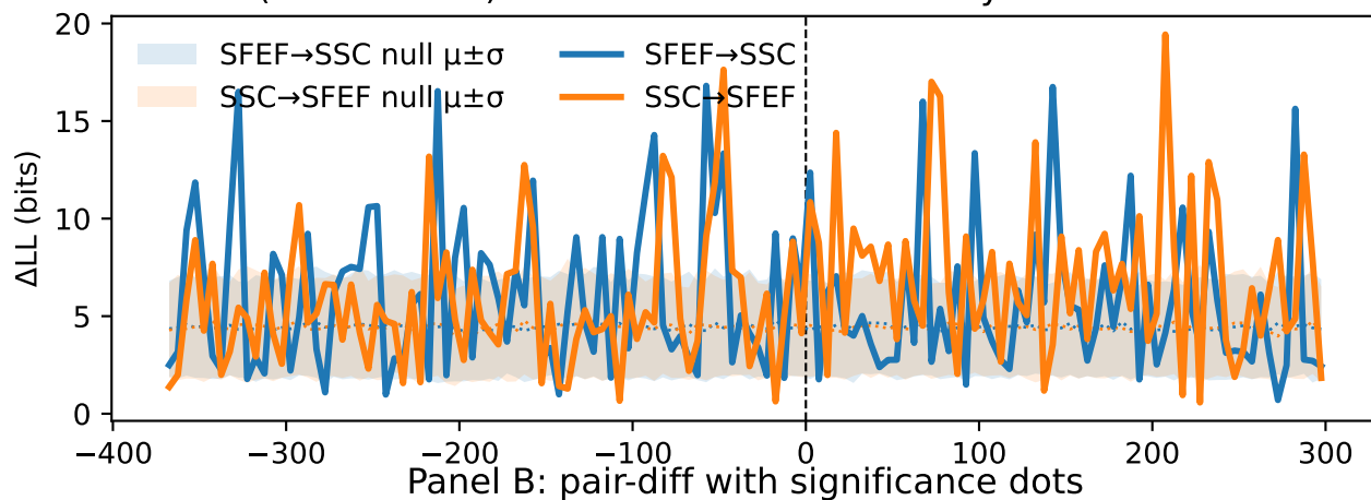
(SFEF vs SSC) — S-flow — Panel A: overlay + null bands
