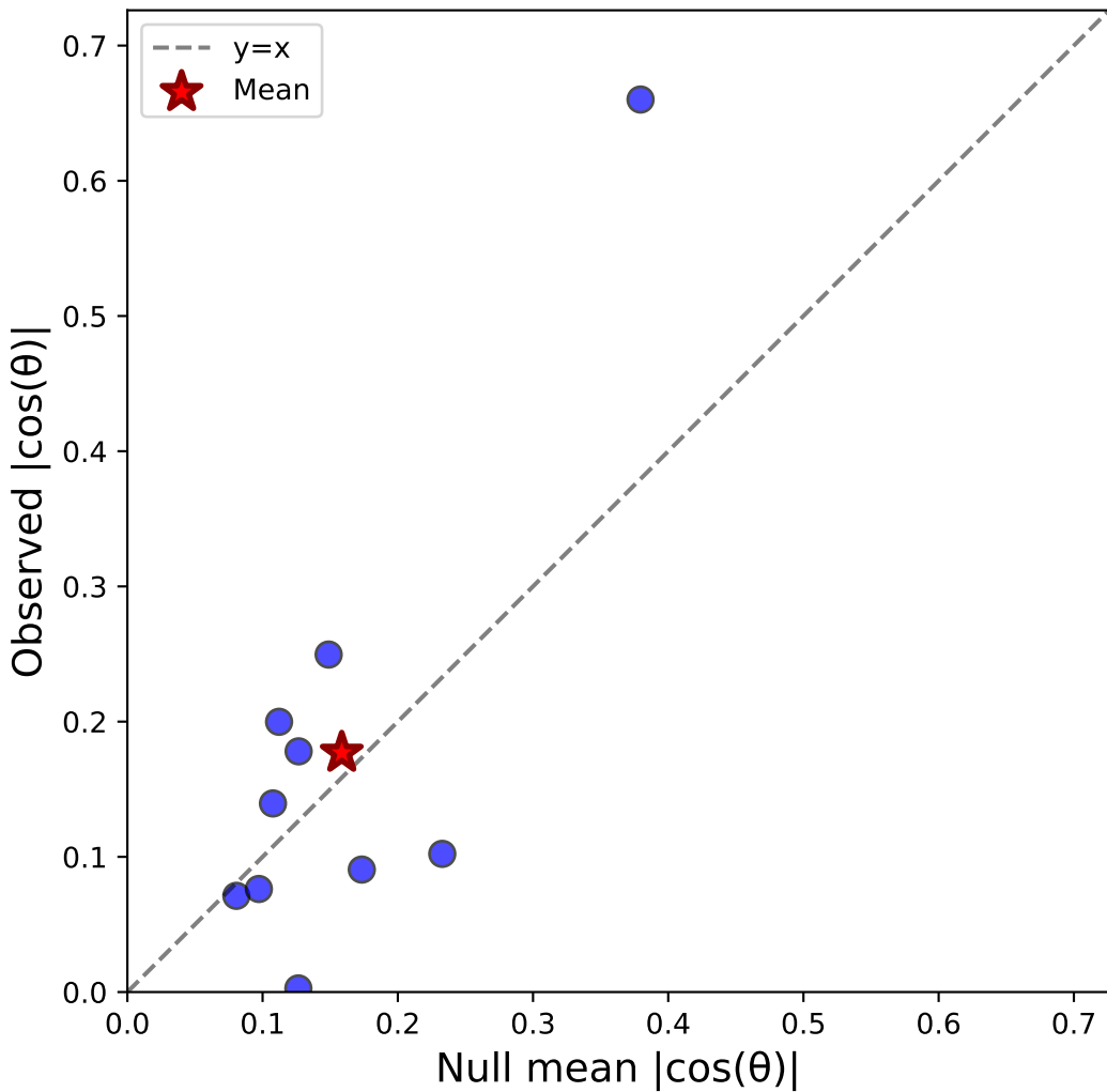
Monkey S: C-S Alignment in FEF N=10 sessions, \Delta=0.018\pm0.037
