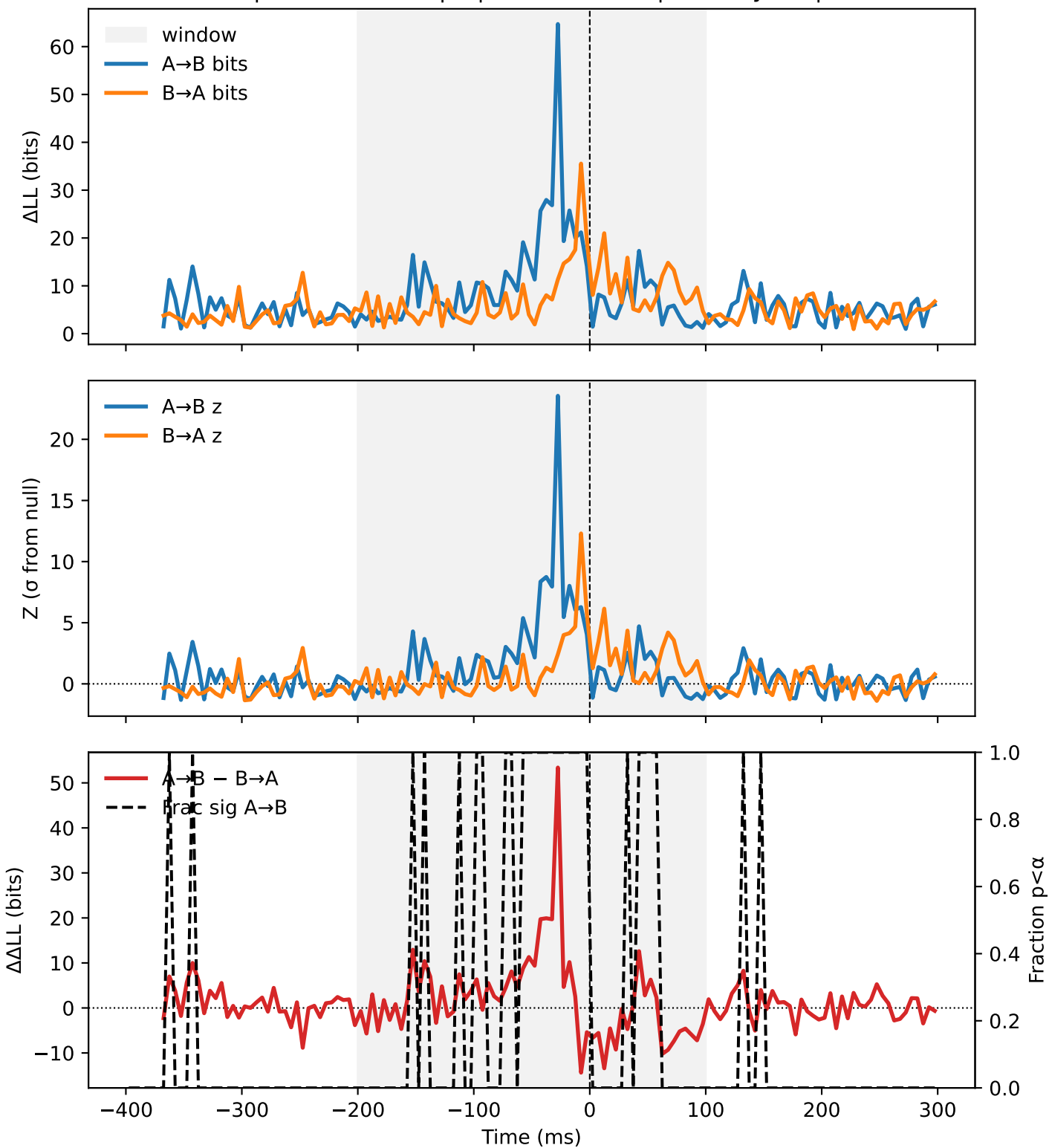
SACC | crnull-vertical | S | MFEF vs MSC | monkey=M | N=1
