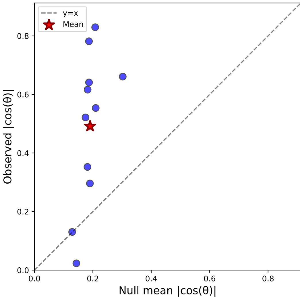
Case iii: Stim-C(ver) vs Sacc-S(horiz) (correct) - Monkey M N=11, \Delta=0.301
