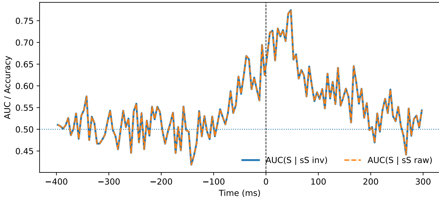
MFEF — QC (sacc, ori=vertical, PT \geq 200.0, norm=global)
