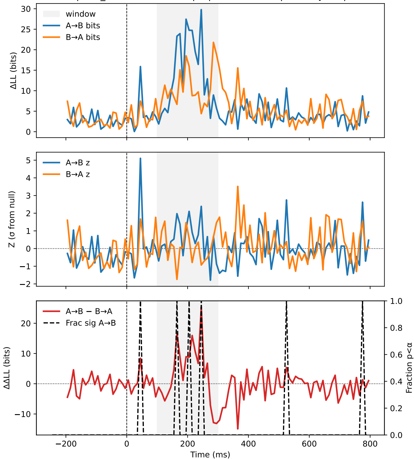
STIM | test_evoked-none-trial | C | MFEF vs MSC | monkey=M | N=1
