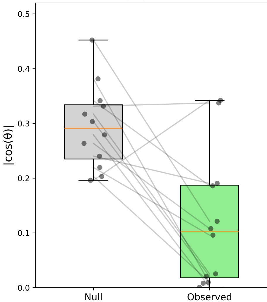
Case iii: Sacc C&S (vert) - Monkey S \Delta|\cos| = -0.174
