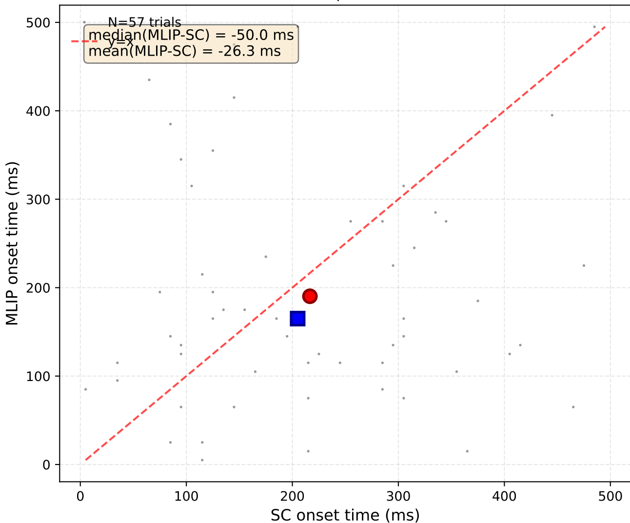
Monkey M (SC vs MLIP) - direction 3 sessions, 57 trials mean: (216.6, 190.3) ms | median: (205.0, 165.0) ms
