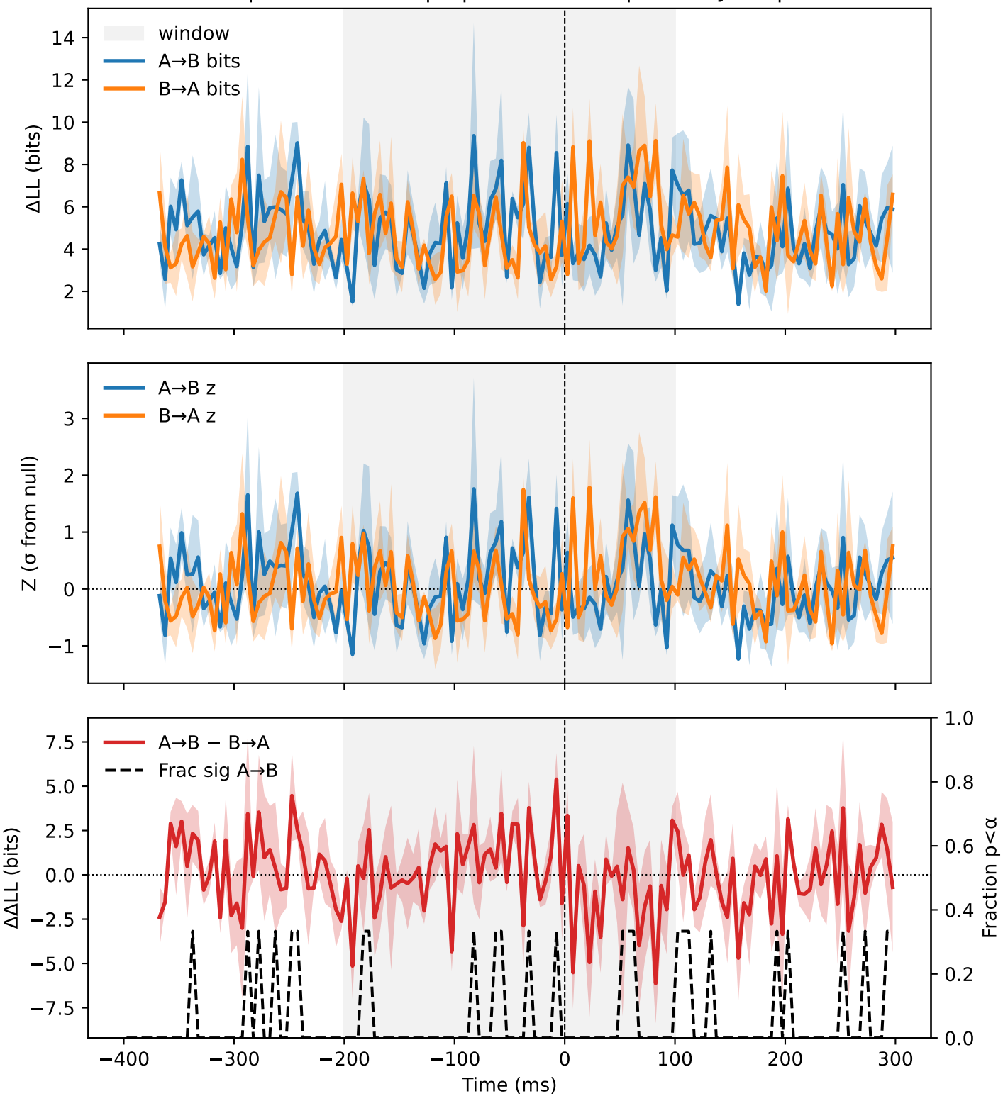
SACC | crnull-vertical | S | MLIP vs MSC | monkey=M | N=3
