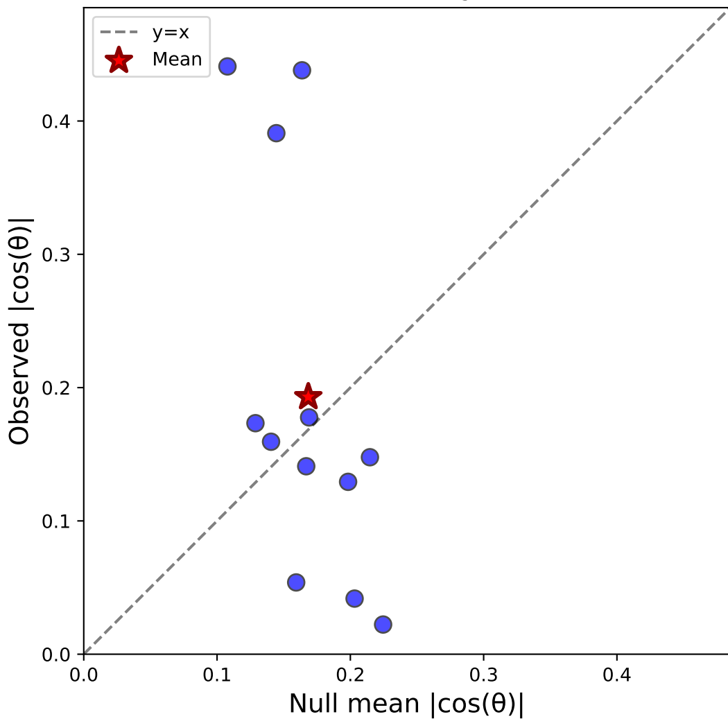
Case v: Stim-C(pool) vs Sacc-S(pool) - Monkey S N=12, \Delta=0.025 , Sig=0/12
