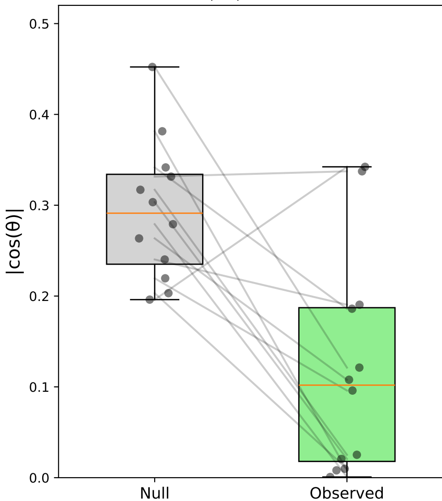
Case vi: Sacc C&S (vert, all) - Monkey S \Delta|\cos| = -0.174
