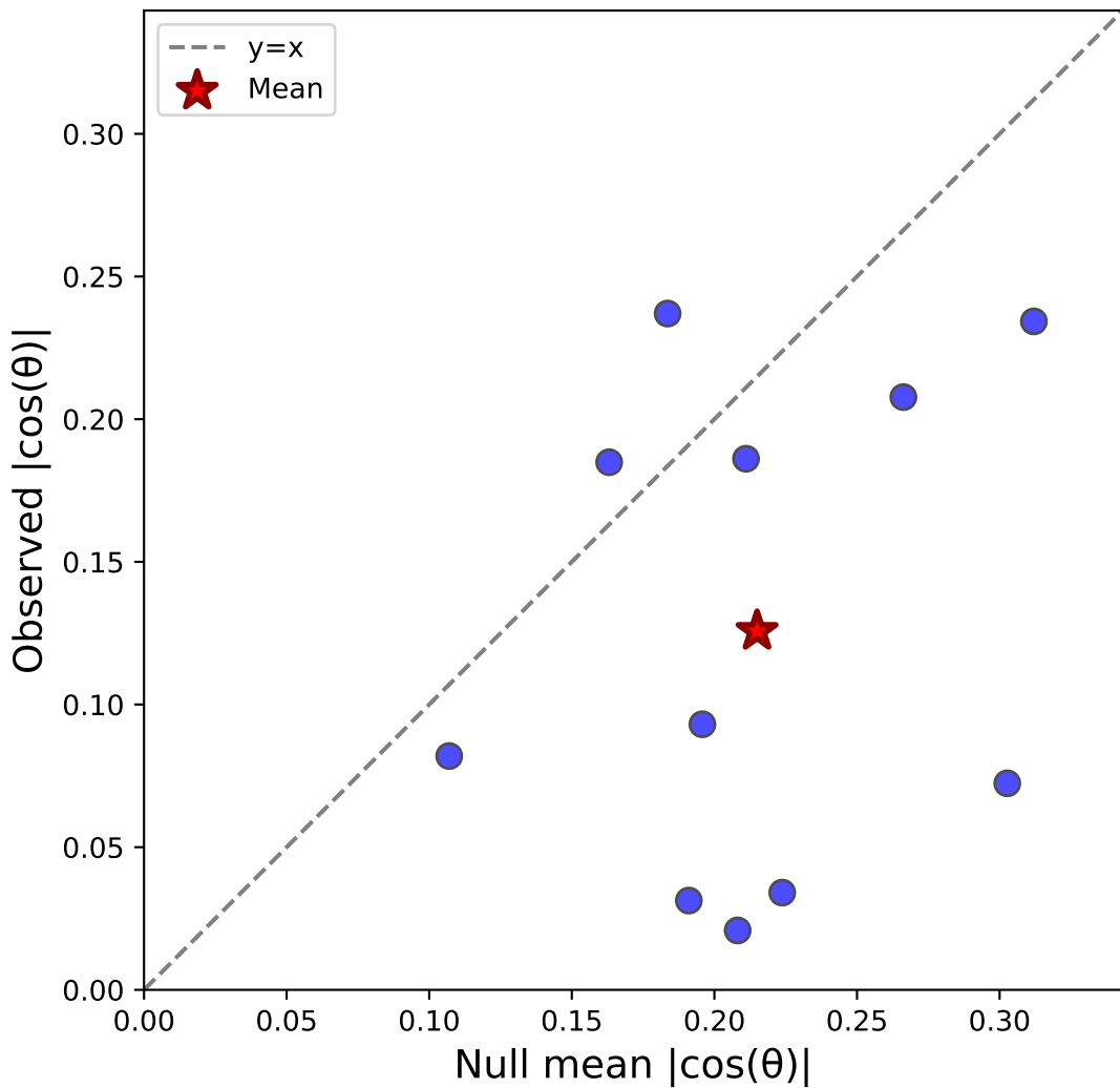
Case iv: Stim-C(horiz) vs Sacc-S(horiz) - Monkey M N=11, \Delta=-0.089 , Sig=0/11
