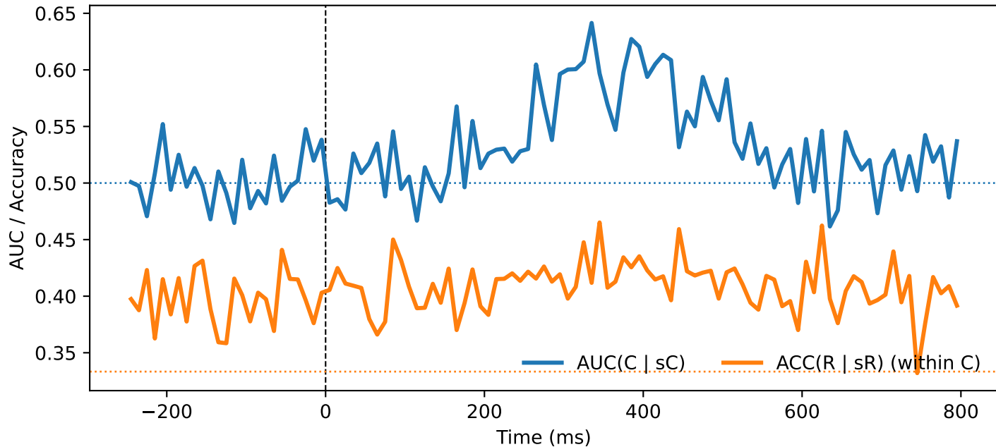
SLIP — QC (stim, ori=vertical, PT \geq 200.0, norm=global)
