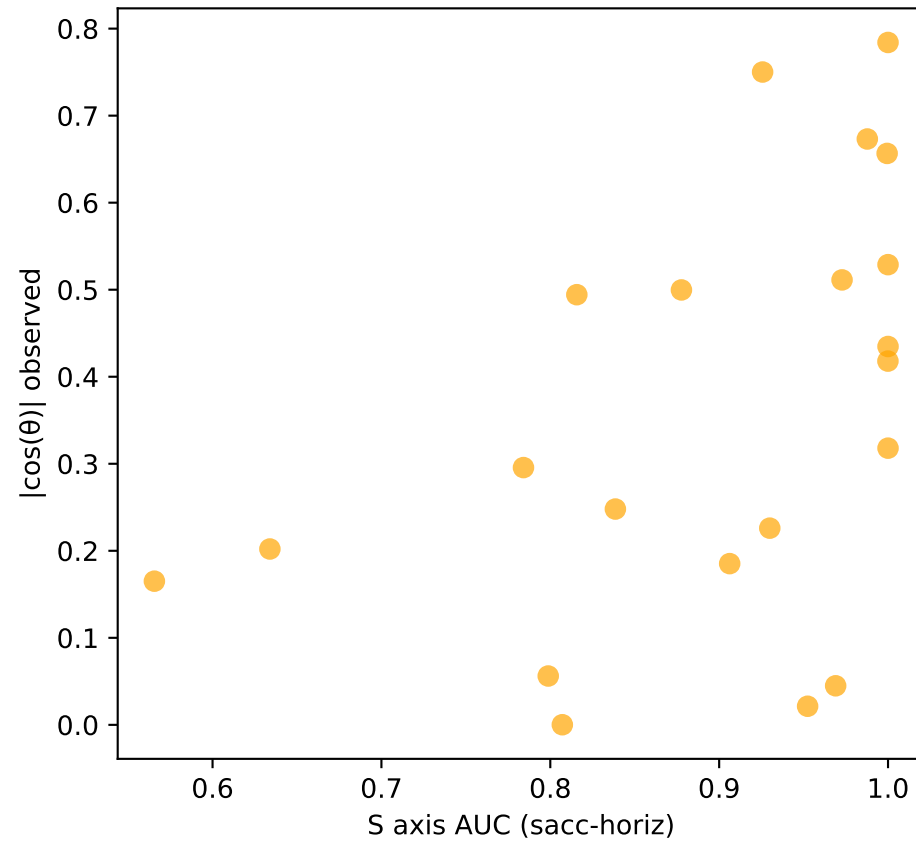
a_obs vs auc_S r=0.453 , p=0.0394
