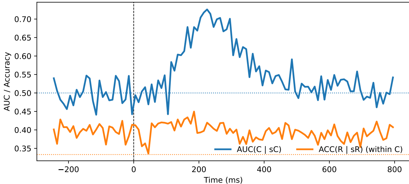
SFEF — QC (stim, ori=horizontal, PT \geq 200.0)
