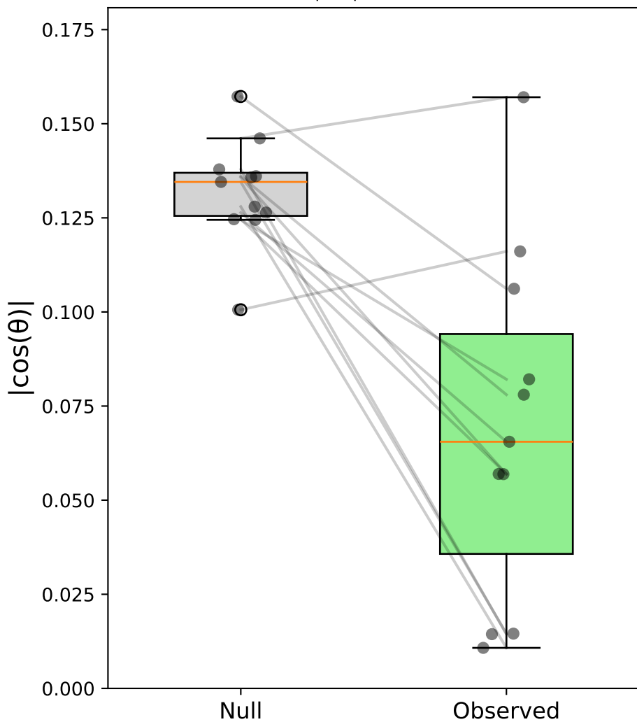
Case iv: Stim-C(horiz) vs Sacc-S(horiz) - Monkey M \Delta|\cos| = -0.063
