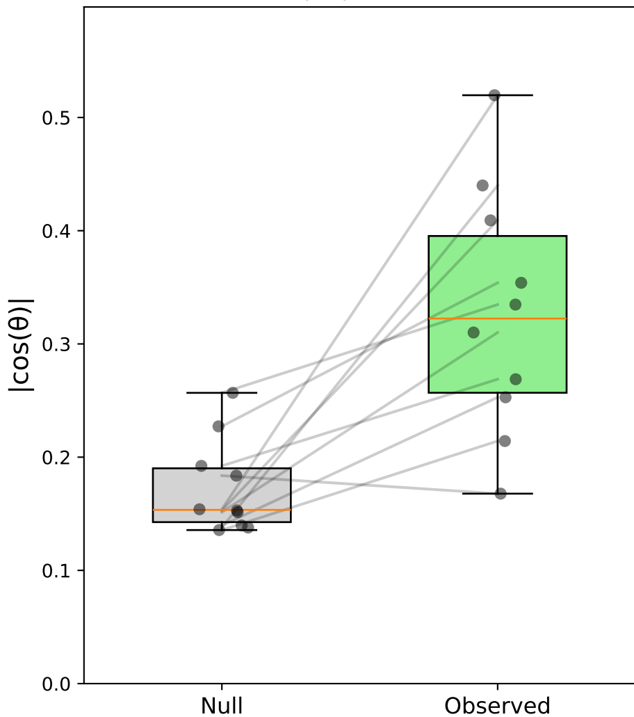
Case vi: Stim-C(ver) vs Sacc-S(horiz) - Monkey S \Delta|\cos| = 0.154
