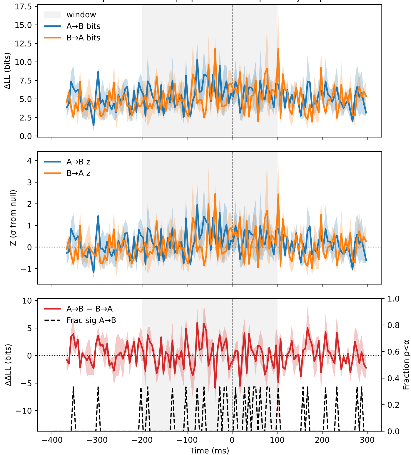
SACC | crnull-vertical | S | SFEF vs SLIP | monkey=S | N=3
