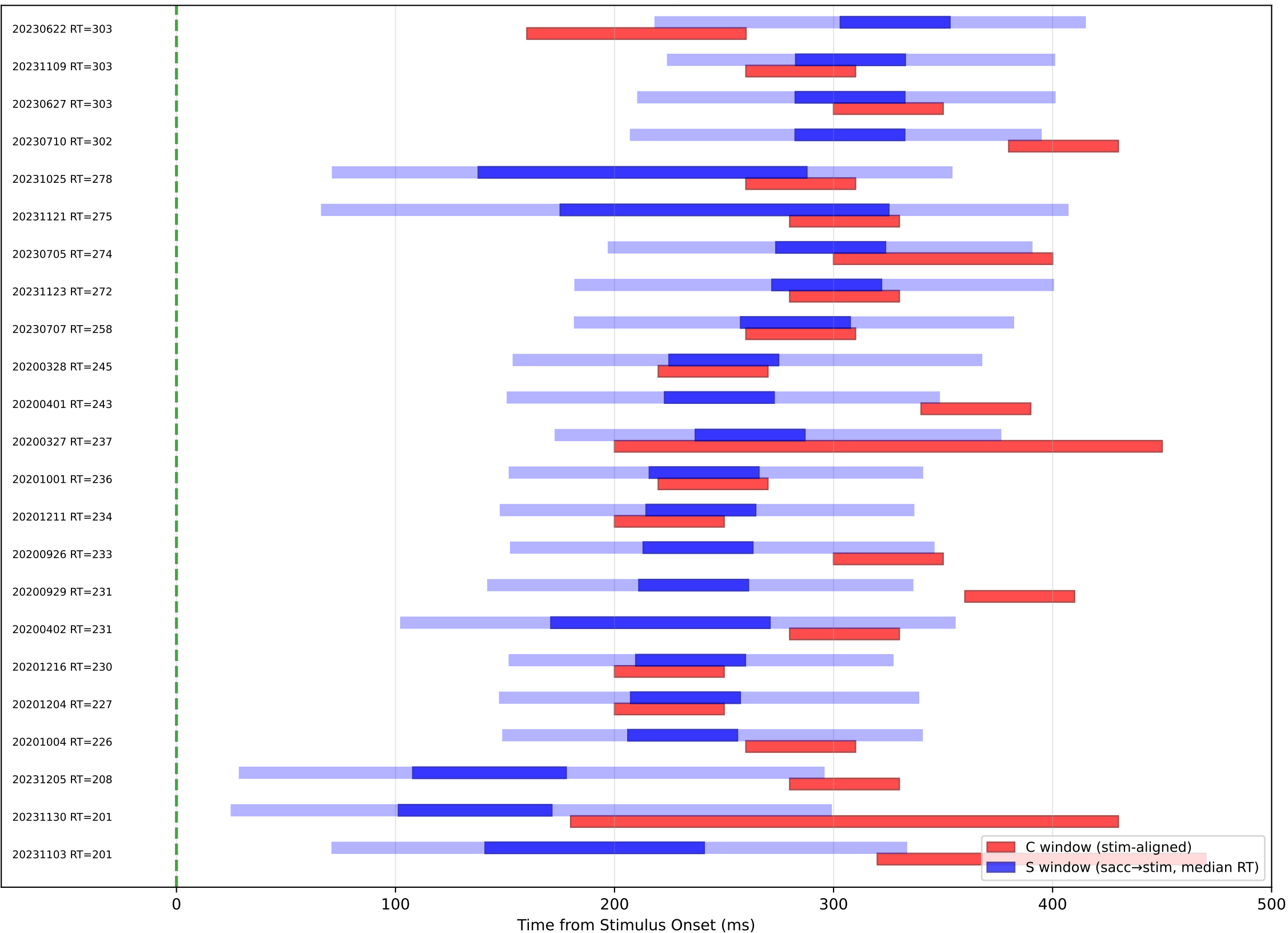
Case vi: Stim-C(ver) vs Sacc-S(horiz) (correctly)
