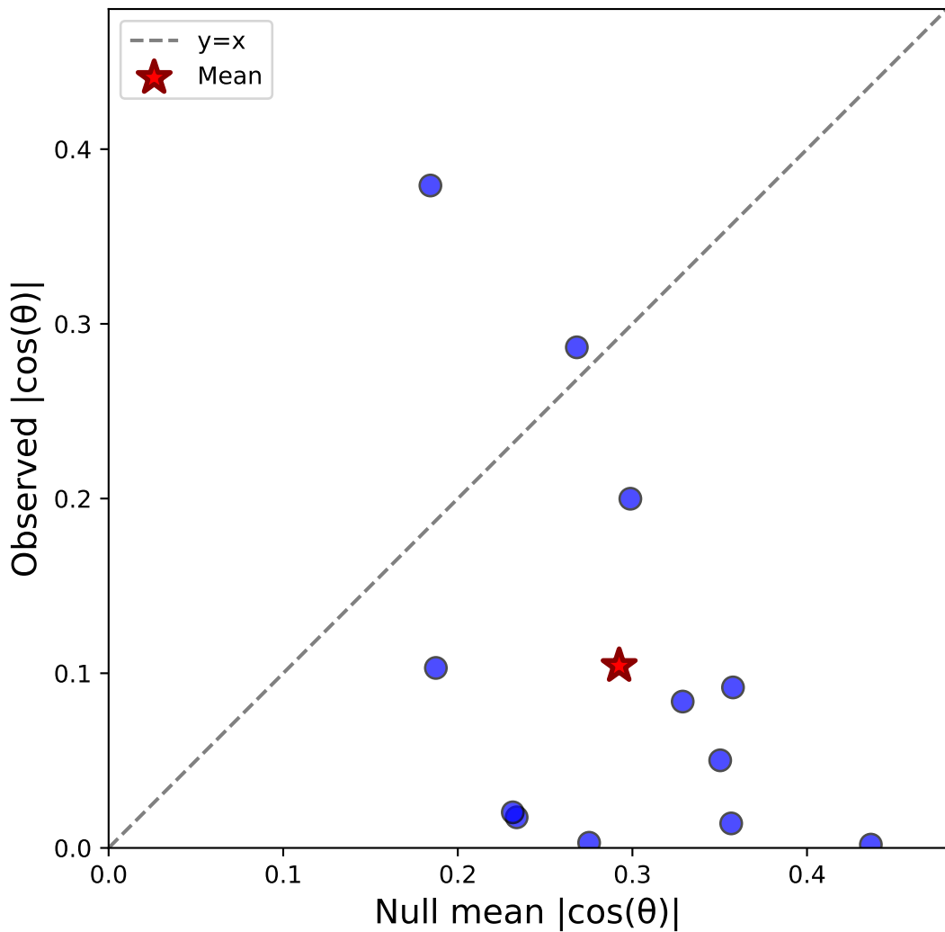
Case ii: Sacc C&S (pooled) - Monkey S N=12, \Delta=-0.188 , Sig=5/12
