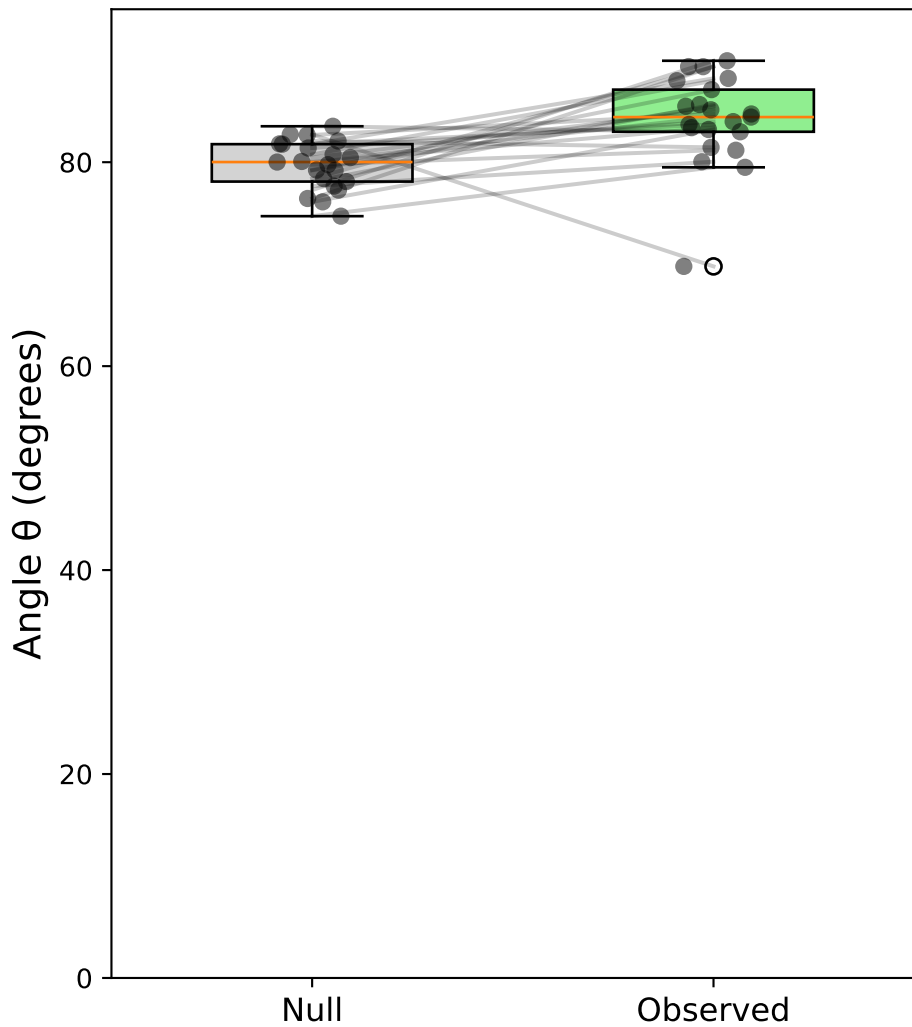
Case i: Sacc C&S (horiz, correct) - Monkey all \Delta\theta = 4.4^\circ
