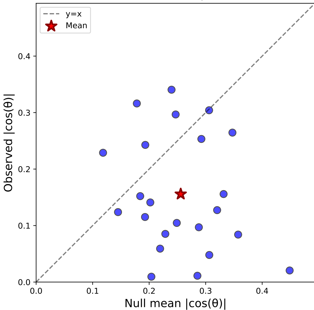
Case v: Stim-C(pool) vs Sacc-S(pool) - Monkey all N=23, \Delta=-0.100 , Sig=3/23
