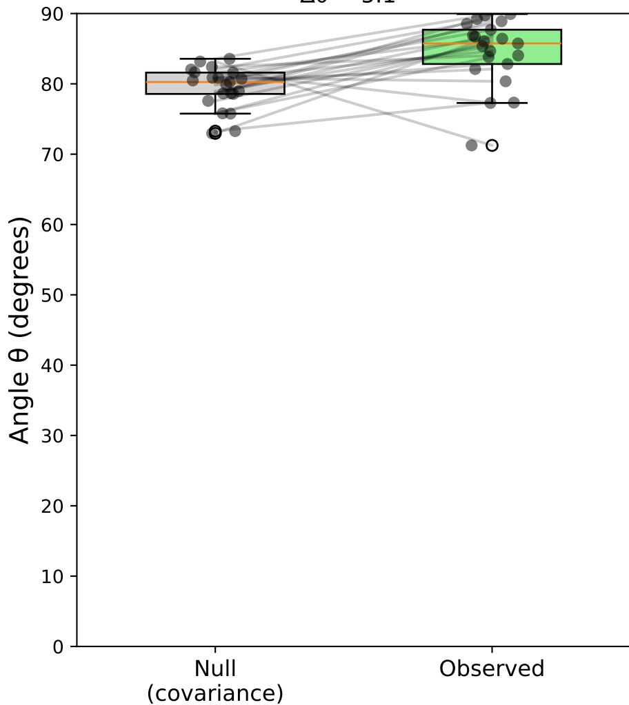
Monkey all: Axis Angle (cov-null) \Delta\theta = 5.1^\circ
