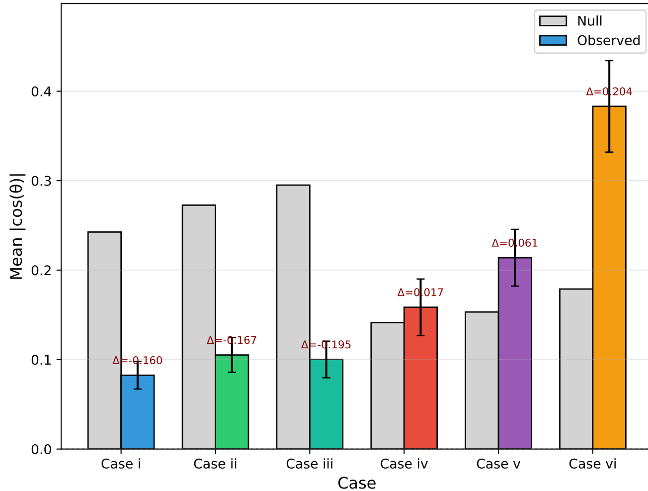
Mean Observed vs Null |\cos(\theta)|
