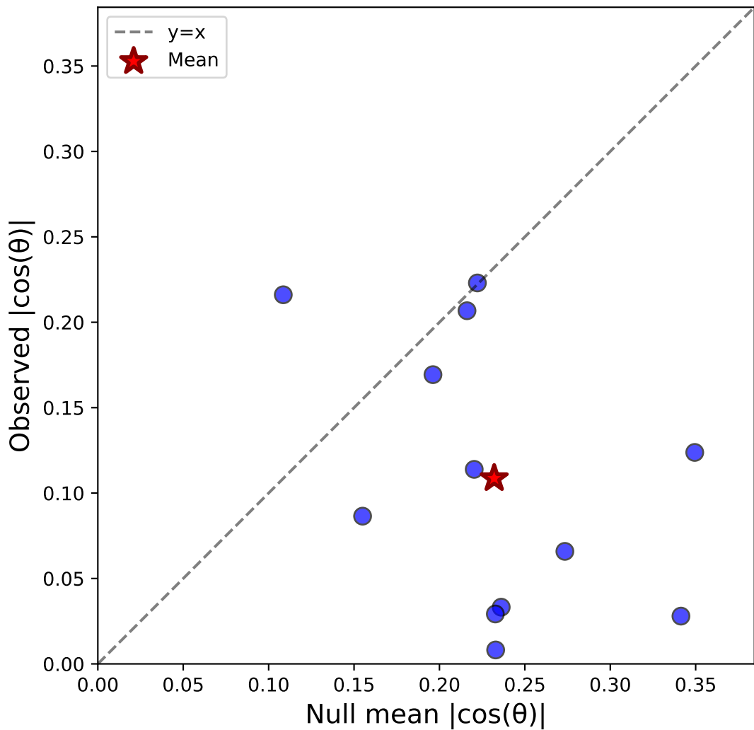
Case ii: Sacc C&S (pooled, all) - Monkey S N=12 , \Delta=-0.123\pm0.034
