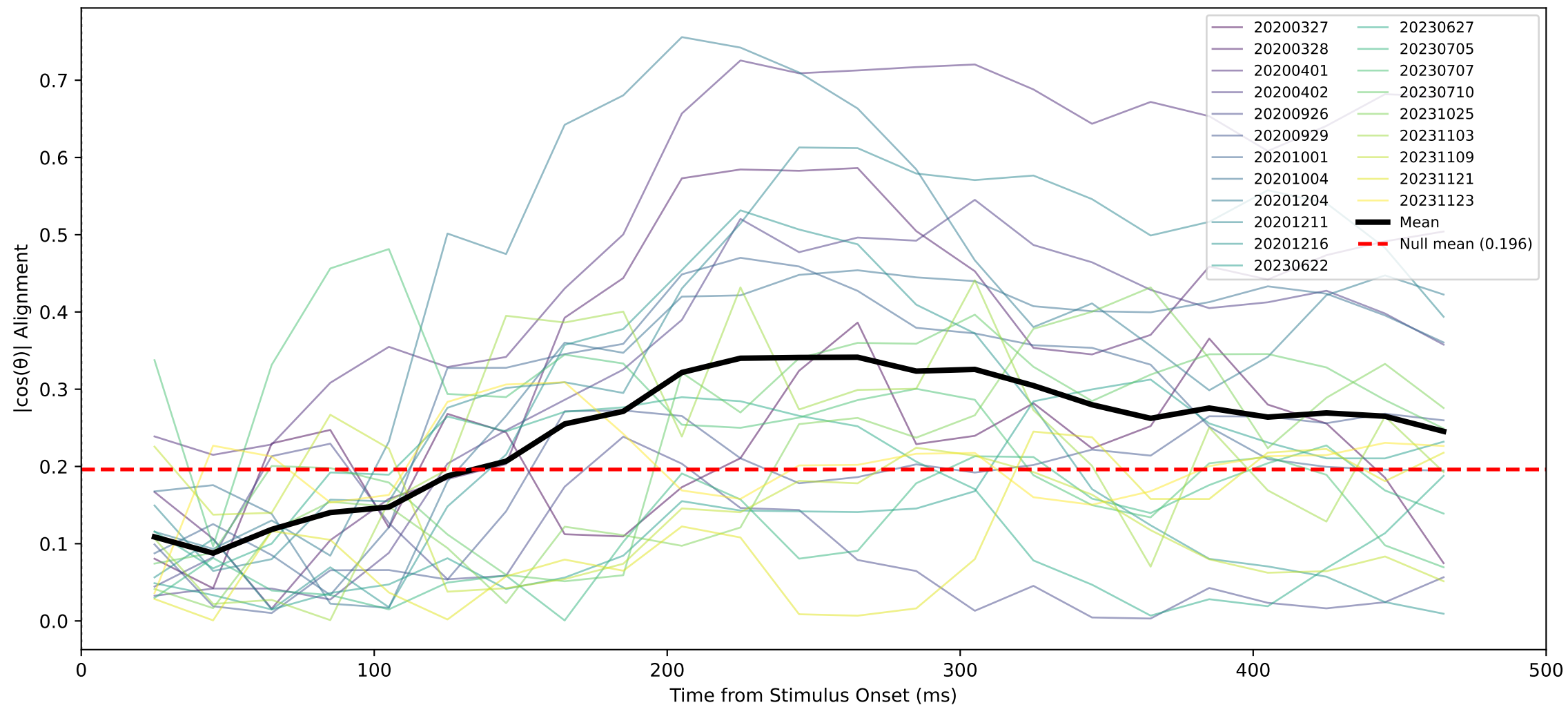
Temporal Cross-Alignment: C(vertical, stim) vs S(horizontal, sacc) N=21 sessions
