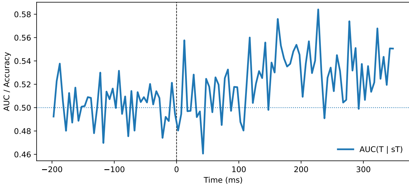
SSC — QC (targ, ori=None, PT \geq 200.0)
