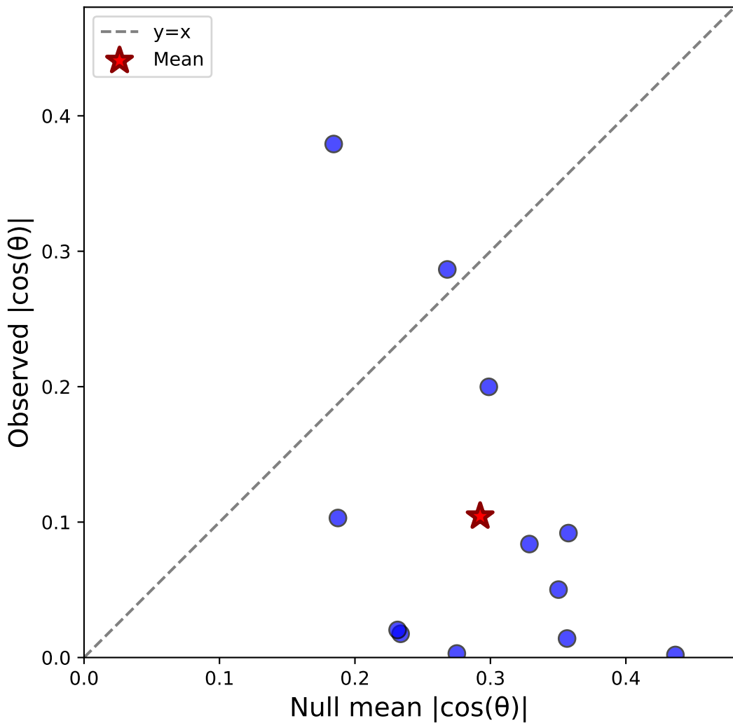
Case ii: Sacc C&S (pooled, all) - Monkey S N=12, \Delta=-0.188
