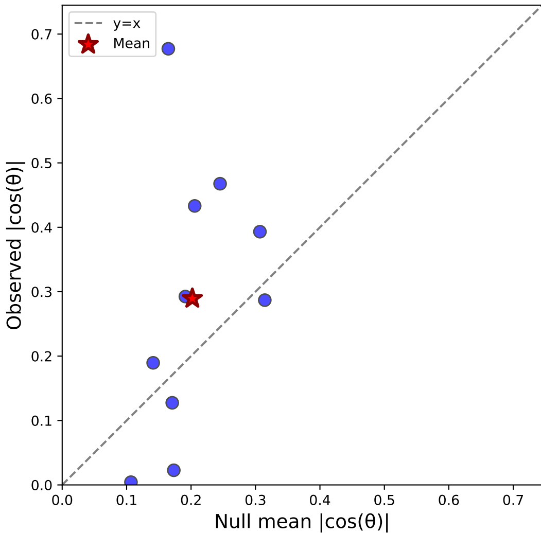
Case vi: Stim-C(ver) vs Sacc-S(horiz) - Monkey S N=10, \Delta=0.087 , Sig=1/10
