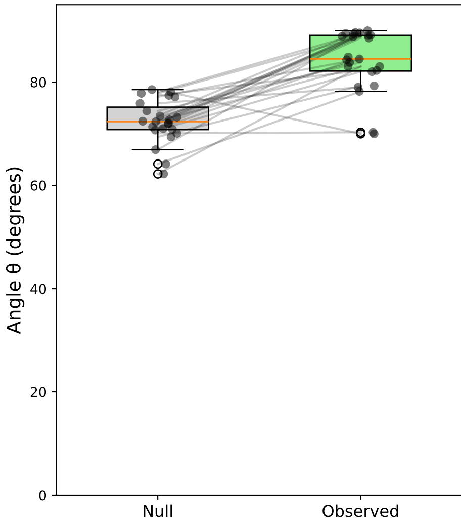
Case vi: Sacc C&S (vert, all) - Monkey all \Delta\theta = 11.9^\circ
