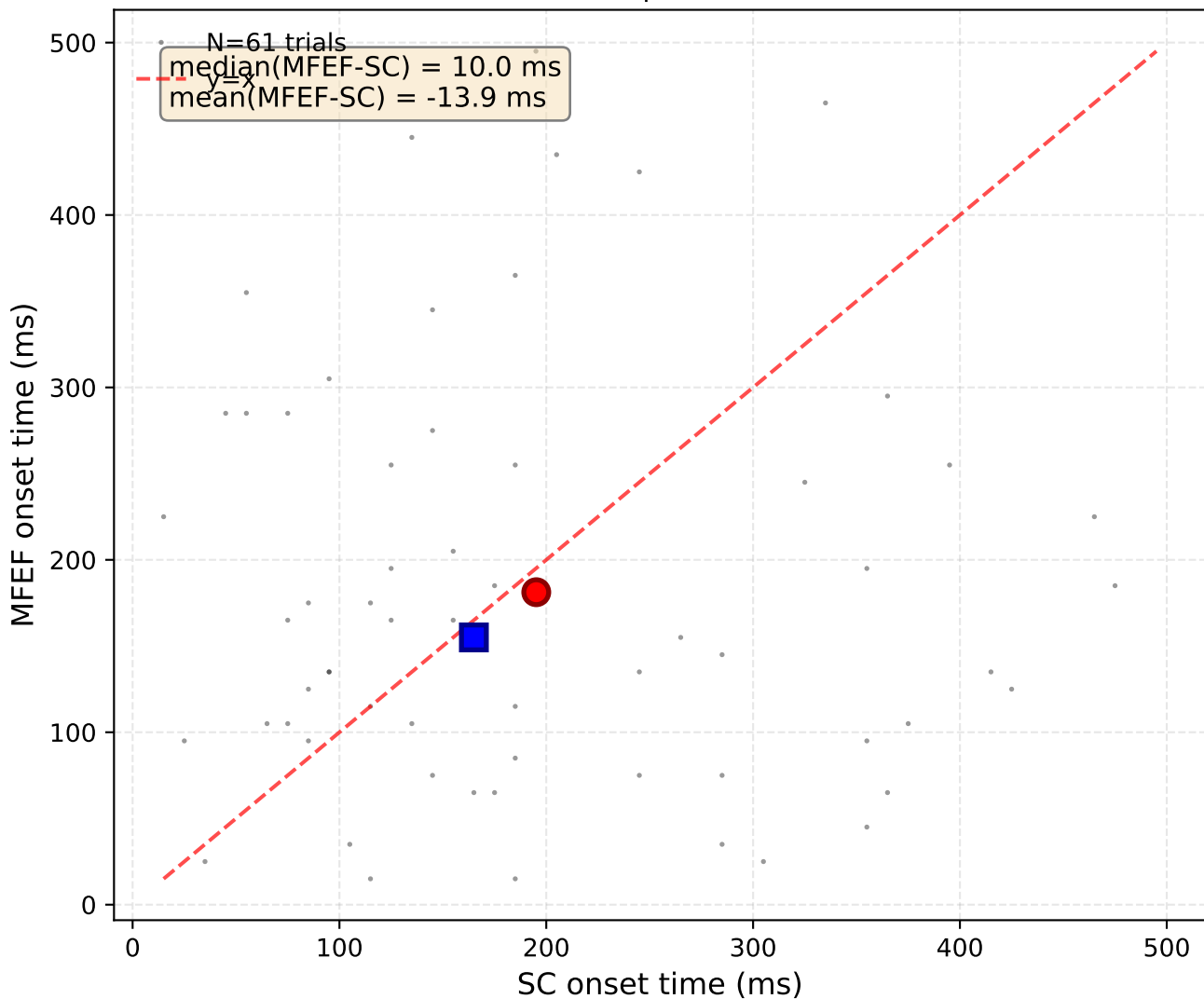
Monkey M (SC vs MFEF) - direction 4 sessions, 61 trials mean: (195.2, 181.2) ms | median: (165.0, 155.0) ms
