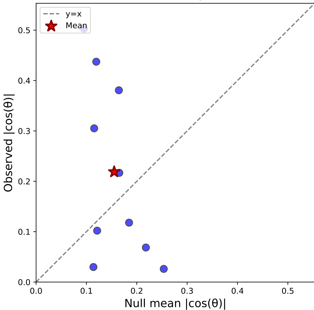
Case iv: Stim-C(horiz) vs Sacc-S(horiz) - Monkey S N=10, \Delta=0.064 , Sig=0/10
