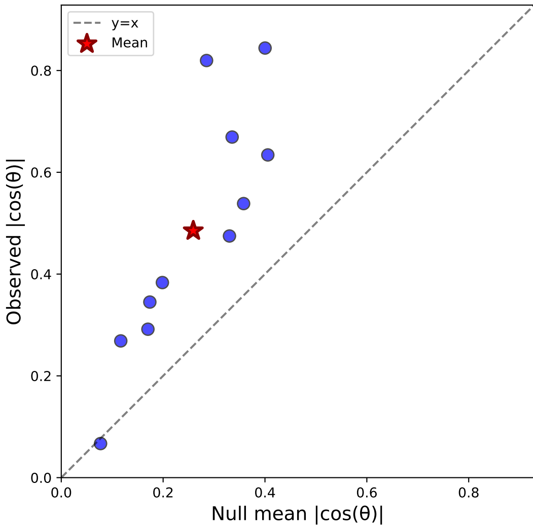
Case vi: Stim-C(ver) vs Sacc-S(horiz) - Monkey M N=11, \Delta=0.226 , Sig=0/11
