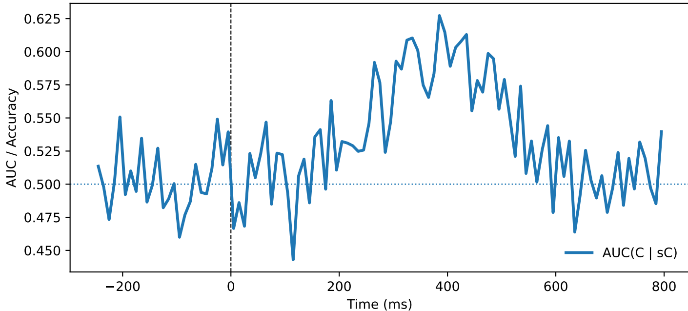
SLIP — QC (stim, ori=vertical, PT \geq 200.0, norm=baseline)
