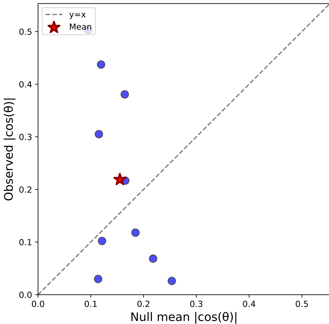
Case v: Stim-C(horiz) vs Sacc-S(horiz) (all) - Monkey S N=10, \Delta=0.064
