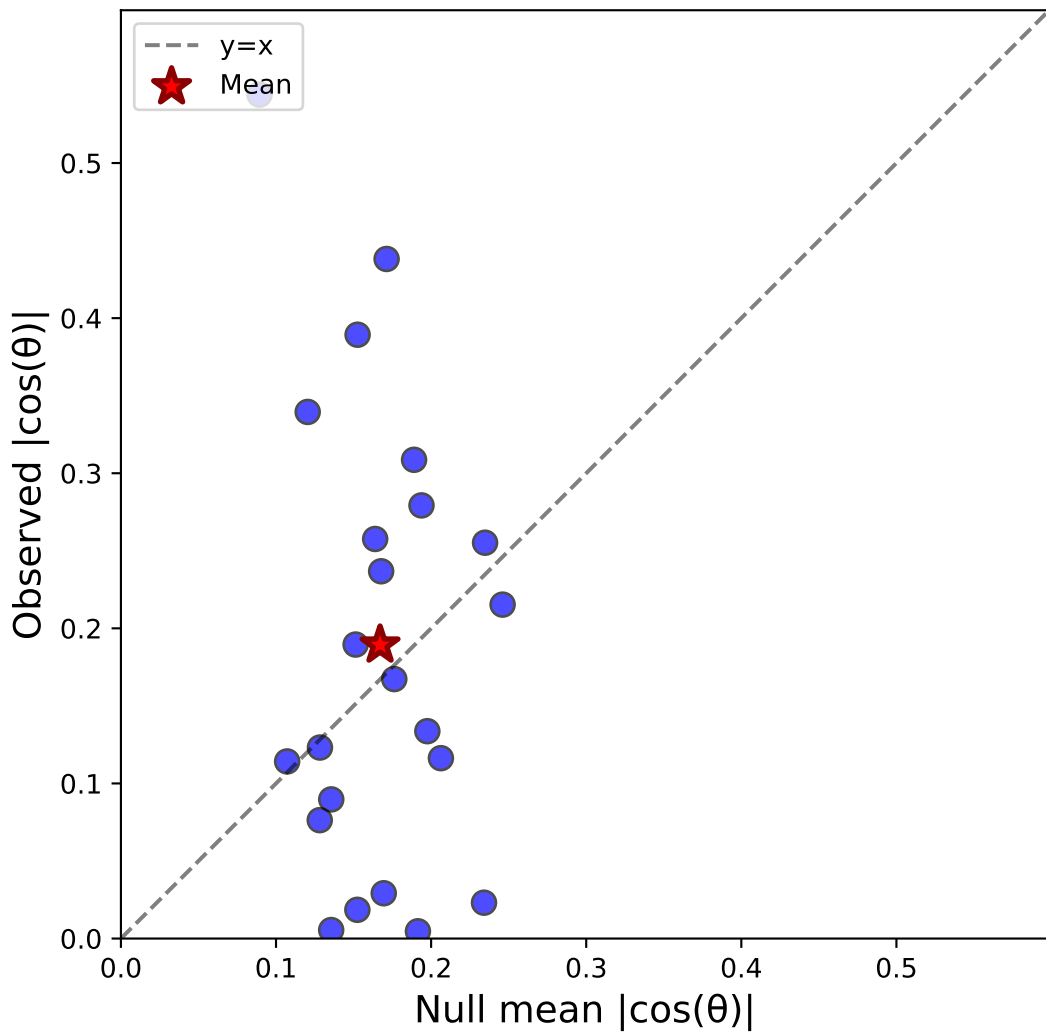
Case iv: Stim-C vs Sacc-S pooled (all) - Monkey all N=23 , \Delta=0.022\pm0.033
