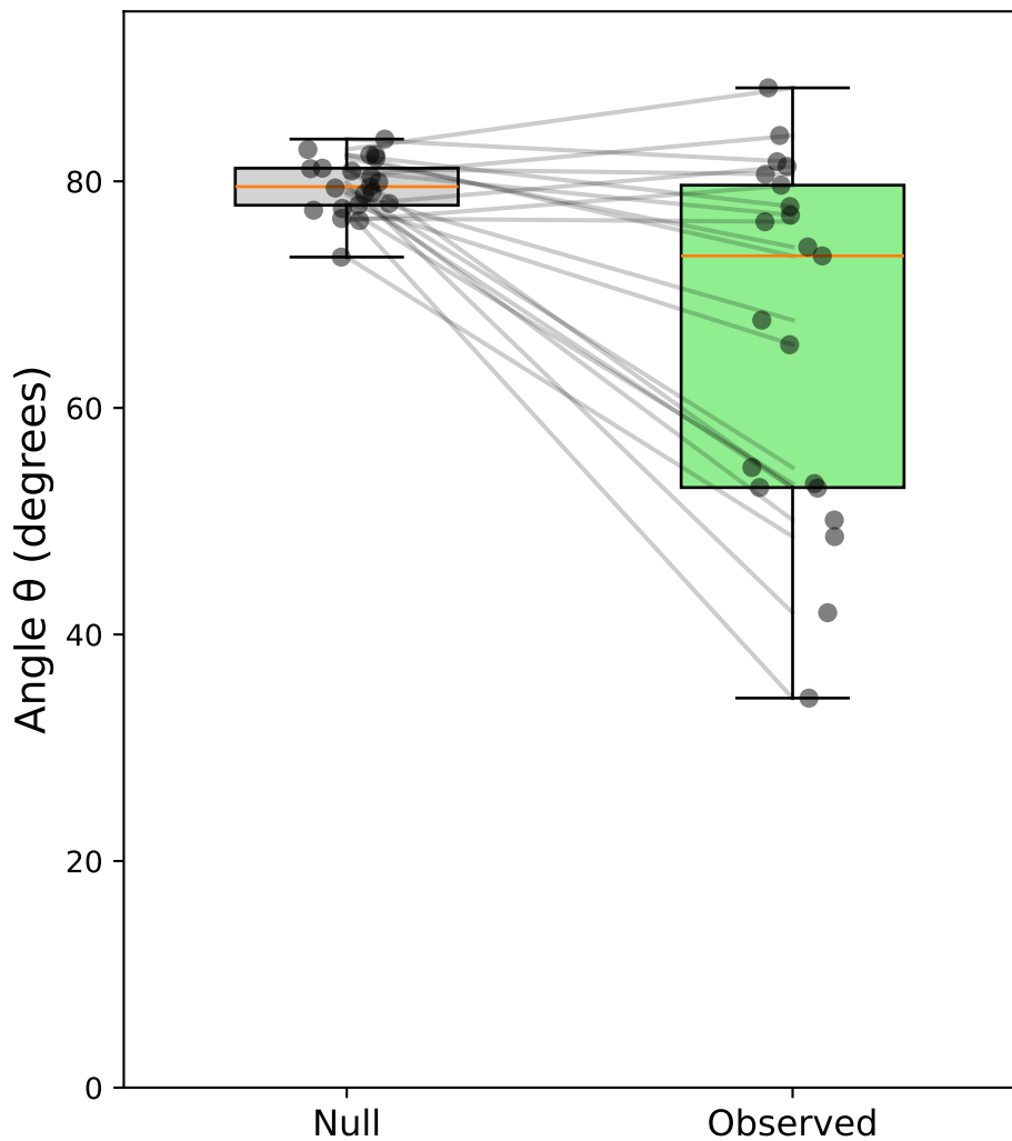
Case iii: Stim-C(ver) vs Sacc-S(horiz) (all) - Monkey all \Delta\theta = -13.1^\circ
