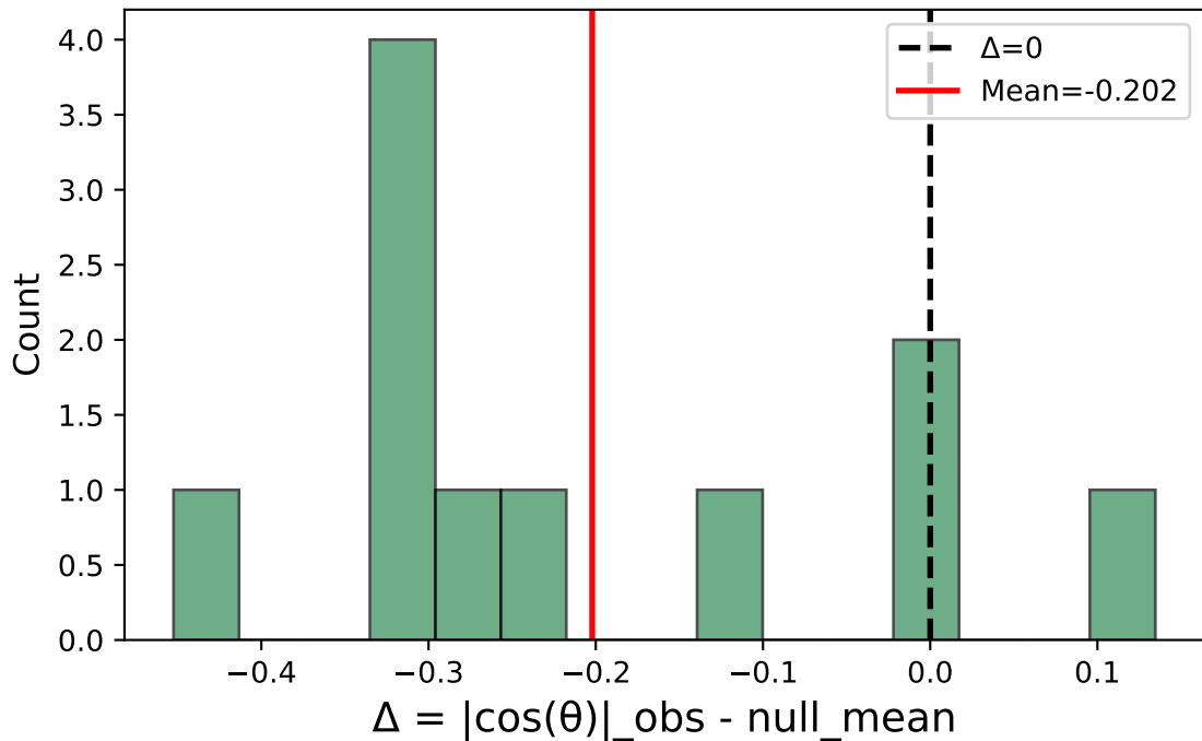
Case ii: Sacc C&S (pooled, correct) - Monkey S
