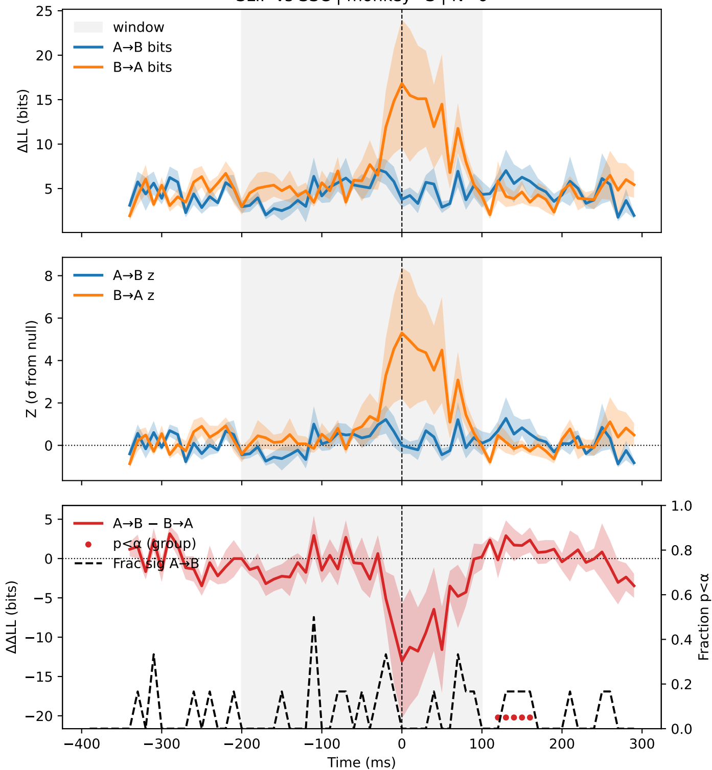
SACC | evoked_peakbin_saccS_horizontal_lag50ms_20mssw-none-trial | S SLIP vs SSC | monkey=S | N=6
