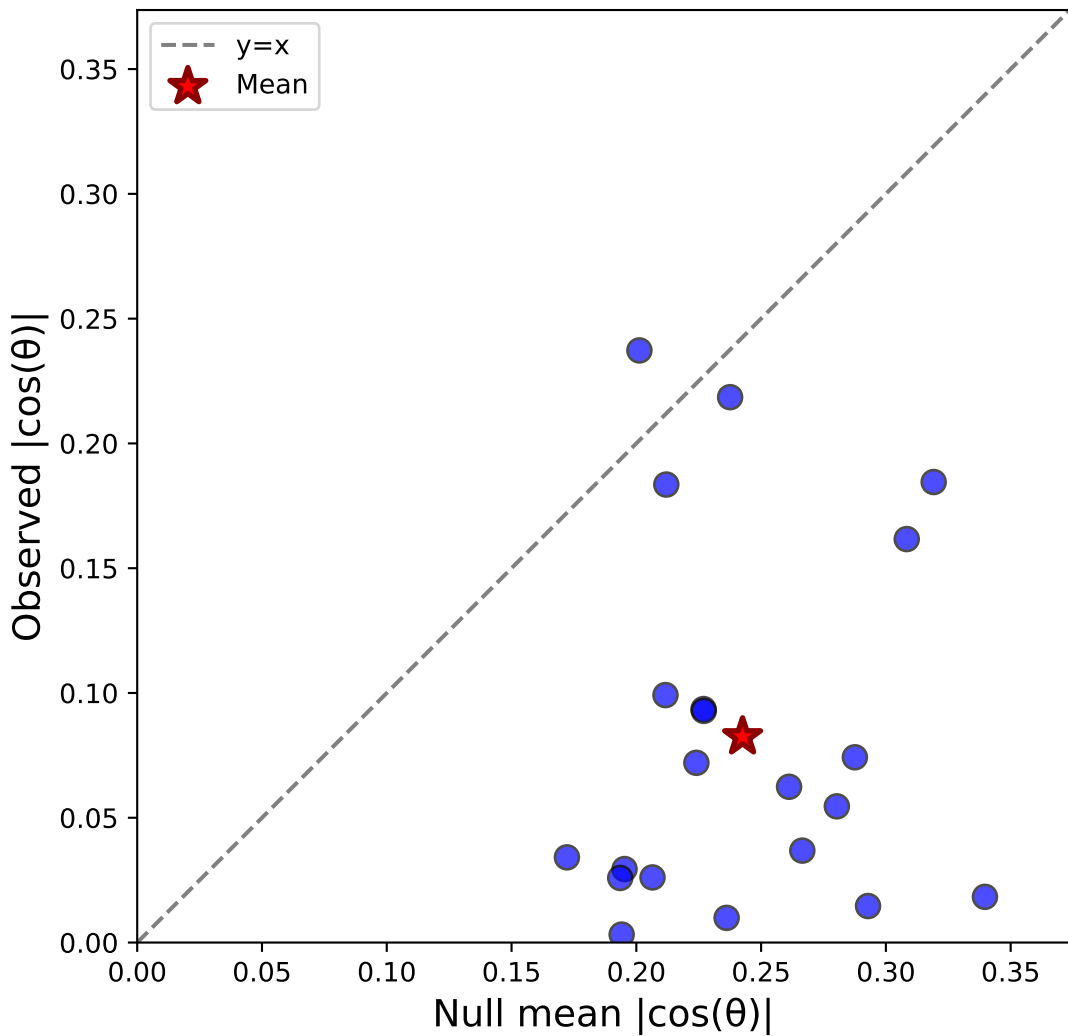
Case i: Sacc C&S (horiz) - Monkey all N=21, \Delta=-0.160 , Sig=4/21
