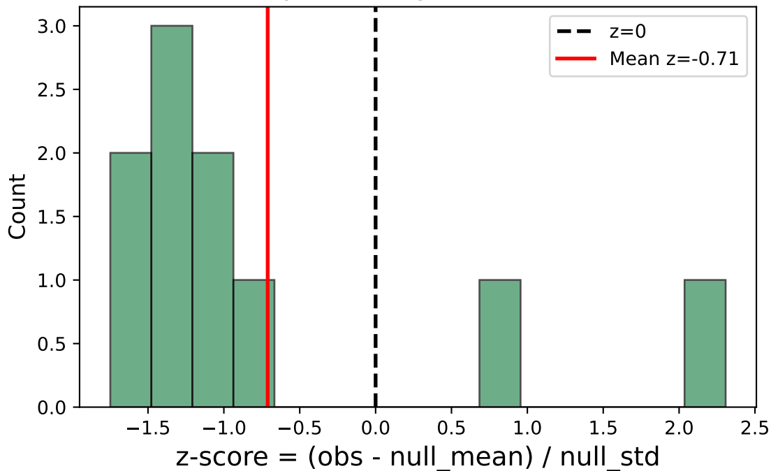
Monkey S: Axis Alignment Effect Size
