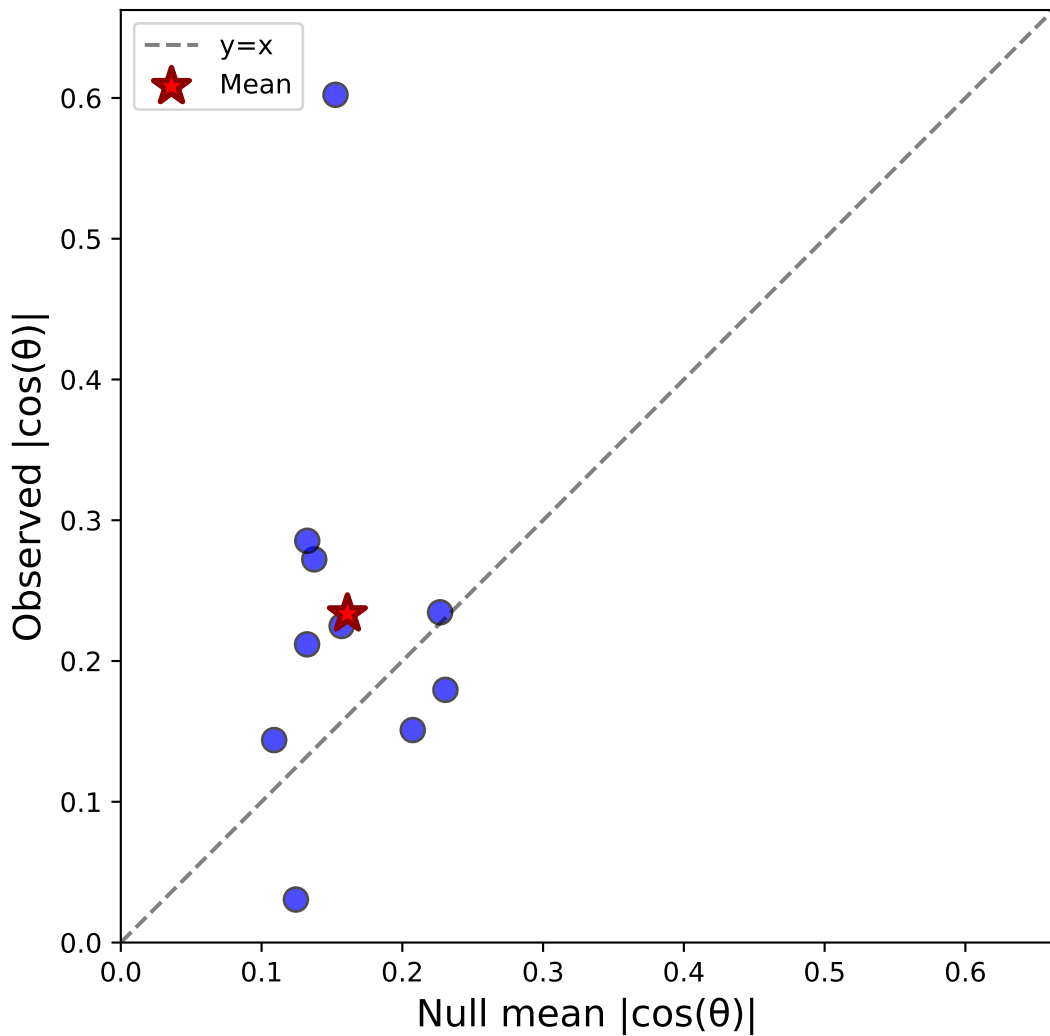
Case iii: Stim-C(ver) vs Sacc-S(horiz) (all) - Monkey S N=10, \Delta=0.073 , Sig=0/10
