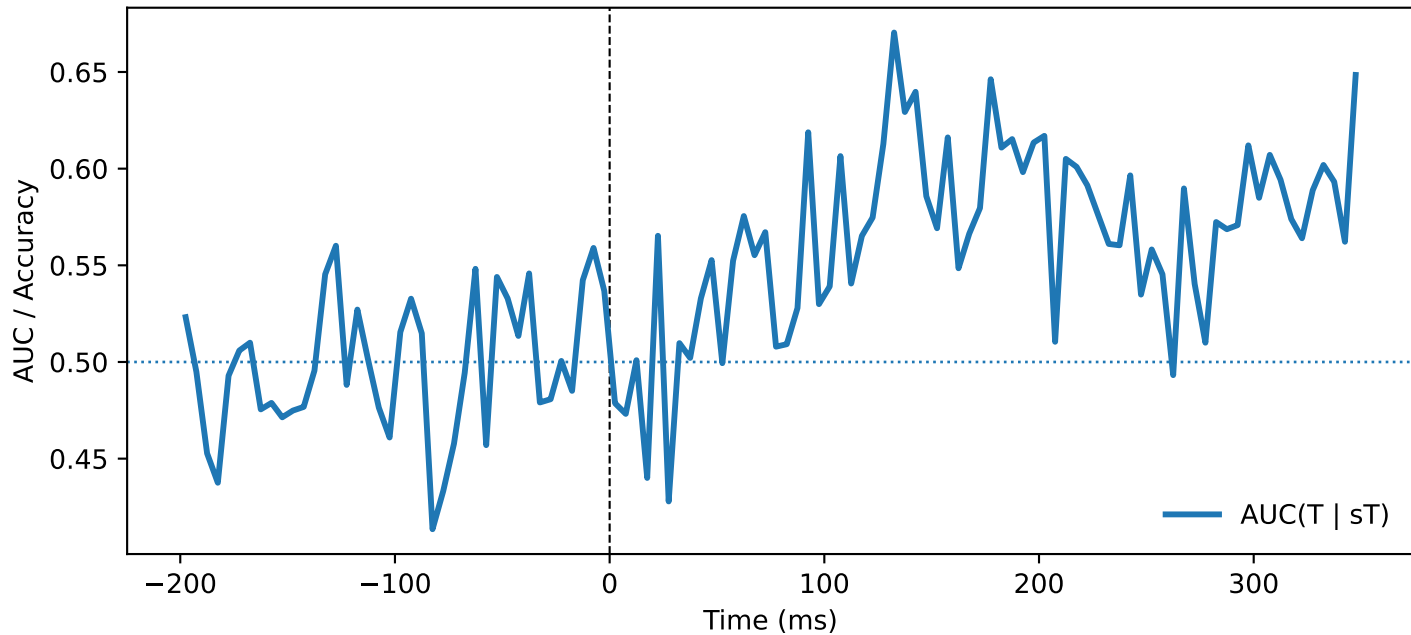
MFEF — QC (targ, ori=horizontal, PT \geq 200.0)
