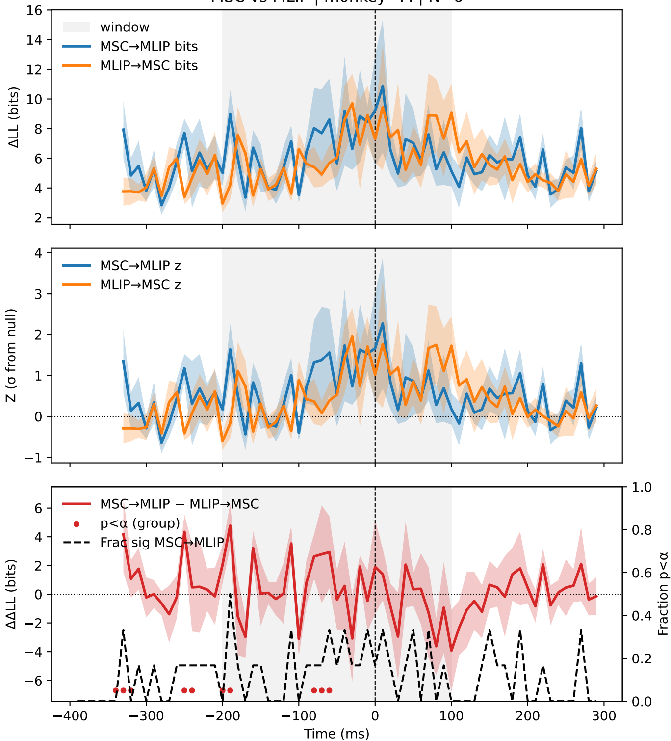
SACC | evoked_peakbin_saccS_horizontal_lag60ms_20mssw-none-trial | S MSC vs MLIP | monkey=M | N=6
