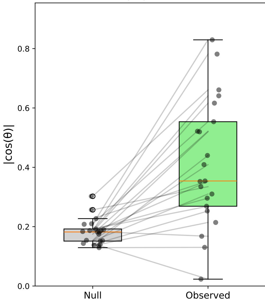
Case iii: Stim-C(ver) vs Sacc-S(horiz) (correct) - Monkey all \Delta|\cos| = 0.231
