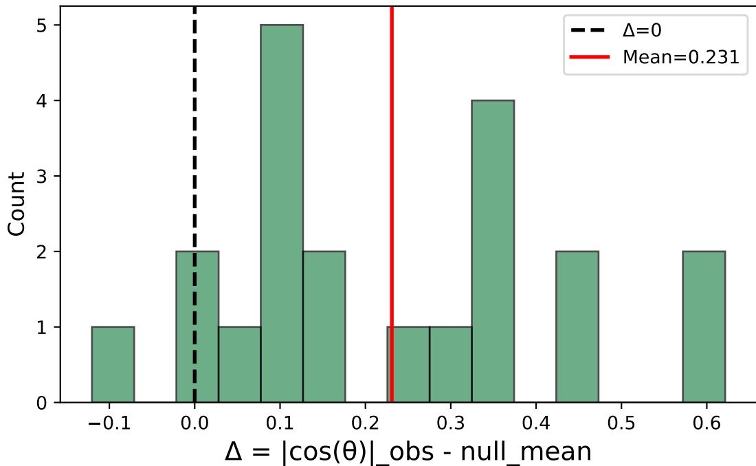
Case iii: Stim-C (vert) vs Sacc-S (horiz) (correct) - Monkey all
