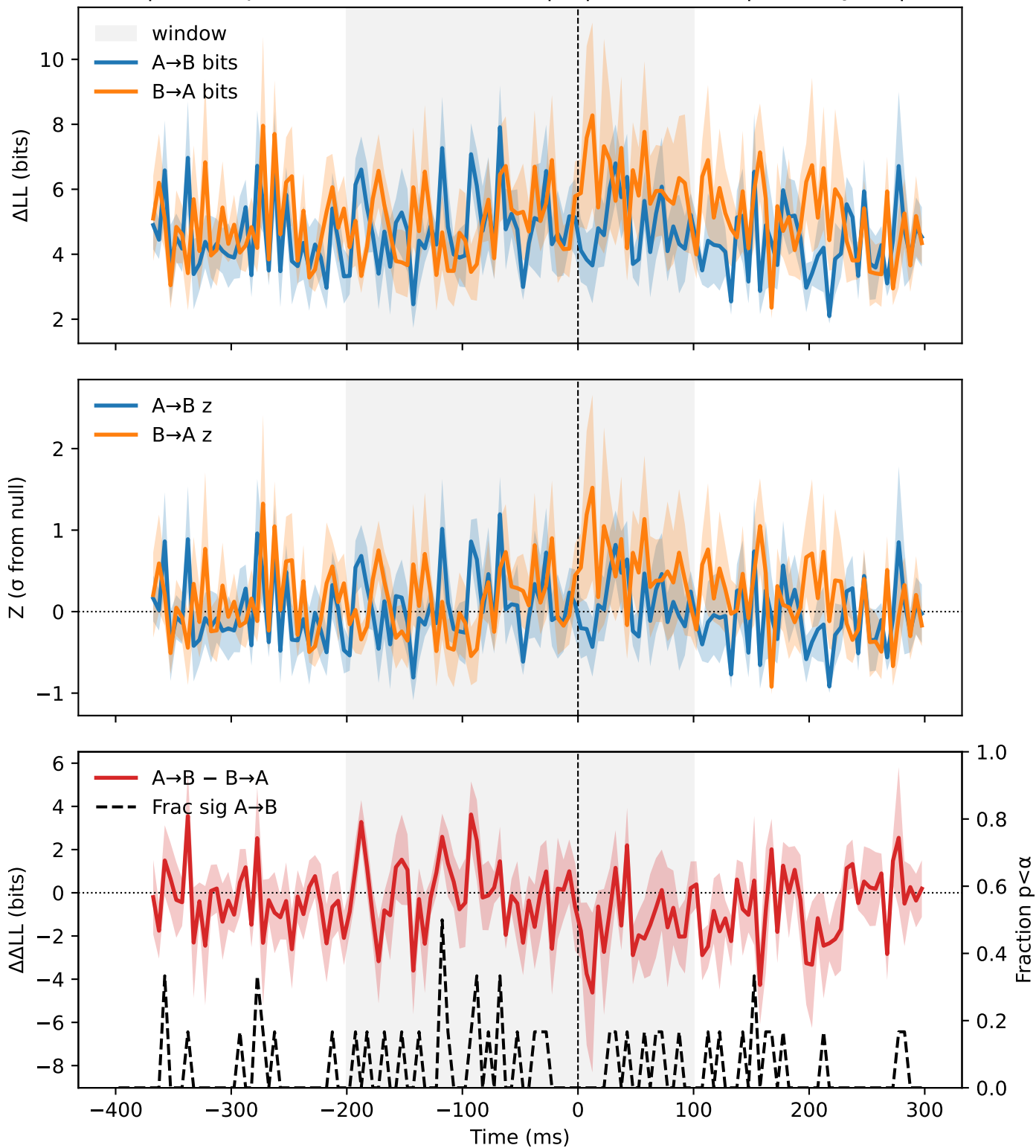
SACC | crsweep-sacc-vertical-none-circ | S | SLIP vs SSC | monkey=S | N=6
