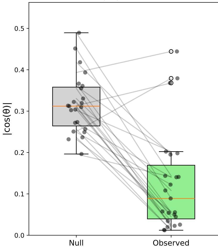
Case iii: Sacc C&S (vert) - Monkey all \Delta|\cos| = -0.191
