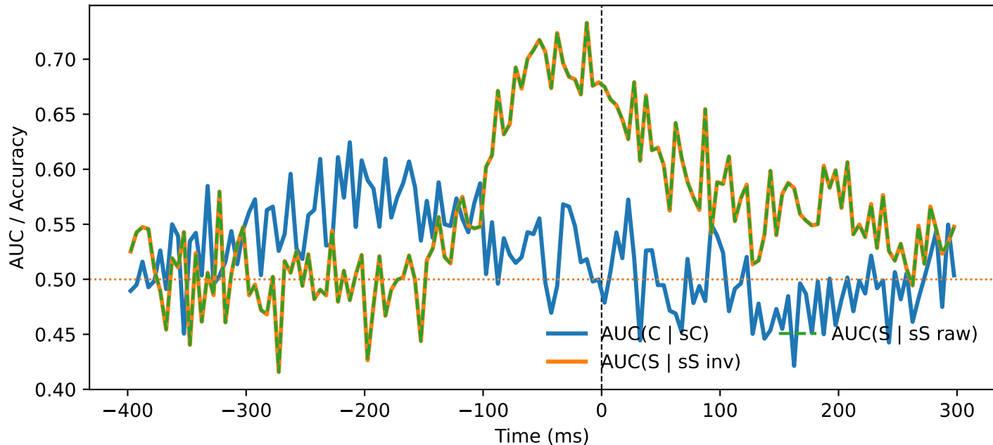
SFEF — QC (sacc, ori=horizontal, PT \geq 200.0)
