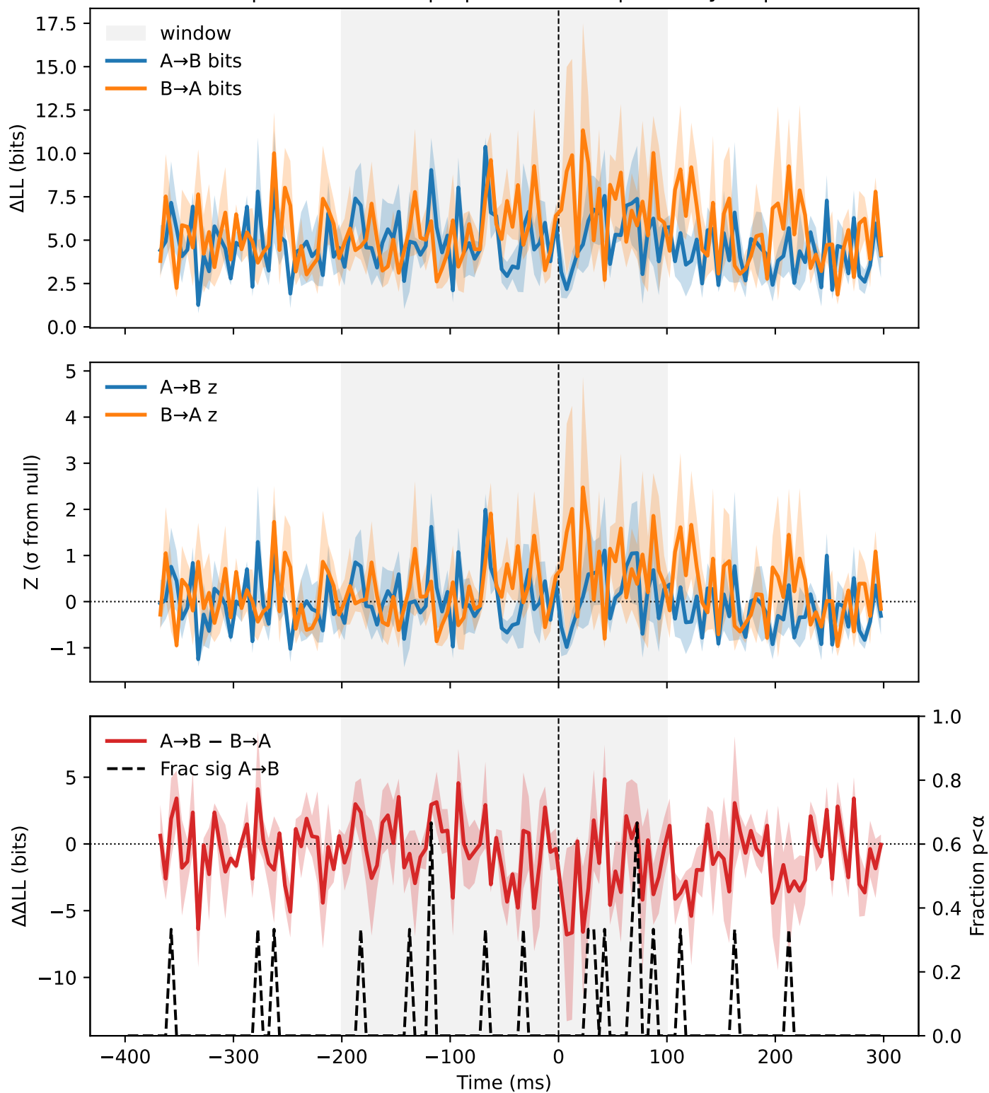
SACC | crnull-vertical | S | SLIP vs SSC | monkey=S | N=3
