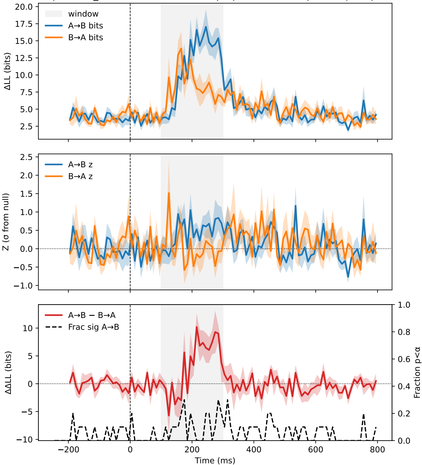
STIM | evoked_subtract-stim-none-trial | C | MFEF vs MLIP | monkey=M | N=10
