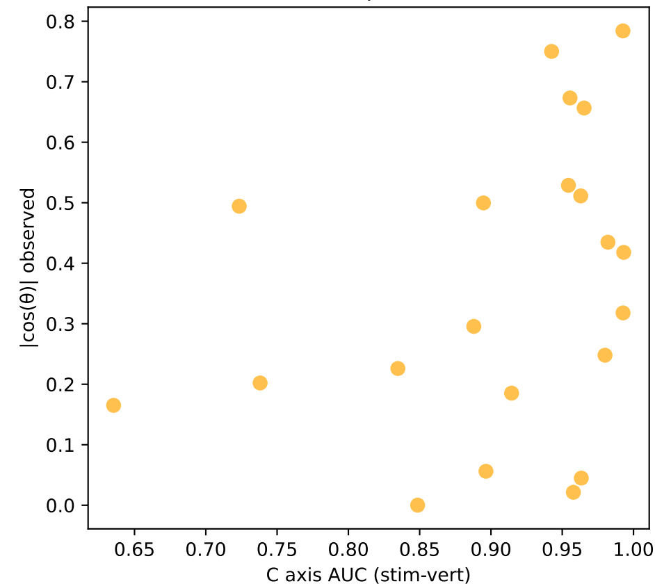
a_obs vs auc_C r=0.311 , p=0.1697
