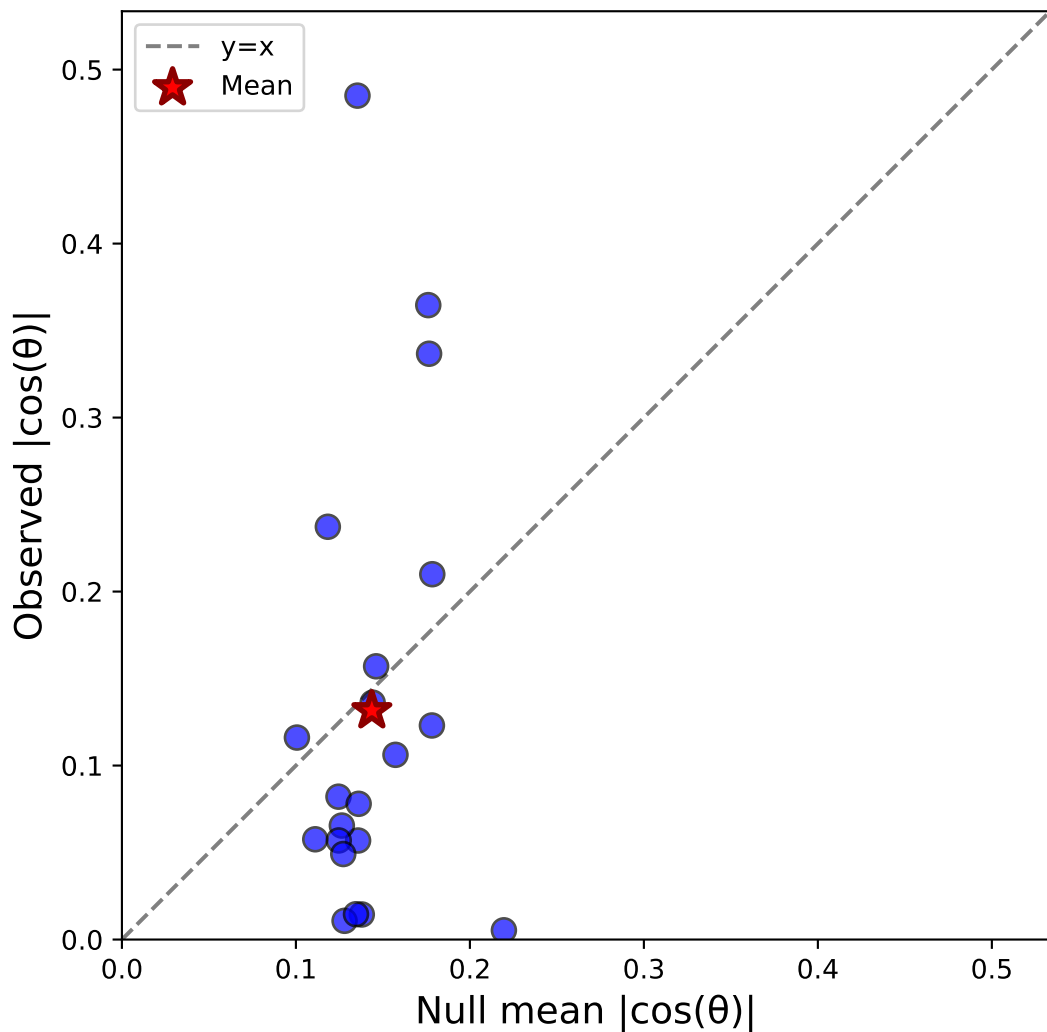
Case v: Stim-C(horiz) vs Sacc-S(horiz) (correct) - Monkey all N=21, \Delta=-0.012
