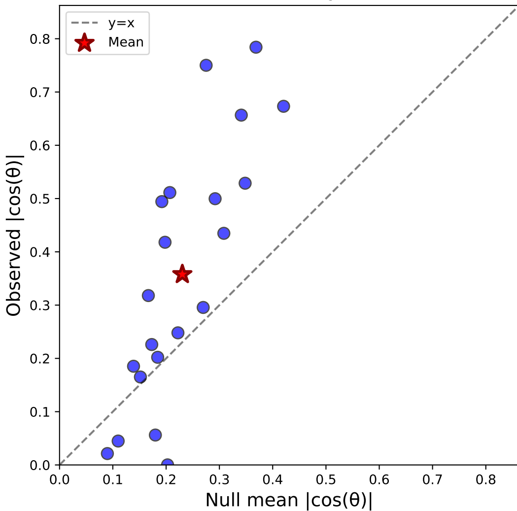
Case vi: Stim-C(vert) vs Sacc-S(horiz) - Monkey all N=21, \Delta=0.127 , Sig=1/21
