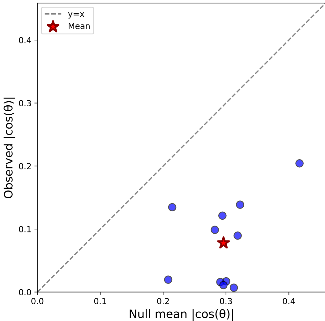
Case vi: Sacc C&S (vert, all) - Monkey M N=11, \Delta=-0.218 , Sig=4/11
