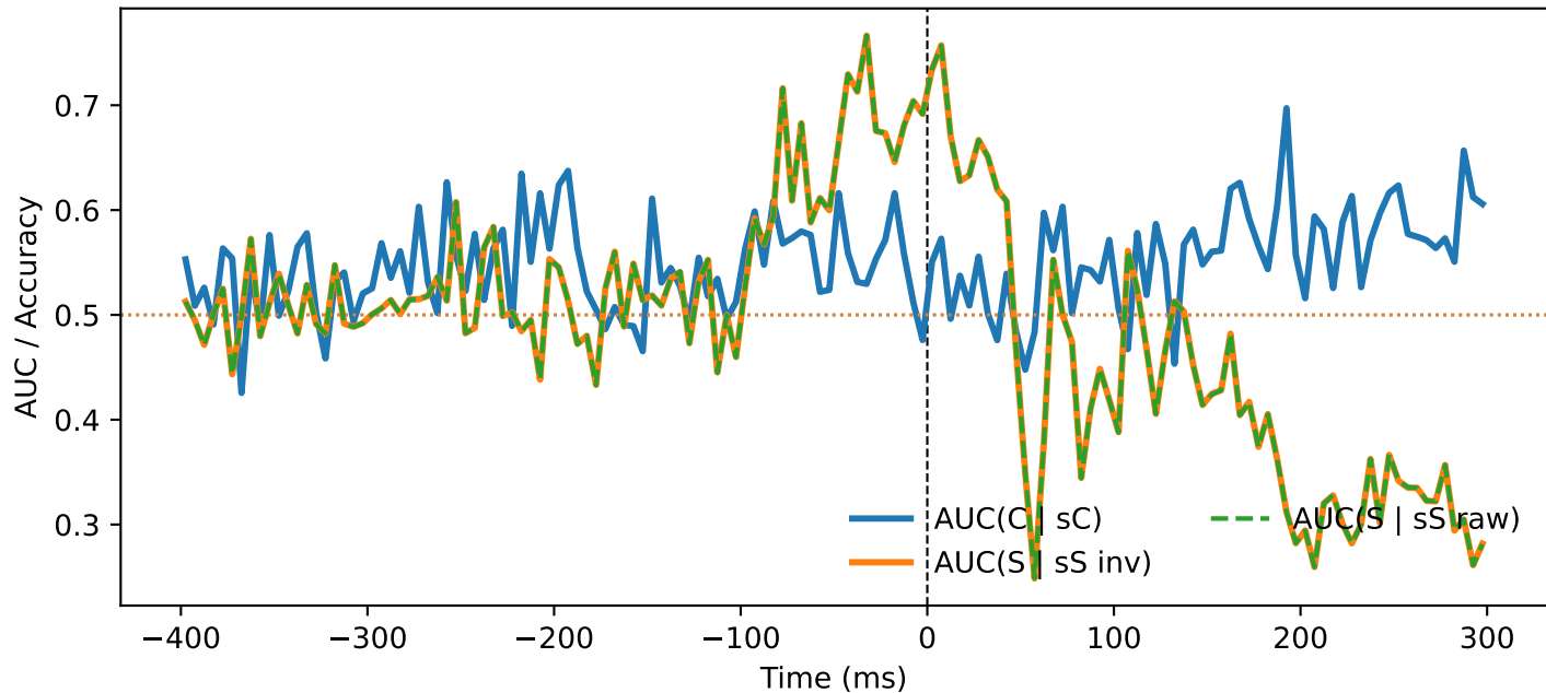
MLIP — QC (sacc, ori=vertical, PT \geq 200.0)
