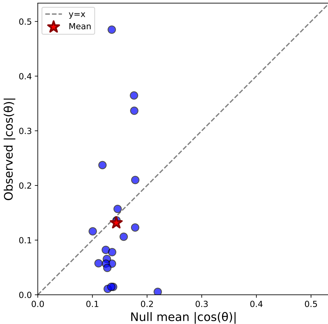
Case iv: Stim-C(horiz) vs Sacc-S(horiz) - Monkey all N=21, \Delta=-0.012 , Sig=2/21
