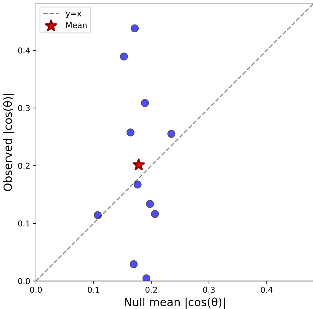
Case iv: Stim-C vs Sacc-S pooled (all) - Monkey M N=11, \Delta=0.023\pm0.042
