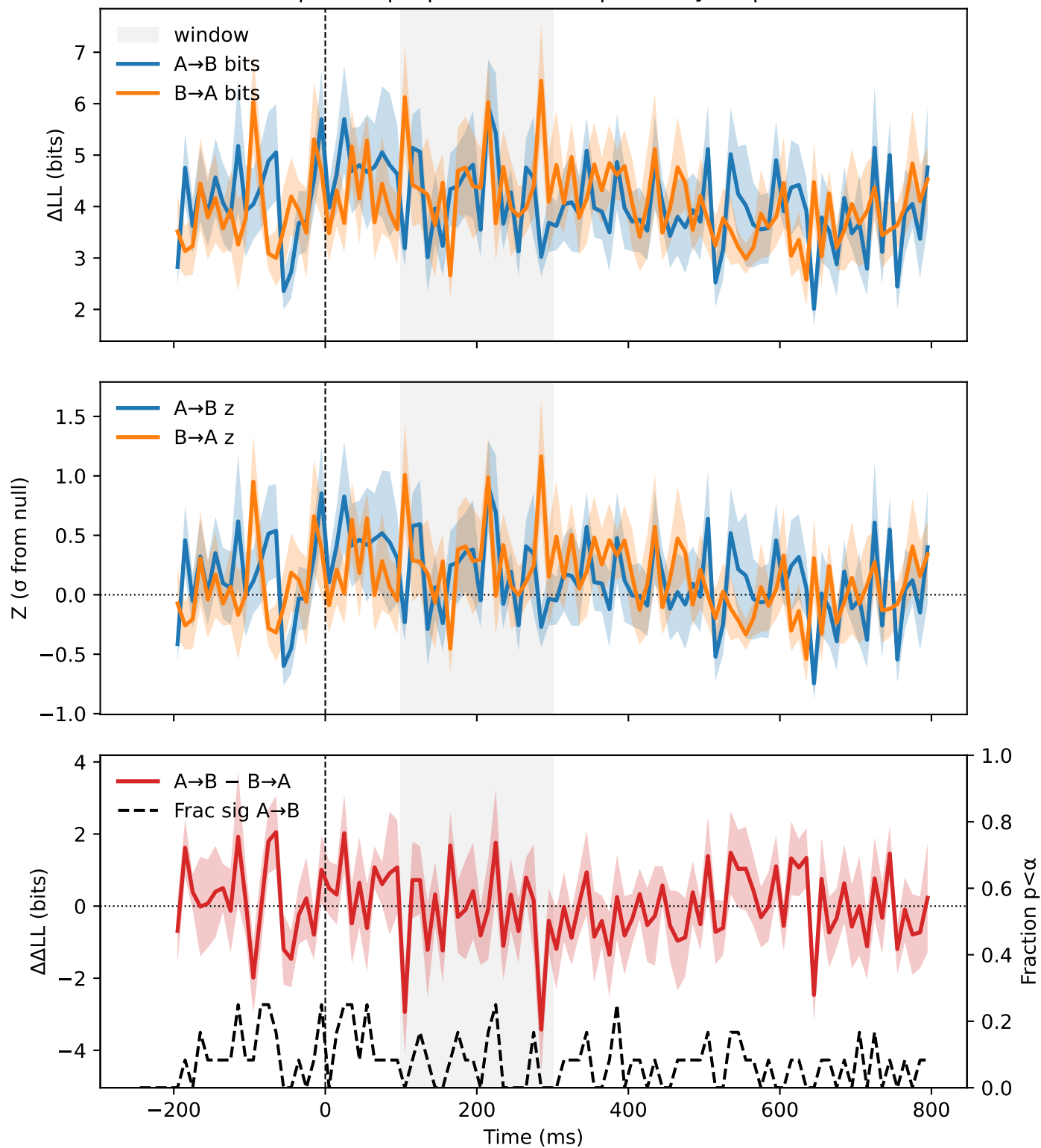
STIM | crnull | C | SFEF vs SLIP | monkey=S | N=12
