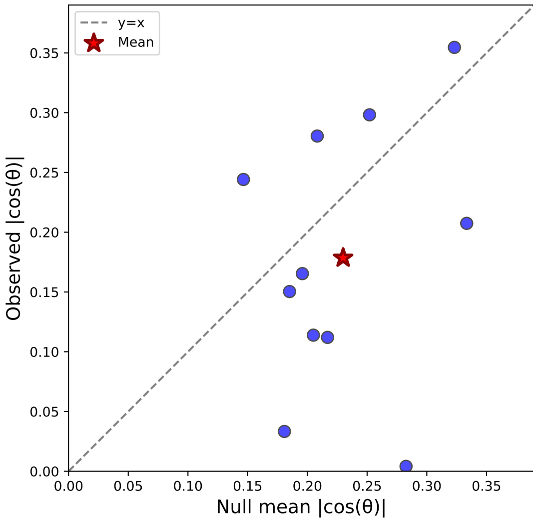
Case v: Stim-C(pool) vs Sacc-S(pool) - Monkey M N=11, \Delta=-0.051 , Sig=1/11
