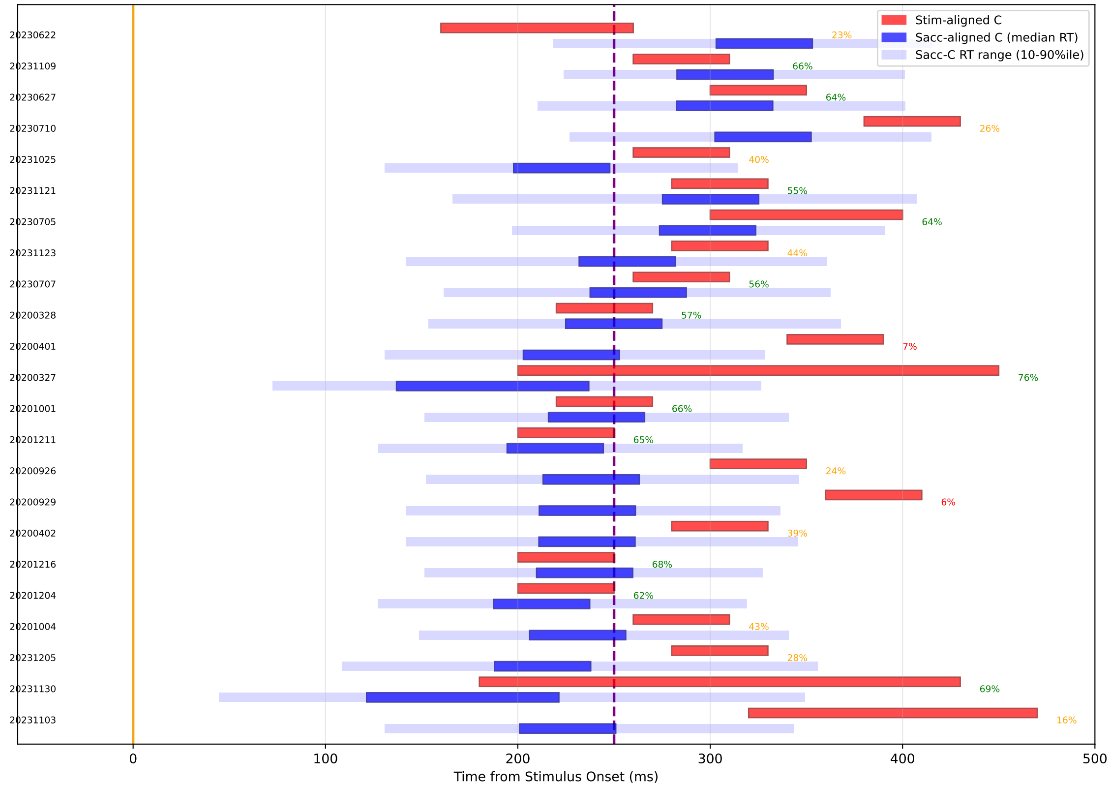
Case iii vs vi: Vertical (correctly) Sacc-C (blue) vs Stim-C (red) (% = fraction of trials with C window overlap)
