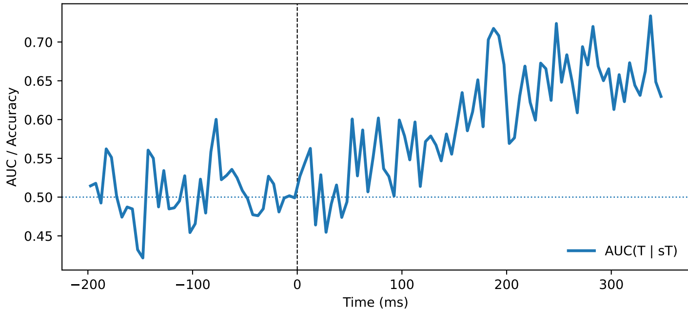
MFEF — QC (targ, ori=vertical, PT \geq 200.0)
