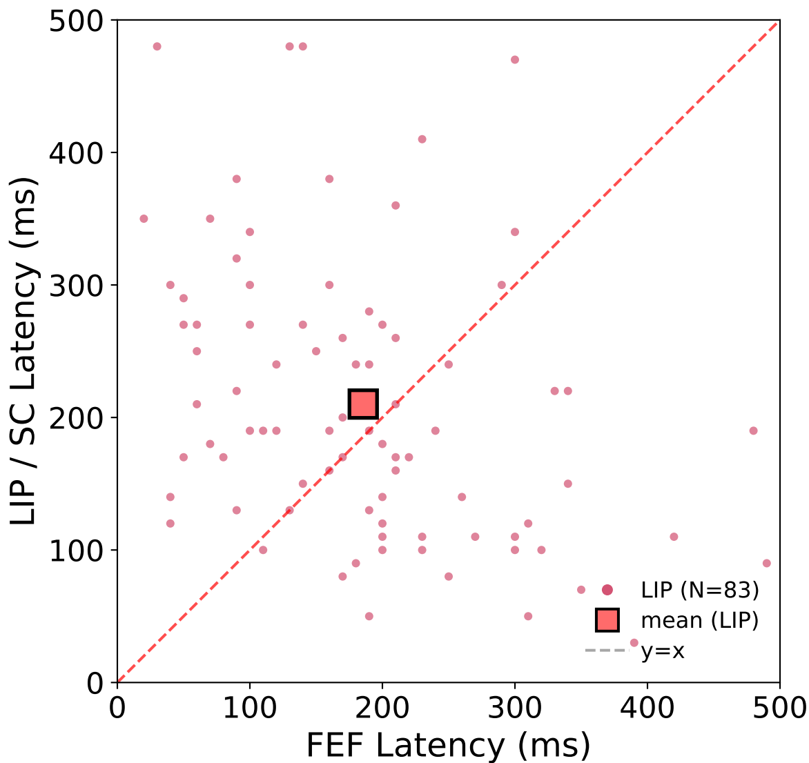
Monkey M - (LIP & SC) vs FEF - direction [stim] LIP-FEF: 3 sess, mean(LIP-FEF)=24.6ms
