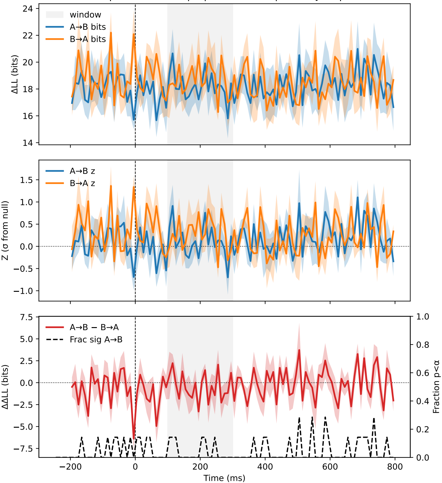
STIM | crnull-vertical | R | SFEF vs SSC | monkey=S | N=7
