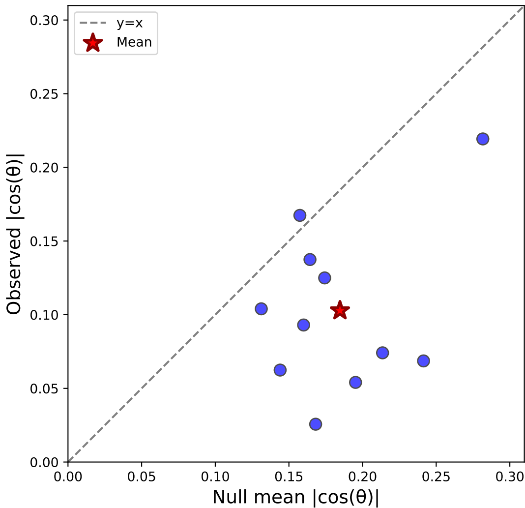
Case i: Sacc C&S (horiz, all) - Monkey M N=11 , \Delta=-0.082\pm0.017
