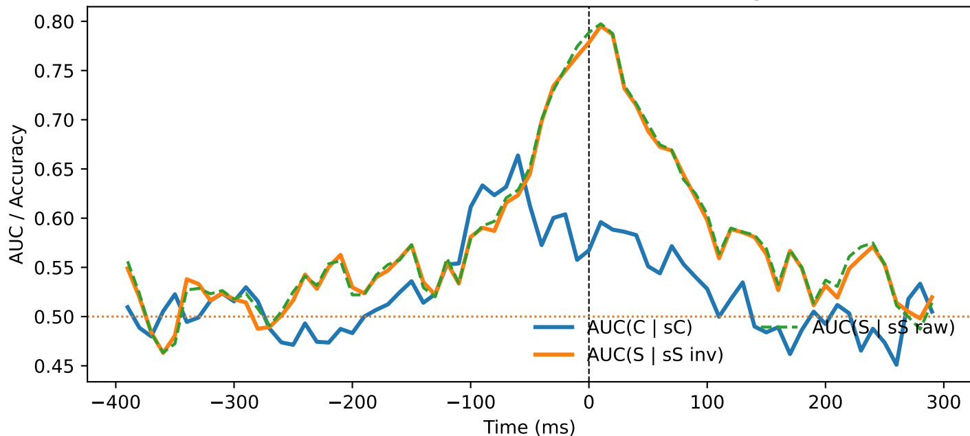
SFEF — QC (sacc, ori=None, PT \geq 200.0, norm=global)
