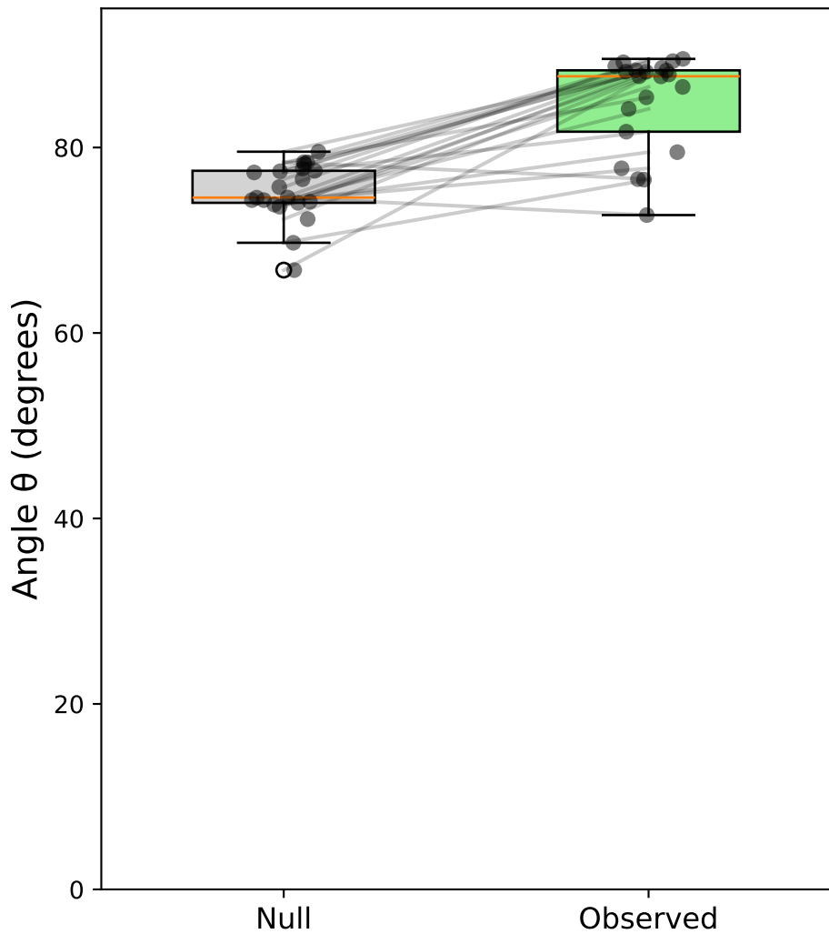
Case i: Sacc C&S (horiz, correct) - Monkey all \Delta\theta = 9.7^\circ
