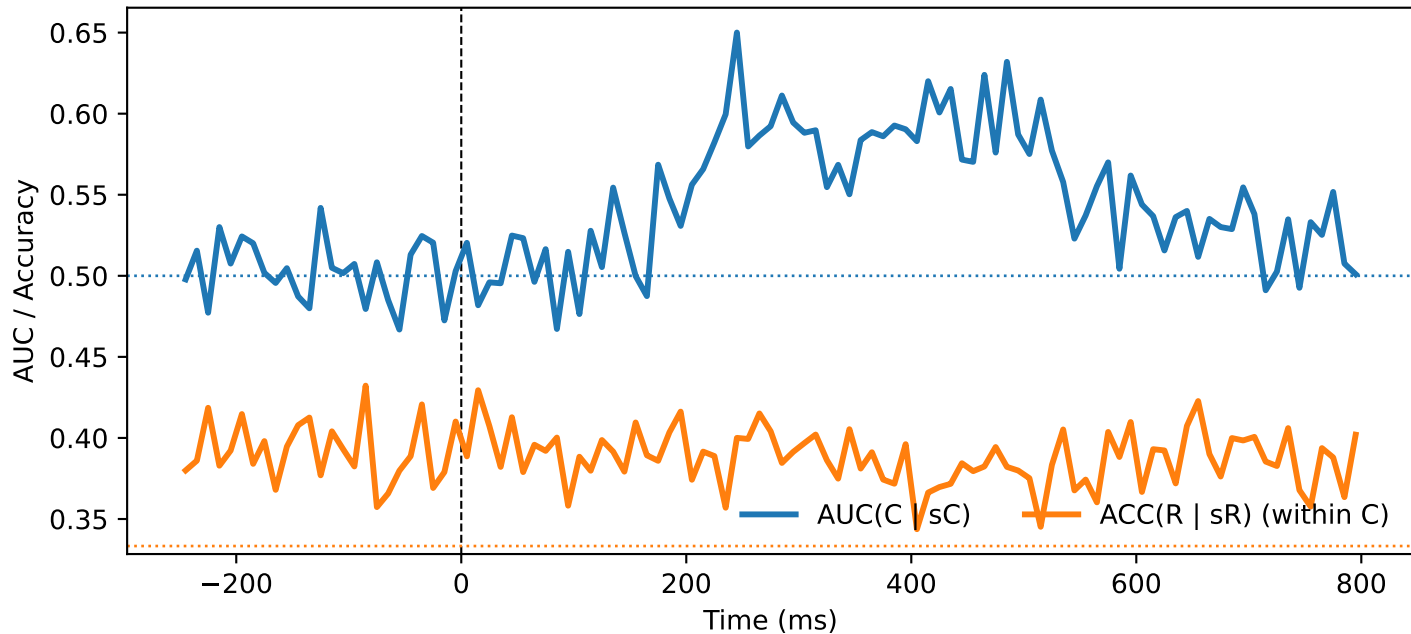
SSC — QC (stim, ori=None, PT \geq 200.0)
