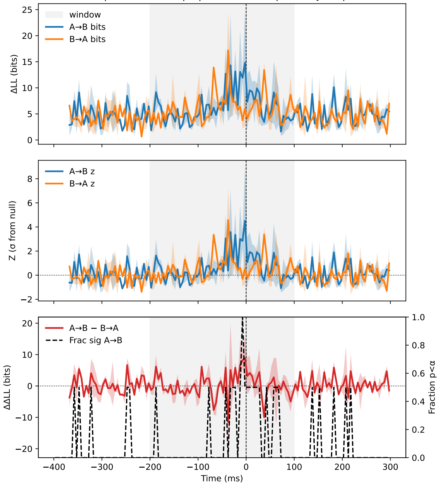
SACC | crnull-vertical | S | MFEF vs MLIP | monkey=M | N=2
