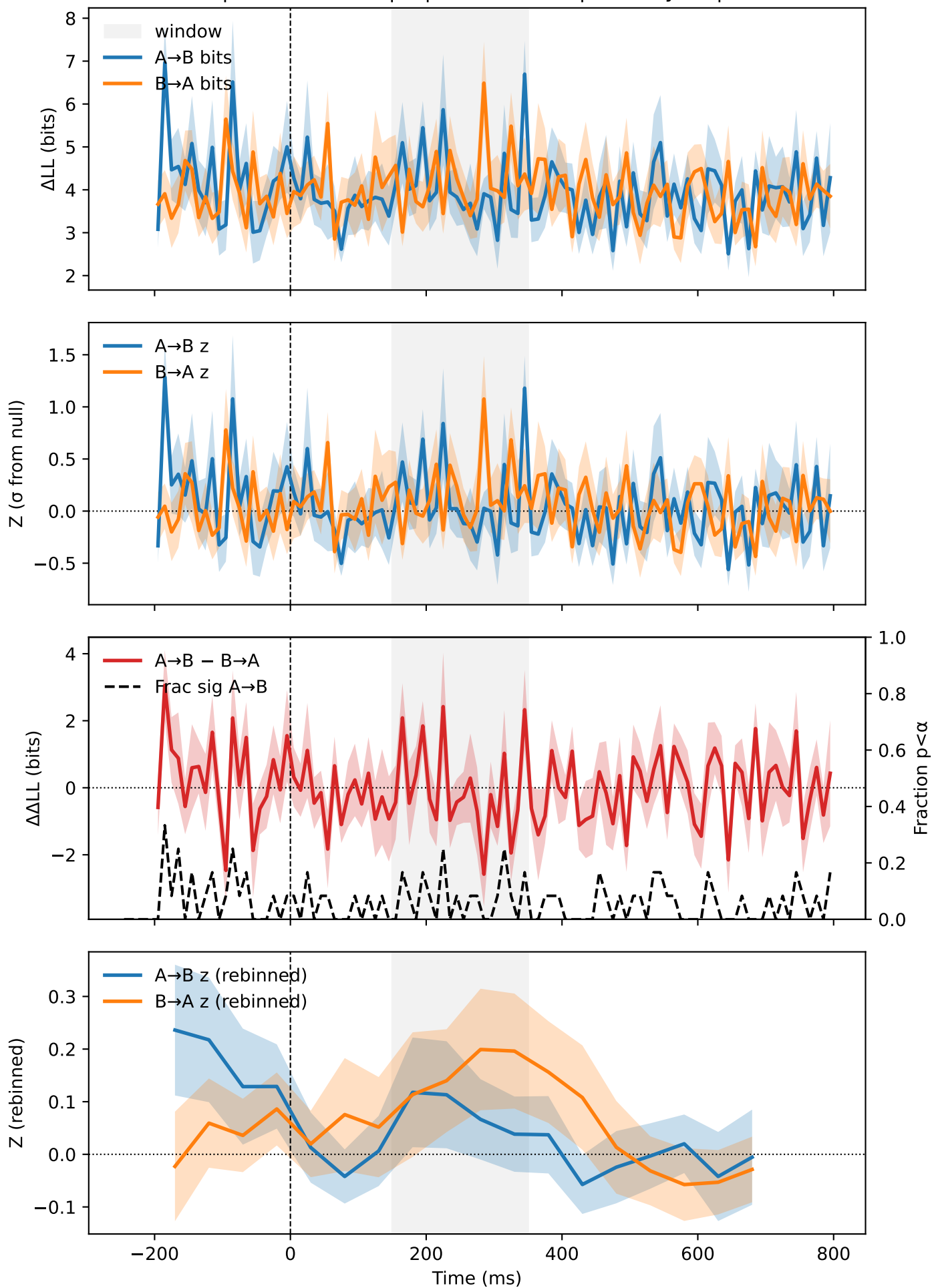
STIM | crnull-vertical | C | SFEF vs SLIP | monkey=S | N=12
