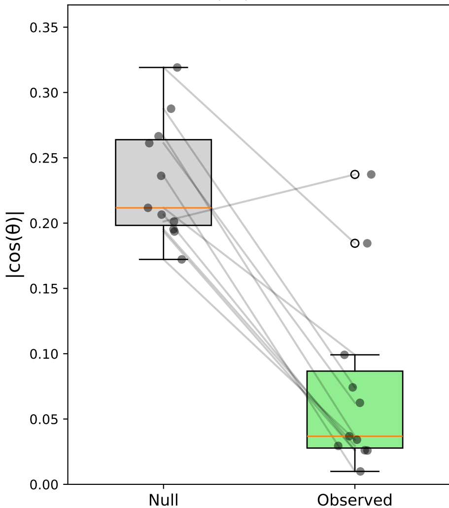
Case i: Sacc C&S (horiz) - Monkey M \Delta|\cos| = -0.157
