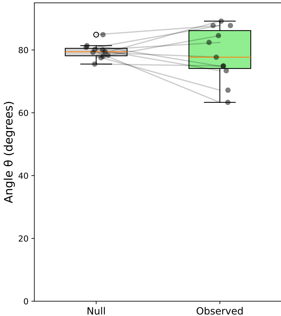
Case iv: Stim-C vs Sacc-S pooled (correct) - Monkey M \Delta\theta = -1.1^\circ
