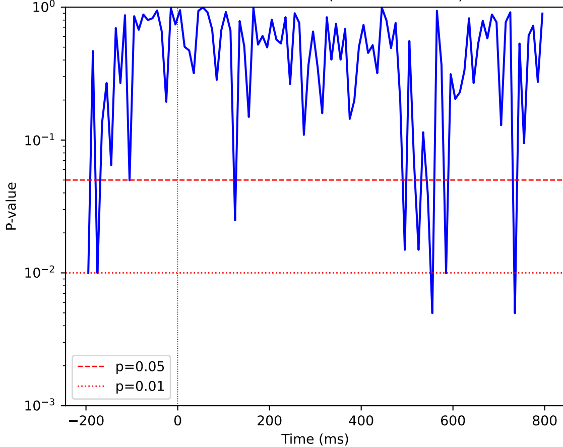
P-values Over Time (Cross-Validated)
