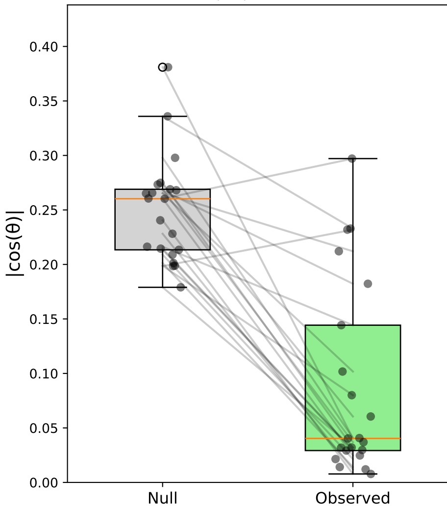
Case i: Sacc C&S (horiz) - Monkey all \Delta|\cos| = -0.161
