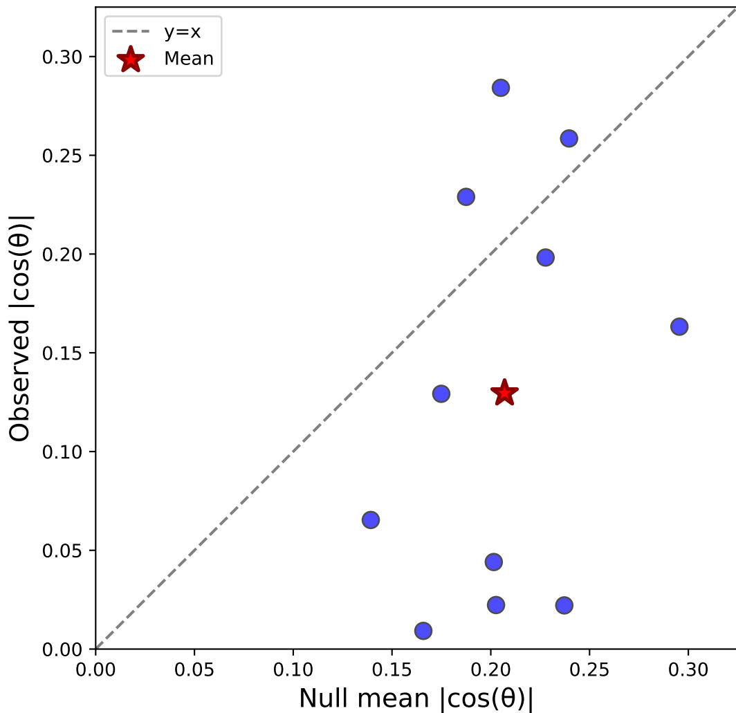
Case ii: Sacc C&S (pooled, all) - Monkey M N=11, \Delta=-0.077\pm0.028
