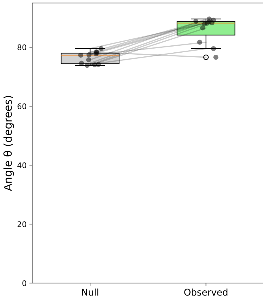
Case i: Sacc C&S (horiz, correct) - Monkey M \Delta\theta = 9.4^\circ
