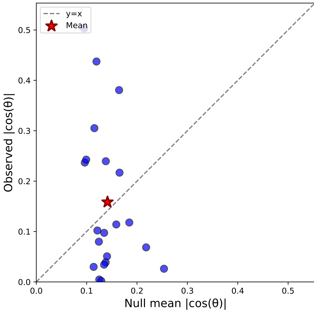
Case v: Stim-C(horiz) vs Sacc-S(horiz) (all) - Monkey all N=21, \Delta=0.017
