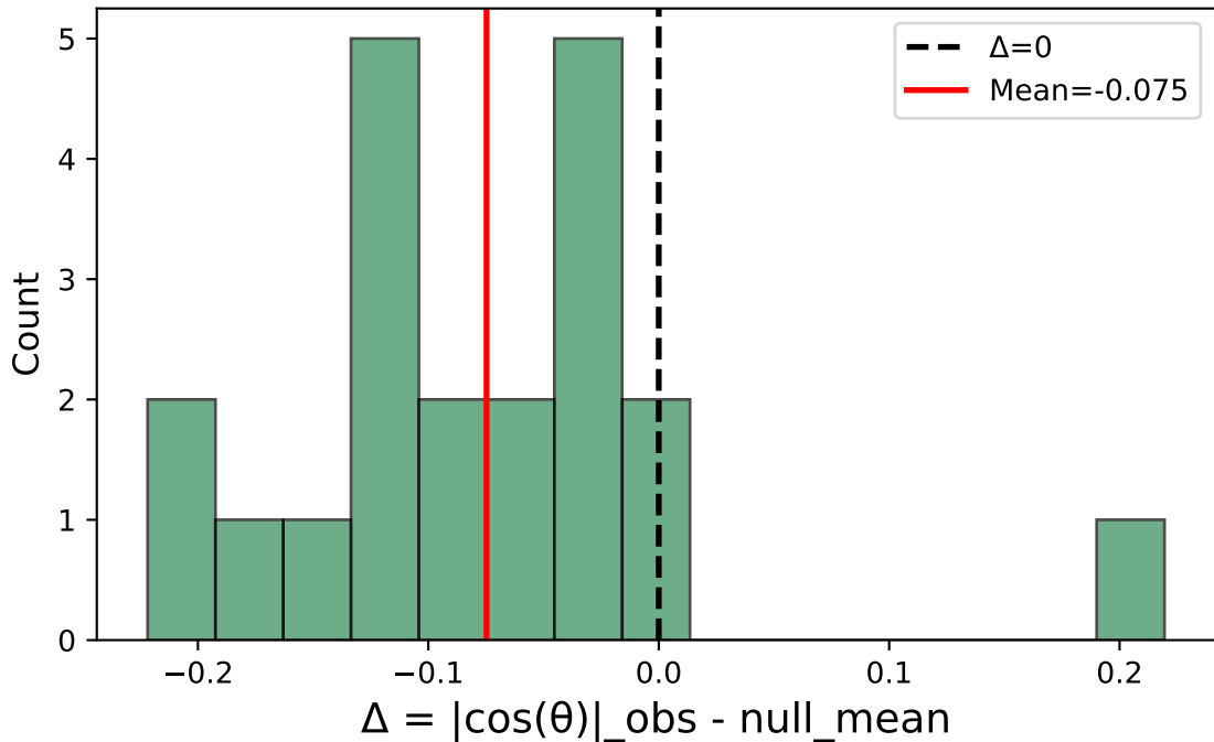
Monkey all: Axis Alignment \Delta (covariance null)
