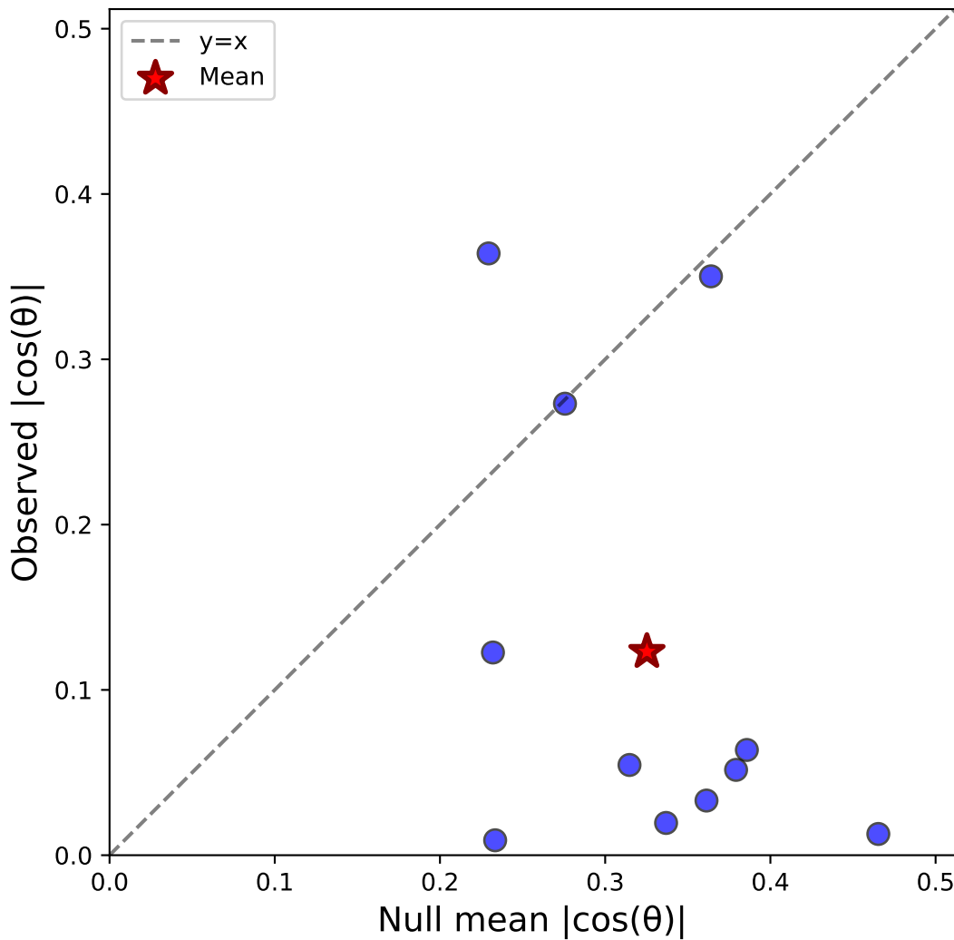
Case ii: Sacc C&S (pooled) - Monkey S N=11, \Delta=-0.202 , Sig=4/11
