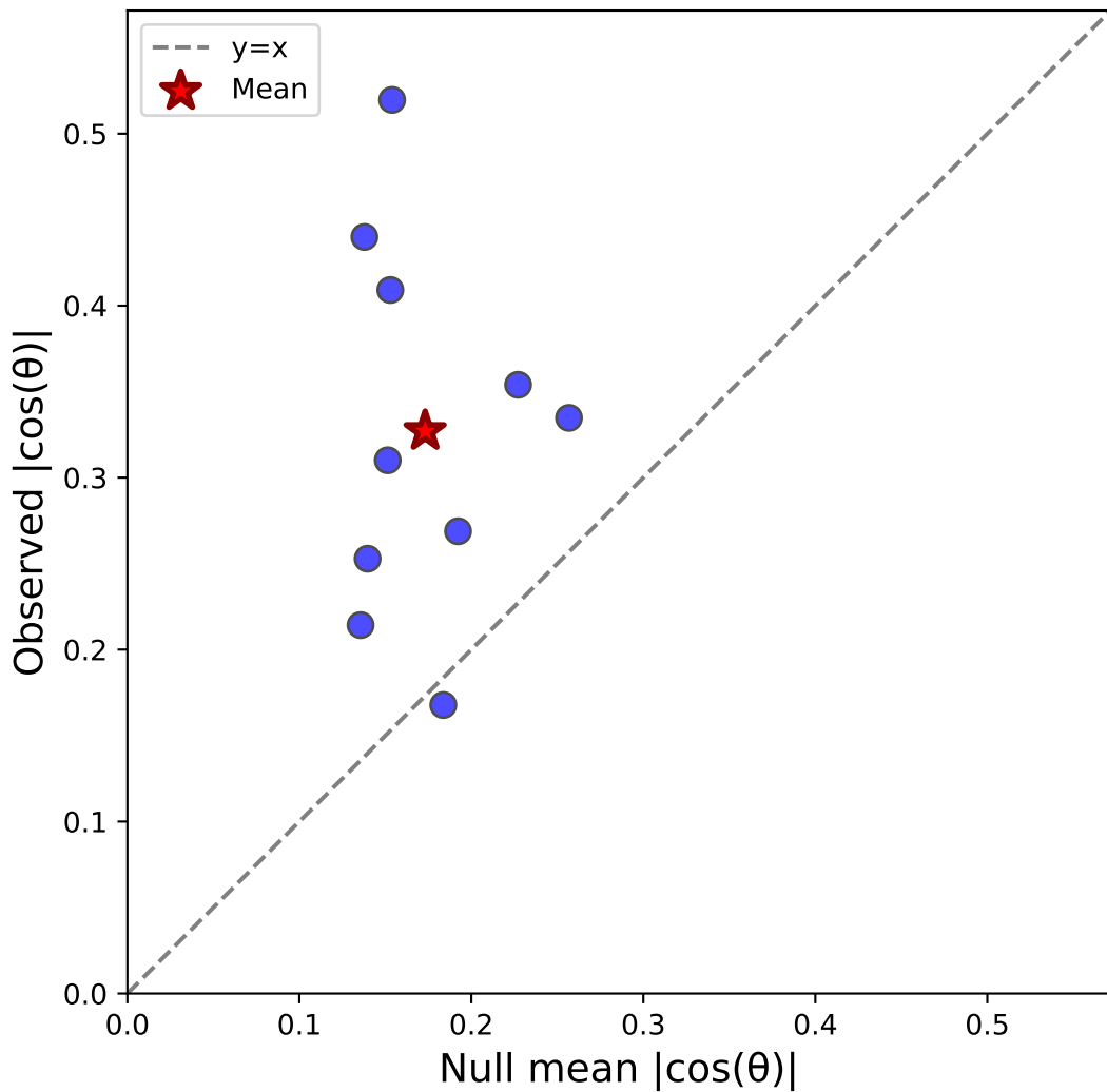
Case iii: Stim-C(vert) vs Sacc-S(horiz) (correct) - Monkey S N=10, \Delta=0.154 , Sig=0/10
