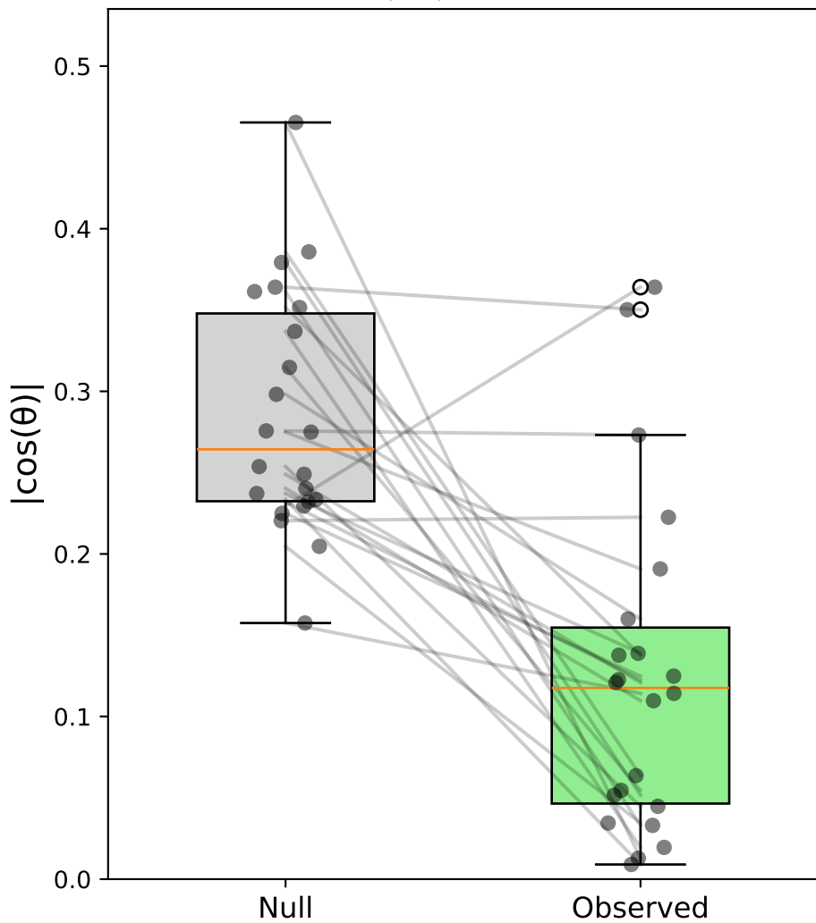
Case ii: Sacc C&S (pooled) - Monkey all \Delta|\cos| = -0.161
