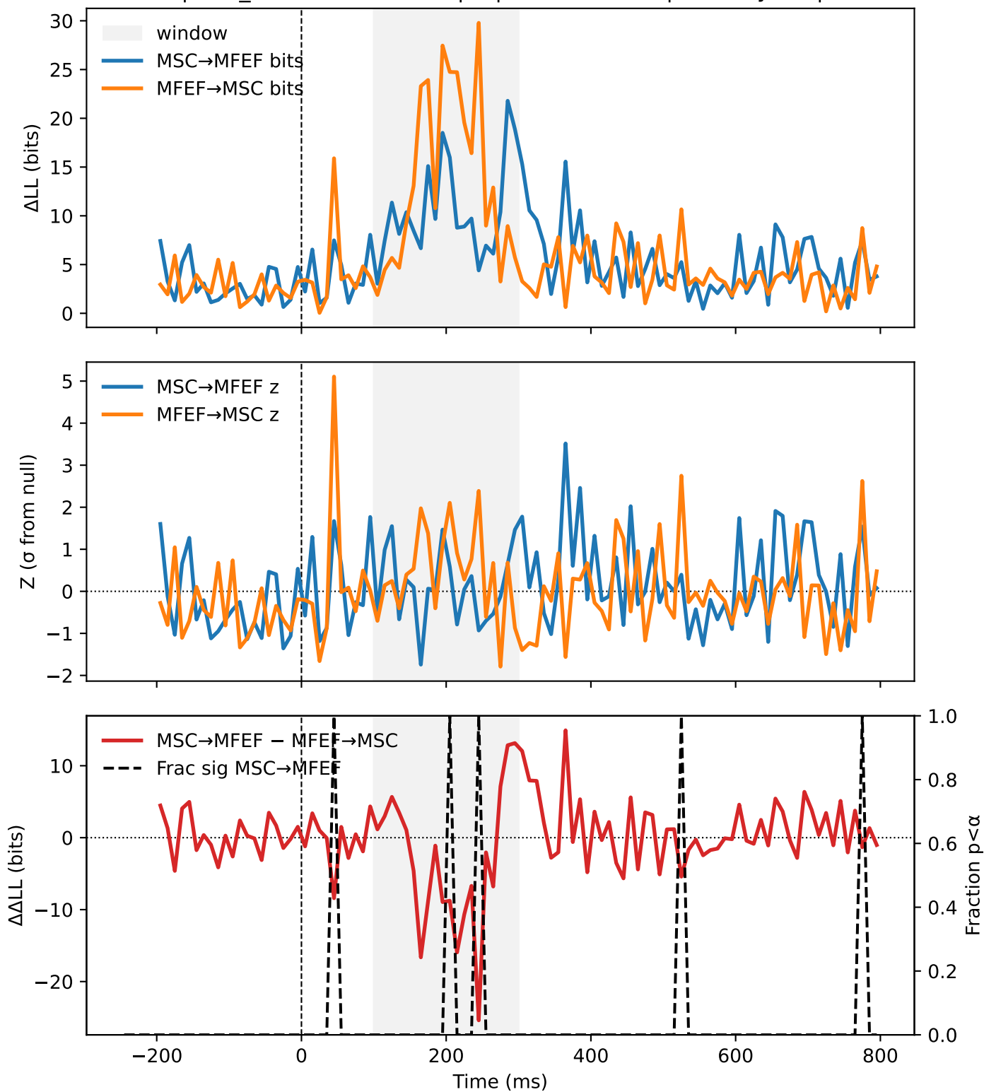
STIM | test_evoked-none-trial | C | MSC vs MFEF | monkey=M | N=1
