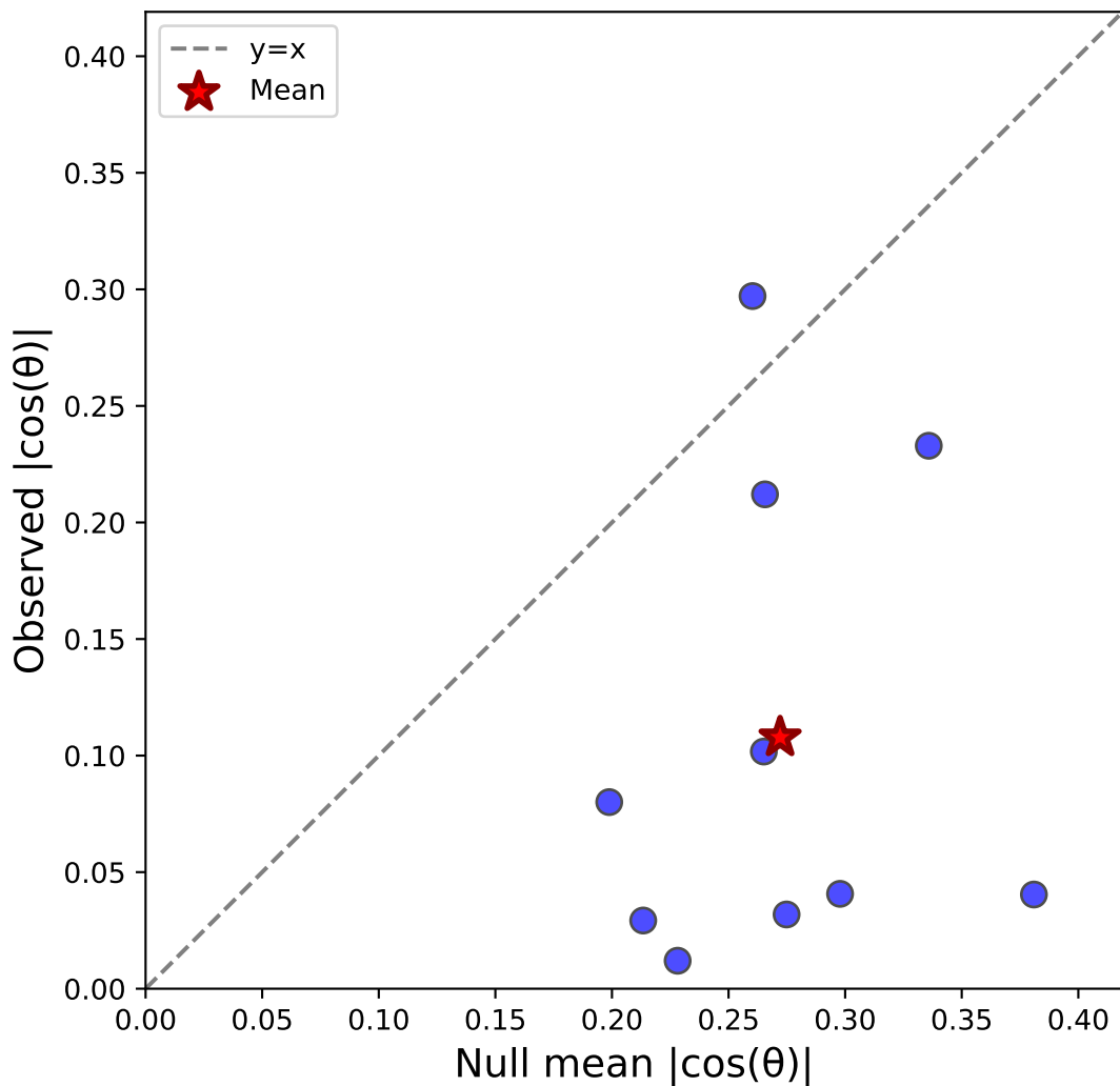
Case i: Sacc C&S (horiz, correct) - Monkey S N=10, \Delta=-0.164
