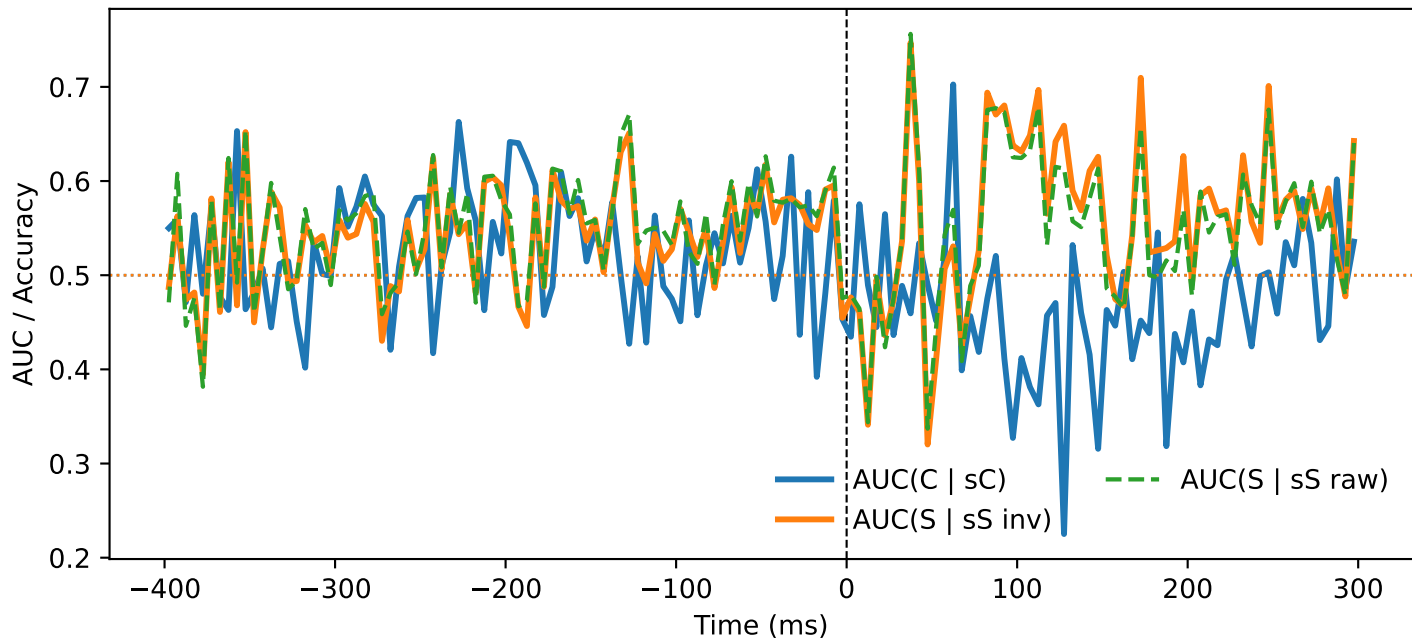
SSC — QC (sacc, ori=vertical, PT \geq 200.0)
