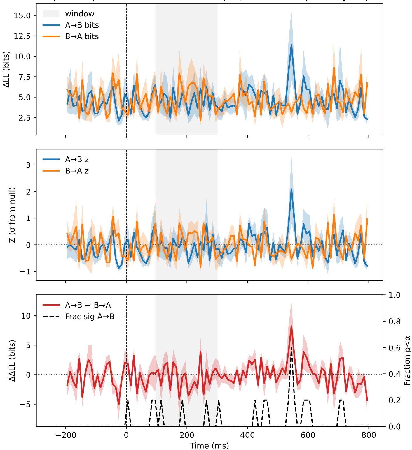
STIM | crsweep-stim-horizontal-none-trial | C | SFEF vs SSC | monkey=S | N=5
