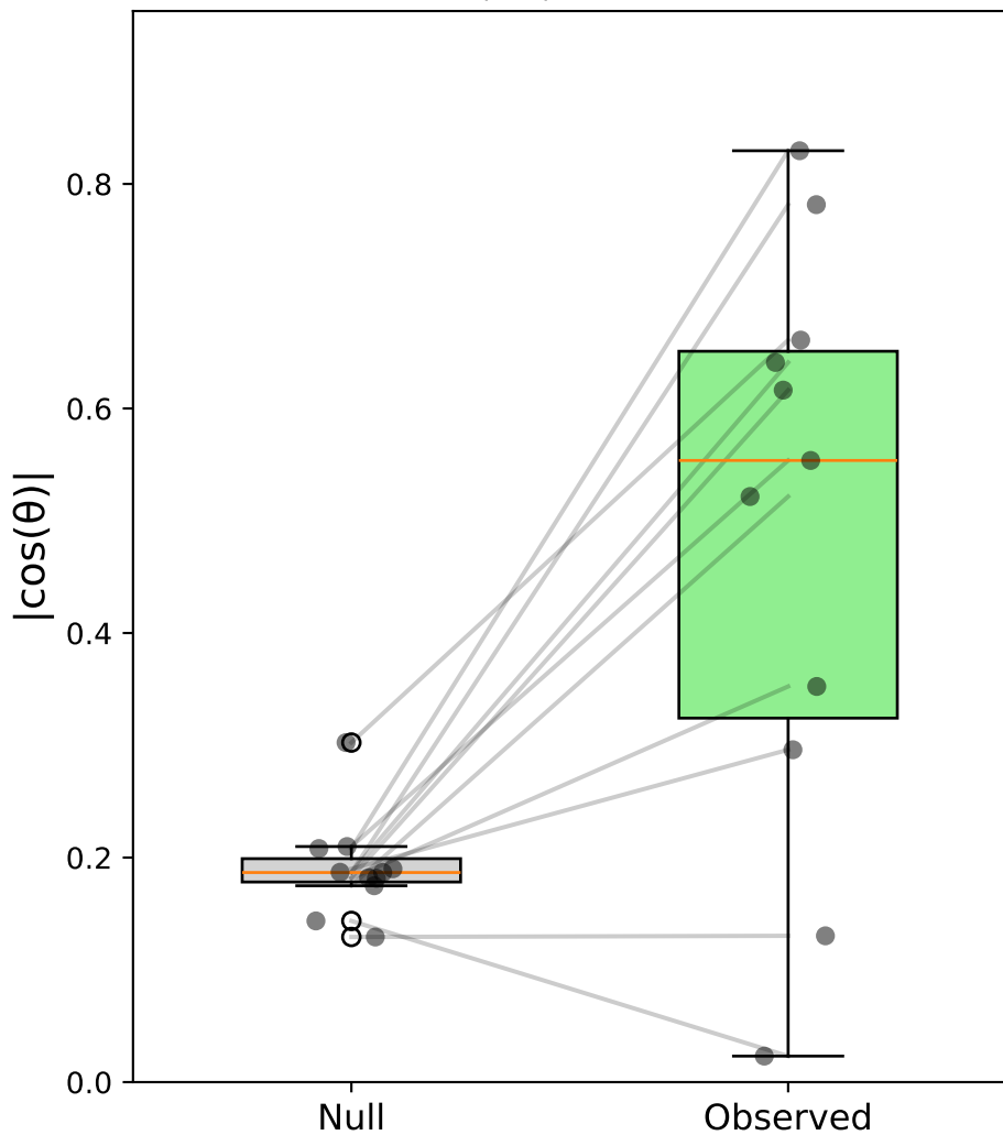
Case vi: Stim-C(ver) vs Sacc-S(horiz) - Monkey M \Delta|\cos| = 0.301
