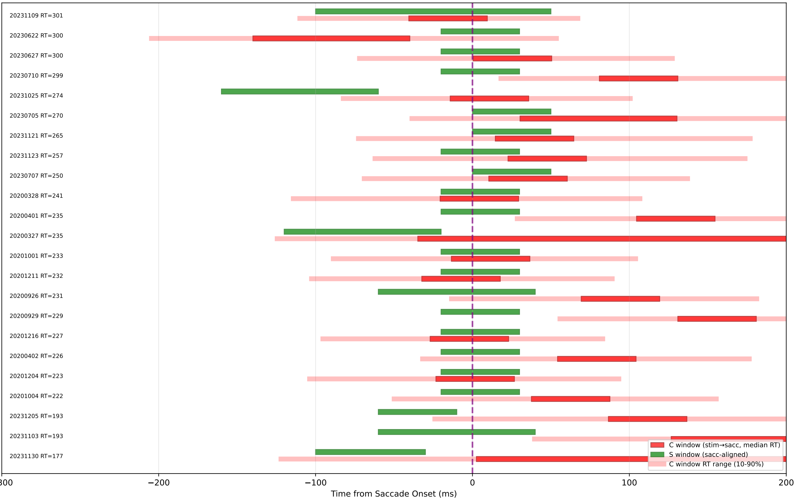
Case vi: Stim-C(ver) & Sacc-S(horiz) → Sacc Timeline (alltrials)
