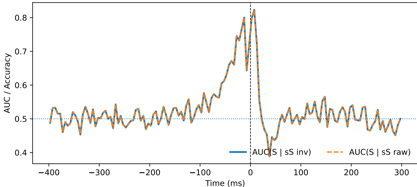
SSC — QC (sacc, ori=vertical, PT \geq 200.0, norm=global)
