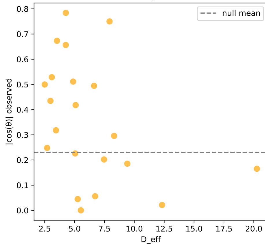
a_obs vs D_eff r=-0.391 , p=0.0794
