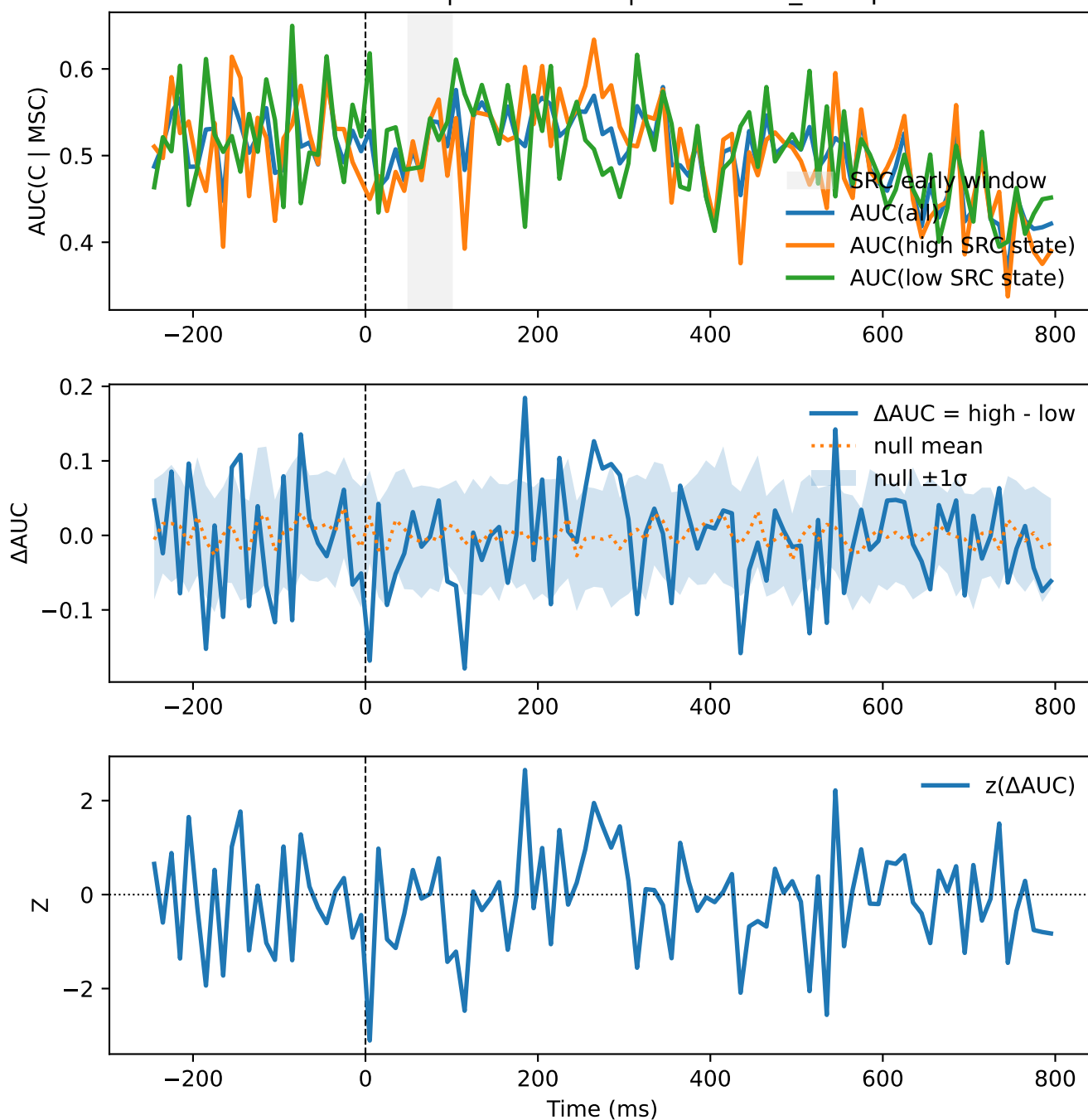
20201004 MFEF→MSC | ori=vertical | axes=axes_sweep-stim-vertical
