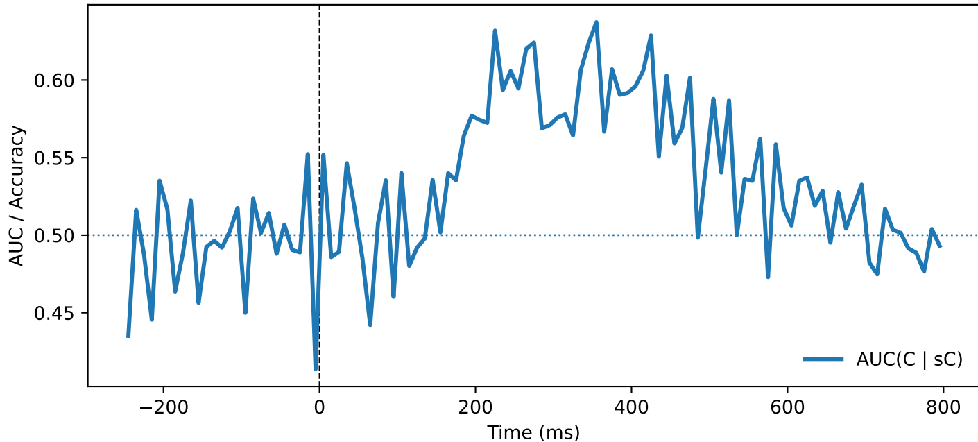
SSC — QC (stim, ori=vertical, PT \geq 200.0, norm=global)
