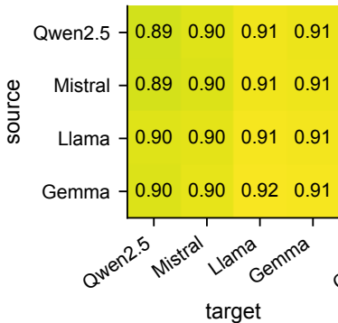
(a) Procrustes
