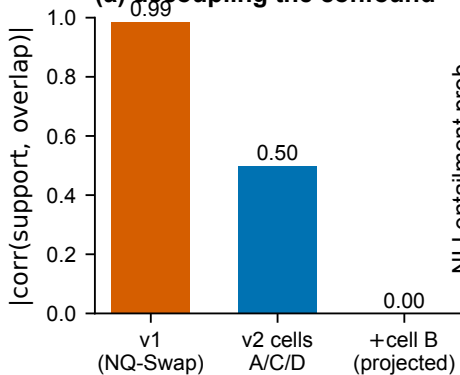
(a) decoupling the confound
