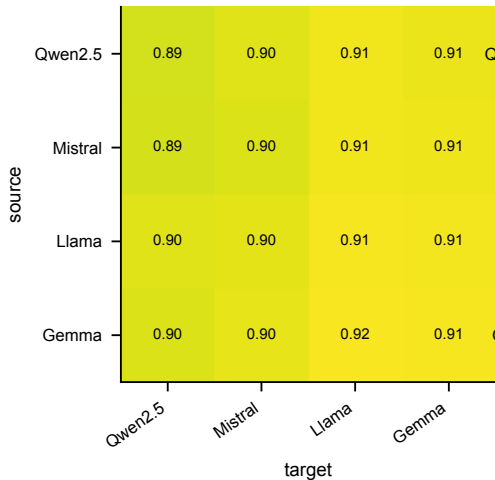
(a) orthogonal Procrustes
