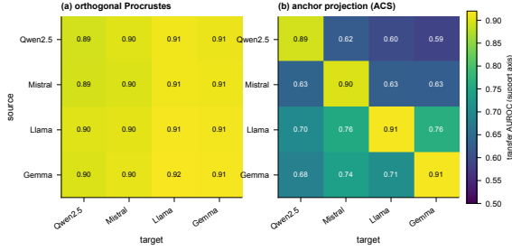
Figure 3: Matched-stimulus contrasts align across families up to a linear map. Source→target transfer AUROC of the support direction. (a) Orthogonal Procrustes is uniformly high on- and off-diagonal; we read this as alignment (cosine 0.98, Table 2), not as lossless transfer, since the AUROC is ceiling-saturated. (b) Anchor projection (ACS) matches it only within-family and degrades sharply across families.
