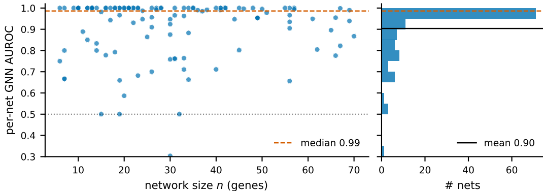
Transfer holds across sizes (118 real GRNs)
