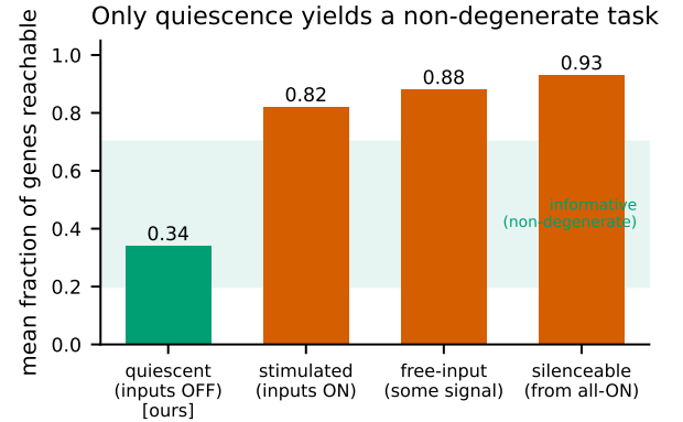
Fig. 6. Only the quiescent condition is non-degenerate. Mean per-net fraction of genes reachable on the real BBM networks under four driving conditions; the quiescent inputs-OFF task we study (green) is the only one that avoids saturation, so it is the principled rather than a cherry-picked choice.
