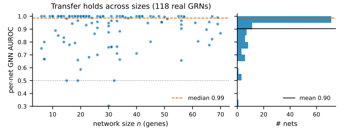
Fig. 4. Zero-shot transfer holds across network sizes (118 real GRNs). Left: per-net AUROC vs size; right: distribution with median 0.99 and mean 0.90.
