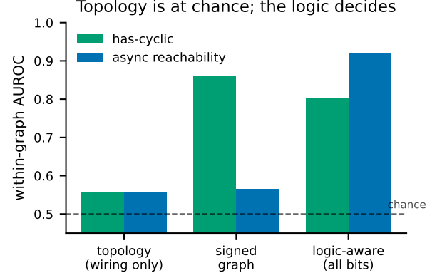
Fig. 2. The interaction graph is at chance; the logic decides. Within-graph AUROC by feature group for has-cyclic and asynchronous reachability.
