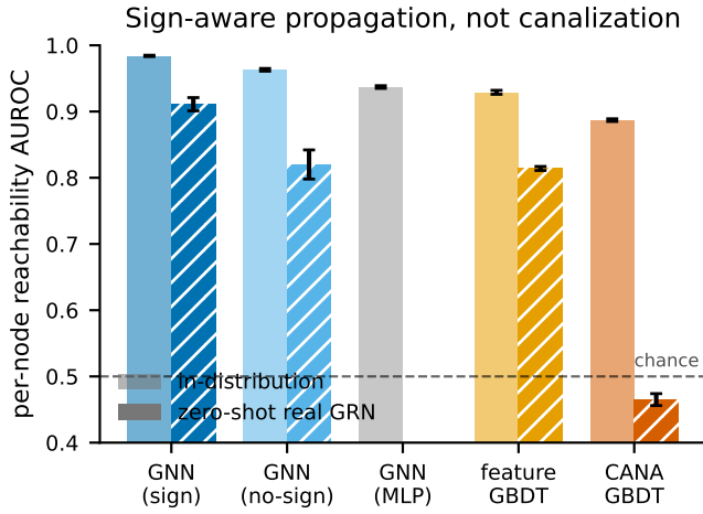
Fig. 5. Sign-aware propagation, not canalization. In-distribution and zero-shot transfer AUROC for the GNN variants and the canalization baselines; the CANA tree anti-transfers below chance.
