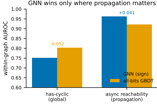
Fig. 3. The GNN wins only where propagation matters: it beats the all-bits tree on asynchronous reachability but not on the global has-cyclic property.
