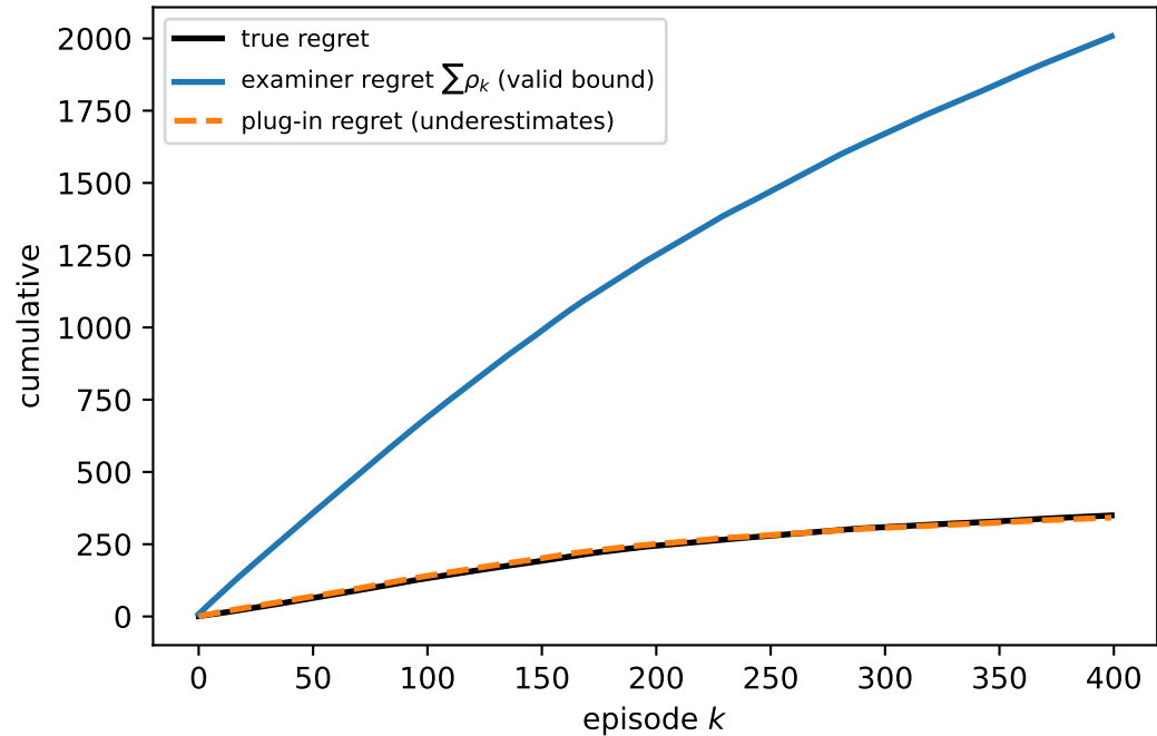
(B) Big-world MDP ( SA \gg budget): unvisited ( s, a )
