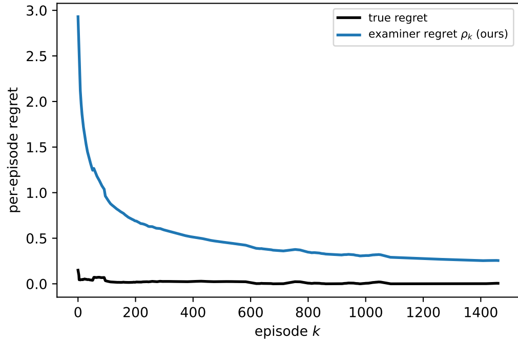
(A) Coverable MDP (small S ): both vanish
