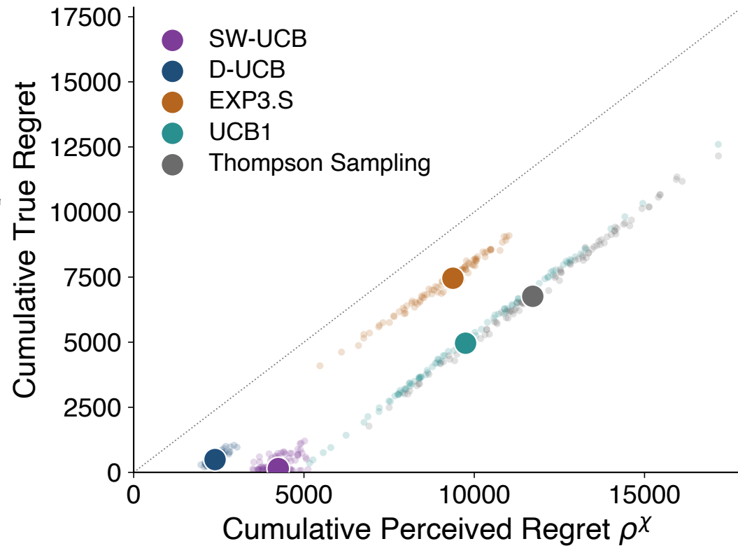
(b) Cumulative-Regret Scatter; Spearman \rho_S = 0.871 Over 5 \times 100 = 500 Pairs
