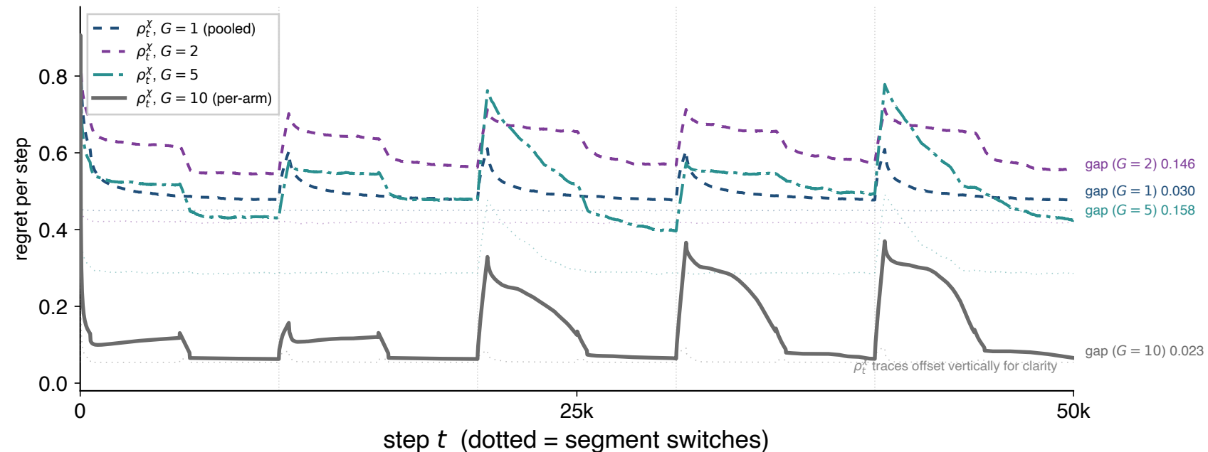
Reverse: agent restricted to G action groups (learner capacity)
