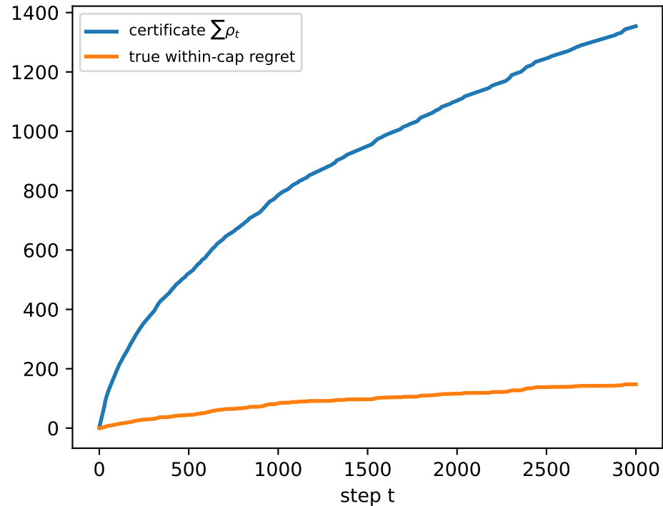
B. Lemma 1: sound \rho_t bounds real regret (coverable)
