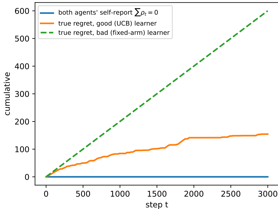
A. Prop 1: self-report certifies nothing
