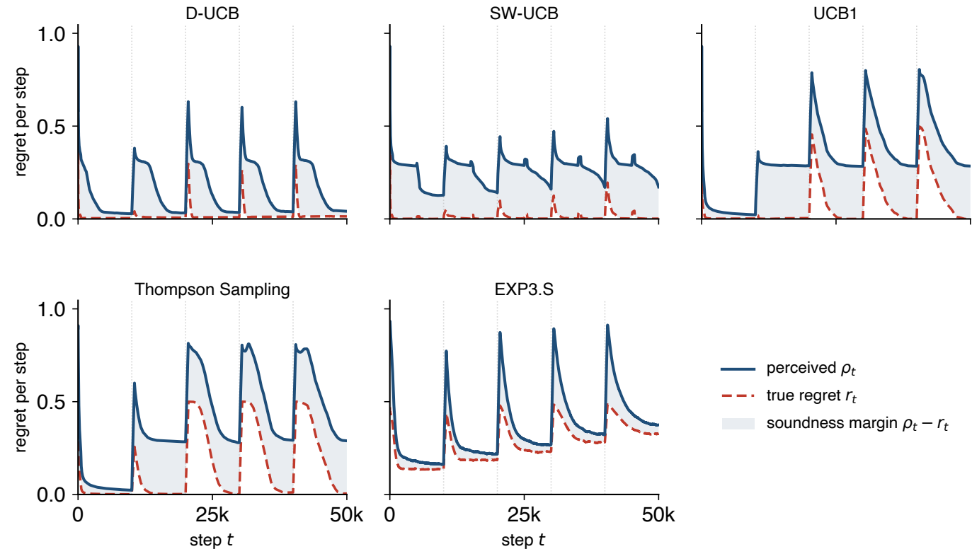
a Perceived regret \rho_t tracks and upper-bounds true regret r_t (dotted = segment switches)
