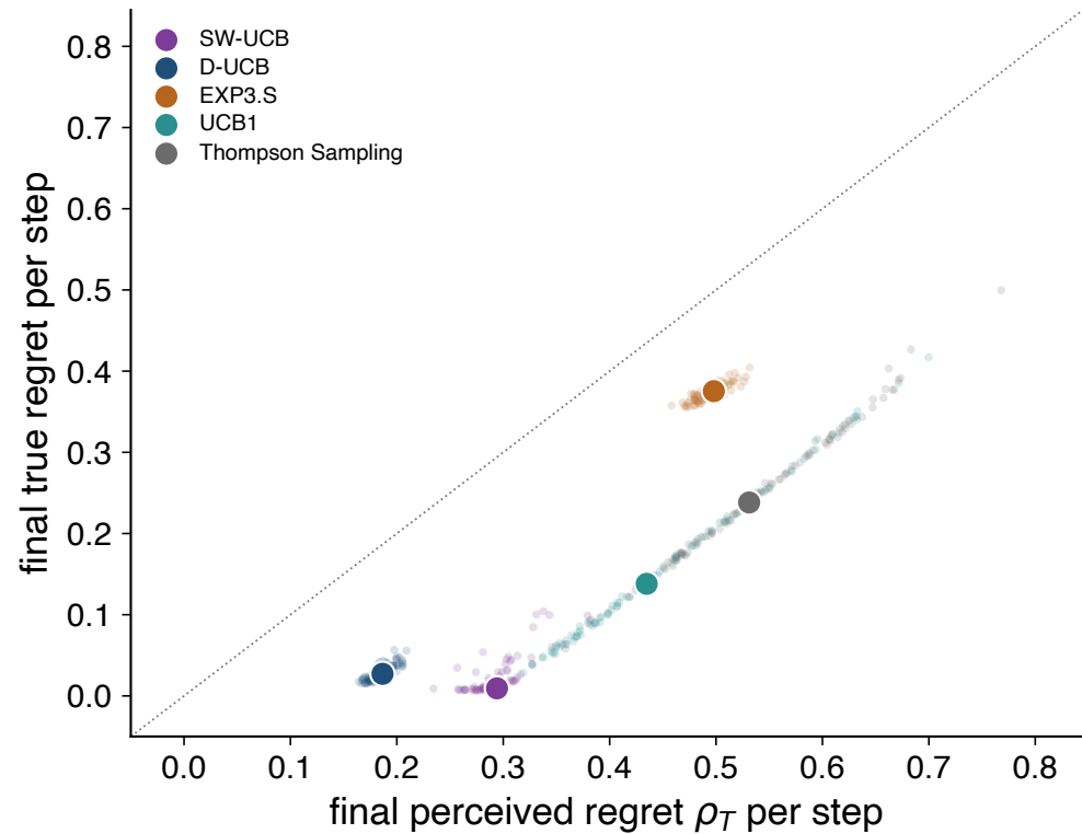
b Final-value scatter; Spearman \rho_S = 0.853 over 5 \times 100 = 500 pairs
