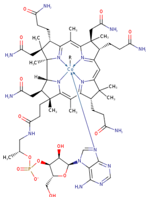
Figure 28: Representation of pseudocoenzyme B12 in ChEBI with metal complexation bonds.
