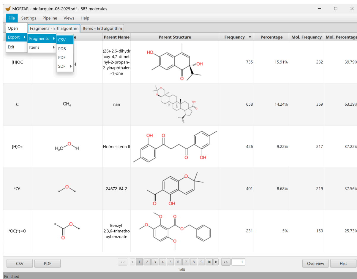
Figure 10: Fragments export menu.
