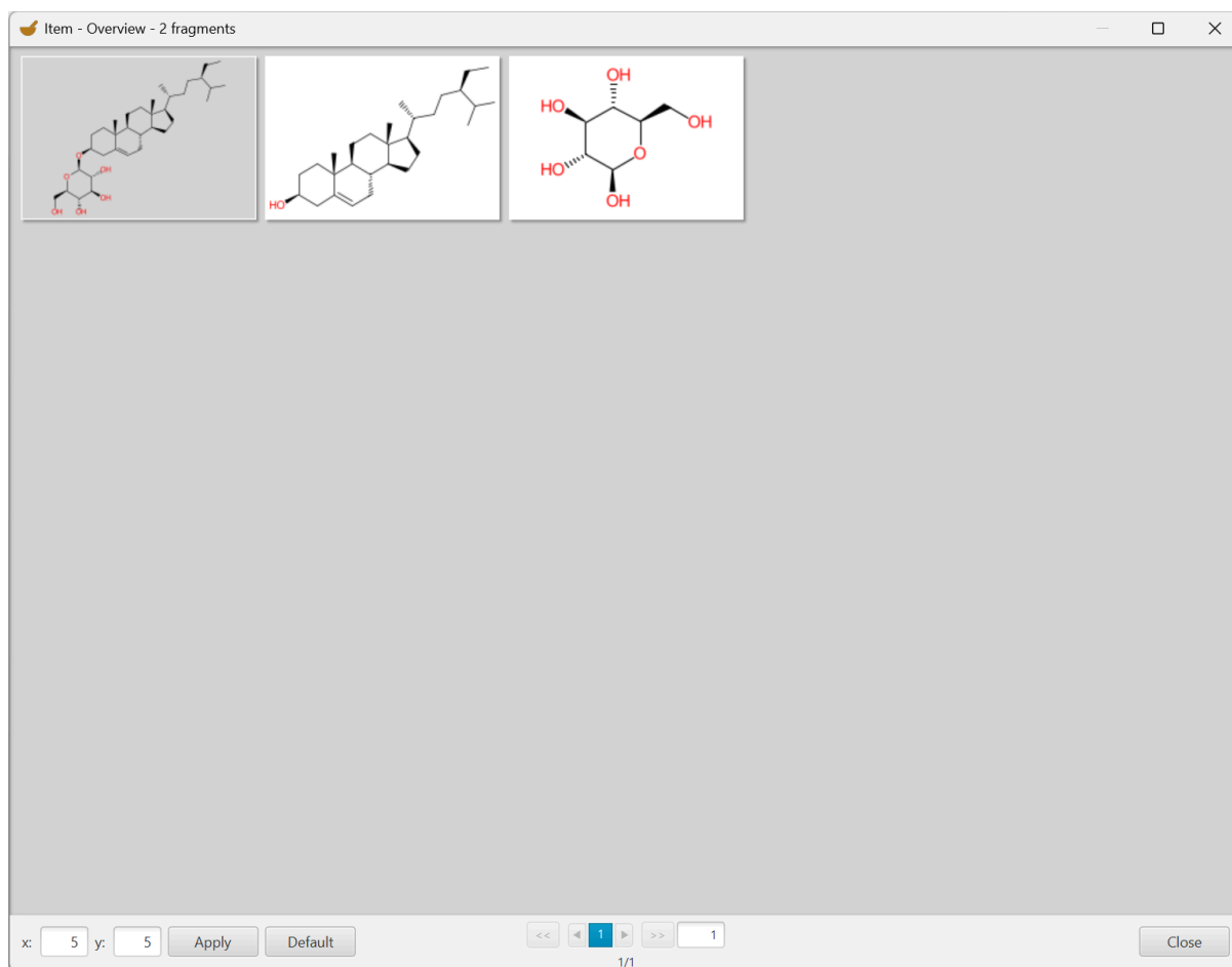
Figure 24: Sugar Removal/Detection Utility fragmentation result of Daucosterol ( CNP0324146.1 , part of the BIOFACQUIM dataset); aglycone and sugar moiety retain their stereo configurations.
