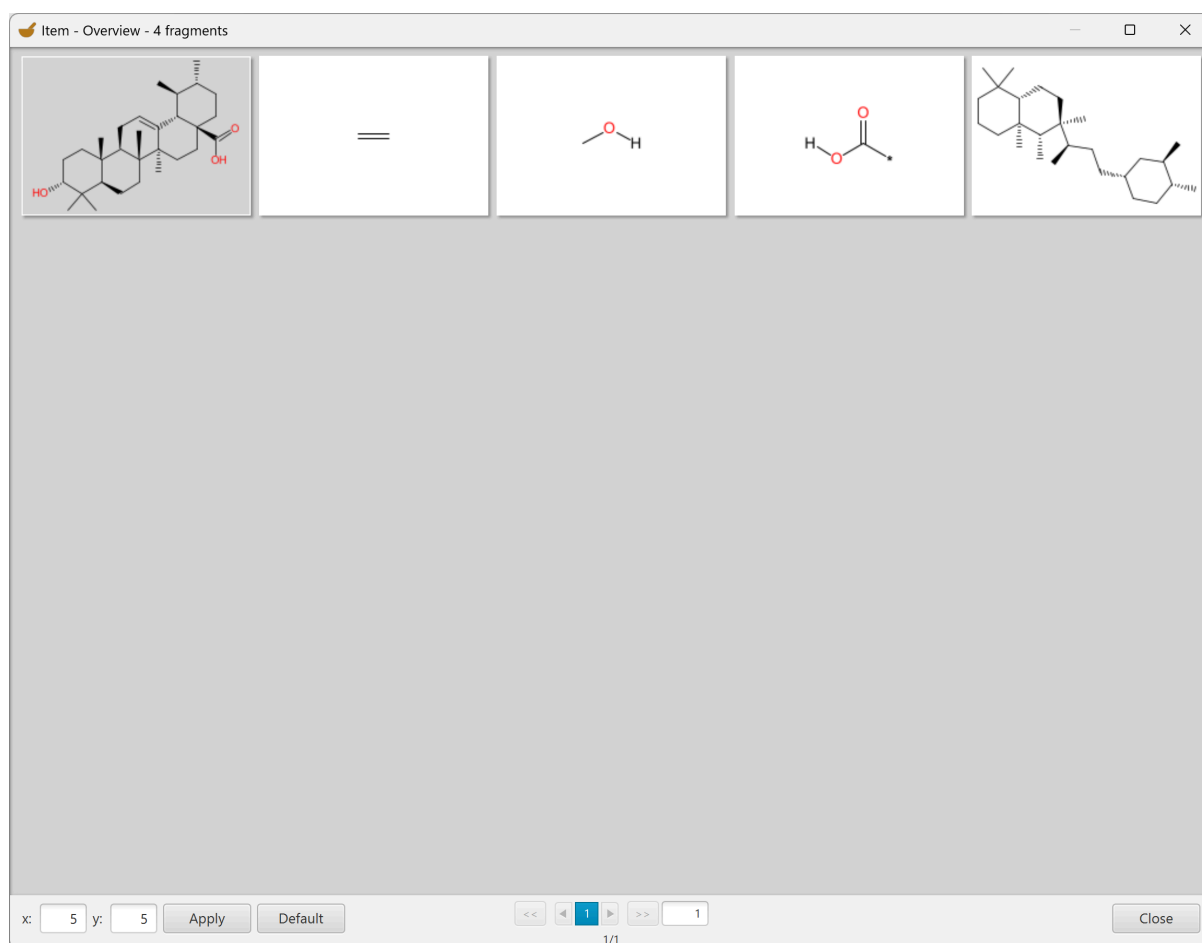
Figure 23: Functional group and alkane fragments of 3-epiursolic acid ( CNP0219063.1 , part of the BIOFACQUIM dataset); the functional groups have lost their stereo configuration, while the alkyl remnant has retained it.
