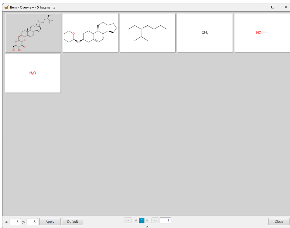
Figure 25: Scaffold Generator fragmentation result of Daucosterol ( CNP0324146.1 , part of the BIOFACQUIM dataset); the scaffold and side chain fragments retain their stereo configuration if possible.
