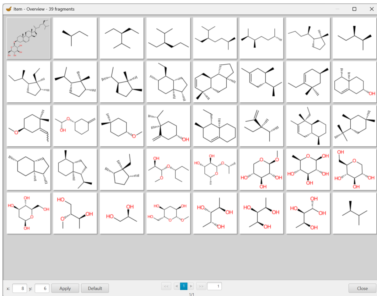
Figure 27: Circular fragmentation result of Daucosterol ( CNP0324146.1 , part of the BIOFACQUIM dataset); the extracted fragments retain their original stereo configuration if the respective setting is turned on.
