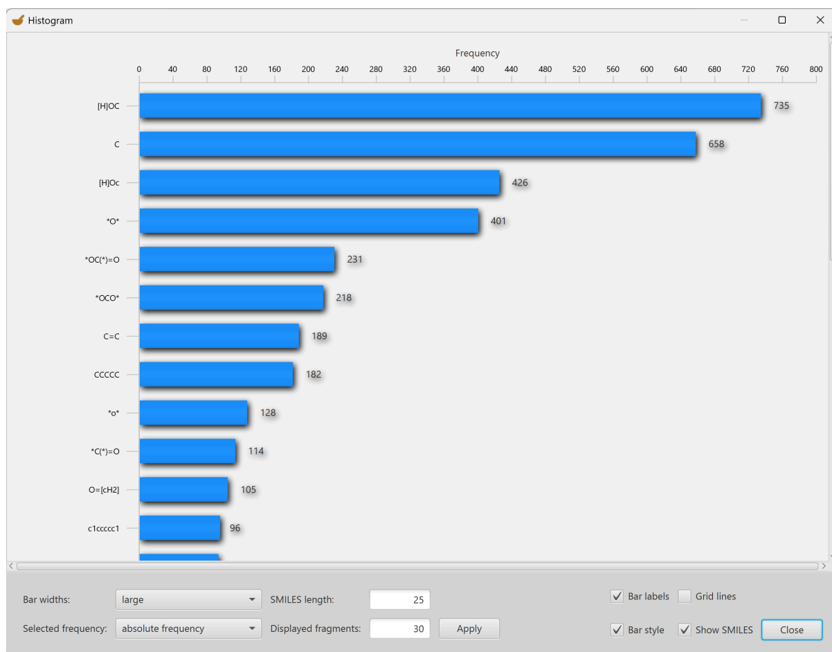
Figure 19: Histogram view.
