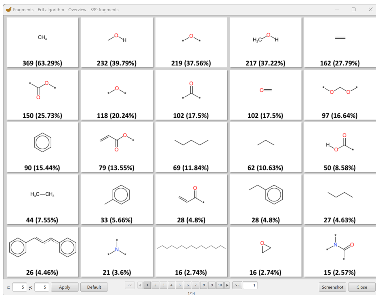
Figure 17: Fragments overview with molecule frequency labels.
