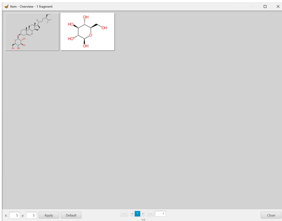
Figure 26: MolWURCS fragmentation result of Daucosterol ( CNP0324146.1 , part of the BIOFACQUIM dataset); the extracted carbohydrate structure retains its original stereo configuration.
