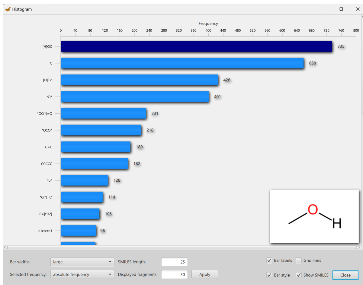
Figure 20: Structure display in histogram view.
