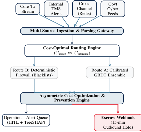
Fig. 1. SentinelFlow v2 multi-source architecture showing cost-optimal dynamic routing, decision engines, and active prevention triggers.
