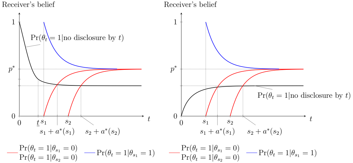
Figure 1: Equilibrium belief evolution for priors p_0 = 1 (left panel) and p_0 = 0 (right panel), and parameters \lambda_0 = 1, \lambda_1 = 1, \mu = 0.5 , and r = 0.1 .
