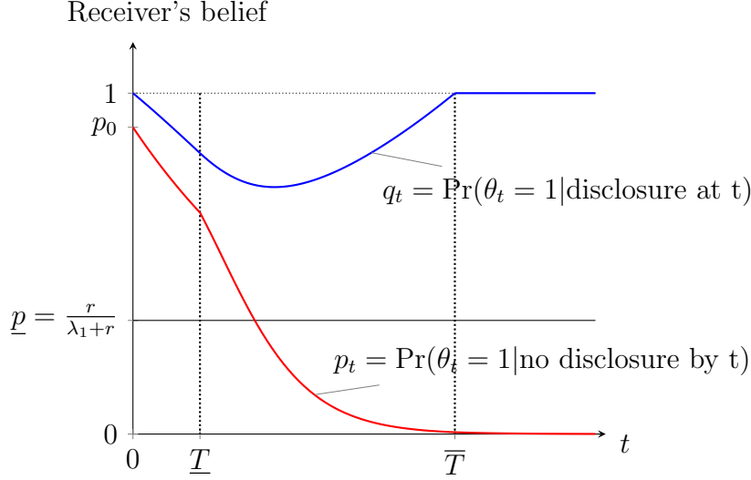
Figure 3: Belief paths in the three-phase for p_0 > \bar{p} , with vertical dashed lines at \underline{T} and \bar{T} for parameters p_0 = 0.9 , \lambda_0 = 0 , \lambda_1 = 1 , \mu = 0.5 , and r = 0.5 .
