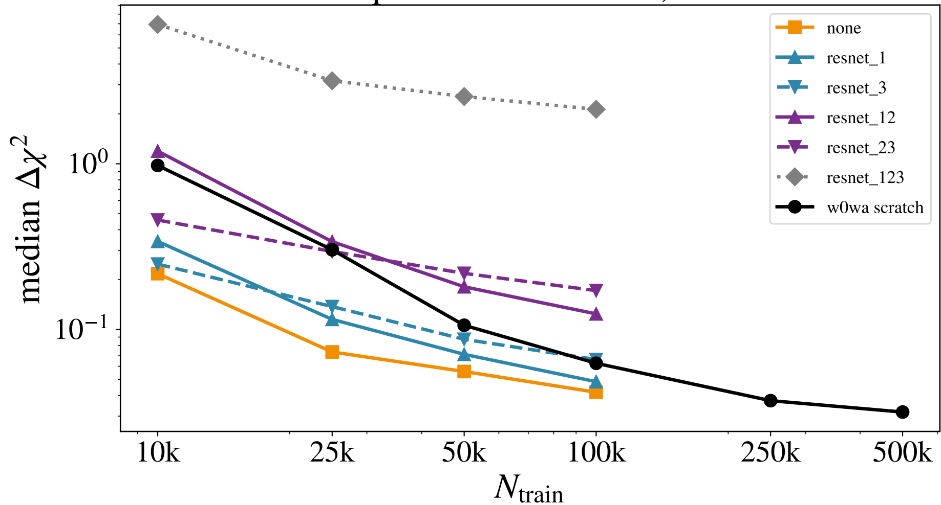
Freeze-depth ladder — Taka, T500 run1
