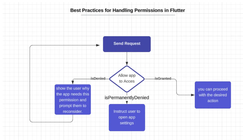
Figure 3.10: Best Practices for Handling Permissions in Flutter
