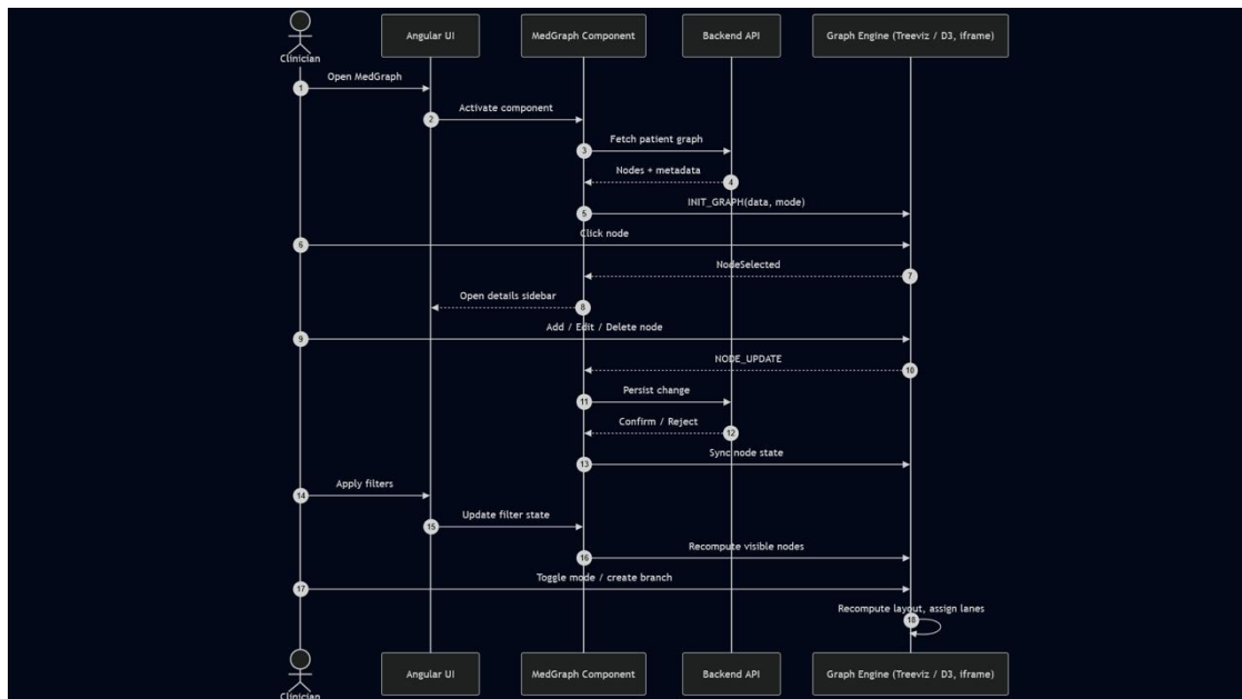
Figure 3.14: Sequence diagram illustrating MedGraph node operations, mode switching, and branching.
