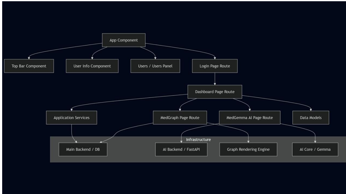
Figure 3.15: Component diagram illustrating the architecture of the dashboard, MedGraph, MedGemma AI modules, application services, and backend integration.
