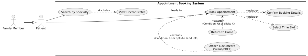
Figure 3.18: Booking Appointments Usecase
