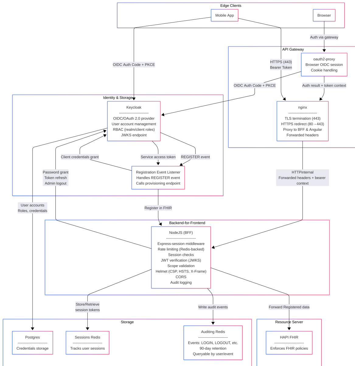
Figure 4.1: Security Architecture Components: Edge clients (Browser, Mobile), API Gateway (Nginx, OAuth2 proxy), Backend-for-Frontend (Node.js), Identity (Keycloak), Storage(Redis, Postgres) and Resource Server (HAPI FHIR) with their security-focused interactions.
