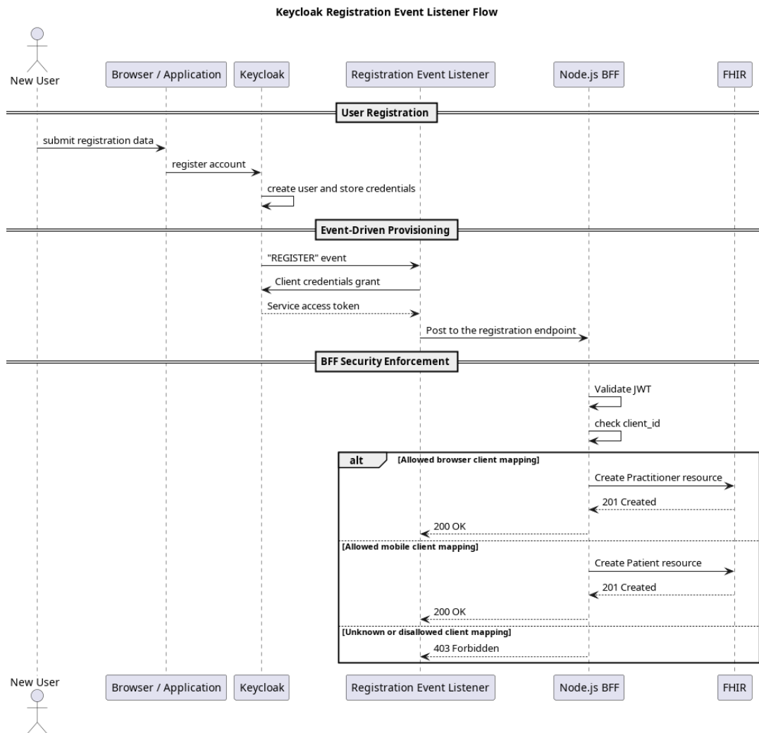
Figure 4.4: Registration Provisioning Sequence: Keycloak emits REGISTER event, the Event Listener obtains a client-credentials token, calls the BFF provisioning endpoint, and the BFF enforces JWT and caller allowlist checks before creating the mapped FHIR resource
