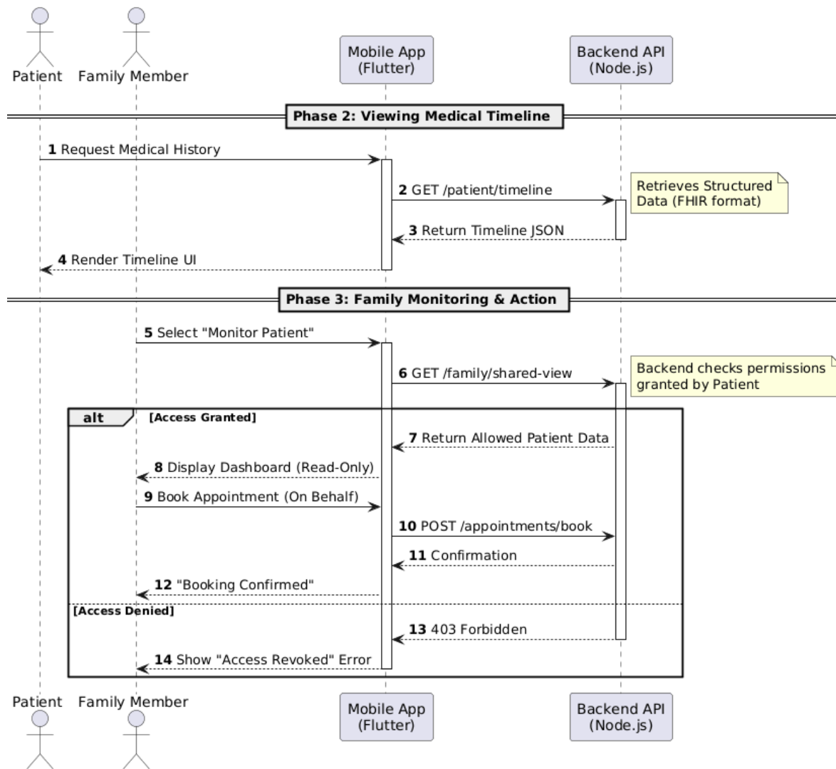
Figure 3.72: Sequence Diagram for Mobile Application
