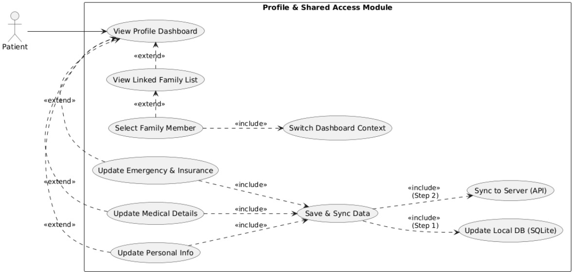
Figure 3.73: My Profile Use Case
