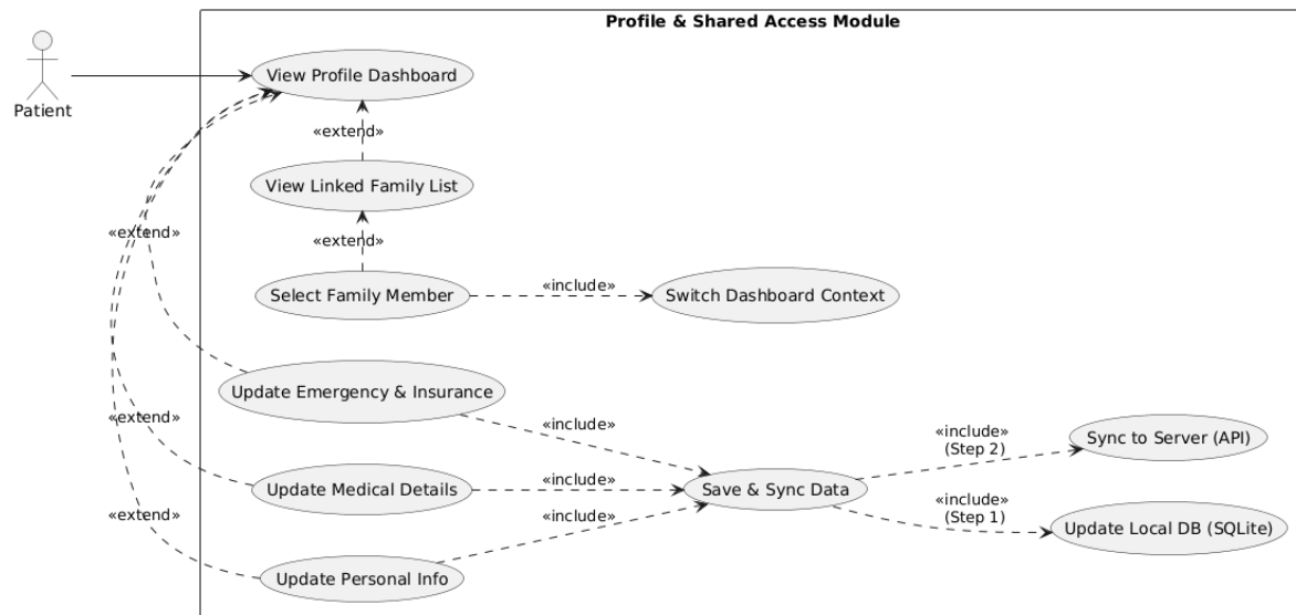
Figure 3.24: My Profile Use Case
