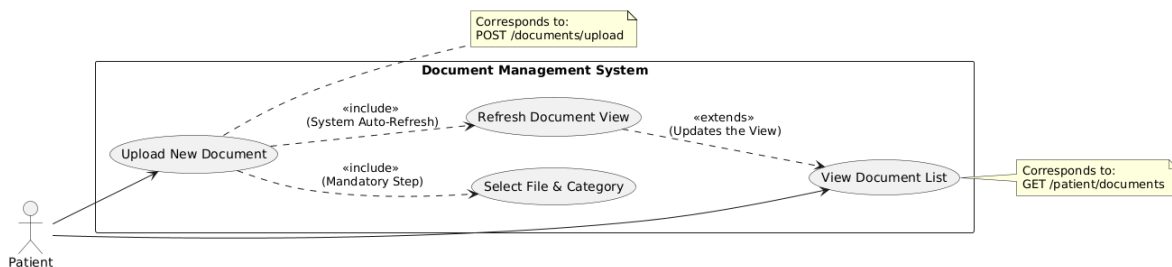
Figure 3.18: Documents Management Use Case
