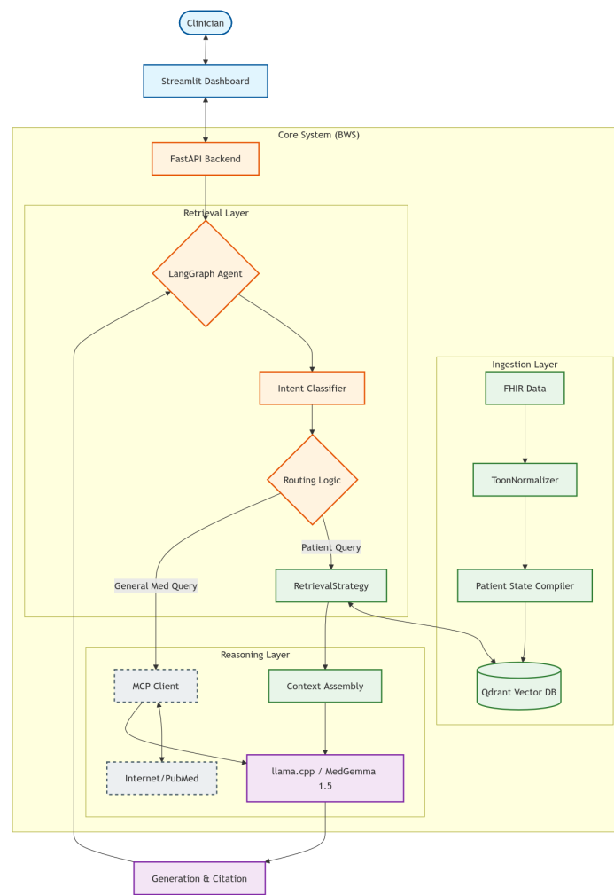
Figure 5.1: High-Level System Architecture. The flow connects the Streamlit UI to the FastAPI backend, which orchestrates the LangGraph agent. The agent routes between the Local RAG pipeline (Ingestion → Qdrant → MedGemma) and the External MCP Tools (PubMed Access) based on query classification.
