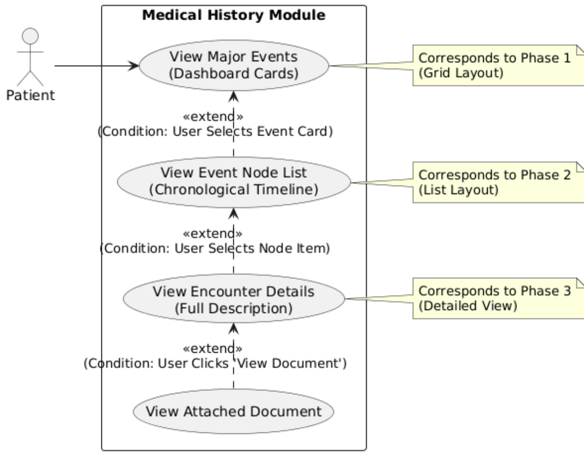
Figure 3.22: History Navigation Use Case
