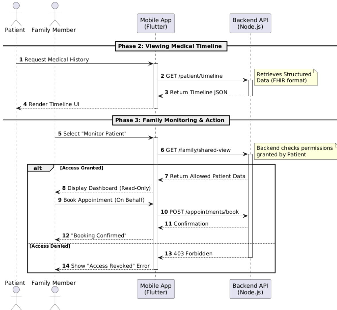
Figure 3.17: Sequence Diagram for Mobile Application
