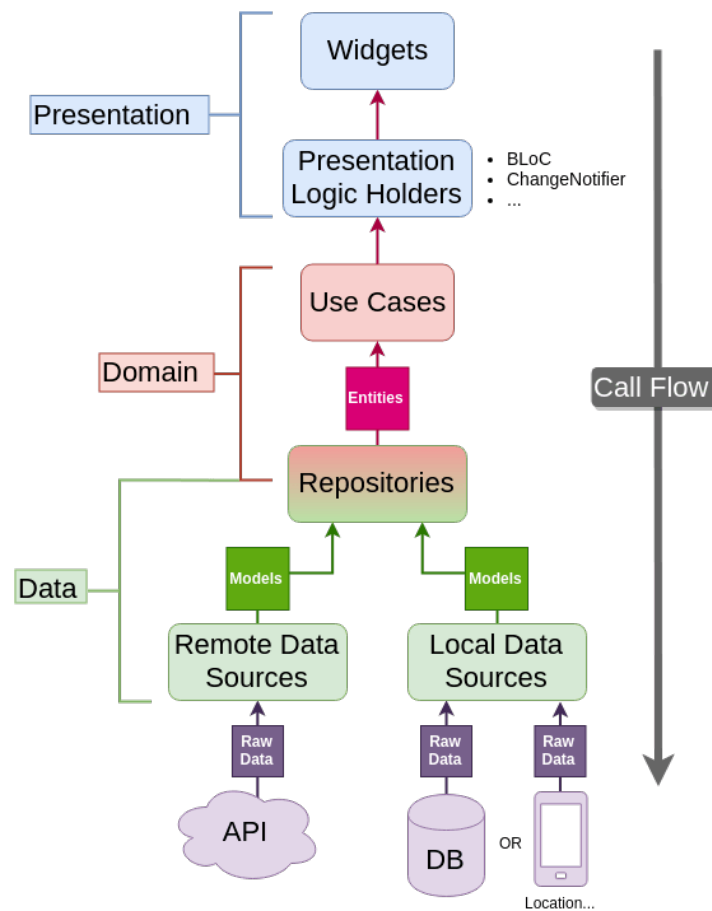
Figure 3.13: Layered Clean Architecture adopted in the mobile application
