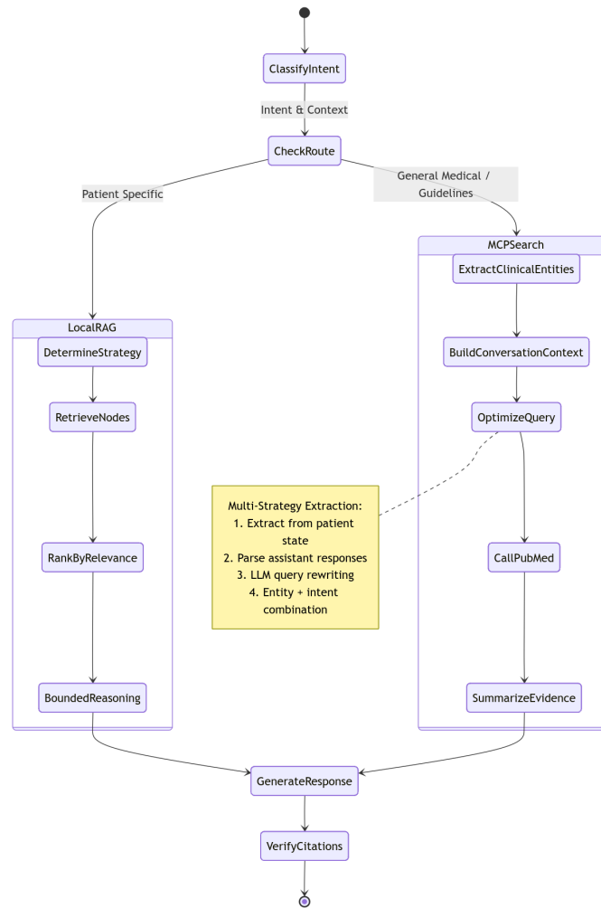
Figure 6.4: LangGraph Reasoning State Machine. The decision logic for the agent, illustrating the bifurcation between LocalRAG (Patient Specific) and MCPSearch (General Knowledge) paths, converging at the grounded generation node.
