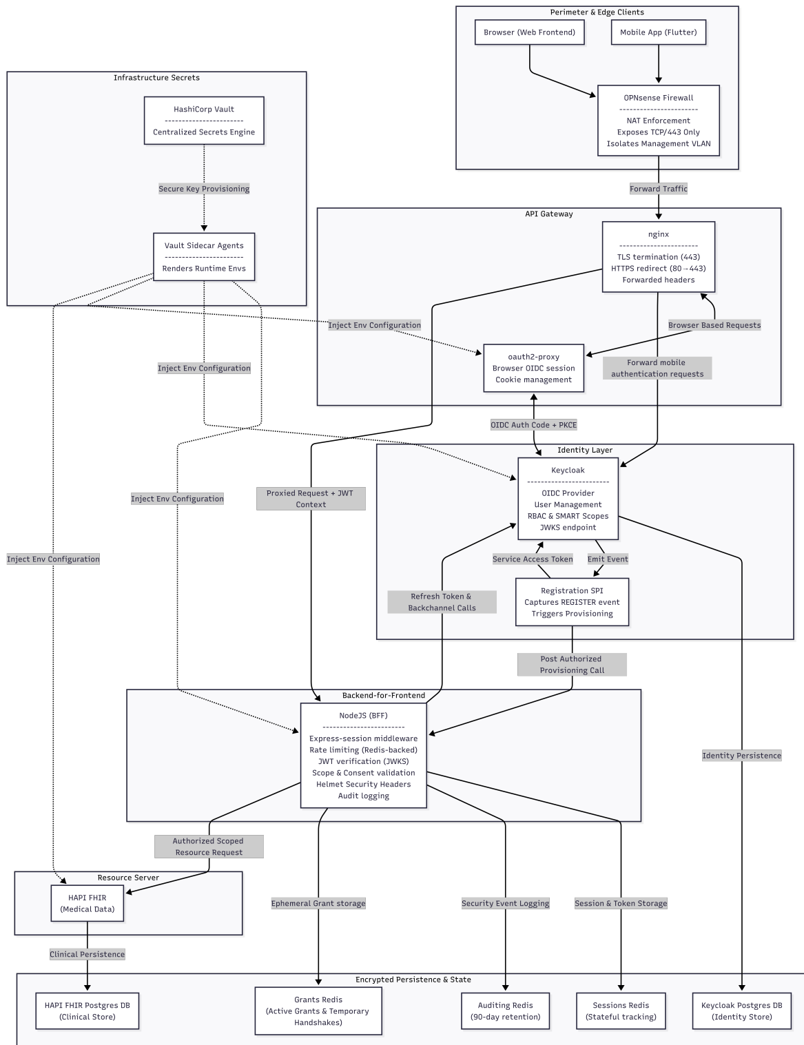
Figure 5.1: Security Architecture Components: Edge clients (Browser, Mobile), API Gateway (Nginx, OAuth2 proxy), Backend-for-Frontend (Node.js), Identity (Keycloak), Storage (Redis, Postgres), and Resource Server (HAPI FHIR).
