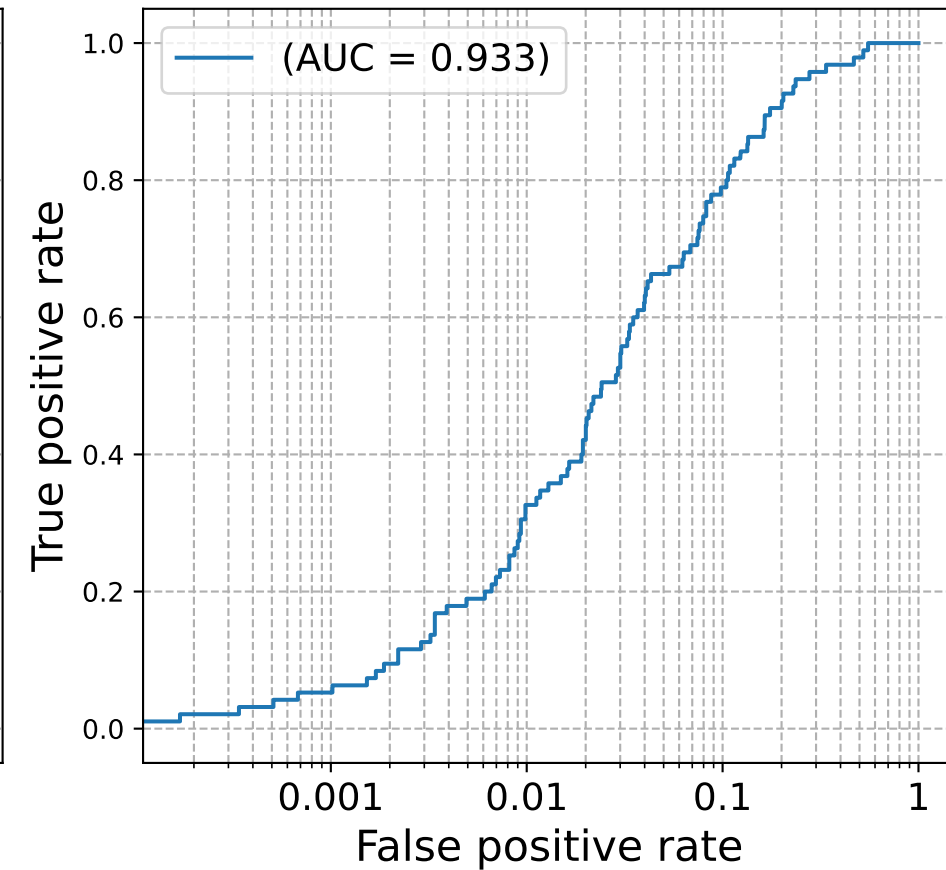
AUC for TDE classifications
