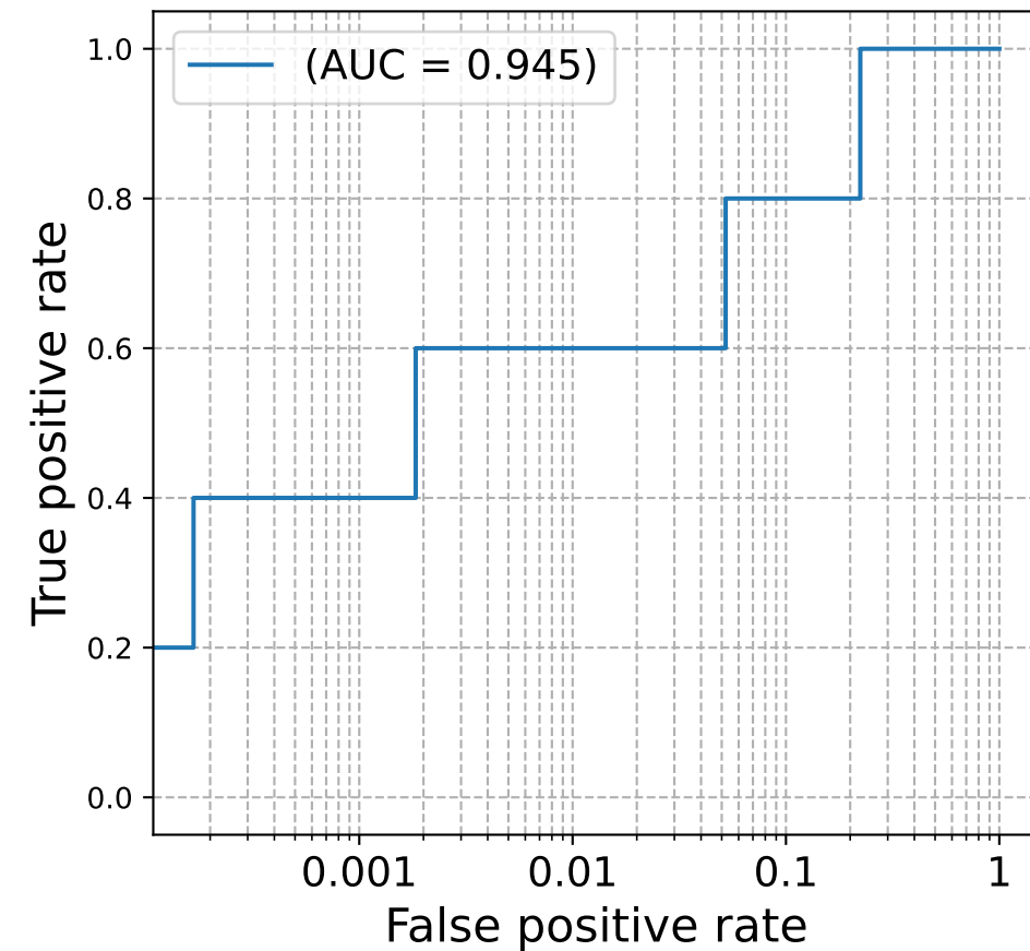
AUC for SLSN classifications
