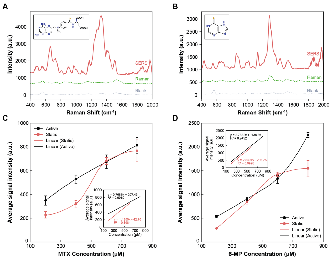
FIGURE 4 | Raman and SERS spectra of (A) MTX and (B) 6-MP on the bare substrates and Zn/Au MMs at 600 μM concentrations. (C) Average signal intensity of 670 cm -1 versus concentration curve for MTX using active and static Zn/Au MMs at concentrations of 200, 400, 600, and 800 μM. The black line represents active Zn/Au MMs, and the red line represents static Zn/Au MMs. A linear function was used to fit the SERS data. (D) Average signal intensity of 440 cm -1 versus concentration curve for 6-MP using active and static Zn/Au MMs at concentrations of 200, 400, 600, and 800 μM. The black line represents active Zn/Au MMs, and the red line represents static Zn/Au MMs. A linear function was used to fit the SERS data (inserts in the C and D). Data are presented as mean ± standard deviation (SD) obtained from three independent Raman mappings per condition.
