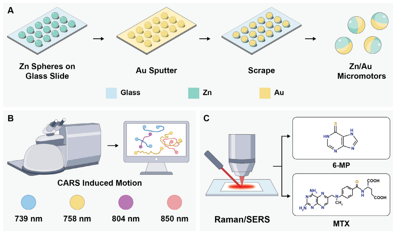
FIGURE 1 | Schematics of (A) fabrication procedure of Janus Zn/Au MMs; (B) motion study, and (C) SERS-based multiplex drug detection.
