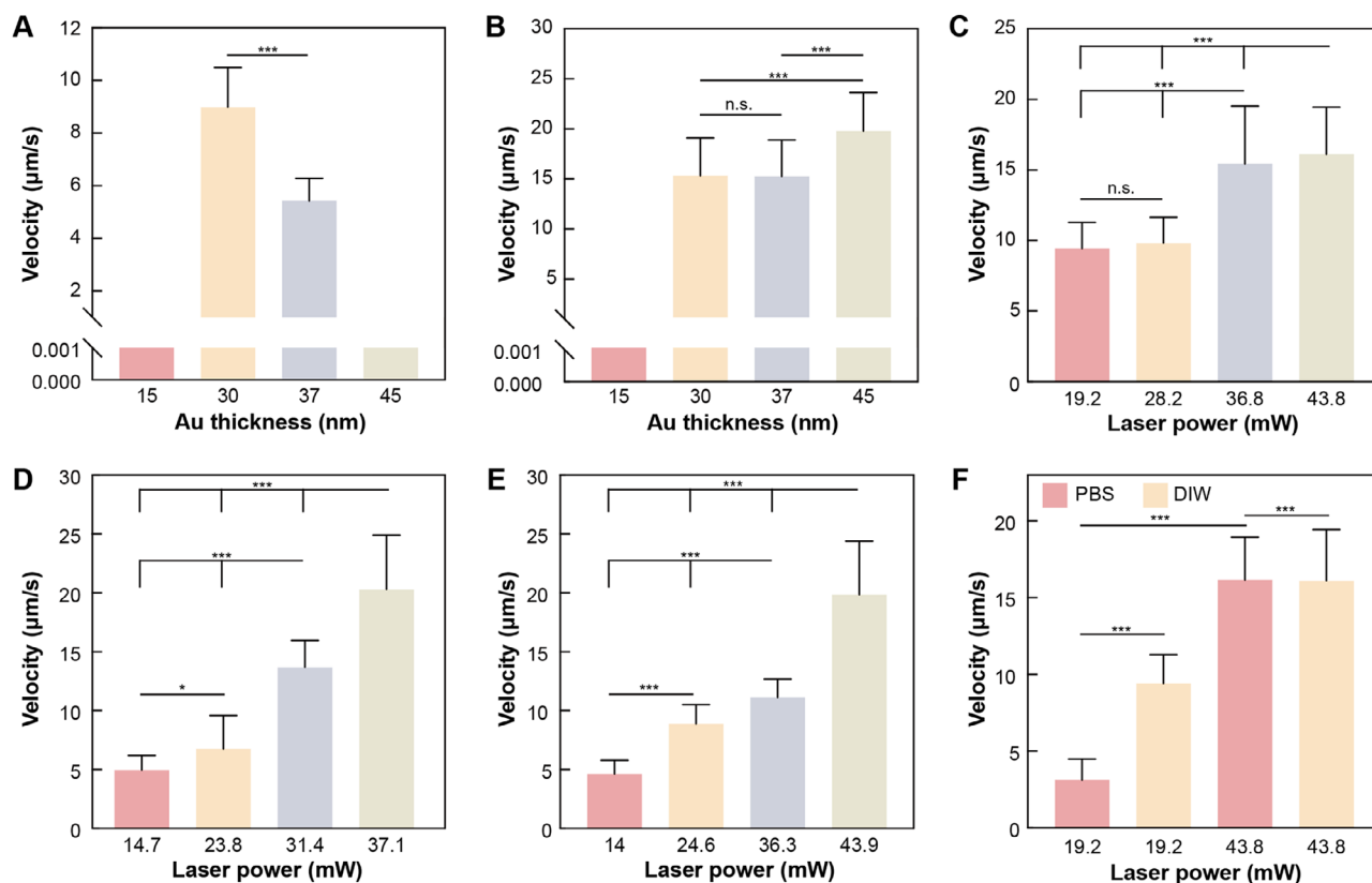
FIGURE 3 | (A) Average velocities of Zn/Au MMs with Au coatings of 15, 30, 37, and 45 nm under dual-beam NIR excitation (total power = 19.2 mW). (B) Effect of increased laser power (43.8 mW) on the average velocity of Zn/Au MMs with different Au coating thicknesses. (C) Dependence of average velocity on total laser power for Zn/Au MMs (30 nm Au coating) under balanced dual-beam excitation. (D) Average velocity of Zn/Au MMs (30 nm Au coating) as a function of Stokes laser power with constant Pump power (20%). (E) Average velocity of Zn/Au MMs (30 nm Au coating) as a function of Pump laser power with constant Stokes power (20%). (F) Comparison of average velocities of Zn/Au MMs (30 nm Au coating) in DI water and PBS at 19.2 and 43.8 mW total power. All experiments were performed under dual-beam NIR excitation with the Pump laser fixed at 800 nm and the Stokes laser at 1031 nm. For all experiments, the Pump laser wavelength was fixed at 800 nm and the Stokes laser at 1031 nm. Velocities were calculated from trajectory analysis of individual MMs ( n = 20 MMs per condition). Data are presented as mean \pm standard deviation (SD). Statistical significance was evaluated using a two-tailed t -test, with p < 0.05 considered statistically significant.
