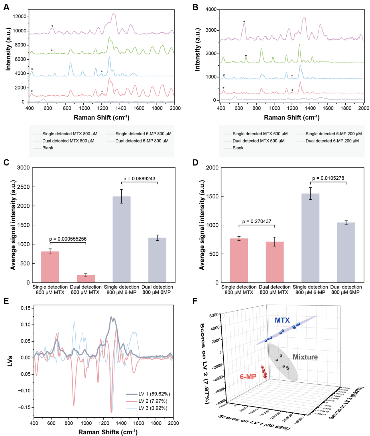
FIGURE 5 | (A) Stacked SERS spectra of dual and single detected 6-MP and MTX at 800 \mu\text{M} compared with blank using active Zn/Au MMs. The stars correspond to the characteristic peak at around 670 \pm 5 \text{ cm}^{-1} for MTX and around 440 and 1220 \text{cm}^{-1} for 6-MP, respectively. (B) Stacked SERS spectra of dual- and single-detected 200 6-MP and 600 \mu\text{M} MTX compared with the blank using active Zn/Au MMs. The stars correspond to the characteristic peak at around 670 \pm 5 \text{ cm}^{-1} for MTX and around 440 and 1220 \text{cm}^{-1} for 6-MP, respectively. Comparison of signal intensities for single and dual detection of 800 \mu\text{M} MTX and 800 \mu\text{M} 6-MP integrated with (C) Static Zn/Au MMs and (D) Active Zn/Au MMs. Corresponding error bars are depicted. p-values are shown between conditions using the two-tailed t-test with a significance level of 0.05. (E) Loading plots of PLS-DA model (LVs = 4). (F) 3D score plots of PLS-DA model for the concentration level of 600 and 800 \mu\text{M} MTX and 6-MP and mixture of 600 \mu\text{M} of each. [Correction added on June 4, 2026, after first online publication: Figure caption of Figure 5 (C) and (D) has been amended in this version.]
