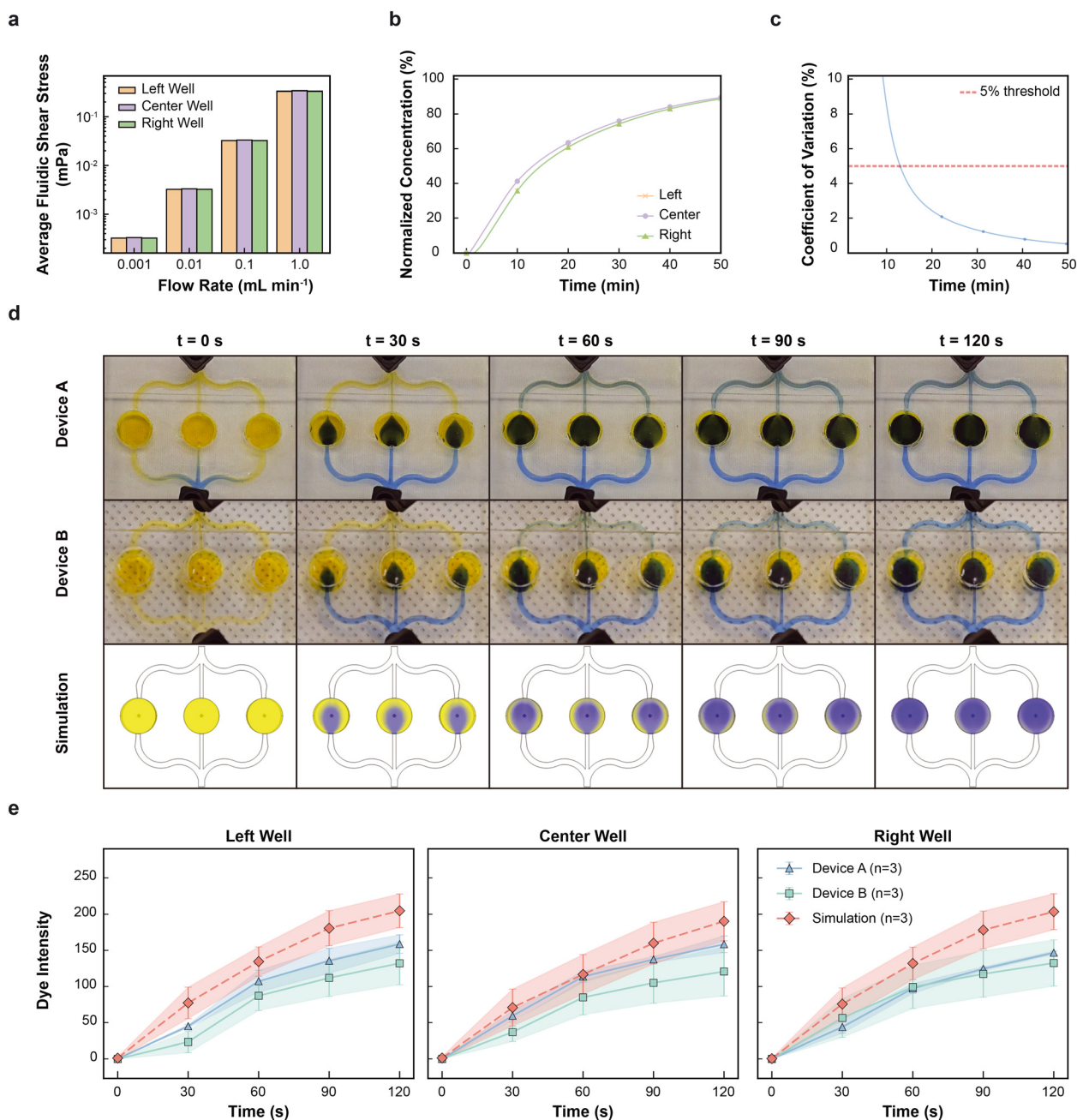
Fig. 3 Computational predictions and experimental validation of uniform flow distribution in the triMEA platform. a) Flow rate-dependent shear stress distribution across left, center, and right wells, across flow rates from 0.001 to 1.0 mL min -1 . b) Simulated normalized concentration profiles for tracer species at 0.1 mL min -1 . c) Coefficient of variation across wells over time. d) Experimental validation using blue dye perfusion at 0, 30, 60, 90, and 120 s in two independent devices (device A, device B) with a flow rate of 1.0 mL min -1 . The bottom row shows the corresponding COMSOL simulations. e) Quantification of dye intensity over time in left, center, and right wells for both devices and simulation ( n = 3 independent repeats per condition).
