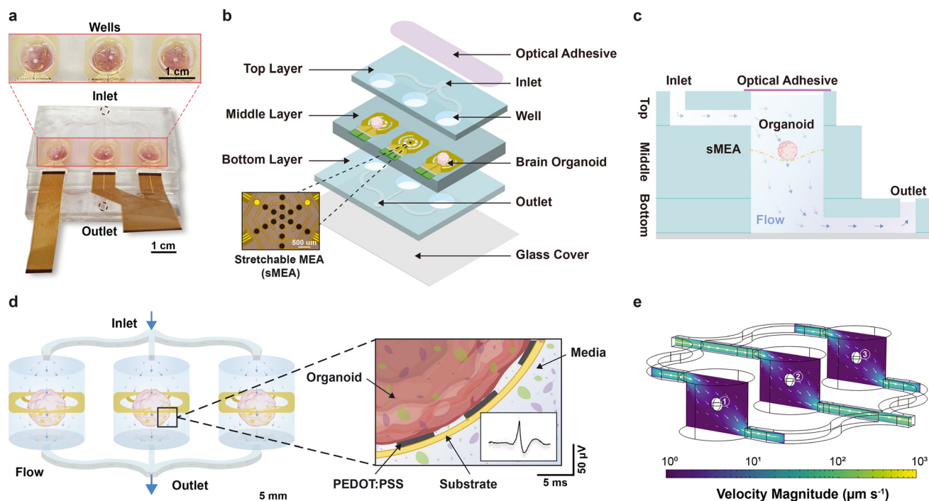
Fig. 1 Millifluidic triMEA platform for organoid monitoring. a) Optical image of the packaged triMEA platform. b) Exploded view of the triMEA platform. Inset shows the layout of the sMEA microelectrodes. c) Cross-sectional view of the platform. d) Schematic of the three-well flow architecture, with a zoomed inset depicting the sMEA–organoid interface (Au and PEDOT:PSS layers) and a representative spike recorded during perfusion. e) Representative simulation of flow velocity magnitude across the three wells.
