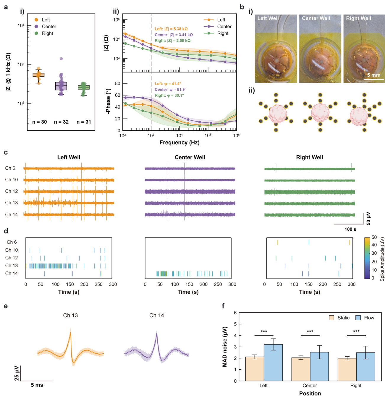
Fig. 5 Electrophysiological recording of mBOs placed in the triMEA platform. a) Electrochemical characterization of sMEA electrodes. i) Box plot of electrode impedance magnitude at 1 kHz across left ( n = 30 ), center ( n = 32 ), and right ( n = 31 ) wells. ii) Bode plots of impedance magnitude (top) and phase (bottom) as a function of frequency for all three wells. b) Placement of mBOs in the triMEA platform. i) Optical images of mBOs seated in the left, center, and right wells. ii) Schematics of organoid positioning relative to the sMEA electrodes in each well. c) Representative extracellular recordings from five channels under continuous perfusion over 300 s across all three wells. d) Raster plots of detected spike events under perfusion across all three wells, color-coded by spike amplitude. e) Representative spike waveforms from channel 13 (left well) and channel 14 (center well). f) MAD noise comparison between static and flow conditions across left, center, and right wells. A statistically significant increase in noise floor was observed under perfusion at all three positions (Mann-Whitney U test with Bonferroni correction, *** p < 0.001 , n = 16 channels per well per condition).
