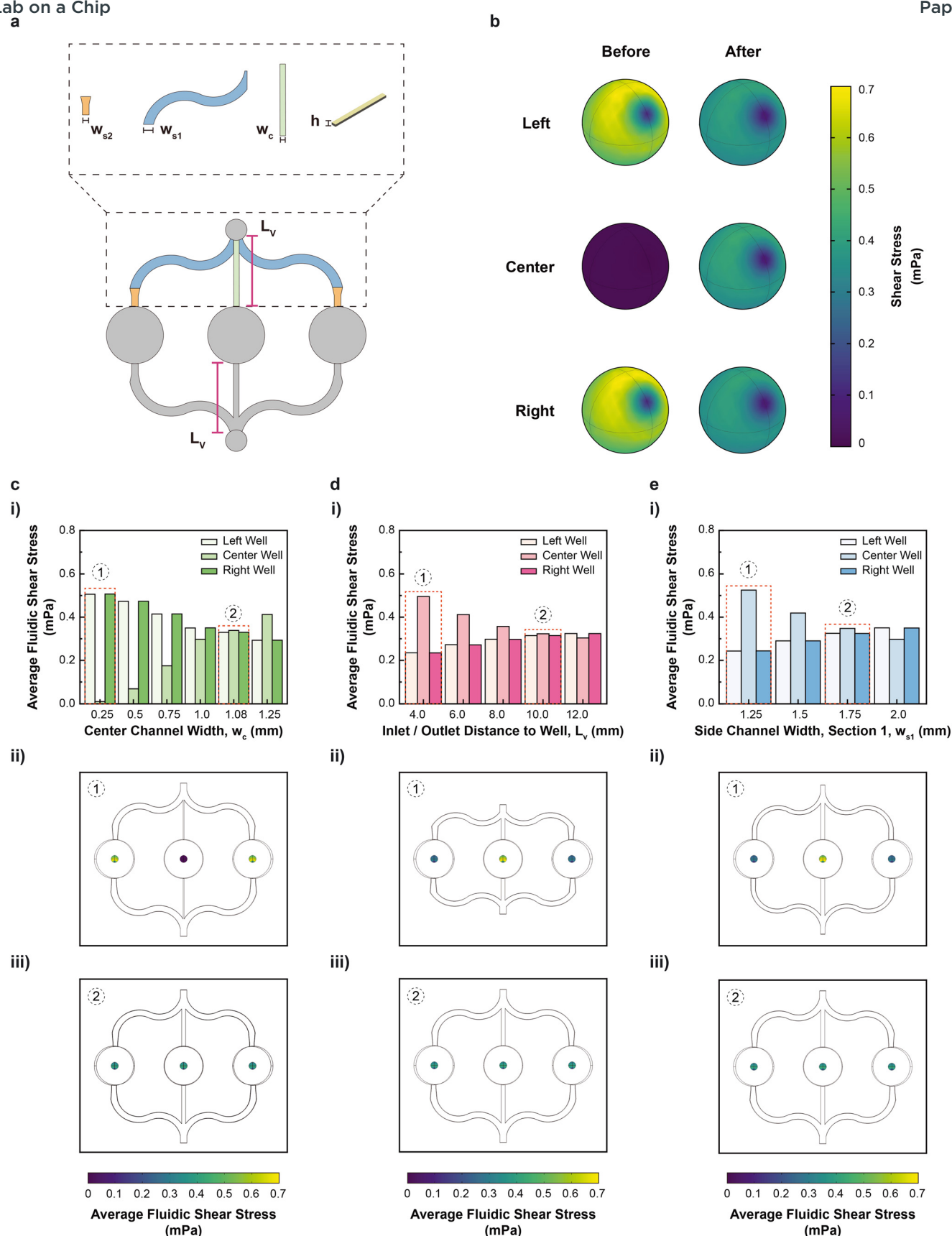
Fig. 2 Geometric optimization of the triMEA platform for uniform multi-well perfusion. a ) Schematic illustration of channel geometry with design parameters. b ) Surface shear stress distributions on left, center, and right organoids before and after geometric optimization. The “before” condition corresponds to an initial, non-optimized geometry with all channel dimensions set to the lower bound of their tested range. c–e ) Effects of c ) center channel constriction width ( w_c ), d ) inlet/outlet distance to well ( L_v ), and e ) side channel width, section 1 ( w_{s1} ) on average fluidic shear stress in each well. For each parameter, i ) average fluidic shear stress per well across the tested range, with dashed lines at the (1) initial (suboptimal) and (2) final (optimized) values, ii ) shear stress distribution at (1), and iii ) shear stress distribution at (2).
