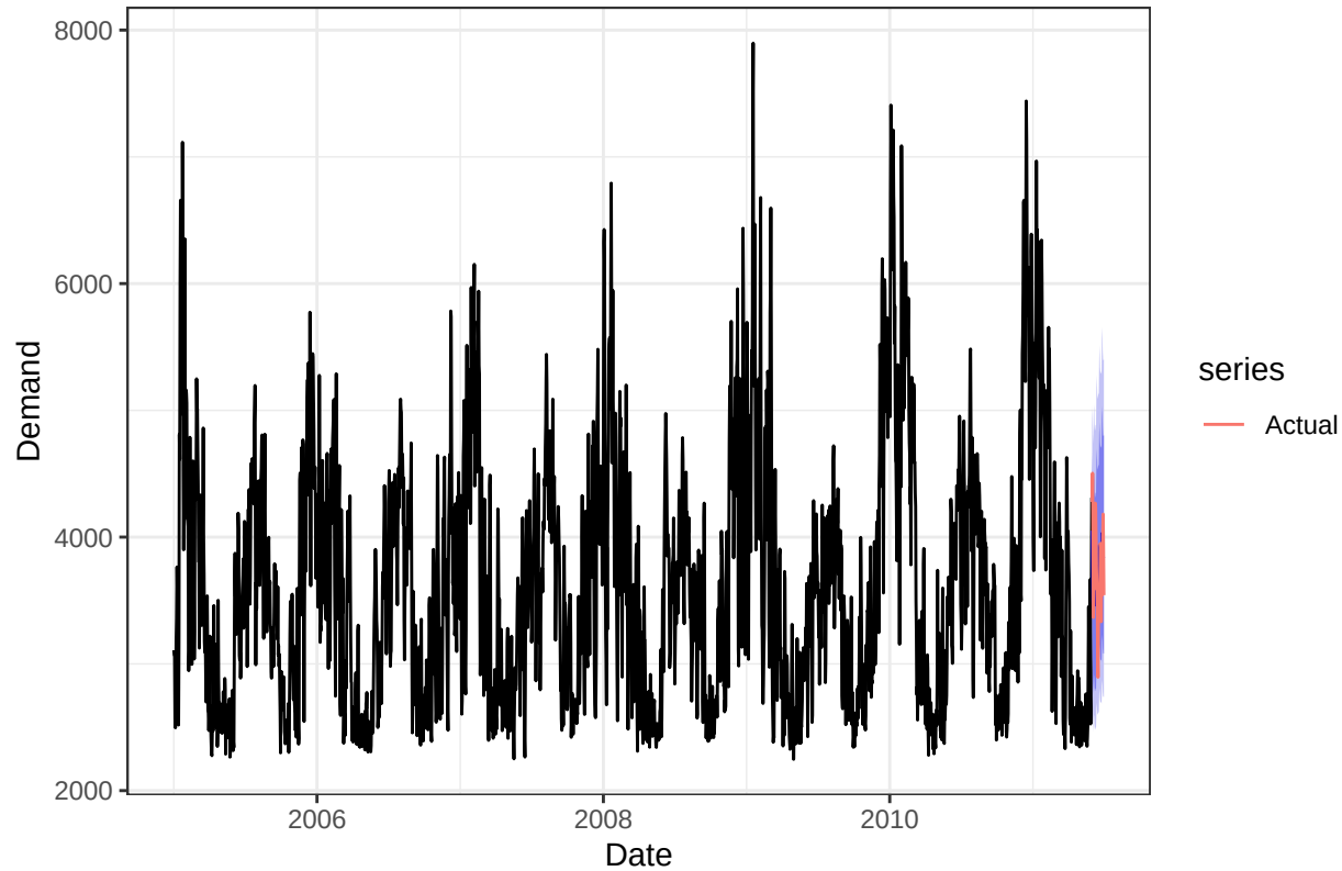
Model 1: TBATS
