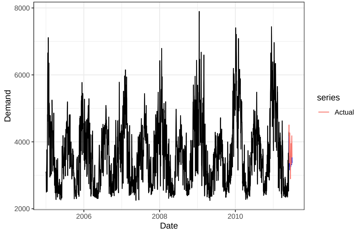
Model 3: NNETAR
