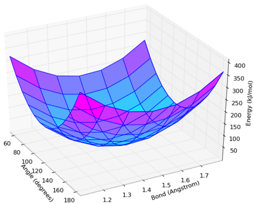
FIGURE 5.2: MM potential energy surface for methanol
