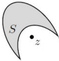
Figure 5.3: Convexity is important
