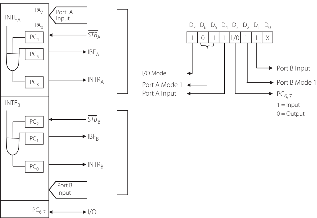
Figure 9.10 | Mode 1: Strobed input – Pin configuration and control word format
