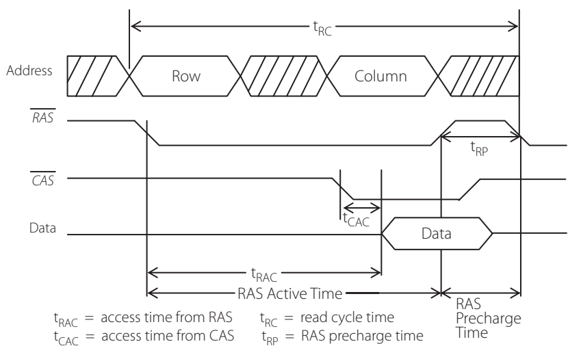
Figure 12.8 | Typical read cycle of DRAM
