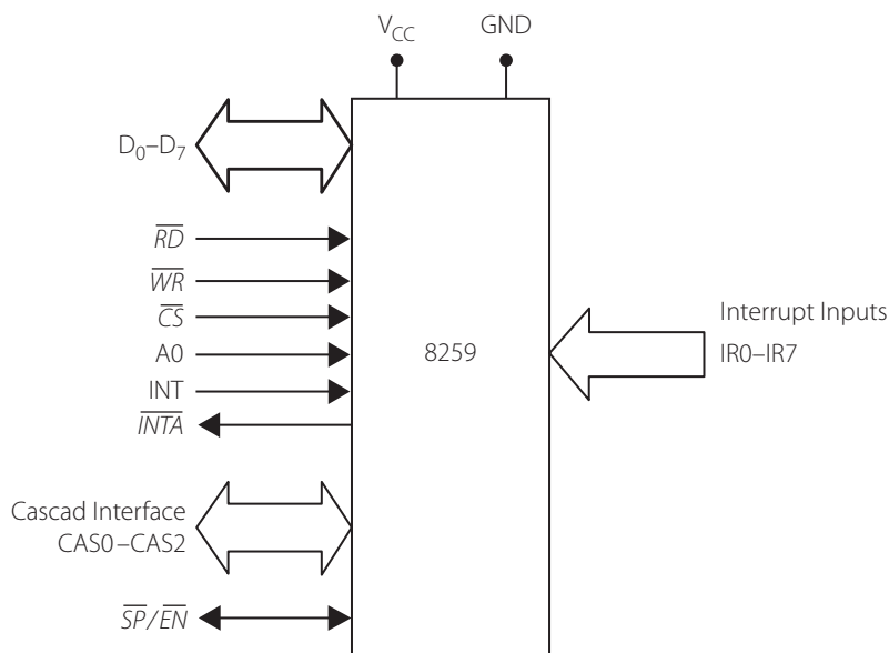
Figure 10.22 | Functional block diagram of the PIC
