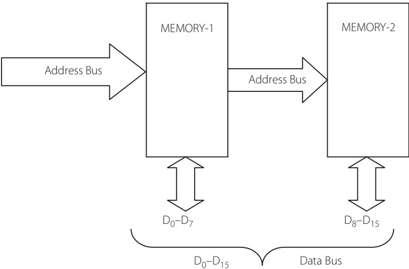
Figure 7.11 | 16-bit memory realized using two 8-bit memory chips
