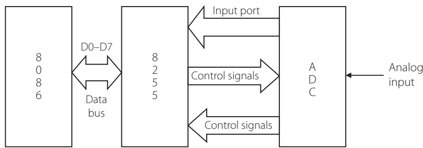
Figure 9.19 | General block diagram of the connection between an ADC, PPI and 8086
