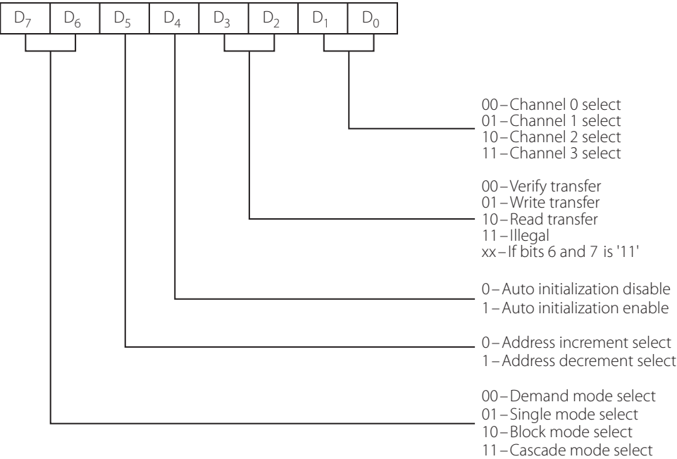
Figure 11.26 | Mode register format
