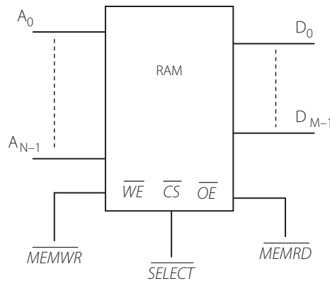
Figure 7.1 | Typical RAM with control pins
