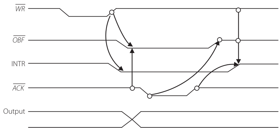
Figure 9.13 | Timing waveform for strobed output mode
