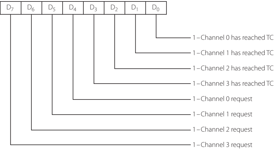
Figure 11.25 | Status register format
