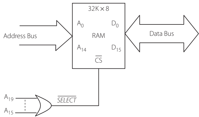
Figure 7.4 | Address decoding using OR logic
