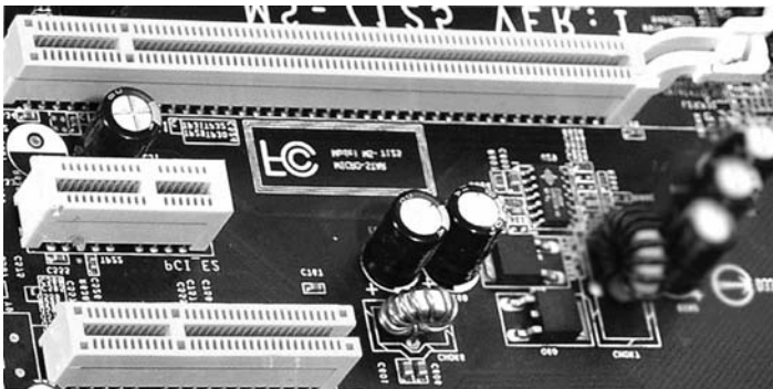
Figure 17.7 | Three PCIe sockets on a motherboard
