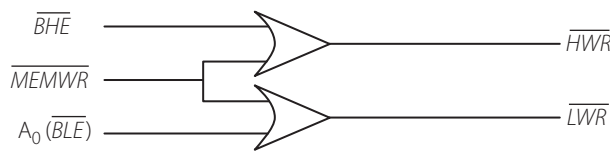
Figure 7.14 | Using separate write strobes
