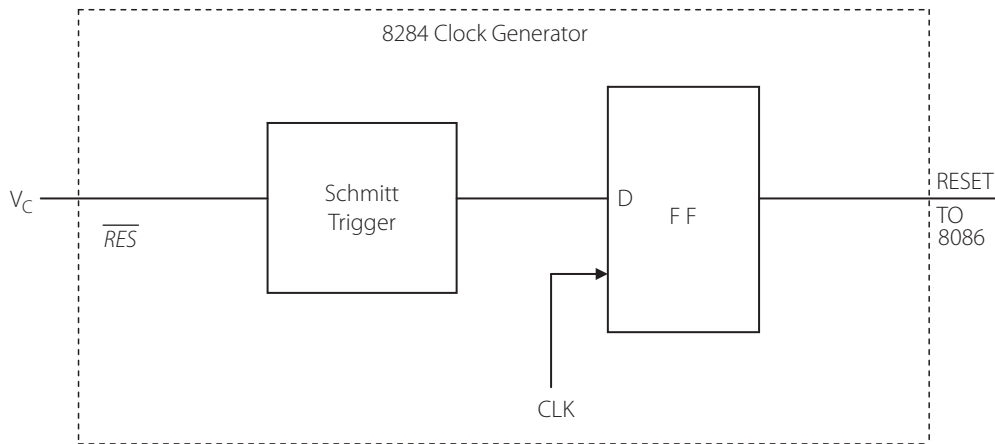
Figure 6.13 | The generation of the reset pulse using a Schmitt trigger (inside the 8284 IC)
