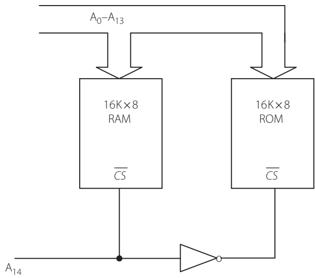
Figure 7.9 | Partial address decoding
