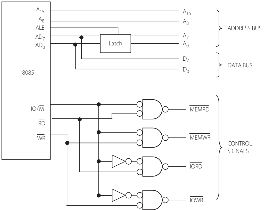
Figure 0.16 | External hardware used for getting separate address and data bus and control signals
