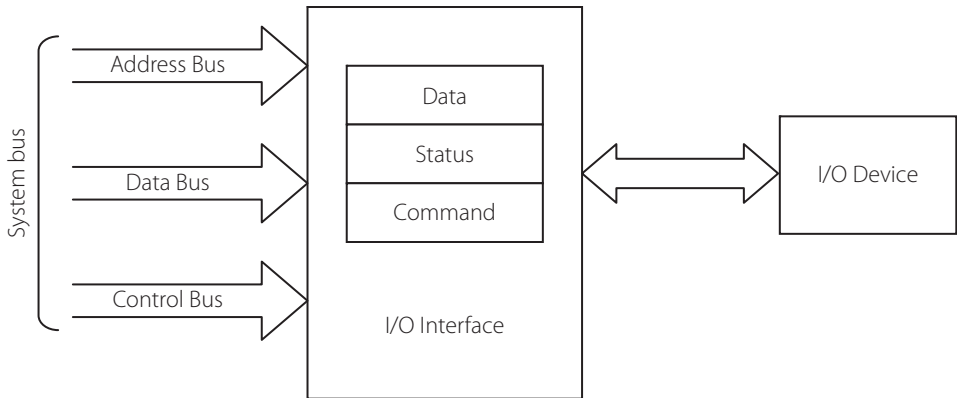
Figure 0.8 | The I/O system
