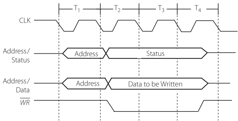
Figure 6.17 | Simplified write machine cycle timing
