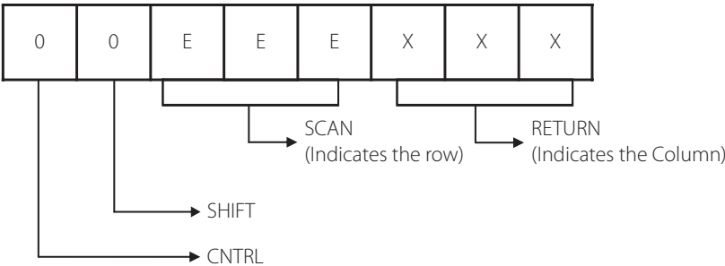
Figure 10.17 | Return key code
