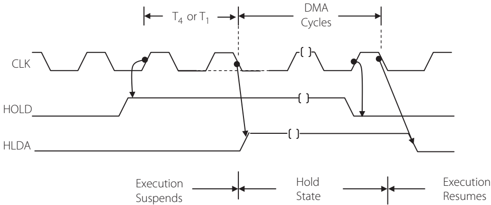
Figure 6.19 | Timing of the HOLD and HLDA signals
