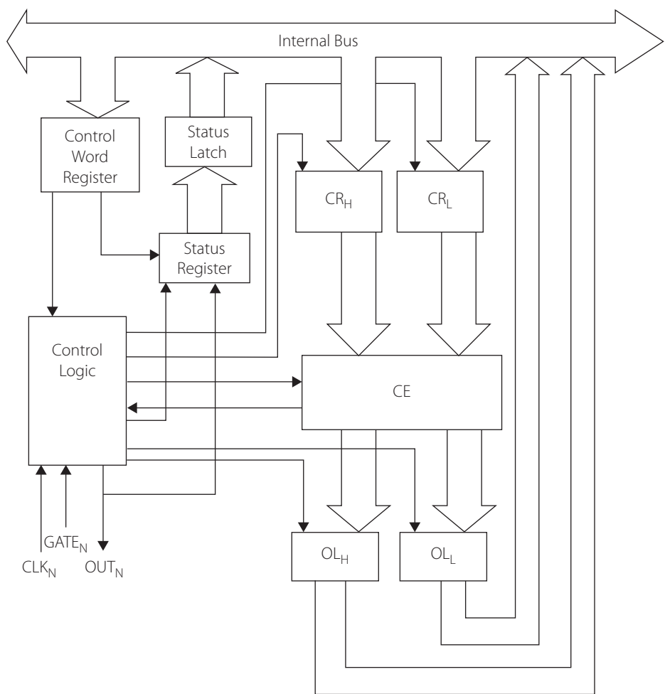
Figure 10.3 | Internal architecture of a counter
