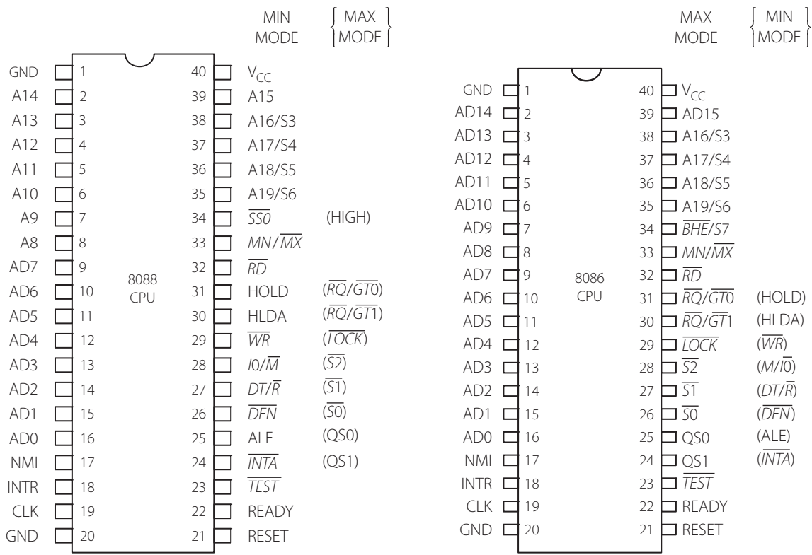
Figure 6.1a | 8088 CPU pin diagram b 8086 CPU pin diagram
