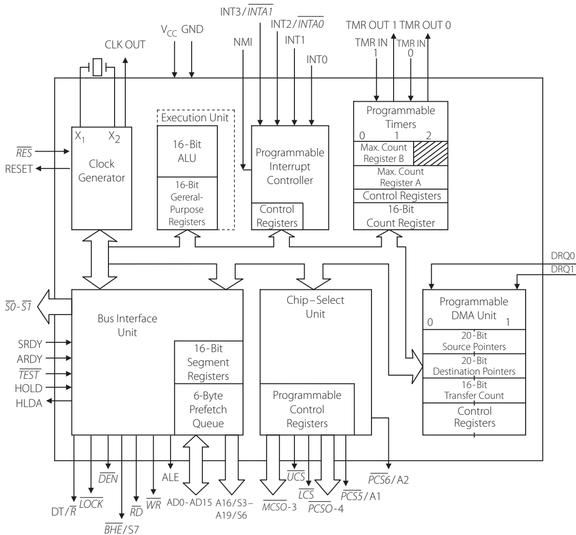
Figure 14.1 | Internal block diagram of the 80186
