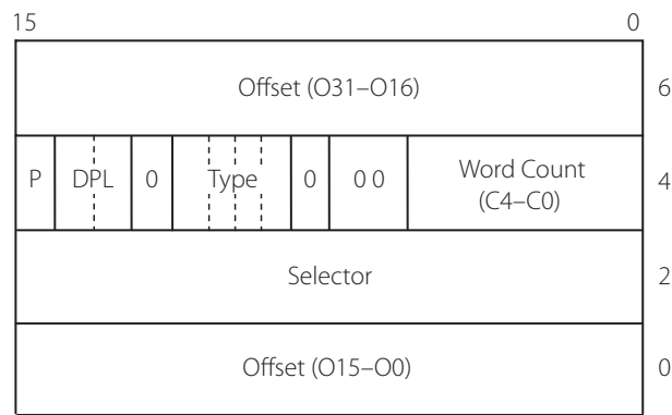
Figure 15.24 | Structure of a call gate
