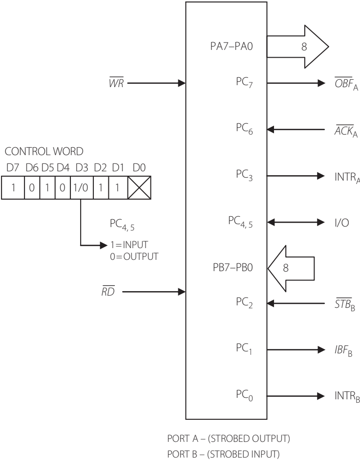
Figure 9.16 | Port A in strobed output and Port B in strobed input mode
