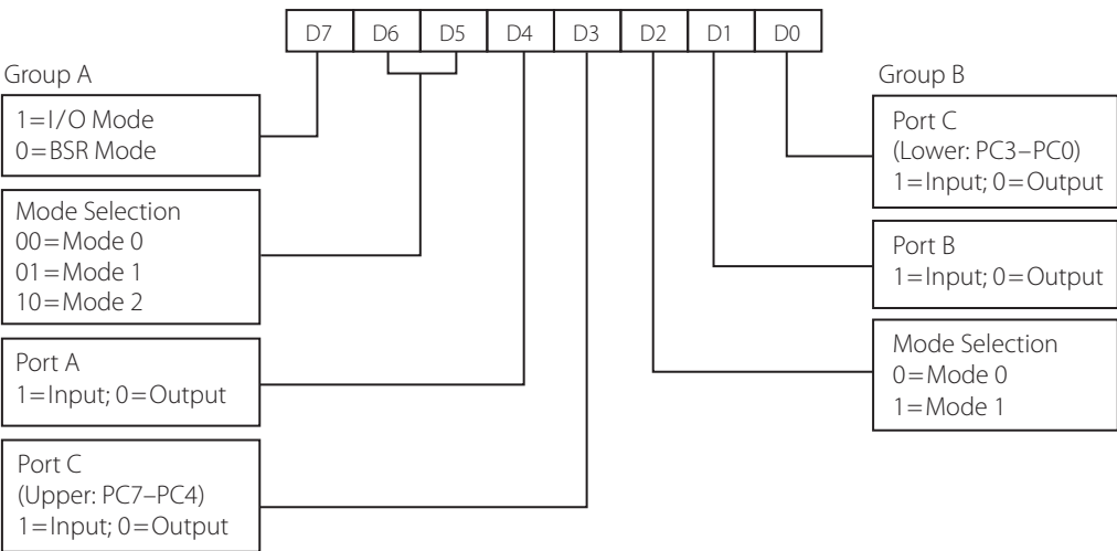
Figure 9.6 | Control word format of 8255
