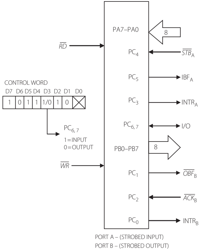
Figure 9.15 | Port A in strobed input and Port B in strobed output mode
