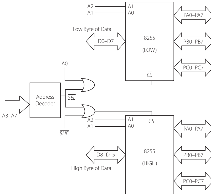
Figure 9.8 | 16-bit port interfacing using two PPIs
