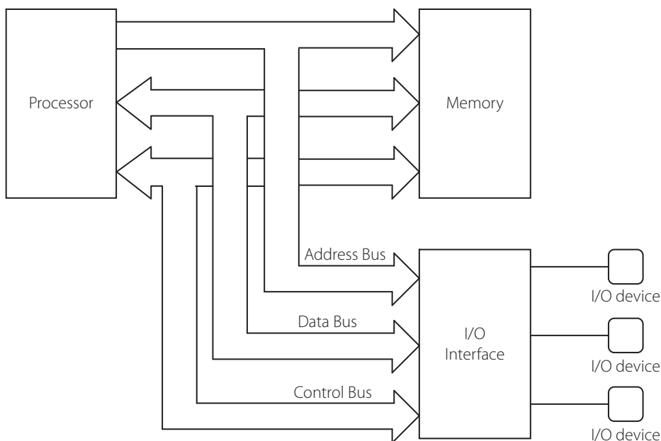
Figure 0.4 | The system bus and its components
