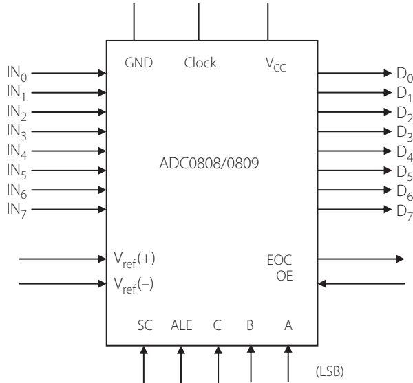
Figure 9.20 | Functional pin diagram of the ADC 0808/0809
