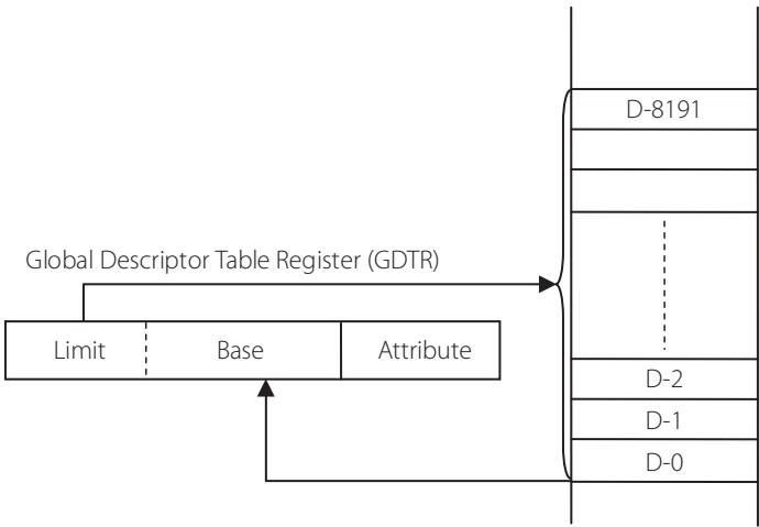
Figure 15.15 | GDT and GDTR
