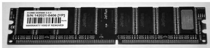
Figure 17.13 | DIMM for DDR – with three notches on the sides and one notch along the contacts
