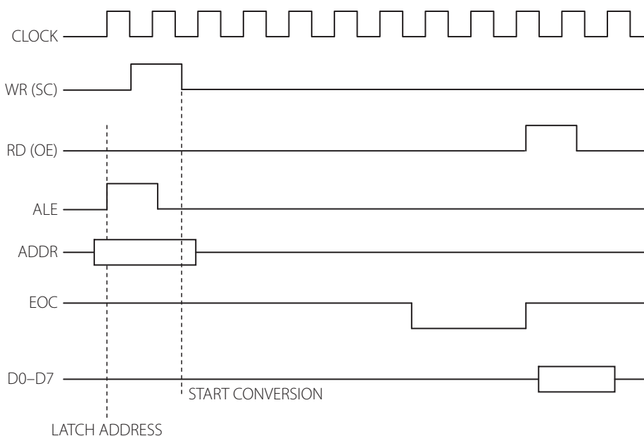
Figure 9.21 | Timing diagram for the ADC 0808/0809
