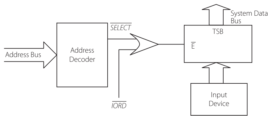
Figure 7.19 | Basic input port
