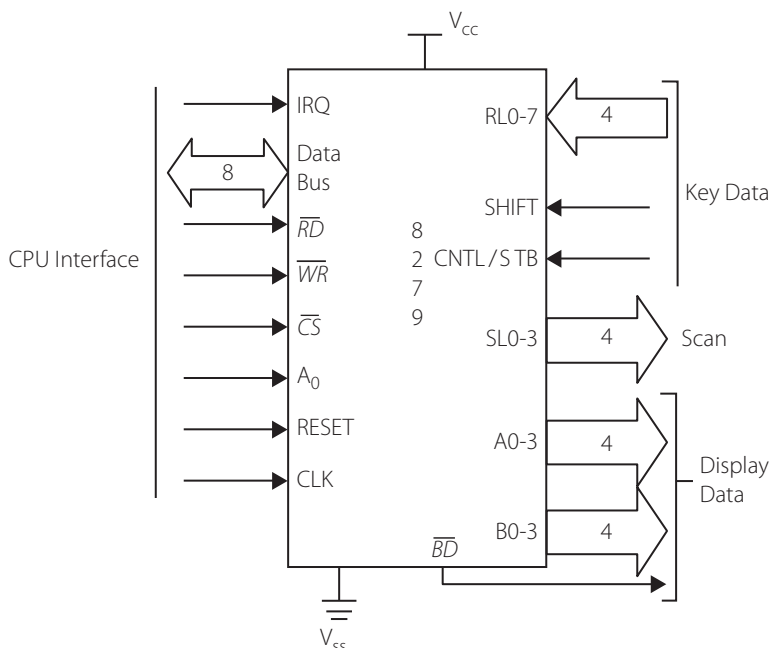
Figure 10.13 | Functional pin diagram of the 8279
