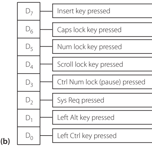
Figure 8.6b | Second keyboard status byte
