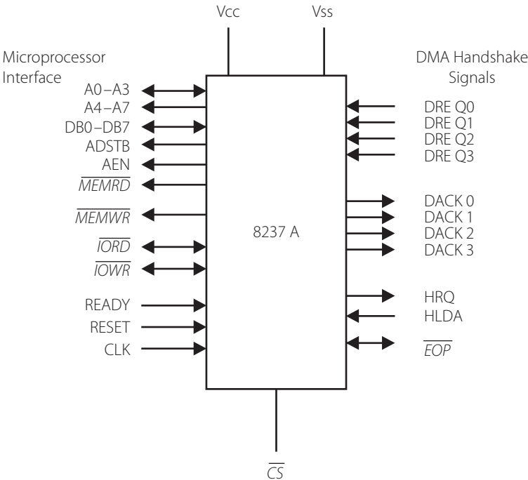
Figure 11.21 | Functional block diagram of the 8237 chip
