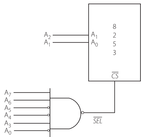
Figure 10.5 | Decoding logic for the chip
