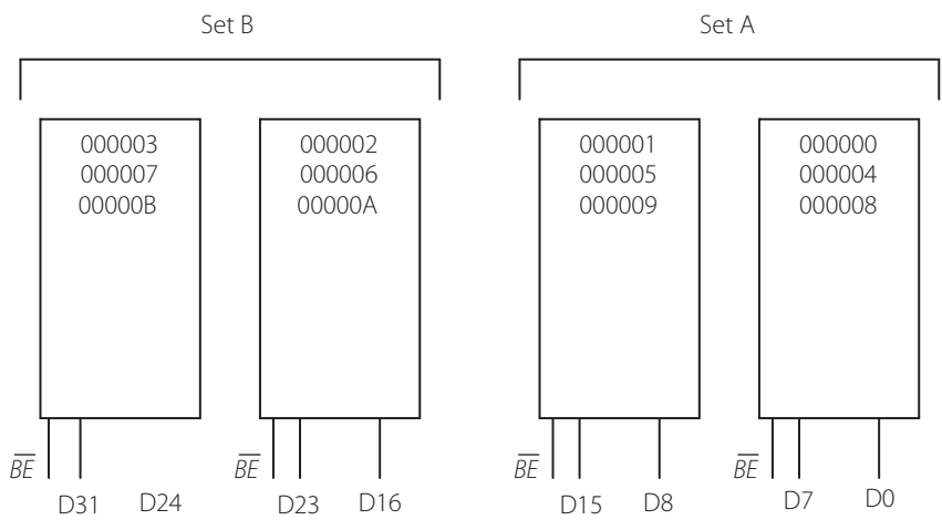
Figure 12.10 | Interleaved memory banks
