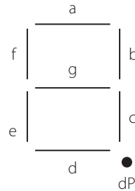
Figure 9.41 | A seven segment LED display unit
