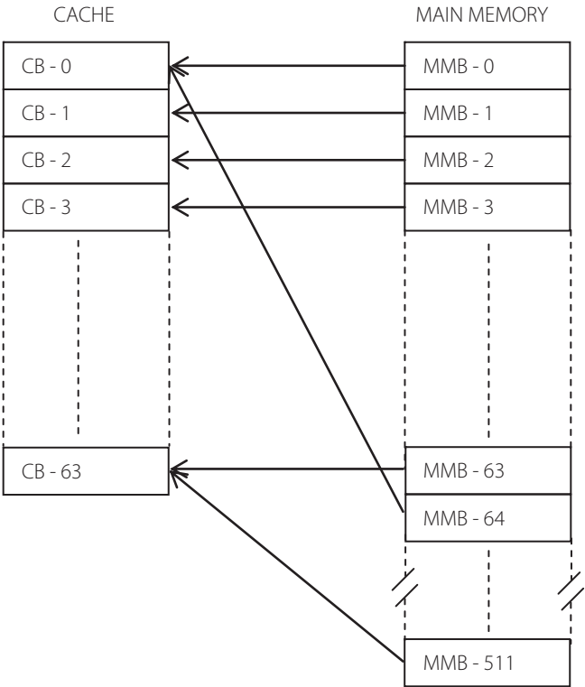
Figure 12.13 | Direct mapping
