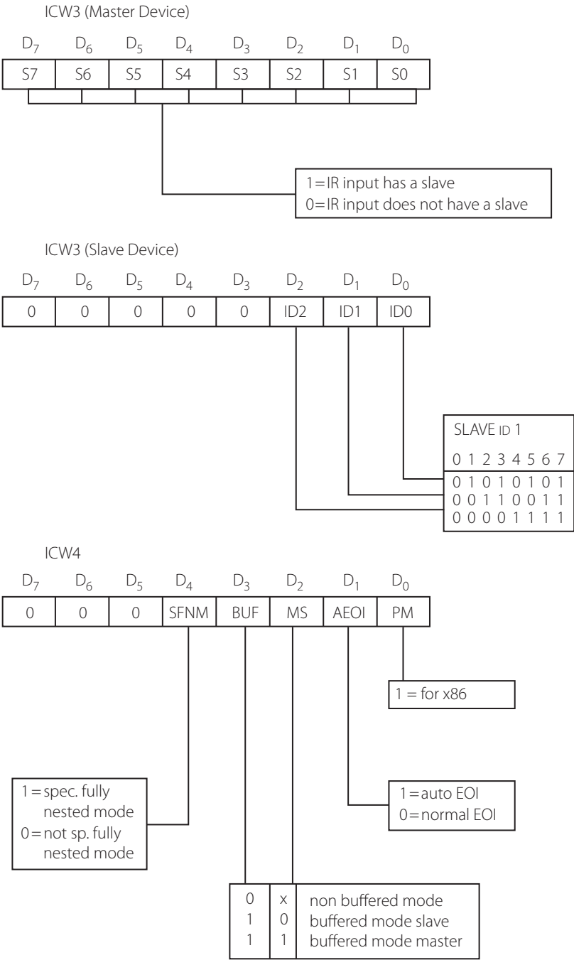
Figure 10.28 | ICW4 and ICW3
