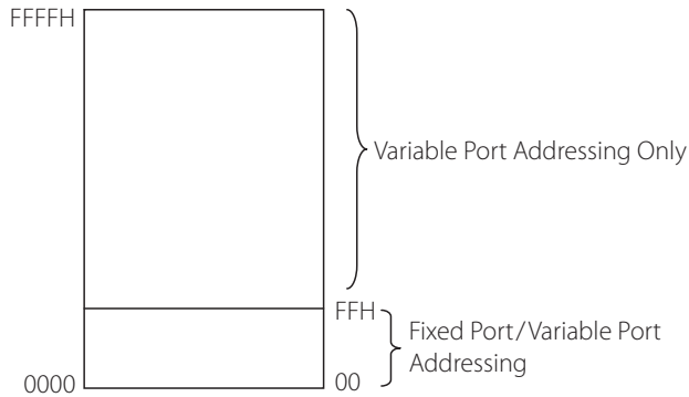
Figure 7.16 | Schemes of port addressing
