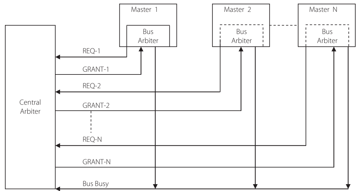
Figure 13.7b | Parallel arbitration scheme of bus arbitration
