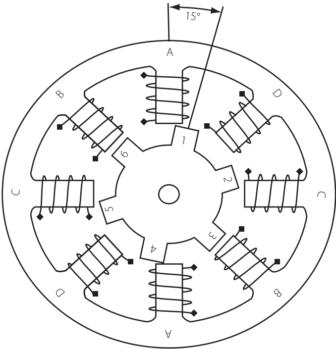
Figure 9.28 | Cross-section of a variable reluctance (VR) motor
