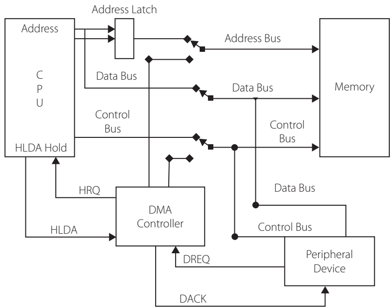
Figure 11.19 | DMA concept
