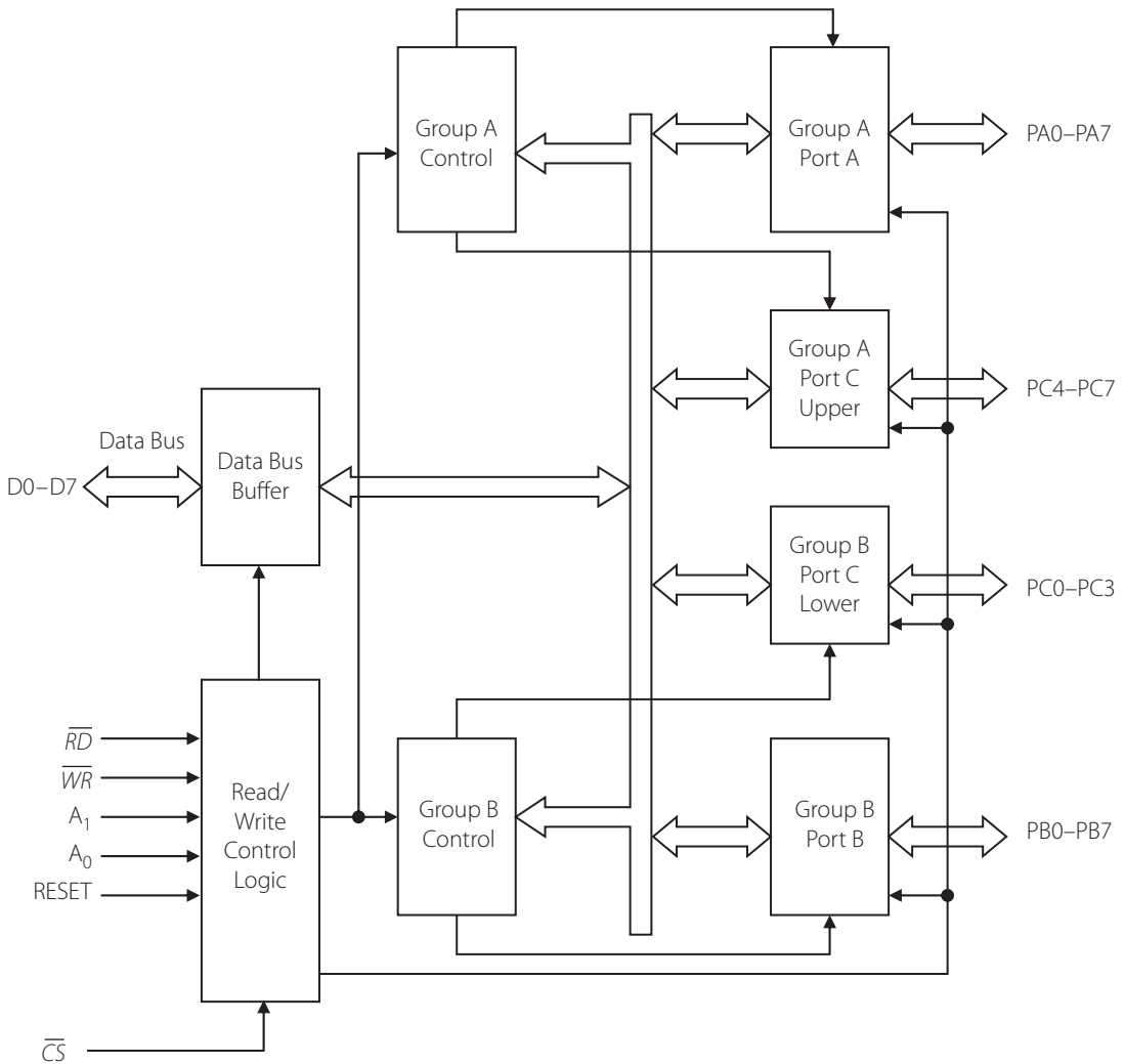
Figure 9.4 | Internal block diagram of the 8255
