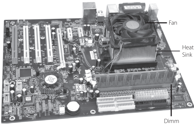
Figure 17.17 | Another view of the same motherboard with the processor covered, and a DIMM (memory module) inserted
