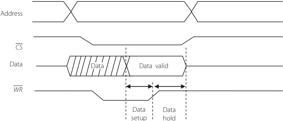
Figure 12.3 | Write cycle of a typical SRAM
