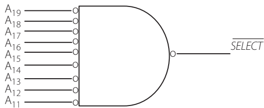
Figure 7.3 | NAND gate decoder
