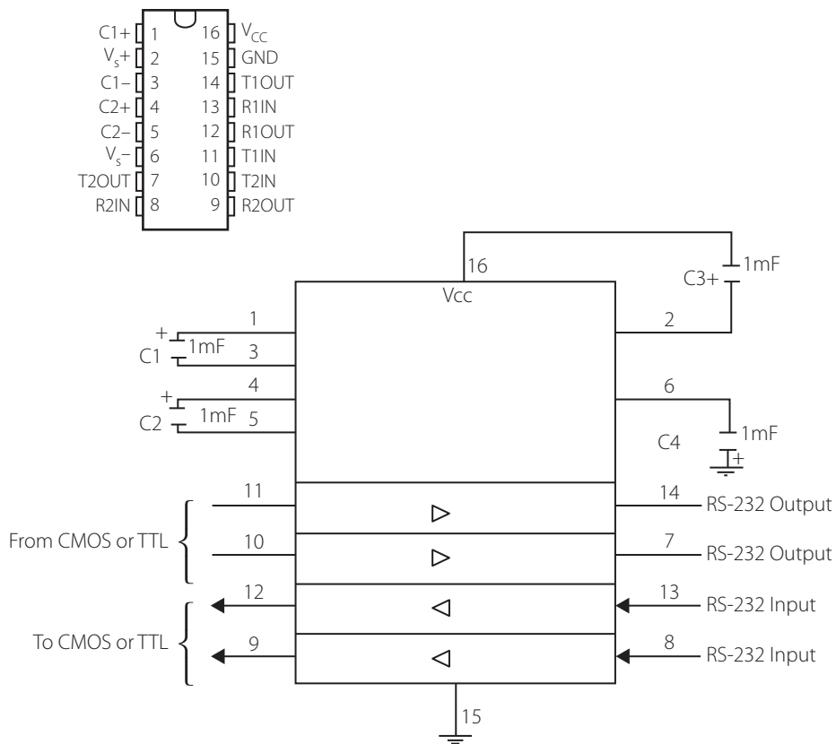
Figure 11.4 | MAX 232 chip pin diagram and a typical connection
