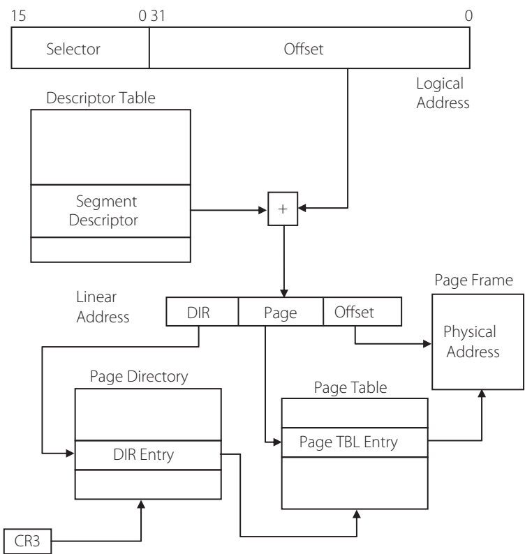
Figure 15.21 | Segmentation and paging combined
