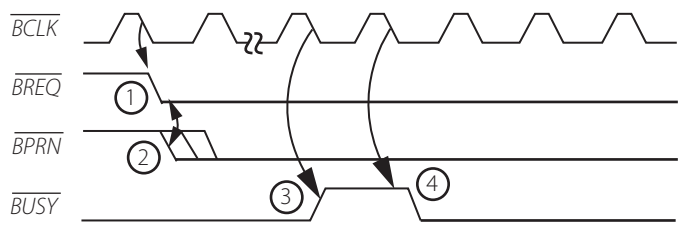
Figure 13.11 | Timing of a higher priority arbiter obtaining the bus from a lower priority arbiter
