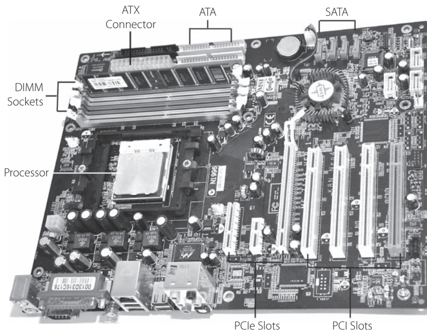
Figure 17.16 | Intel motherboard showing all the important sockets and connectors
