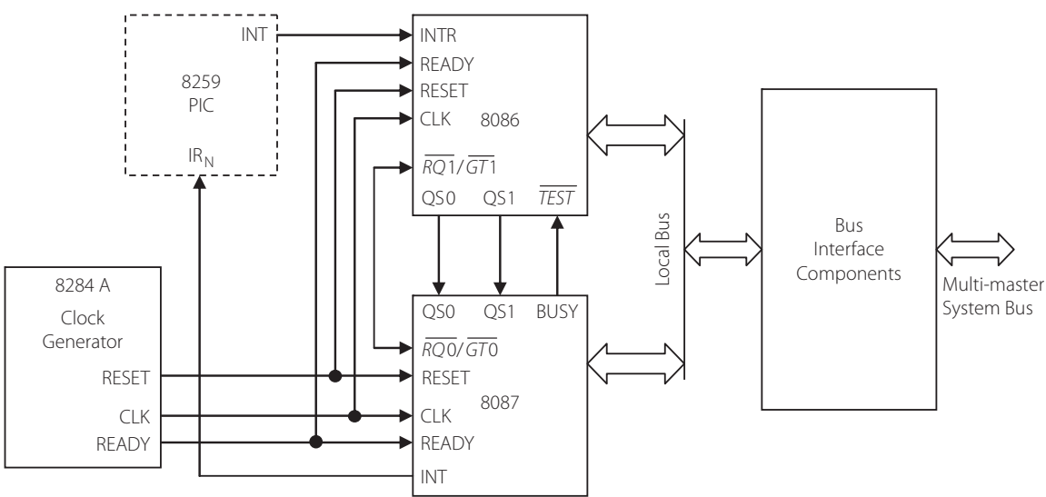
Figure 13.4 | 8086 and 8087 in a coprocessor configuration
