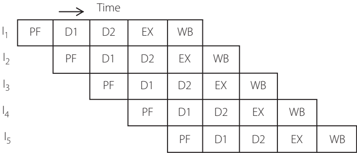
Figure 16.1 | Five stage pipeline of the 80486
