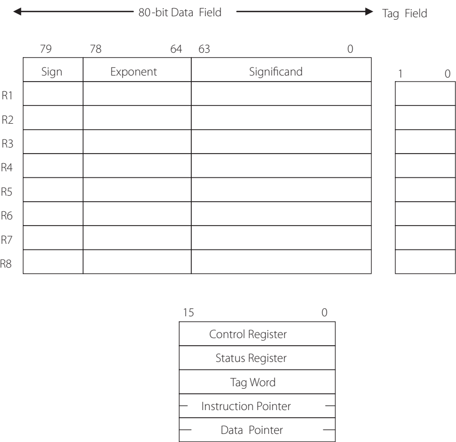
Figure 13.15 | Register structure of the 8087
