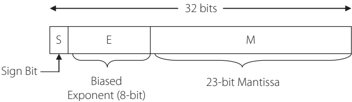
Figure 13.13 | Single precision representation
