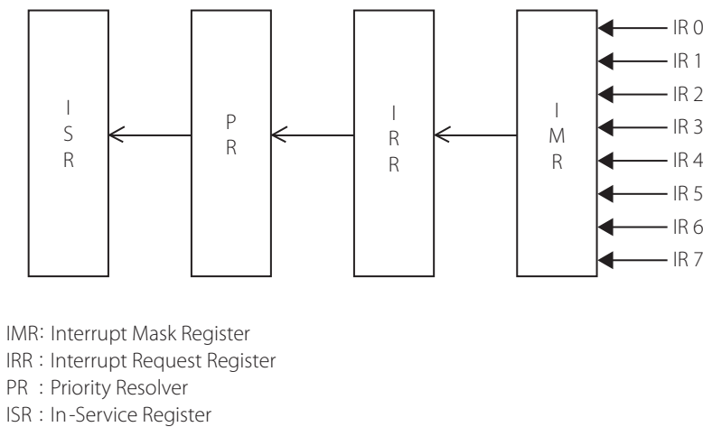
Figure 10.24 | Interrupt Sequence and the registers involved
