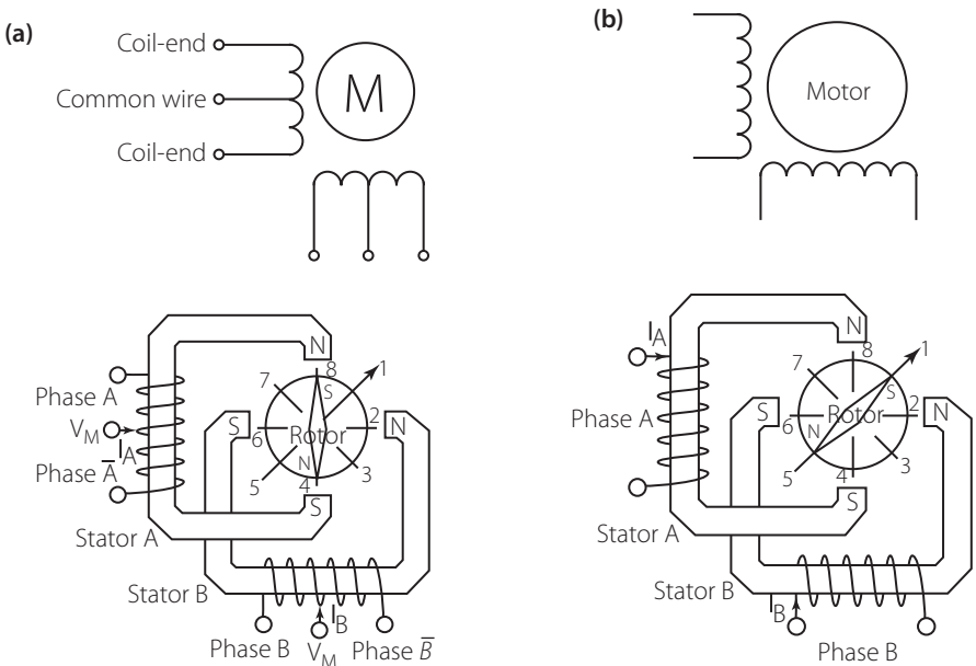
Figure 9.31 | a Unipolar motor
