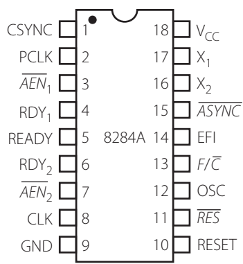
Figure 6.9 | Pin configuration of the clock generator 8284A
