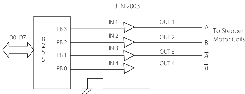
Figure 9.33 | Connection diagram of a stepper motor using the ULN 2003 IC
