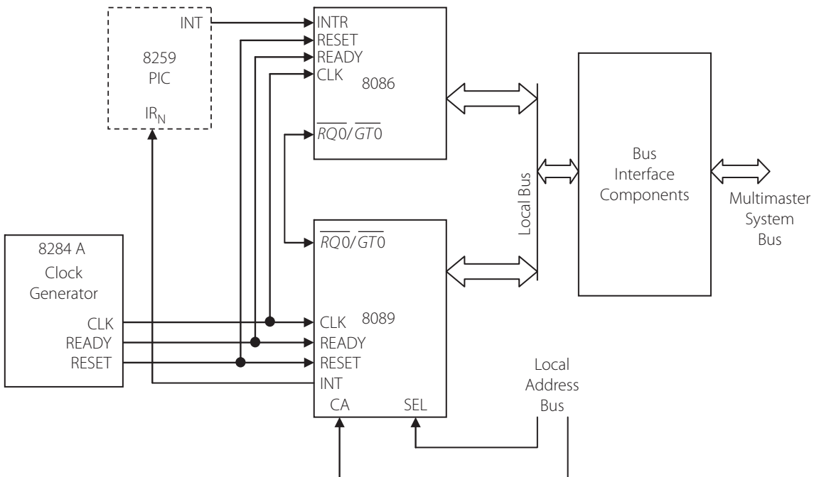
Figure 13.5 | The 8086 in a tightly coupled configuration with the 8089 IOP
