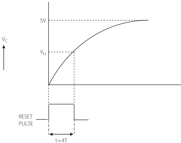
Figure 6.12 | Charging of the capacitor and generation of reset pulse
