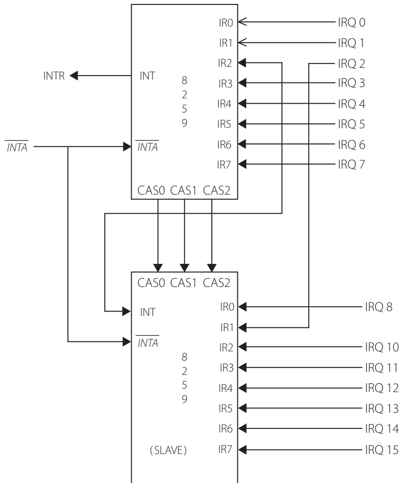
Figure 10.31 | PICs used in the PC-AT
