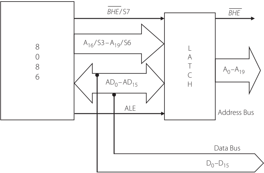
Figure 6.3 | Block diagram of the de-multiplexed address /data bus
