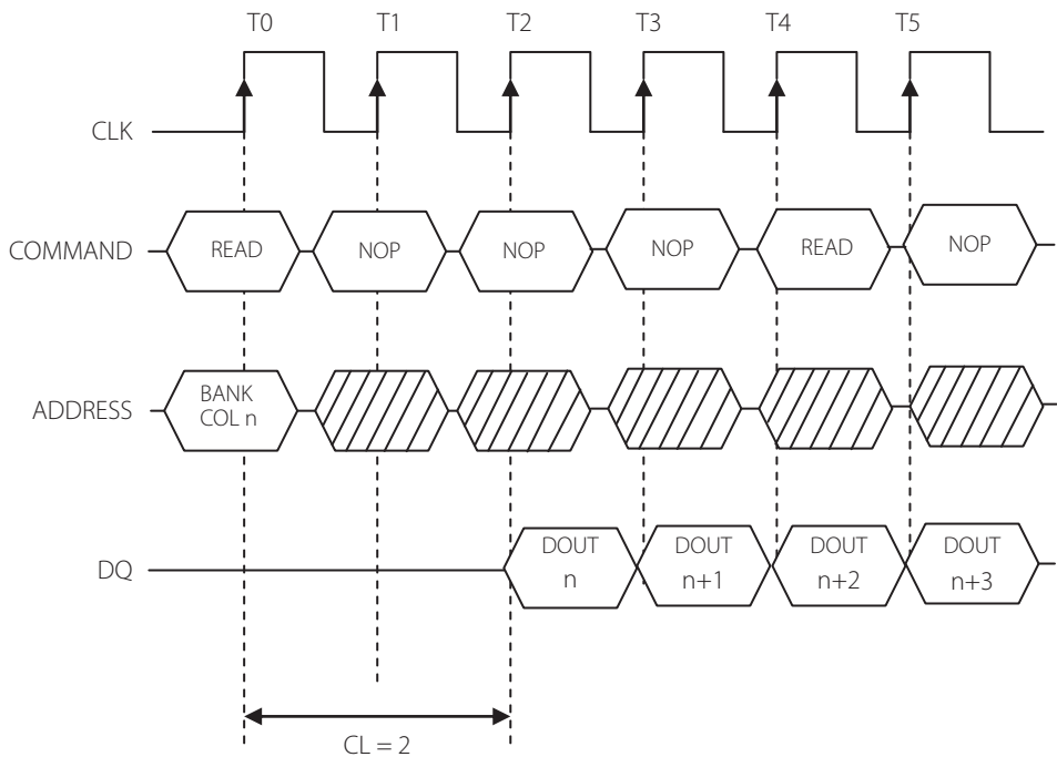
Figure 12.11 | DRAM ‘read’ cycle with a burst length of 4
