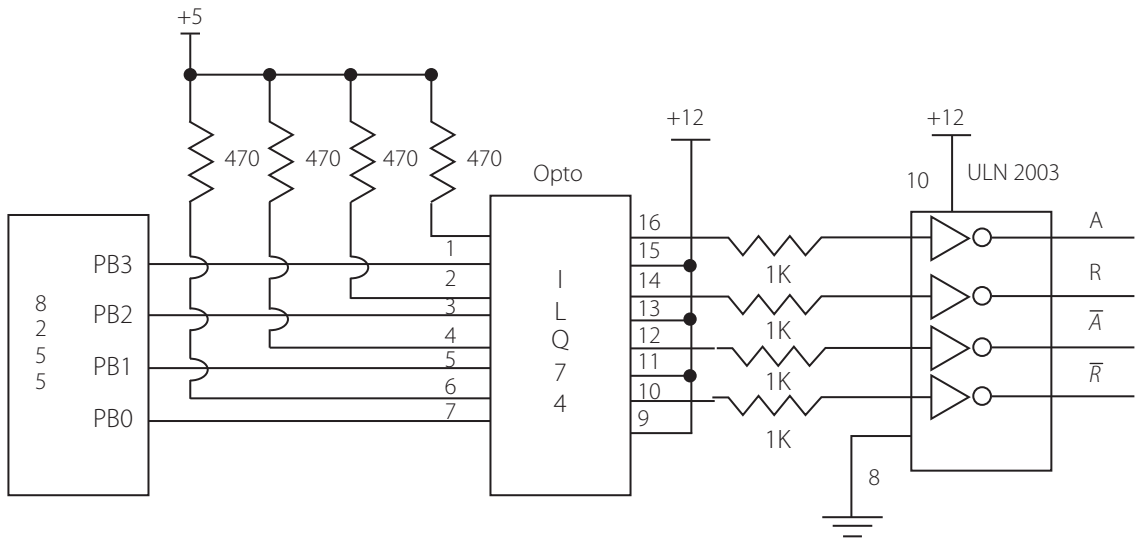
Figure 9.37 | Optocoupler used in a stepper motor driving circuit
