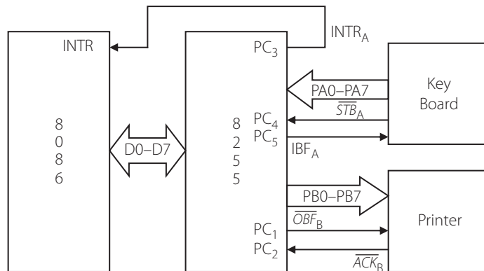
Figure 9.17 | Connecting a keyboard and a printer to the 8086 in Mode 1
