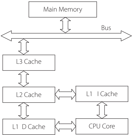
Figure 12.16 | Caches for a current x86 processor
