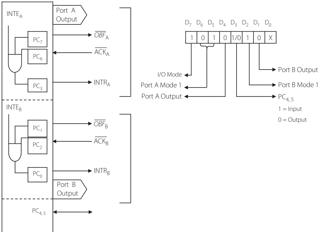
Figure 9.12 | Mode 1: Strobed output – Pin configuration and control word format
