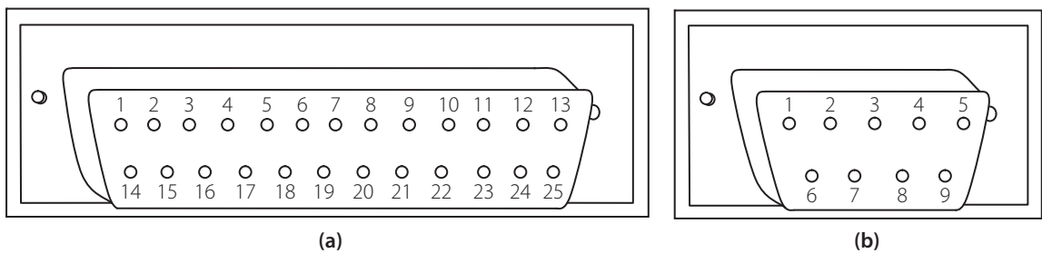
Figure 11.5 | RS-232 connectors a DB-25 male connector b DB-9 male connector
