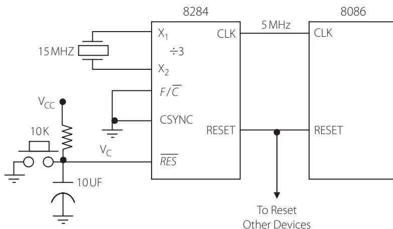
Figure 6.11 | 'Power on reset' circuit
