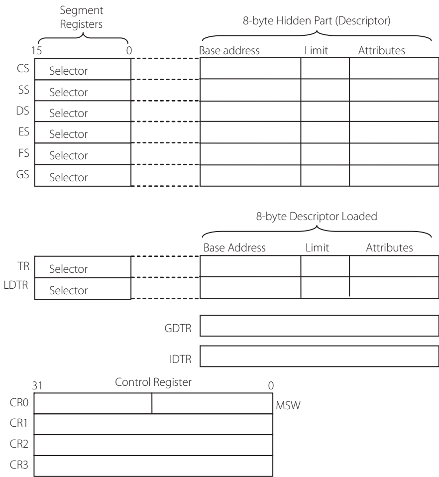
Figure 15.14 | Address translation registers
