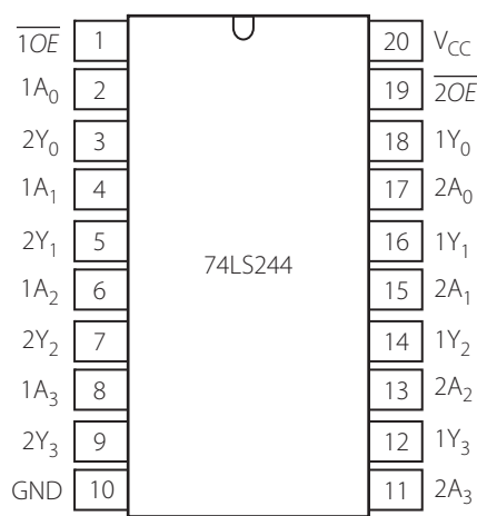
Figure 7.20 | Functional pin diagram of the octal tri-state buffer 74LS244
