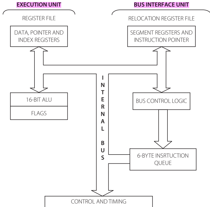
Figure 1.1a | Internal block diagram of the 8086 (simplified model)
