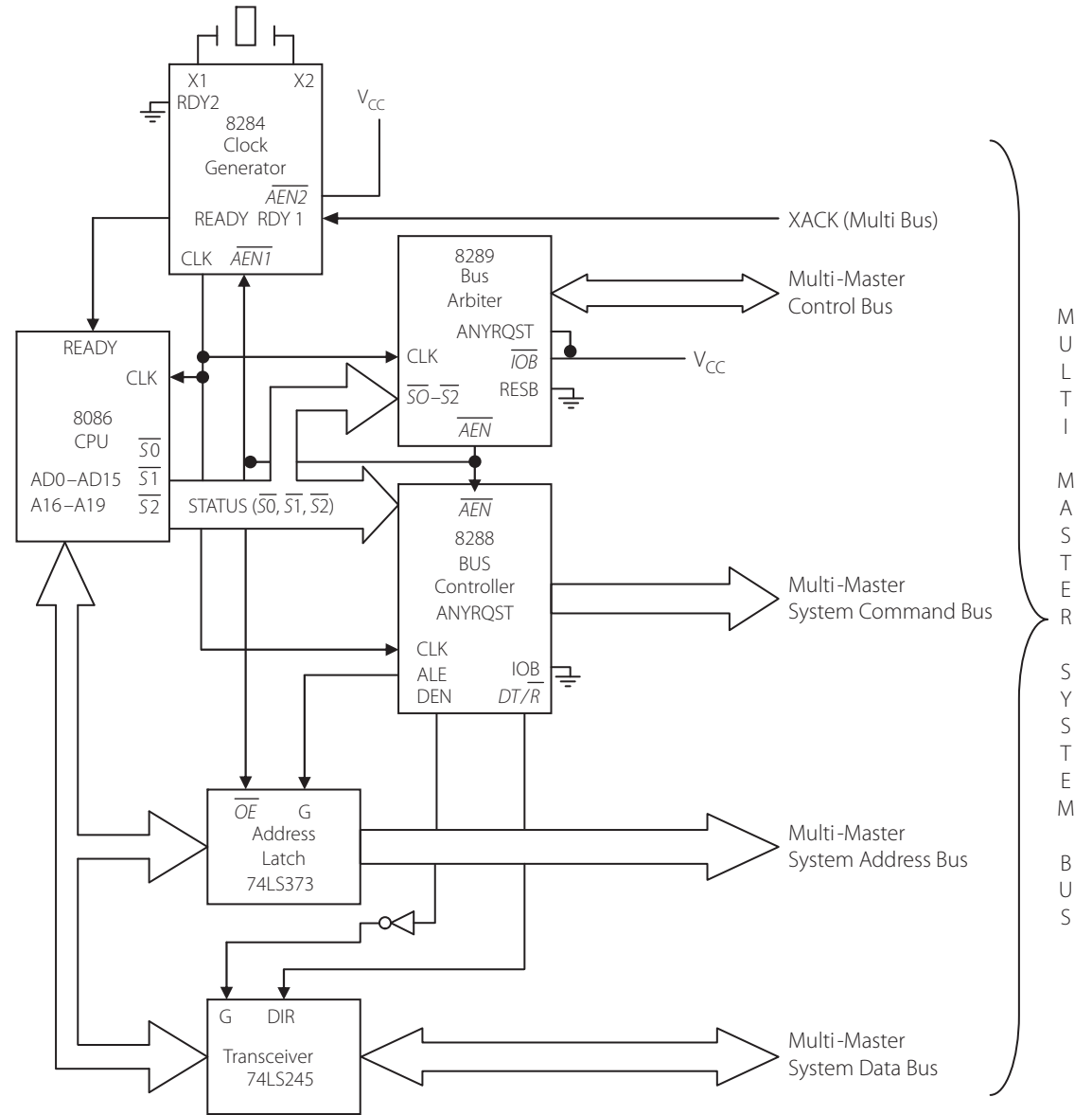
Figure 13.9 | One processing module in a loosely coupled system, shown with the bus arbiter
