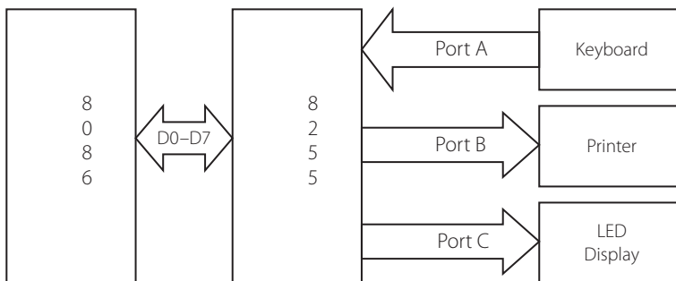
Figure 9.2 | The connections between an 8086, 8255 and three peripherals
