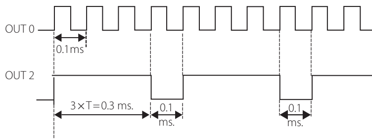
Figure 10.11 | OUT 0 and OUT 2 outputs
