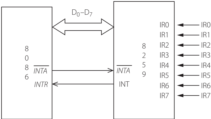
Figure 10.21 | Basic connections between a PIC 8259 and the 8086
