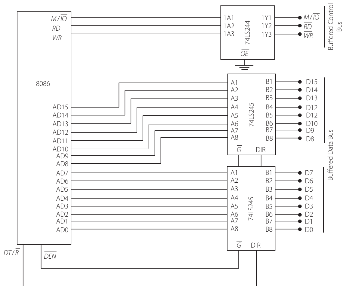
Figure 6.7 | Buffered data bus and control pins
