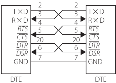
Figure 11.7 | DTE–DTE connection using a null modem connection
