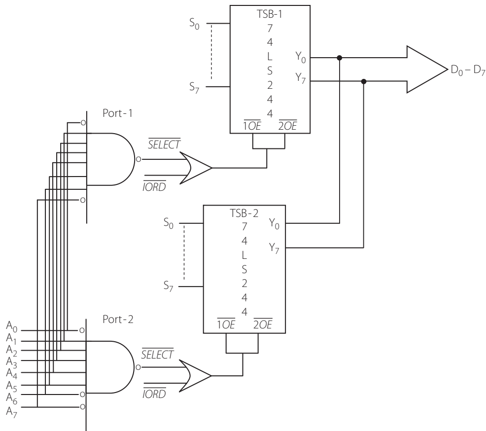
Figure 7.21 | Two sets of switches acting as two 8-bit input ports
