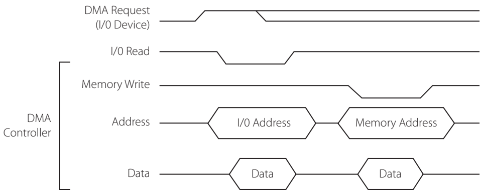
Figure 11.18 | Timing for fetch and deposit DMA
