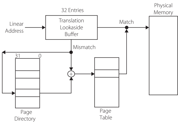
Figure 15.20 | Translation lookaside buffer inside the 80386 chip
