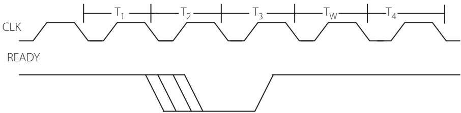
Figure 6.15 | Sampling the READY signal and inserting wait states
