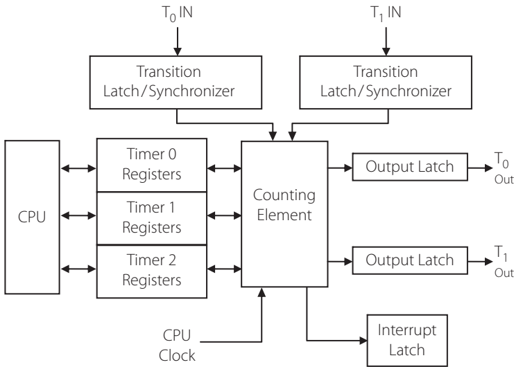
Figure 14.5 | Timer/counter – internal block diagram
