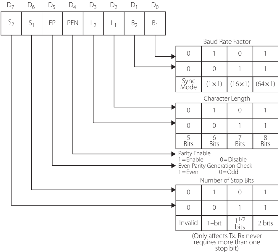
Figure 11.11 | Mode control word
