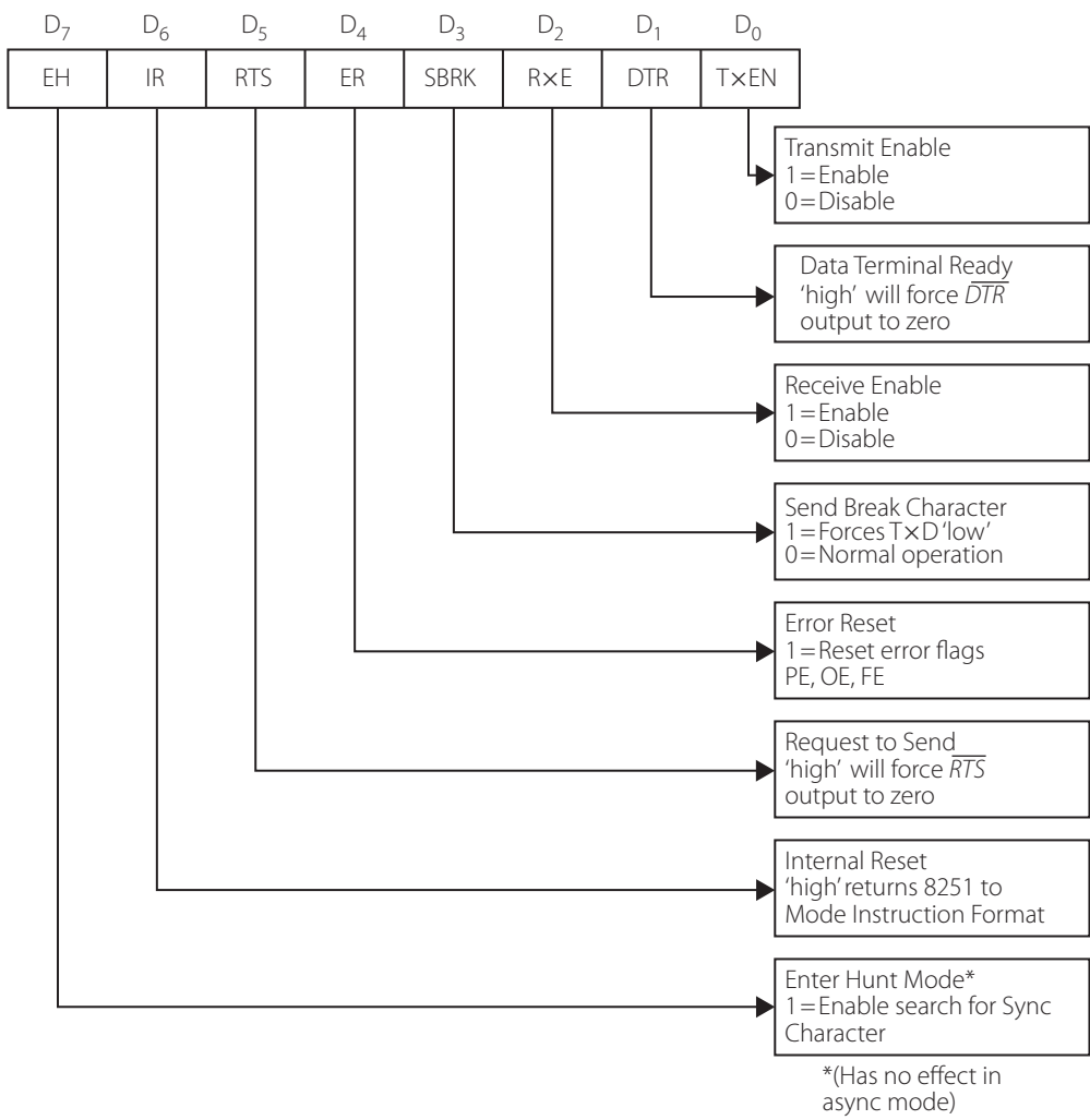
Figure 11.14 | Command instruction format
