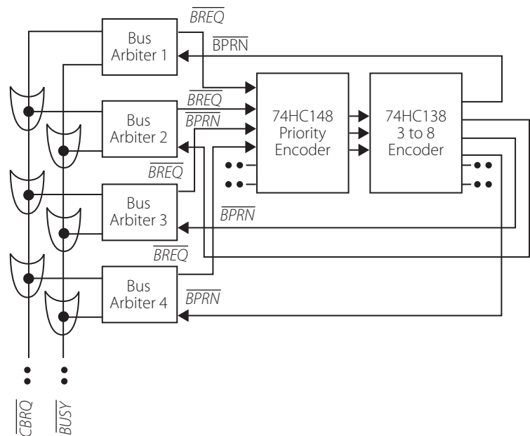
Figure 13.10 | Implementing the parallel arbitration scheme using an 8289
