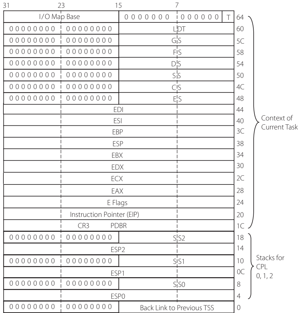
Figure 15.25 | Structure of a typical TSS
