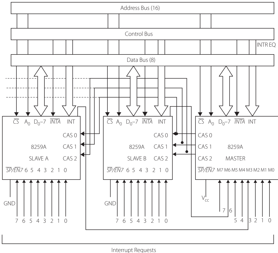
Figure 10.30 | Cascaded connection of three PICs
