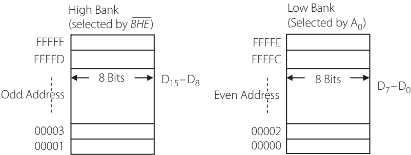
Figure 7.12 | Memory banks of 8086
