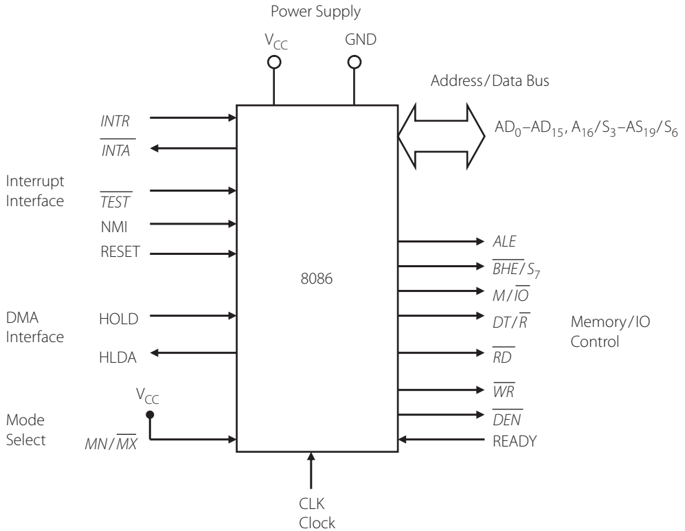
Figure 6.20 | 8086 in the minimum mode configuration
