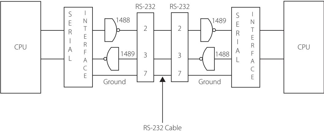
Figure 11.3 | Serial communication using RS 232 cable and line drivers/receivers
