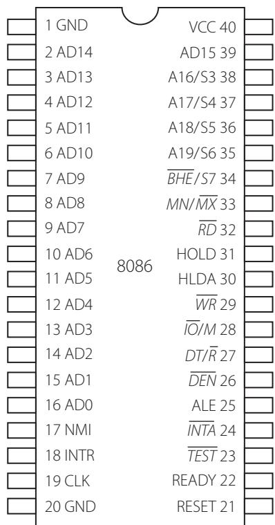
Figure 6.2 | 8086 pins in the minimum mode
