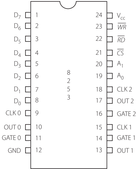
Figure 10.1 | Pin diagram of 8253/8254
