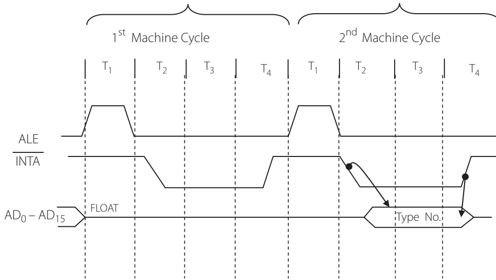
Figure 8.3 | Interrupt acknowledge machine cycle of the 8086
