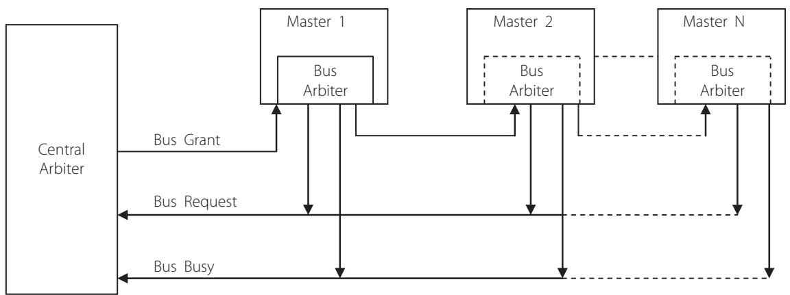
Figure 13.7a | Daisy chaining scheme of bus arbitration
