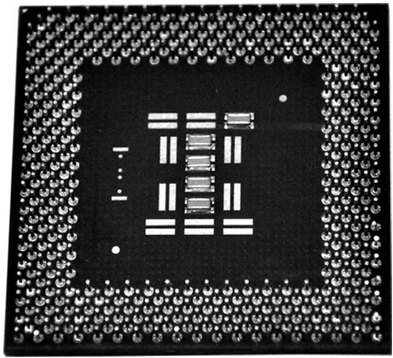
Figure 15.4 | A pin grade array (PGA)
