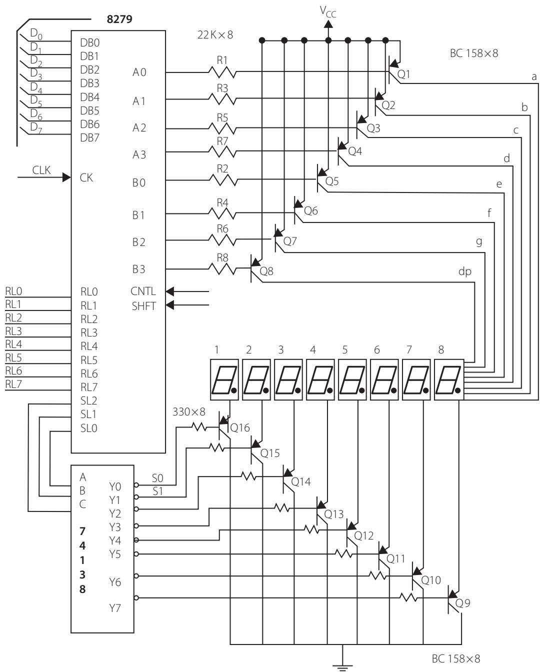
Figure 10.14 | Display interface part of the 8279
