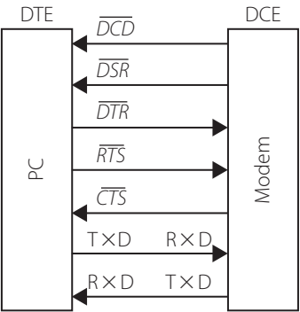
Figure 11.6 | Typical DTE–DCE connection
