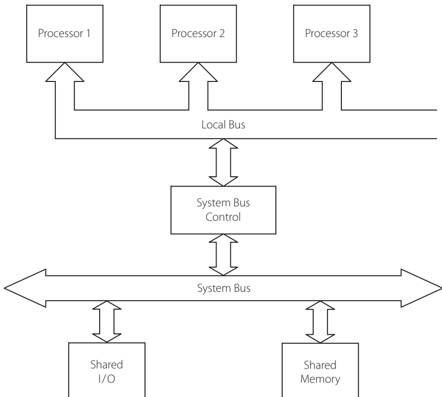
Figure 13.1 | Tightly coupled multiprocessor system
