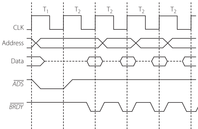
Figure 16.3 | Burst mode data transfer
