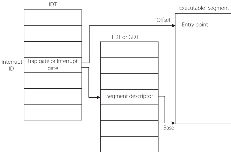
Figure 15.26 | Interrupt vectoring
