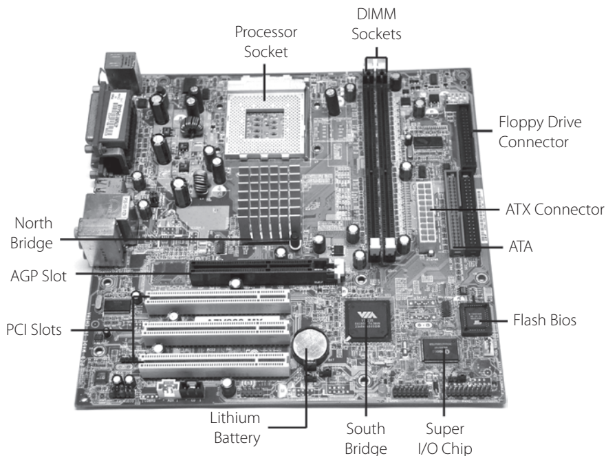
Figure 17.1 | A motherboard with important parts marked and labeled
