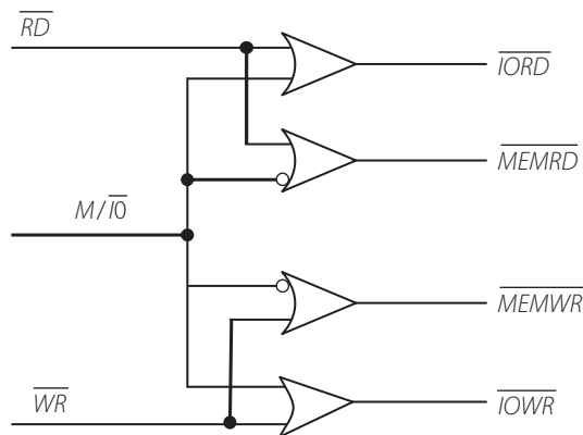
Figure 6.8 | Generation of memory and I/O read/write signals
