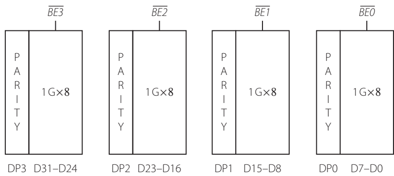
Figure 16.4 | Memory banks of 80486
