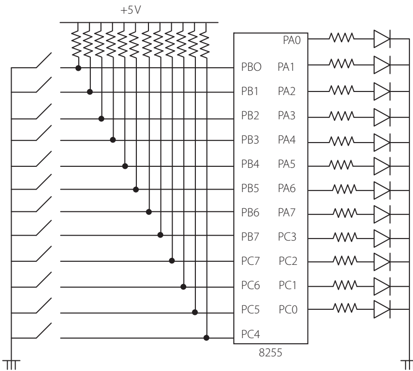
Figure 9.7 | Connection of switches and LEDs to an 8255
