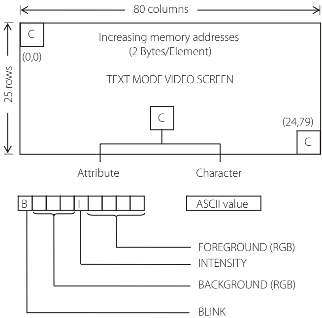
Figure 8.5 | Text mode video screen
