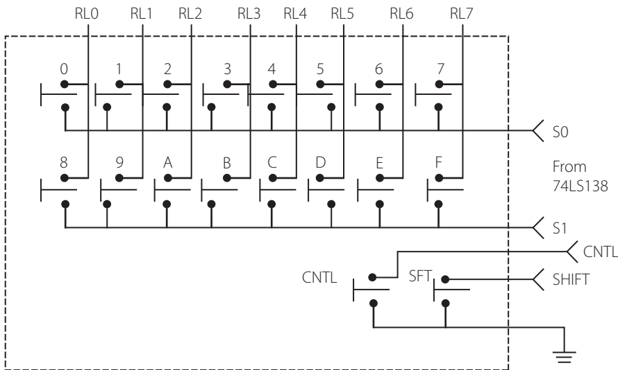
Figure 10.16 | Keyboard section
