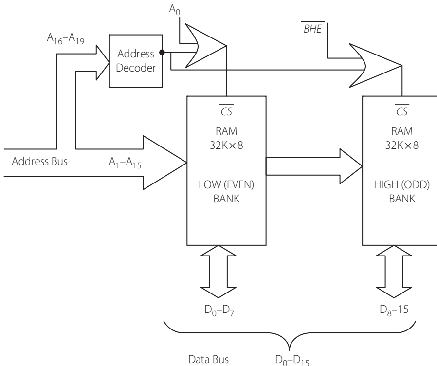
Figure 7.13 | Memory banks with the respective bank enables signals, along with the decoder
