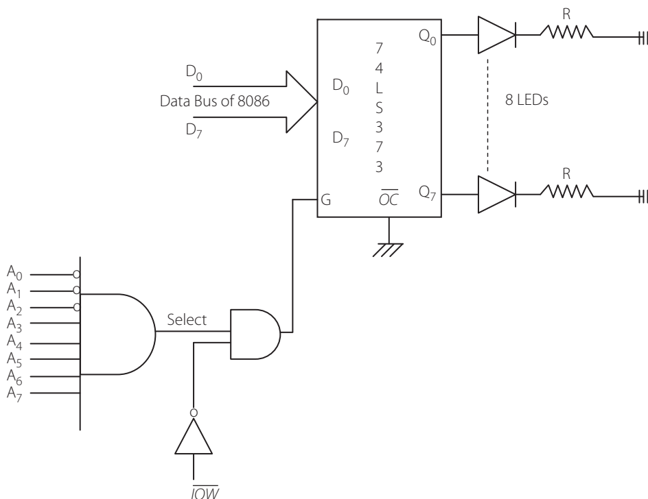
Figure 7.18 | Output port with 8 LEDs interfaced to it
