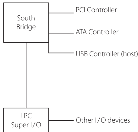
Figure 17.4 | South bridge supplemented by the super I/O chip
