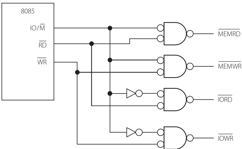
Figure 0.15 | Generating separate control signals for memory and I/O
