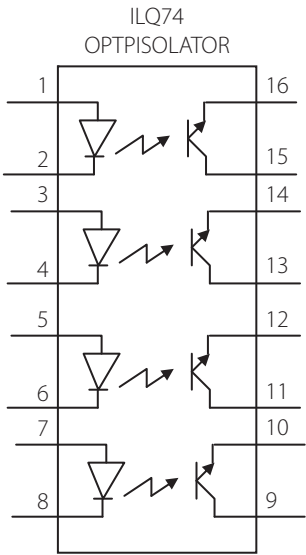
Figure 9.35 | Principle of operation of an optocoupler
