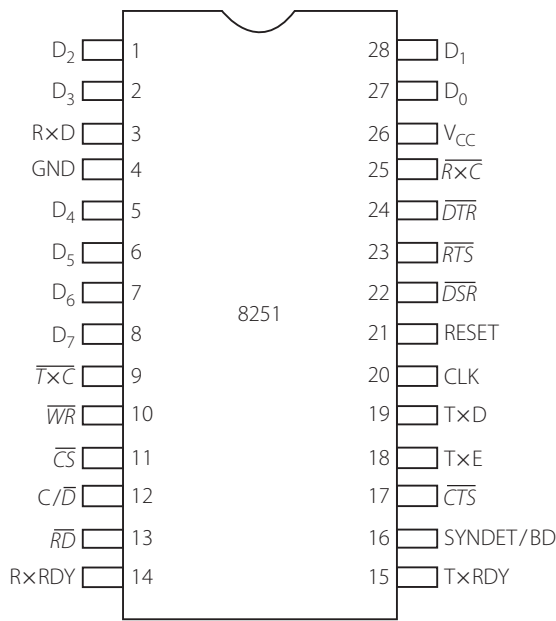
Figure 11.9 | Pin diagram of the USART
