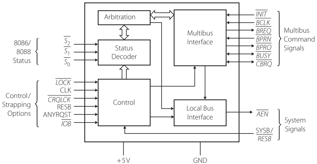
Figure 13.8 | Internal block diagram of the 8289 bus arbiter
