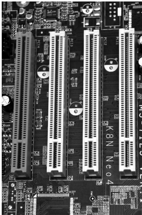
Figure 17.6 | Four PCI slots on a motherboard
