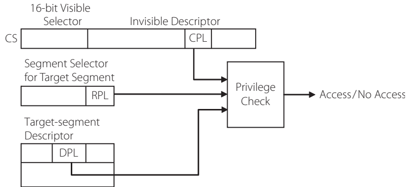
Figure 15.23 | Privilege level checks for a task when accessing a data segment
