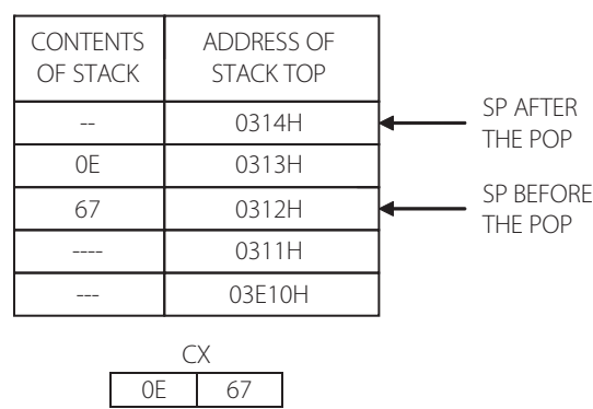
Figure 3.2 | POP operation in a stack
