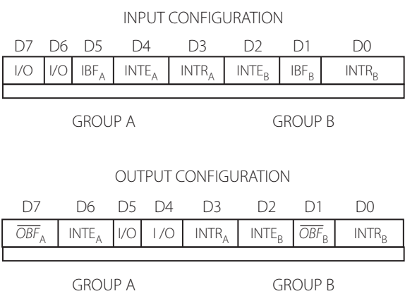
Figure 9.14 | Status of Port C for input and output configurations of Mode 1
