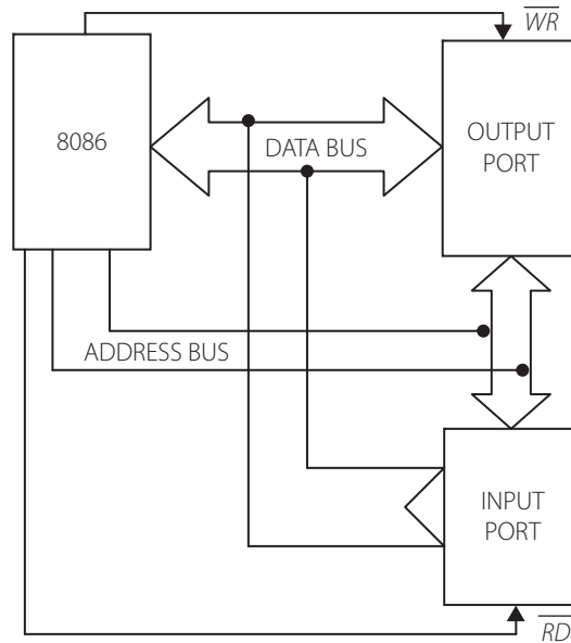
Figure 5.1 | I/O ports with address bus and data bus and the read and write control signals
