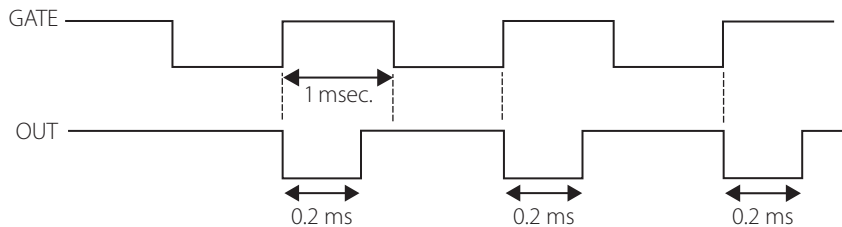
Figure 10.9 | Output waveform of Example 10.6
