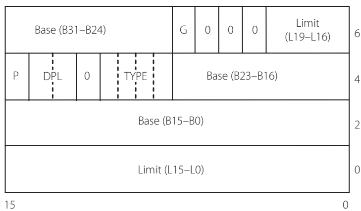
Figure 15.11 | Descriptor for a system segment
