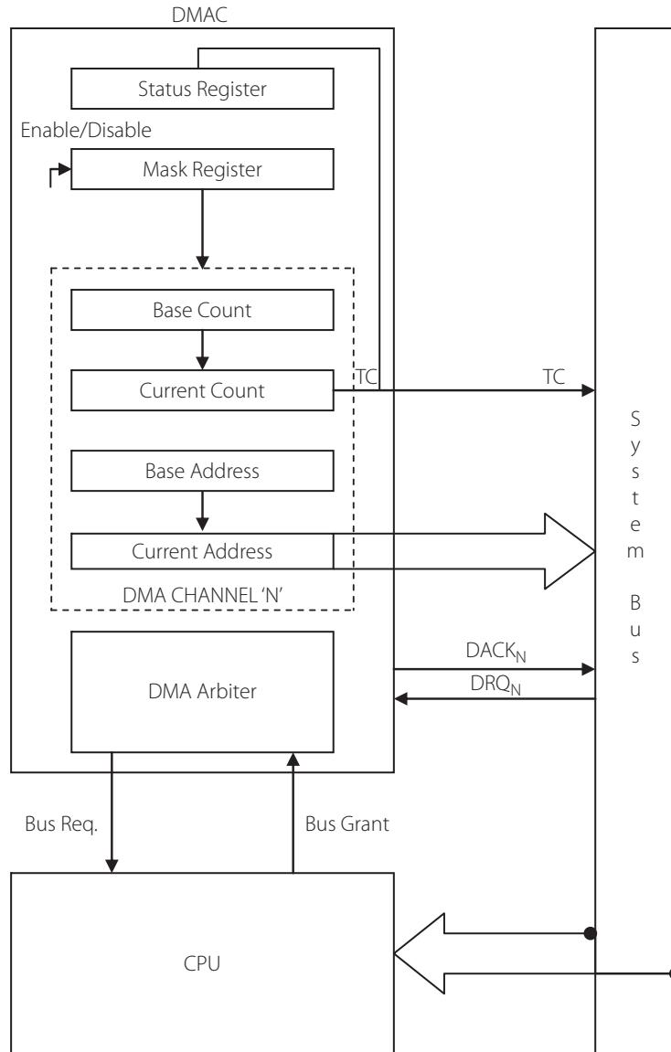
Figure 11.20 | A general block diagram of a DMA controller
