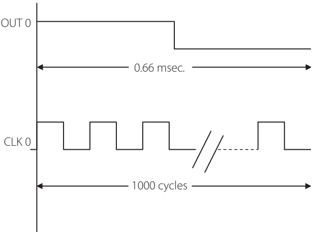
Figure 10.6 | Output waveform corresponding to Example 10.3
