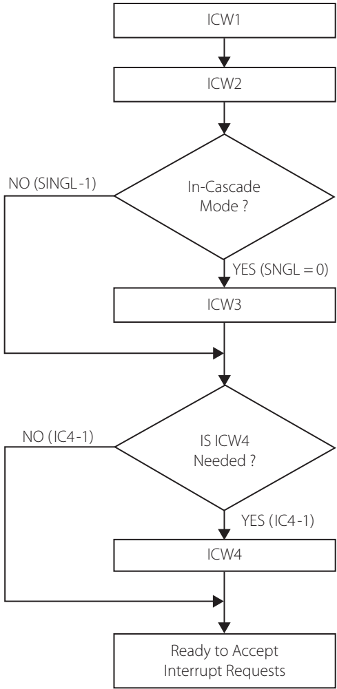
Figure 10.25 | Flow chart showing the initialization sequence for the PIC
