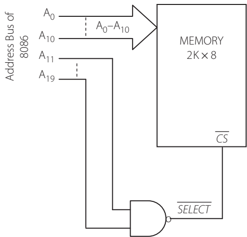
Figure 7.2 | Memory with address decoding
