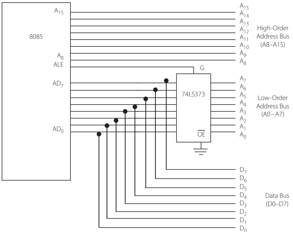
Figure 0.14 | Address and data de-multiplexing
