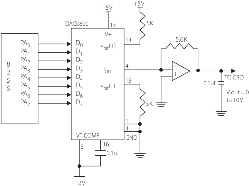
Figure 9.24 | Connections between the 8255 and DAC
