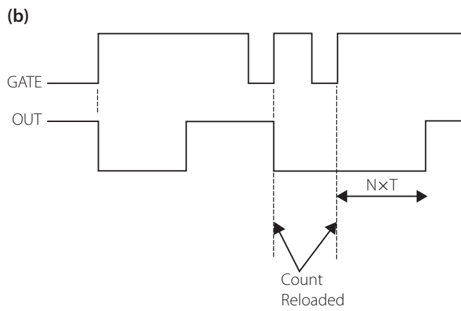
Figure 10.8b | Output waveform when a new L to H transition is given to the GATE before N \times T is reached
