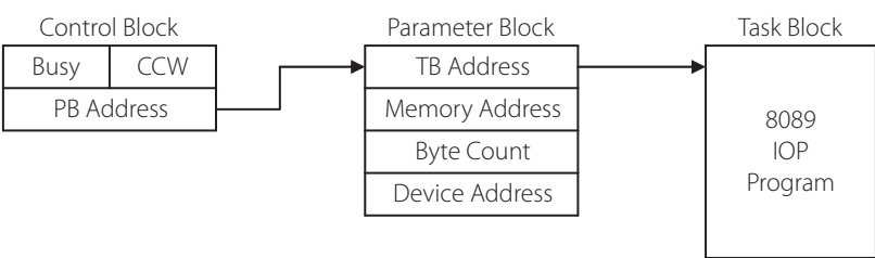
Figure 13.6 | Location of information in memory for I/O operations in an 8089 system
