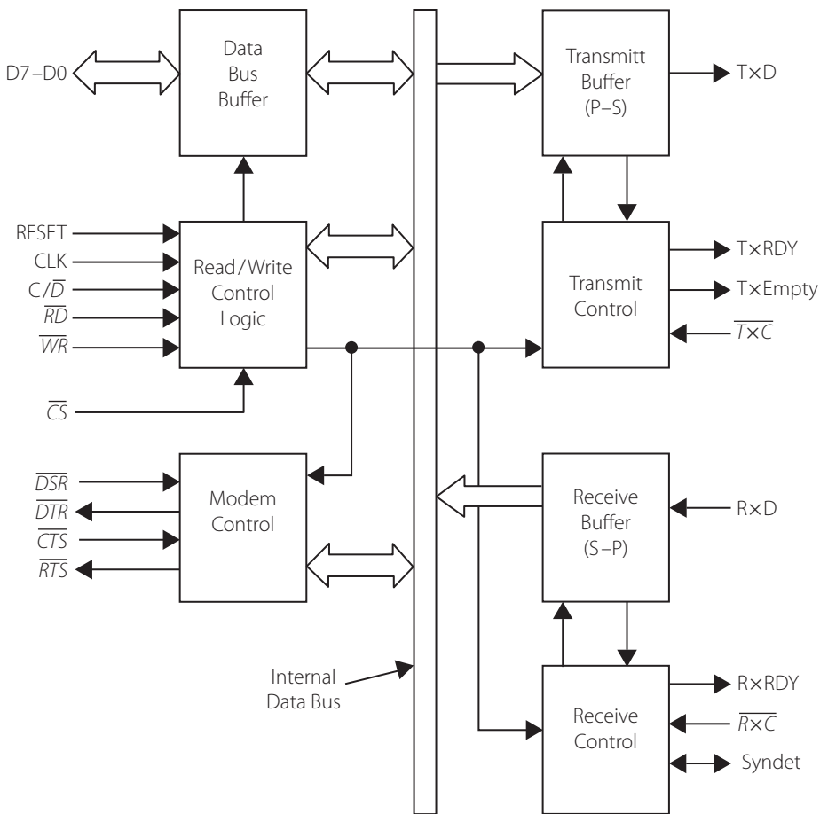
Figure 11.10 | Internal block diagram of the 8251
