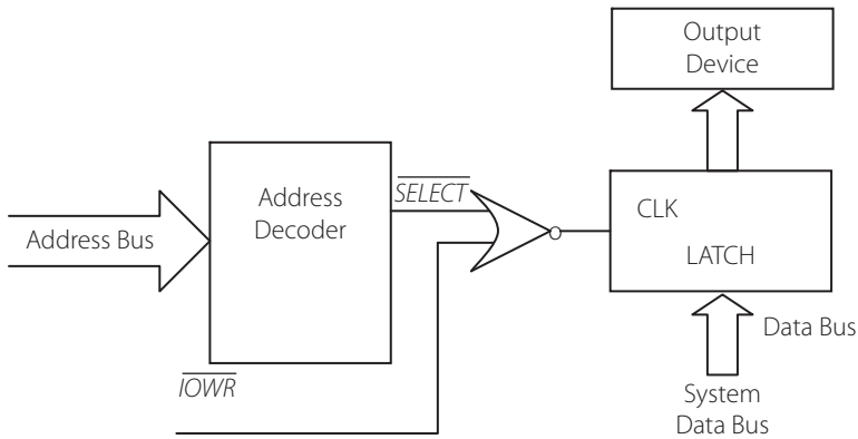
Figure 7.17 | Basic output port setup
