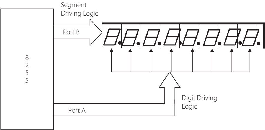
Figure 9.42 | Eight digit dynamic display connected to two ports of an 8255
