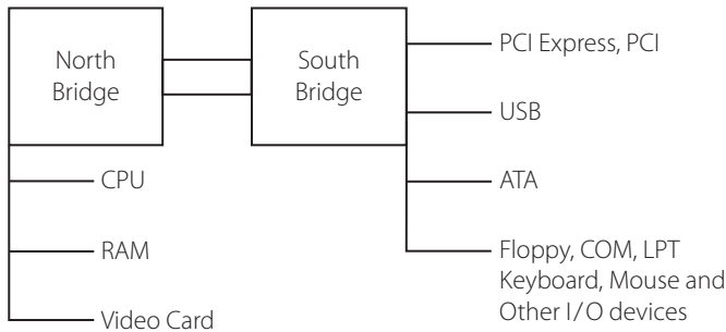
Figure 17.3 | The north bridge and the south bridge
