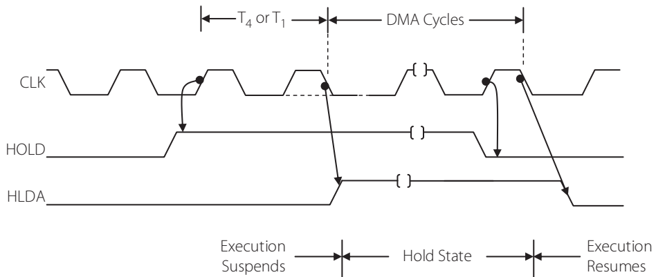
Figure 11.16 | DMA cycle timings
