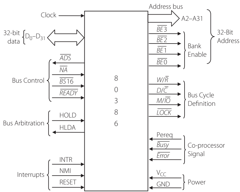
Figure 15.3 | Functional pin diagram of the 80386
