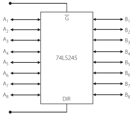
Figure 6.6 | Pin diagram of the octal tri-state bi-directional buffer 74LS245
