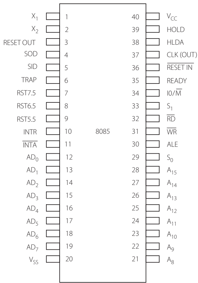
Figure 0.13 | Pin Diagram of the 8085
