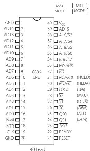
Figure 2 | 8086 pin configuration
