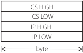
Figure 8.2b | A typical interrupt vector (4 bytes)
