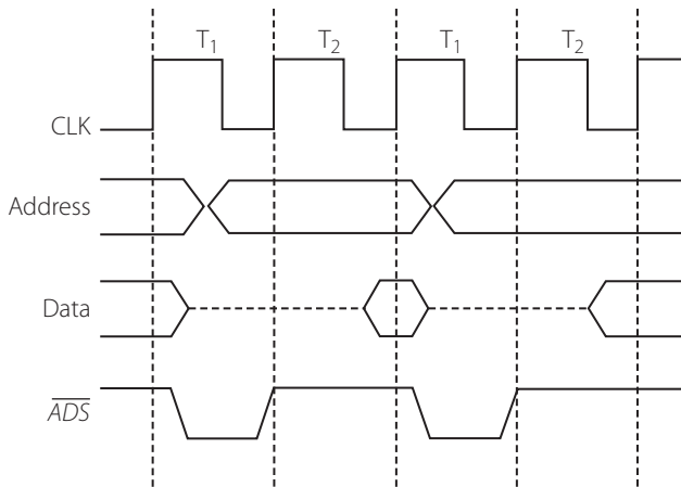
Figure 16.2 | Non-burst bus cycle
