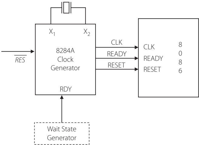
Figure 6.16 | Insertion of a wait state generator to add wait states
