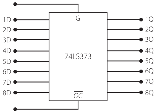
Figure 6.4 | Pin diagram of the octal latch IC 74LS373
