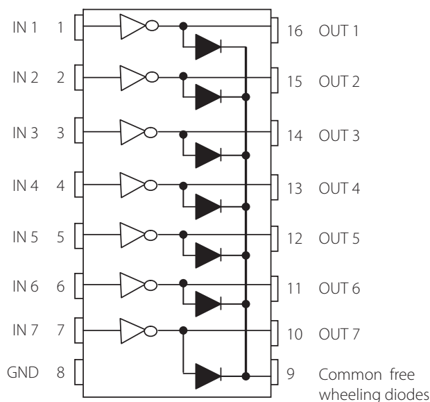
Figure 9.32 | Functional pin diagram of the driver IC ULN2003
