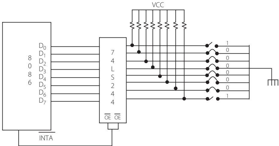
Figure 8.4 | Generation of a type number during the INTA cycle
