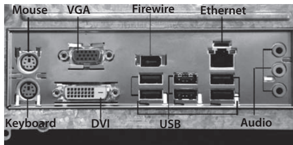
Figure 17.18 | Connectors seen at the back of a new PC
