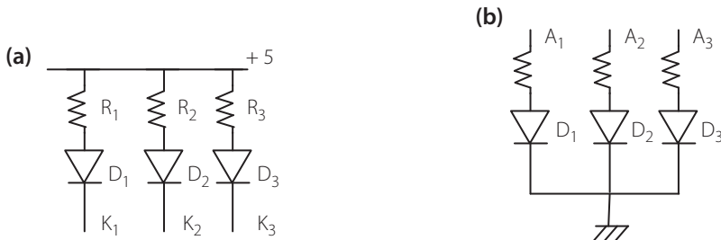
Figure 9.40 | a Common anode LEDs
