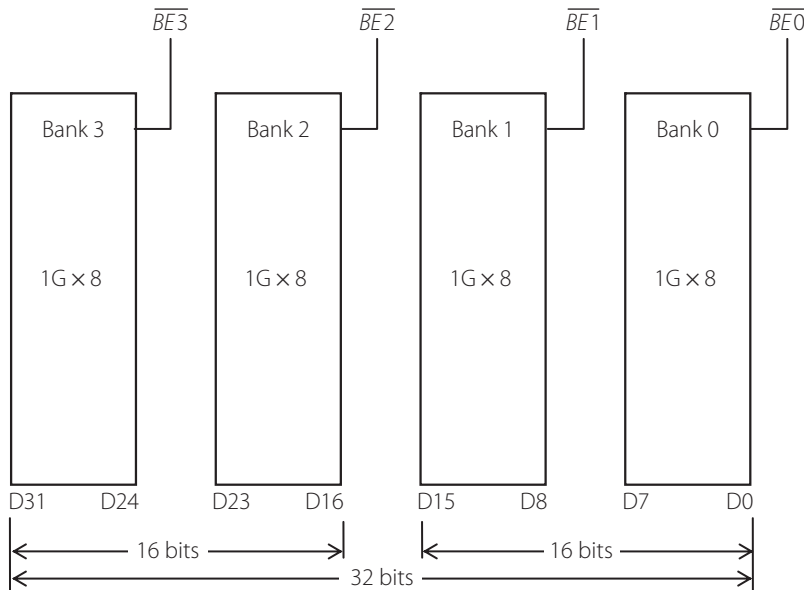
Figure 15.5 | Memory banks for the 80386
