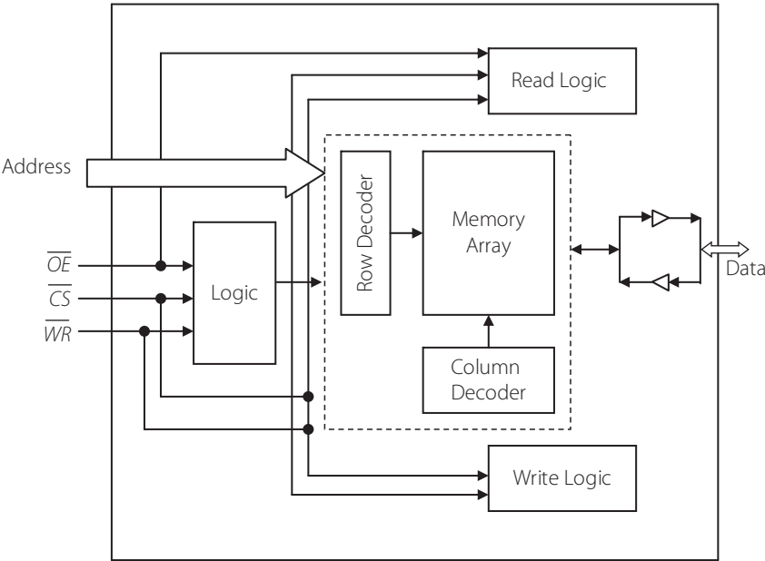
Figure 12.4 | Internal architecture of a typical SRAM chip
