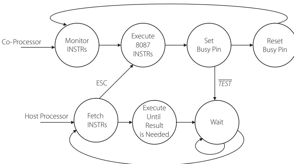
Figure 13.3 | Synchronized activities of the 8086 and the 8087
