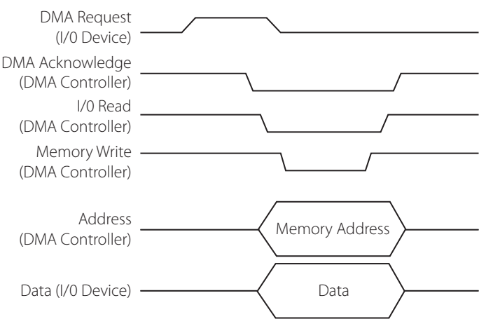
Figure 11.17 | Timing associated with flyby DMA operation (DMA write)
