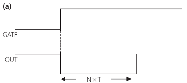
Figure 10.8a | Output waveform corresponding to mode 1
