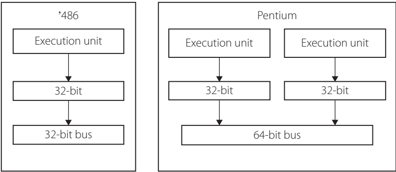
Figure 16.6 | Execution units of pentium and the '486 compared
