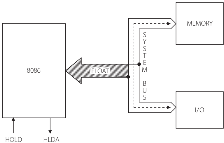
Figure 6.18 | Concept of direct memory access
