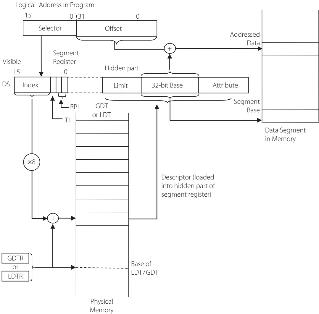
Figure 15.16 | Address translation of a logical address to a physical address
