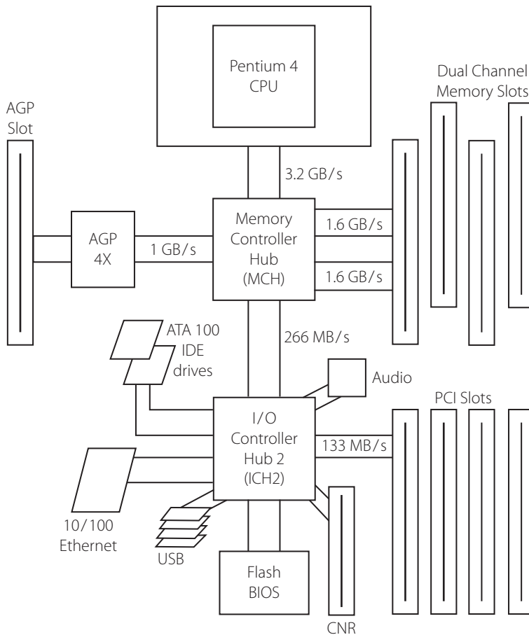
Figure 17.5 | Components of the IHA for a typical Intel motherboard (8xx series)
