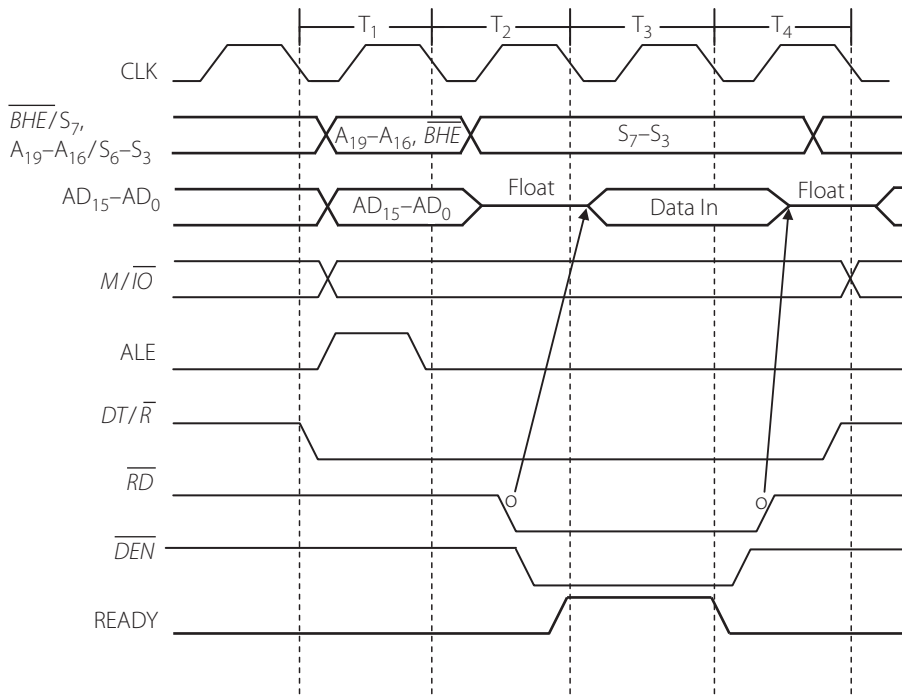
Figure 6.14 | Read machine cycle timing diagram
