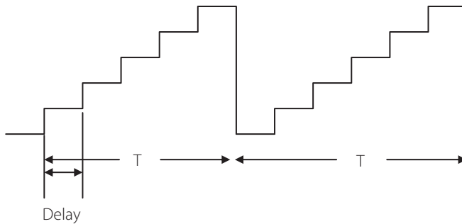
Figure 9.25 | Staircase waveform generated
