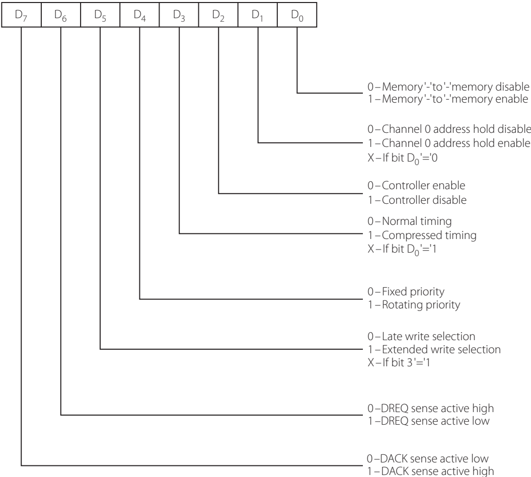
Figure 11.24 | Status of the command register
