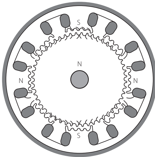
Figure 9.30 | Cross-section of a hybrid stepper motor
