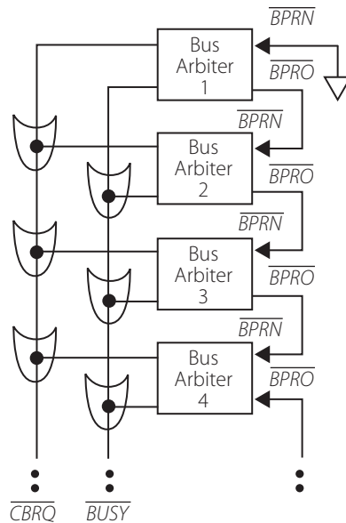
Figure 13.12 | Daisy chaining scheme using the 8289
