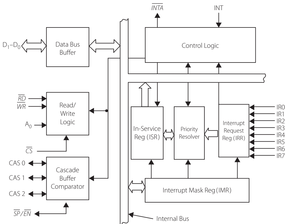
Figure 10.23 | Internal block diagram of a programmable interrupt controller (PIC)
