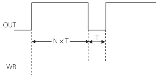
Figure 10.10 | Output waveform corresponding to mode 2 operation
