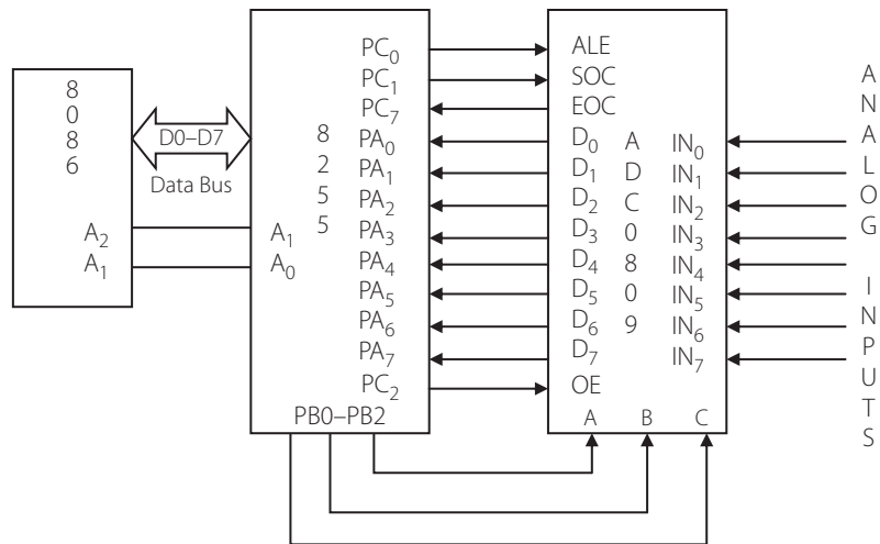
Figure 9.22 | ADC with its control and data pins connected to an 8086
