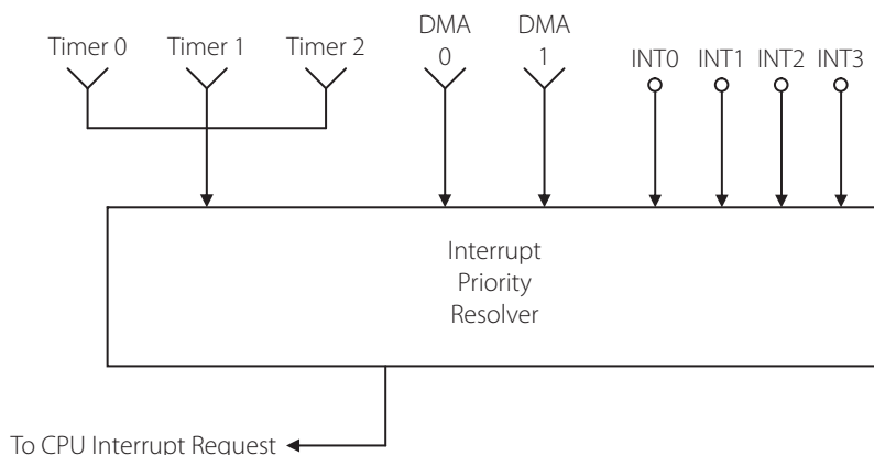
Figure 14.4 | Interrupt control unit in master mode
