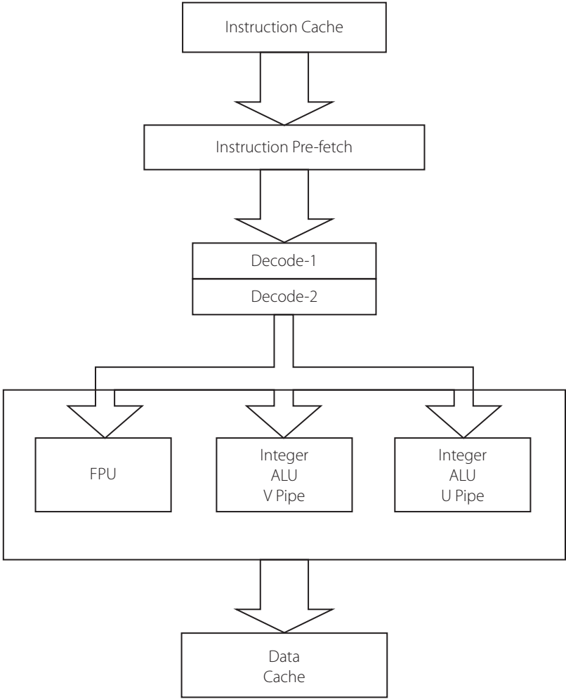
Figure 16.7 | Execution unit of Pentium
