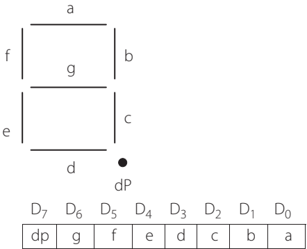
Figure 9.43 | Segments of the display and the data byte
