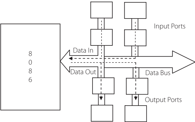
Figure 7.15 | Input and output ports connected to the 8086
