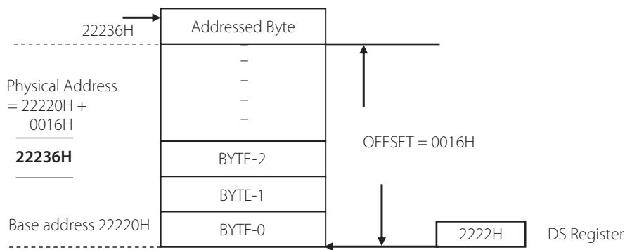
Figure 1.4 | Calculation of a physical address from the logical address for a data segment
