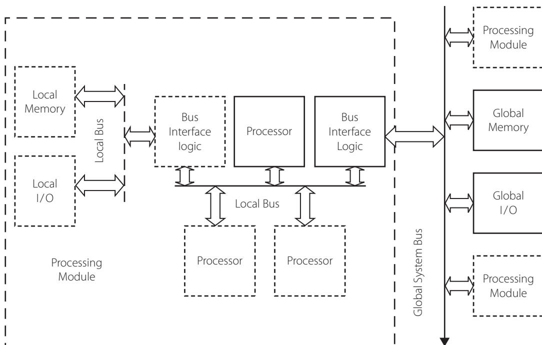
Figure 13.2 | Loosely coupled multiprocessor system
