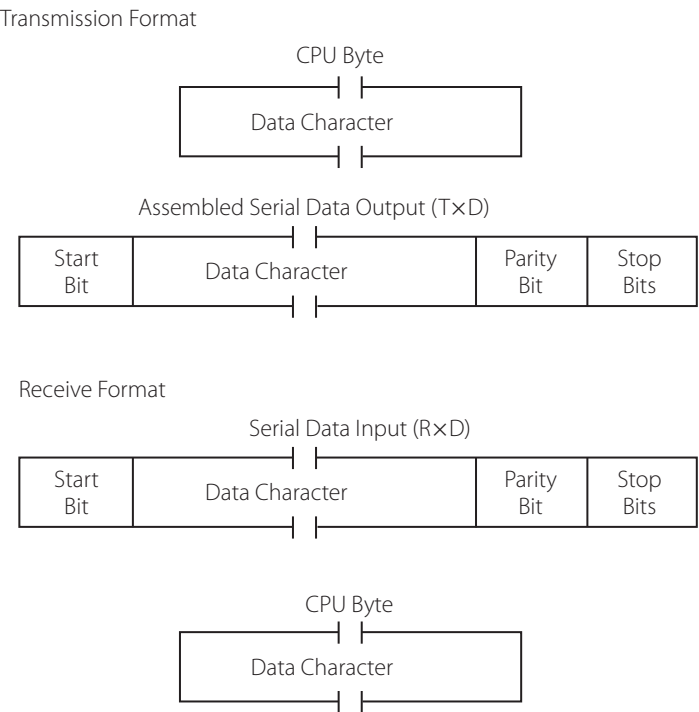
Figure 11.13 | Transmission and reception formats
