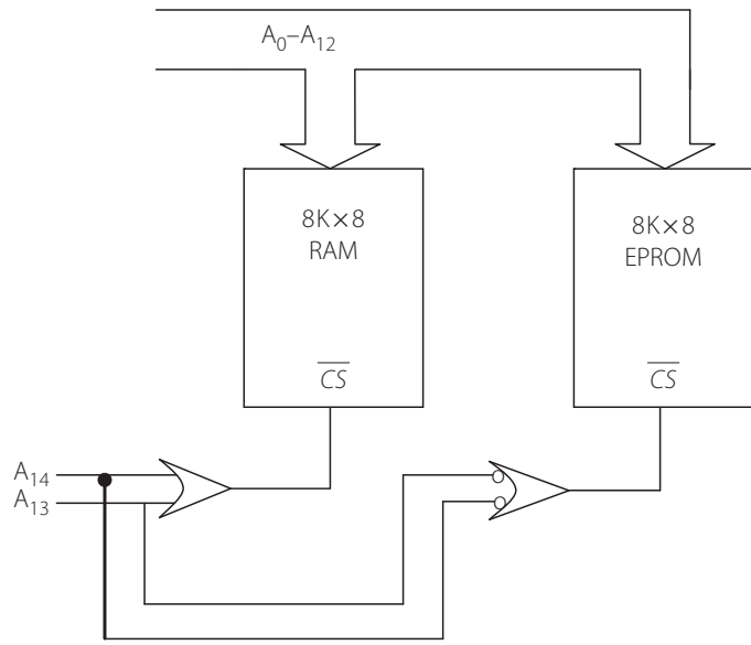
Figure 7.10 | Partial address decoding using two address lines
