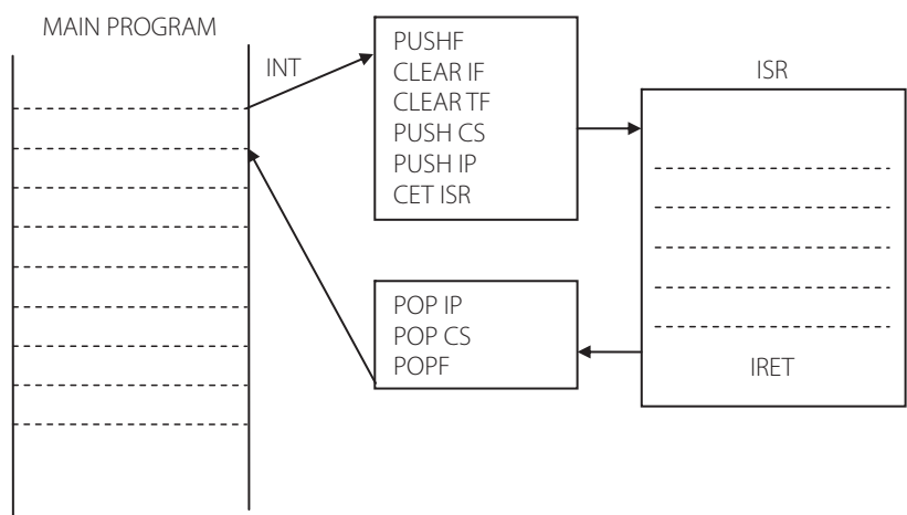
Figure 8.1 | Steps in processing an interrupt request
