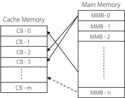
Figure 12.14 | Fully associative mapping
