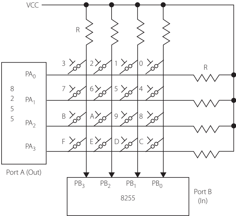
Figure 9.38 | Hex keyboard connected to an 8255
