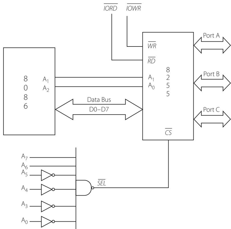
Figure 9.5 | Address decoding and connections between the 8086 and the 8255
