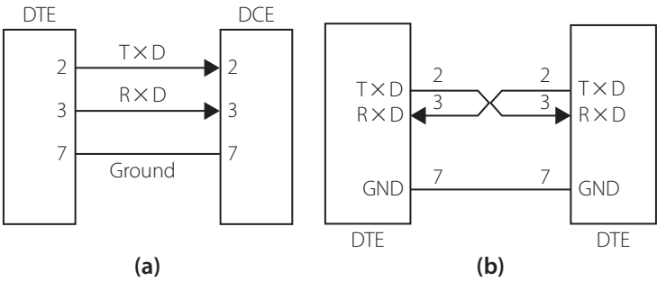
Figure 11.8a | DTE–DCE connection using 3 pins b DTE–DTE connection with a null modem
