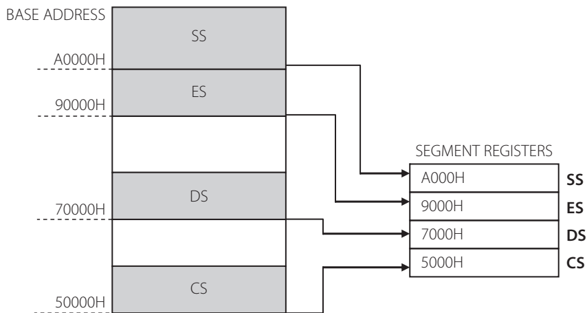
Figure 1.5 | Segment registers and corresponding segments
