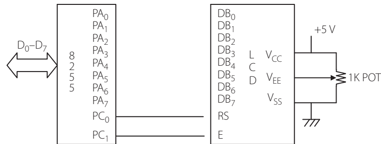
Figure 9.27 | The LCD connected to the 8255
