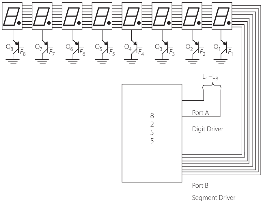
Figure 9.44 | Eight digit dynamic display with segment and digit drivers
