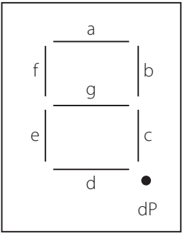
Figure 10.15 | Correspondance between the segments and the data bus lines
