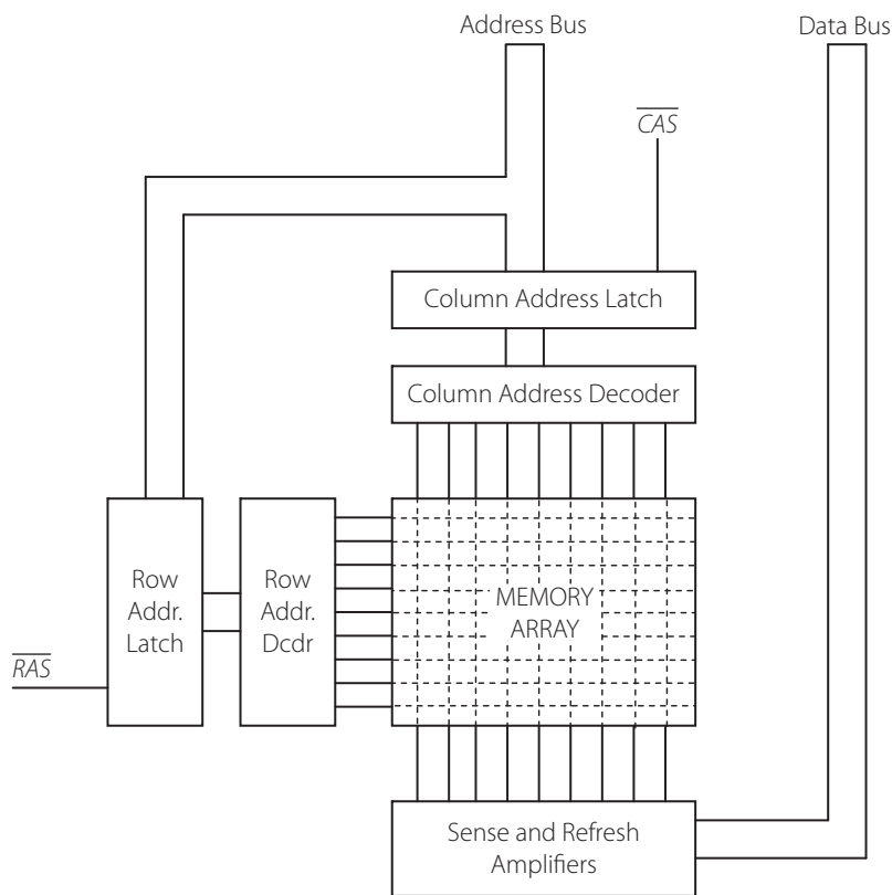
Figure 12.7 | Internal architecture of a DRAM chip
