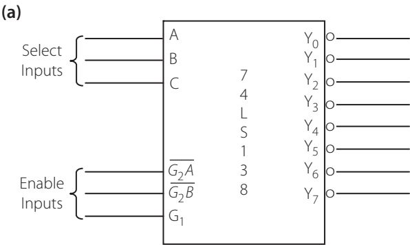
Figure 7.6a | Functional block diagram of the 3 to 8 decoder 74LS138
