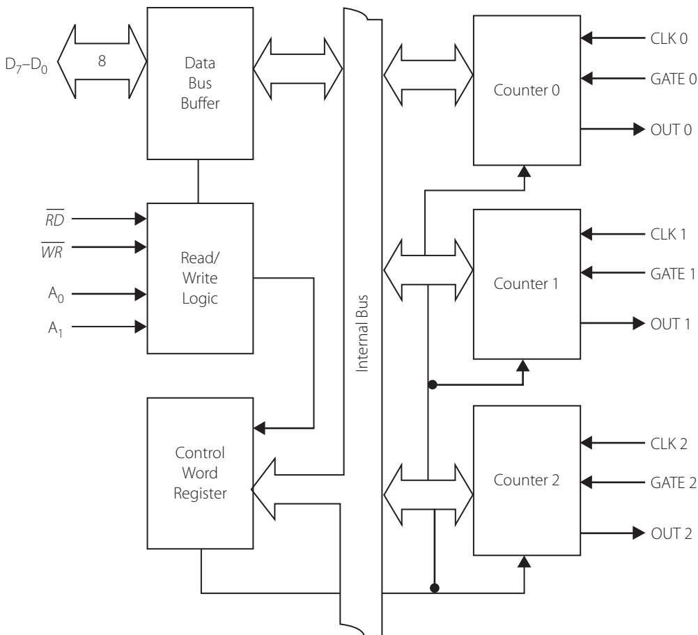
Figure 10.2 | Functional block diagram of 8253/8254
