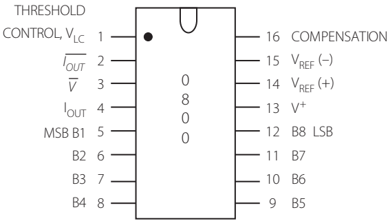
Figure 9.23 | Pin diagram of the DAC 0800
