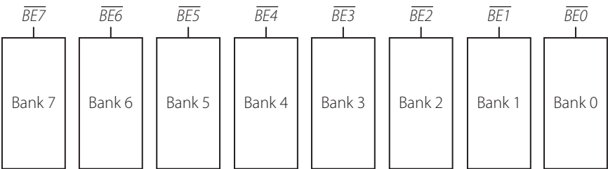
Figure 16.5 | Memory banks of Pentium
