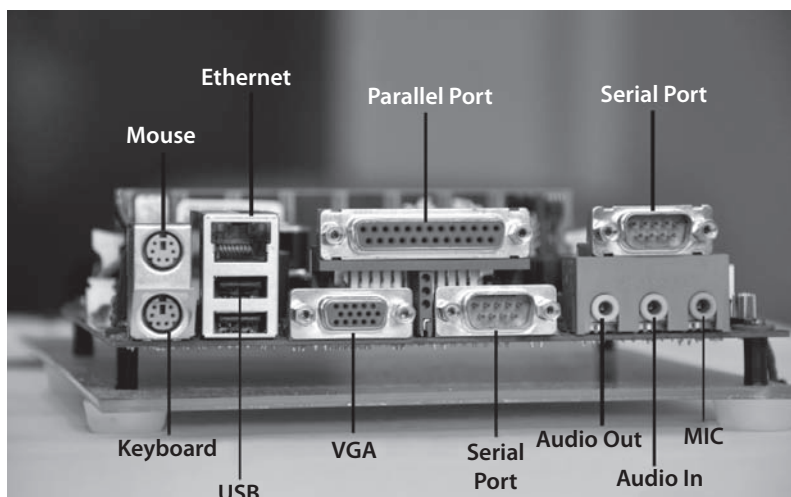
Figure 17.2 | Connectors of the motherboard, accessible outside the PC
