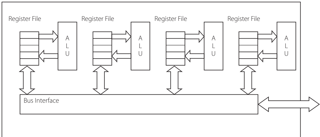
Figure 16.8 | b A multi core microprocessor
