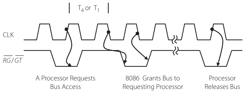
Figure 6.24 | Timing associated with the \overline{RQ}/\overline{GT} pin
