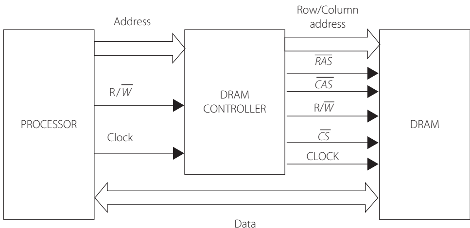
Figure 12.6 | Memory controller for a DRAM
