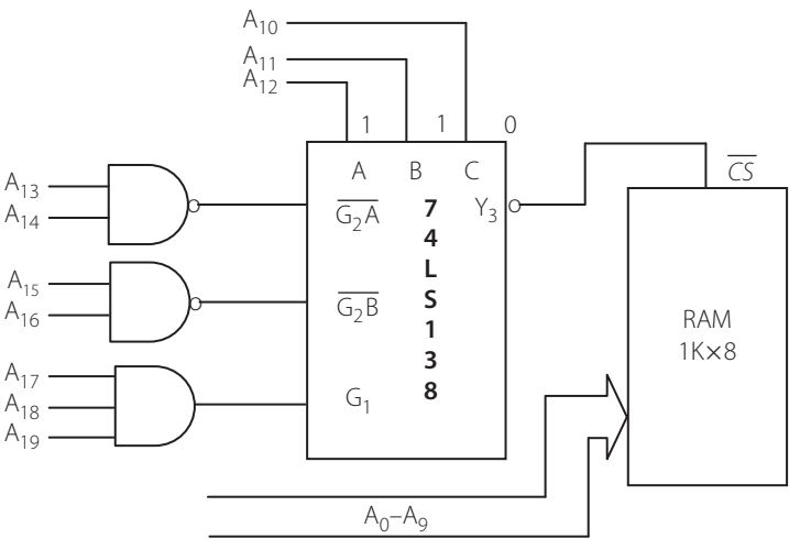
Figure 7.7 | Address decoding of a RAM using a block decoder
