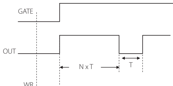
Figure 10.12 | Output waveform for mode 5, starting from the L to H transition of the GATE
