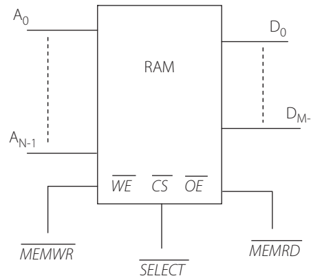
Figure 12.1 | Pins of a typical SRAM chip
