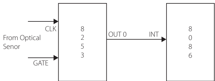
Figure 10.7 | An example of a practical application of mode 0
