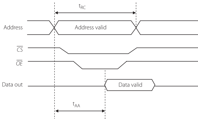
Figure 12.2 | Read cycle of a typical SRAM
