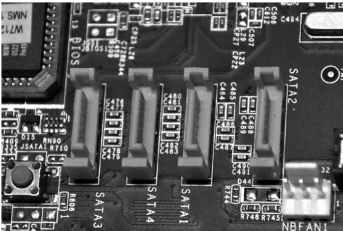
Figure 17.12 | Four SATA connectors on a motherboard
