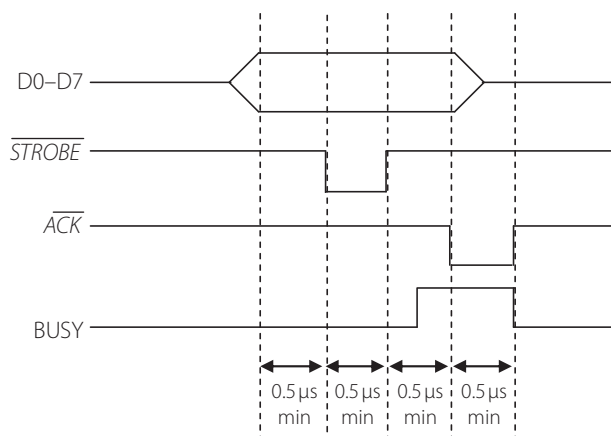
Figure 9.18 | Timing diagram of the Centronics interface
