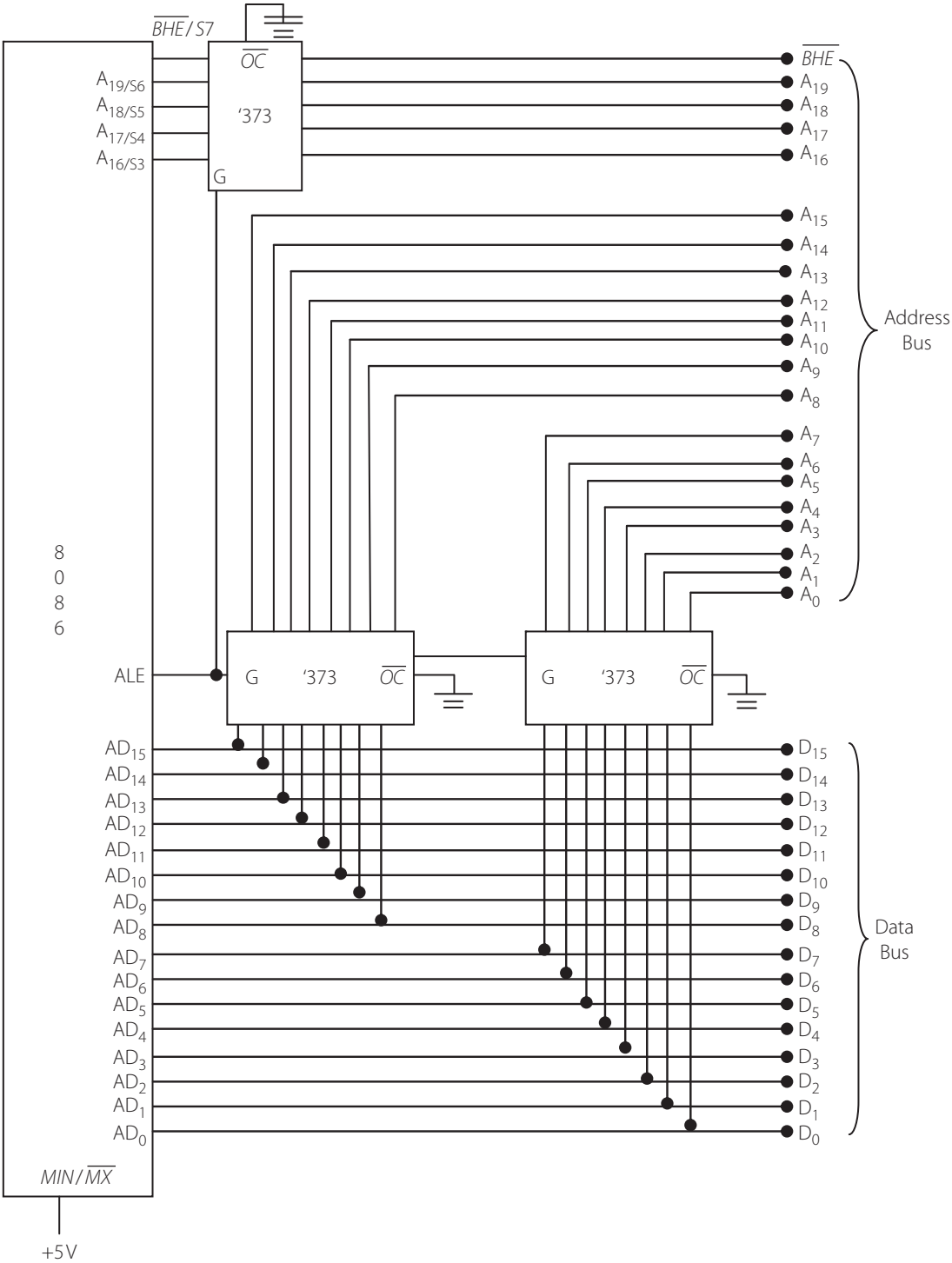
Figure 6.5 | The buffered and de-multiplexed address bus
