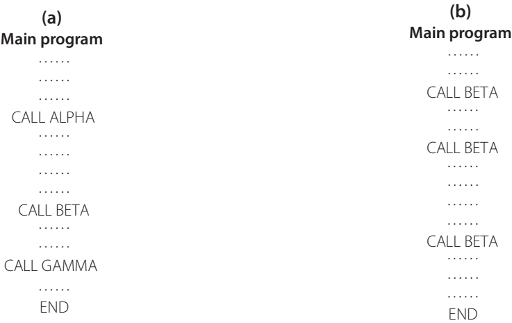
Figure 4.1 | a Main program calling different procedures b Main program calling the same procedure repeatedly
