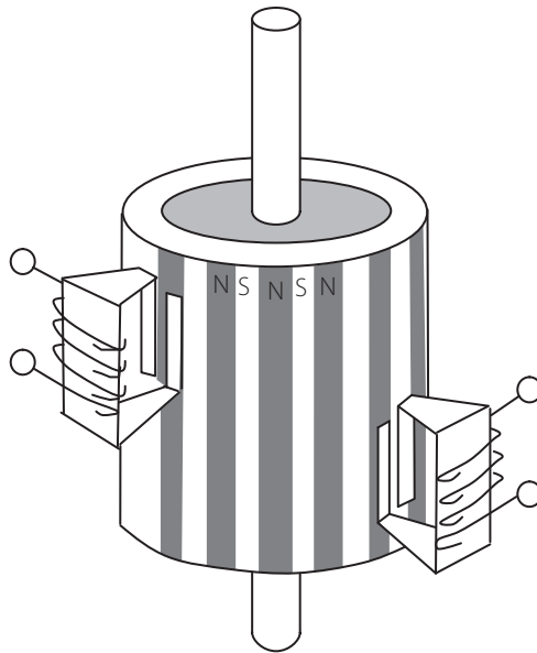
Figure 9.29 | A permanent magnet stepper motor
