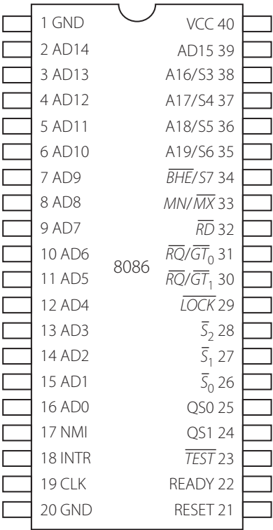
Figure 6.21 | Maximum mode pins of 8086
