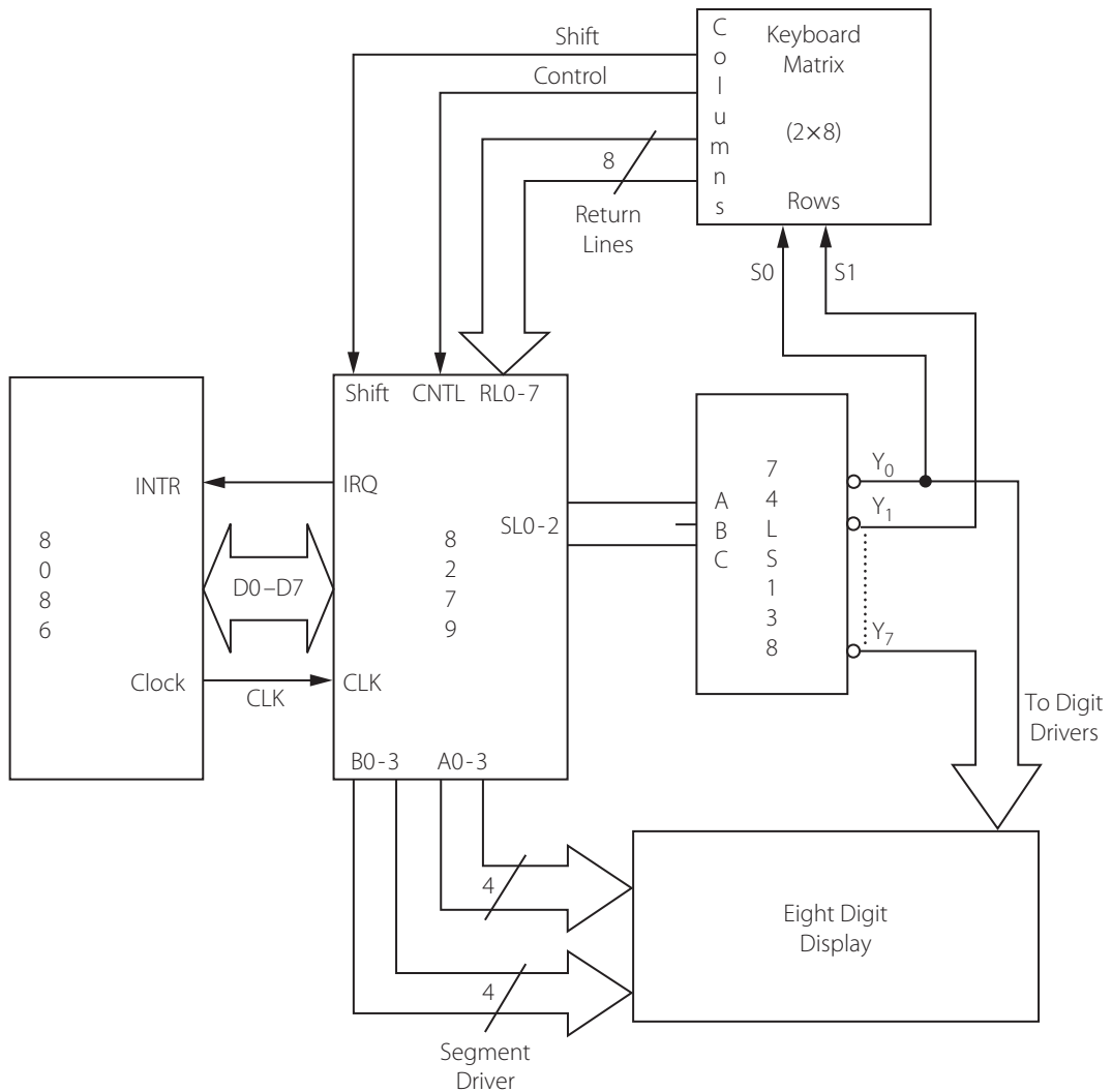
Figure 10.18 | Connections between the 8279, an 8 digit display and a 2 × 8 keyboard
