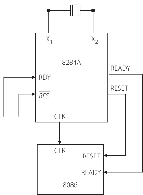
Figure 6.10 | Connections of the clock generator IC to 8086
