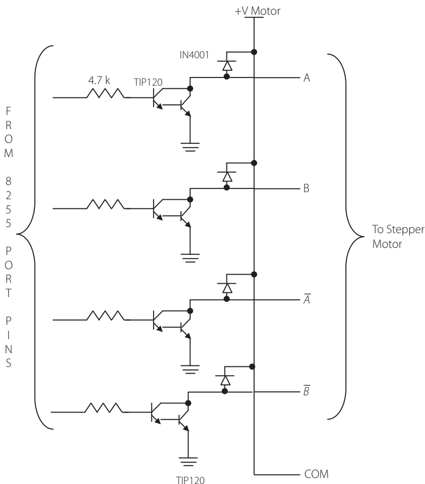
Figure 9.34 | Current driver Darlington transistors and back EMF suppressing diodes in a stepper circuit
