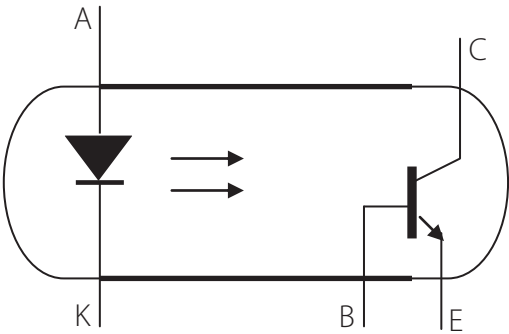
Figure 9.35 | Principle of operation of an optocoupler
