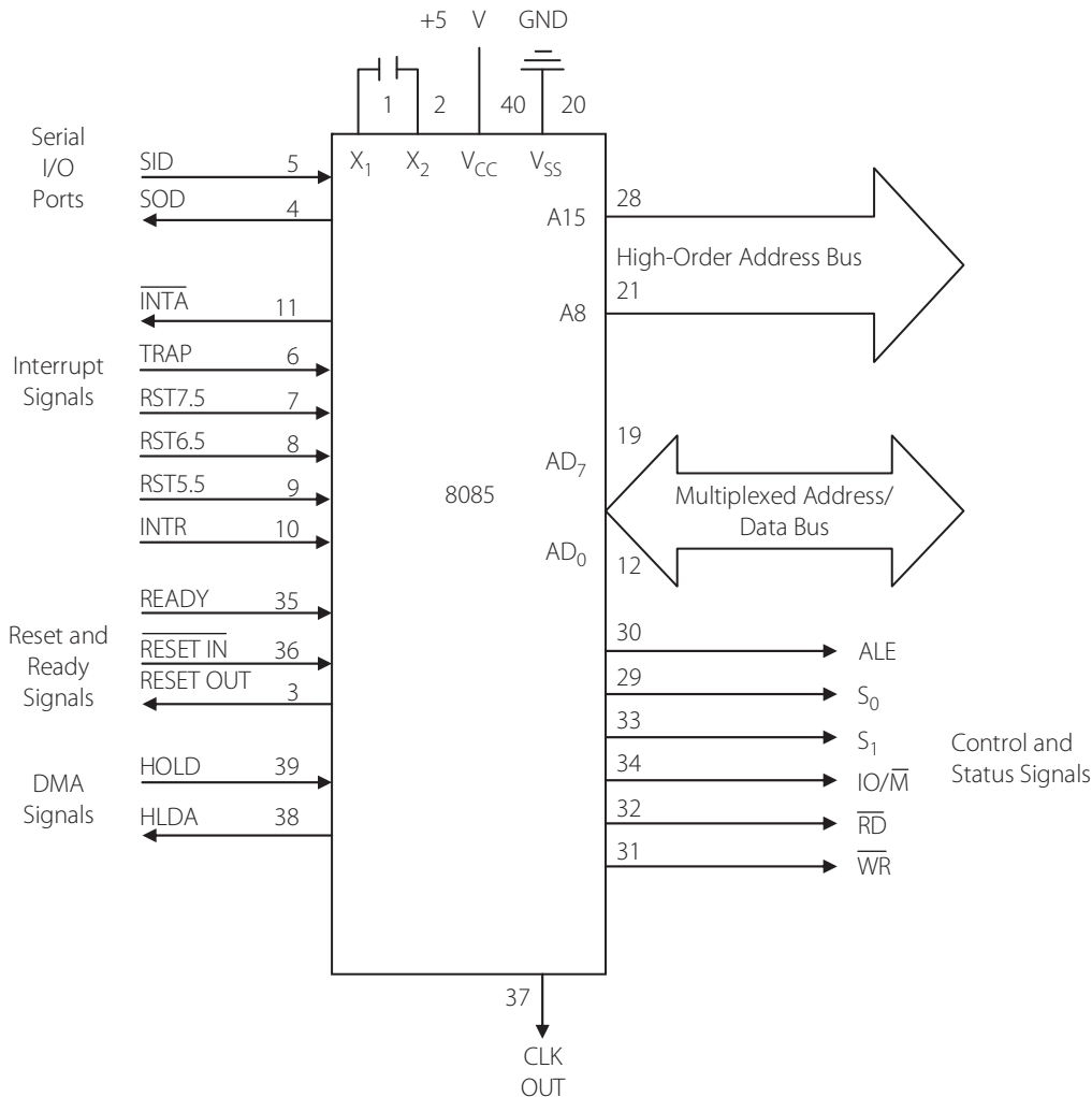
Figure 0.17 | Functional block diagram of 8085
