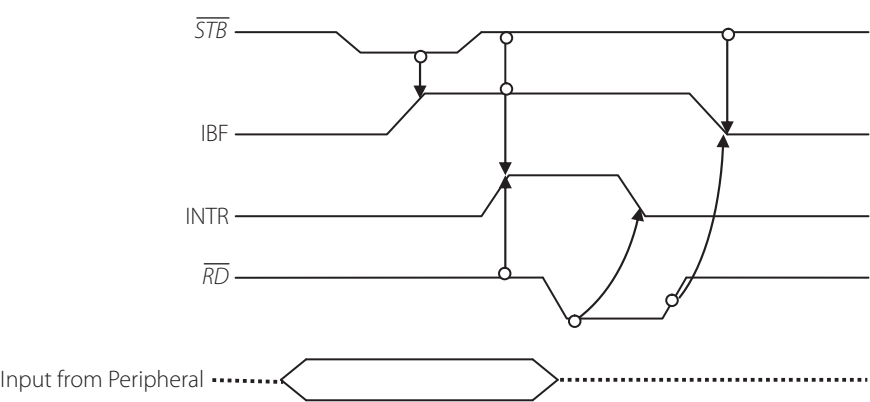
Figure 9.11 | Timing waveforms for strobed input mode
