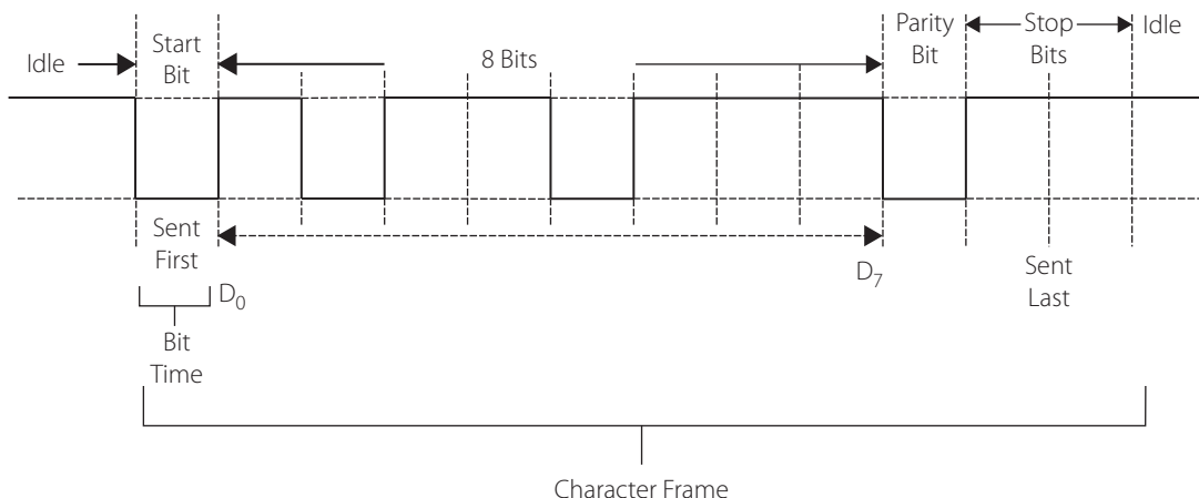
Figure 11.1 | A typical asynchronous character frame
