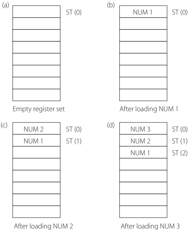
Figure 13.16 | Using the general-purpose registers for loading NUM1, NUM2 and NUM3
