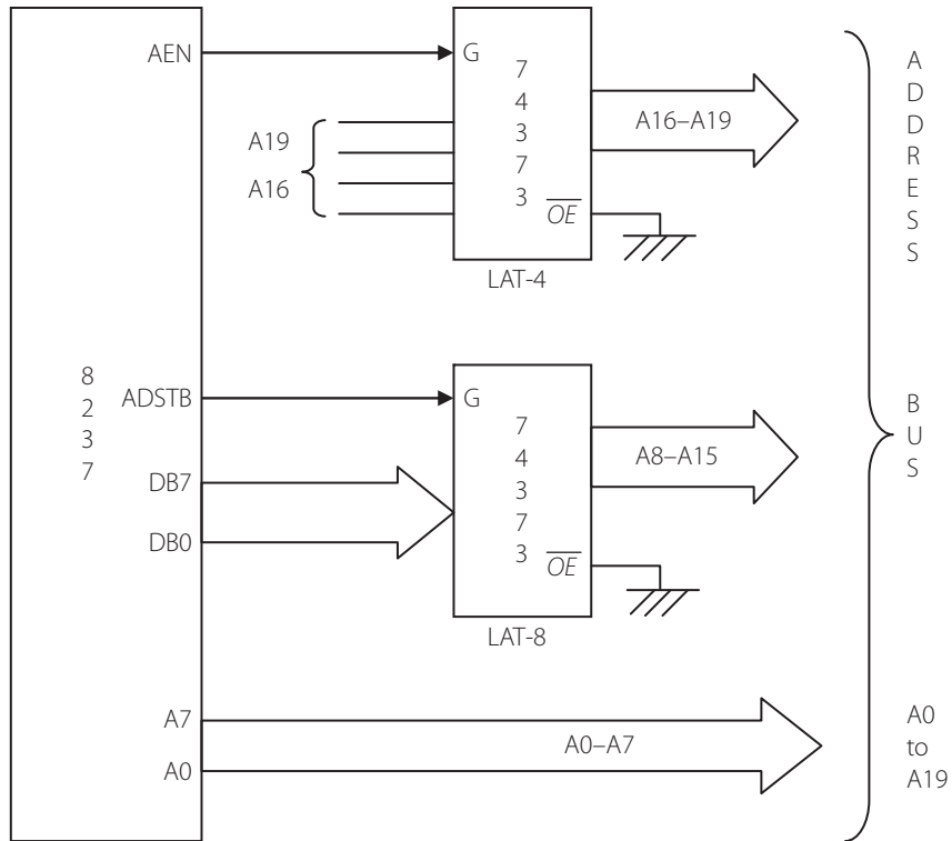
Figure 11.23 | Address generation for DMA operation
