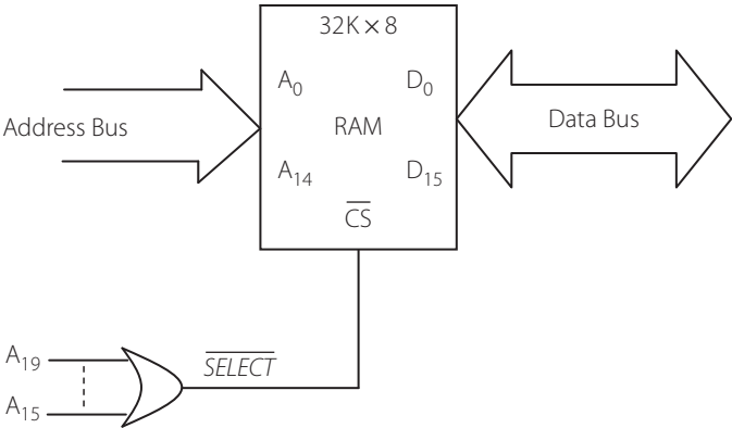
Figure 7.4 | Address decoding using OR logic
