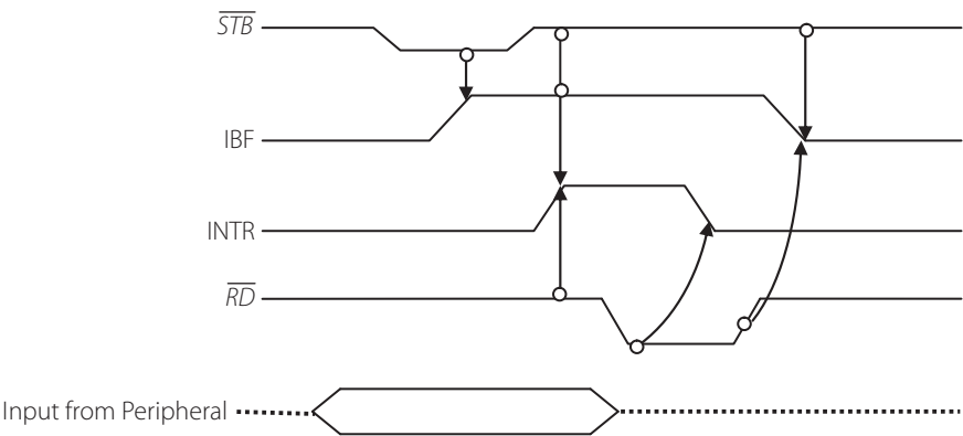
Figure 9.11 | Timing waveforms for strobed input mode
