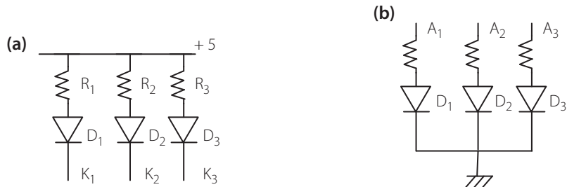
Figure 9.40 | a Common anode LEDs
