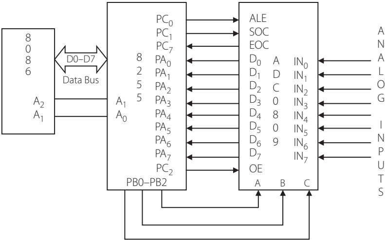
Figure 9.22 | ADC with its control and data pins connected to an 8086
