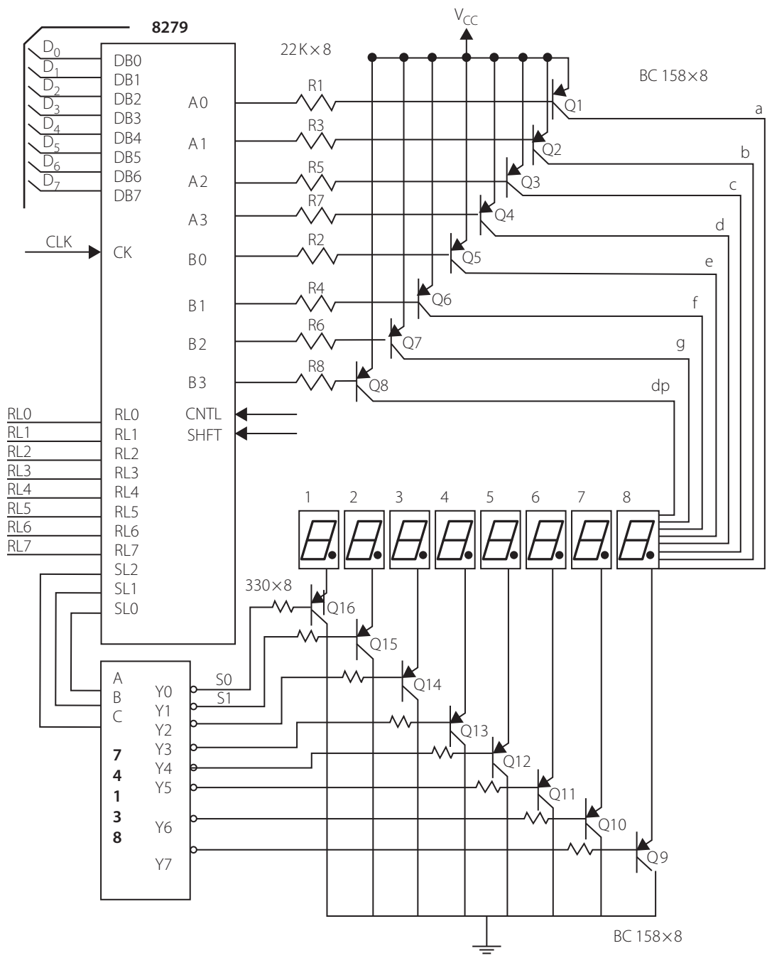
Figure 10.14 | Display interface part of the 8279
