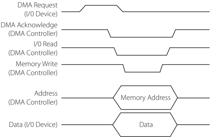
Figure 11.17 | Timing associated with flyby DMA operation (DMA write)
