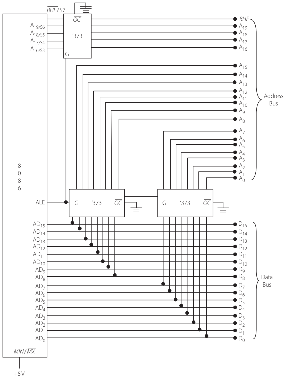
Figure 6.5 | The buffered and de-multiplexed address bus
