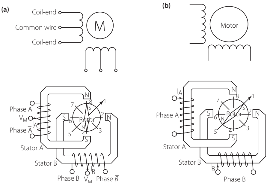
Figure 9.31 | a Unipolar motor b Bipolar motor
