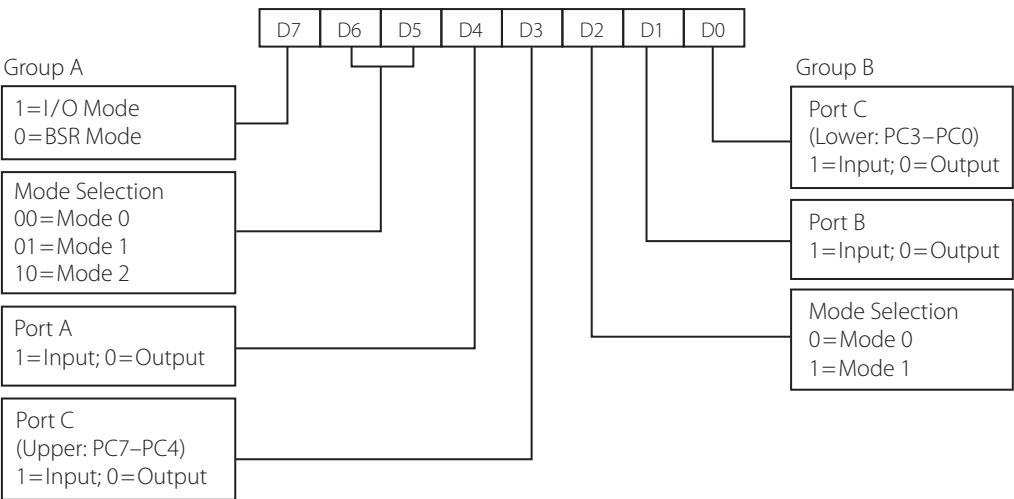
Figure 9.6 | Control word format of 8255
