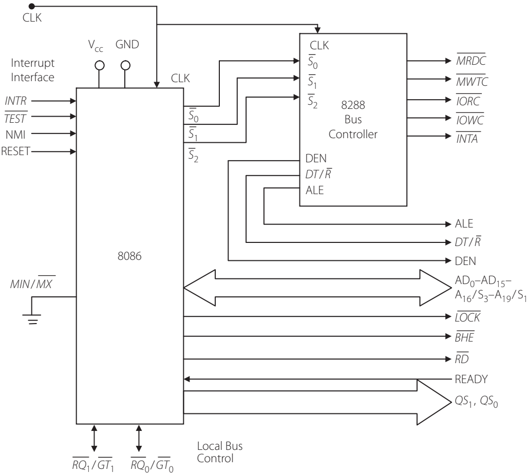
Figure 6.25 | Maximum mode configuration of the 8086
