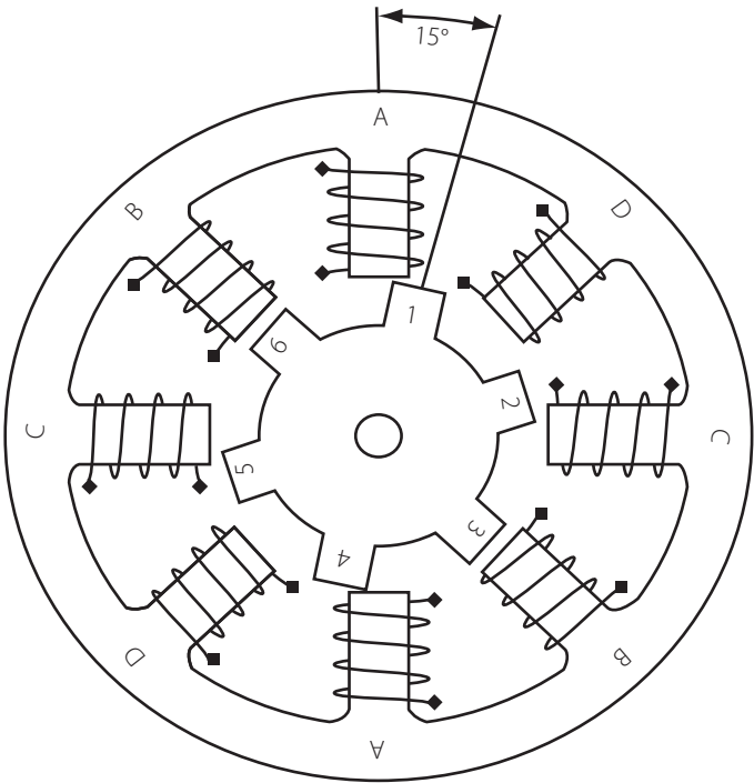
Figure 9.28 | Cross-section of a variable reluctance (VR) motor
