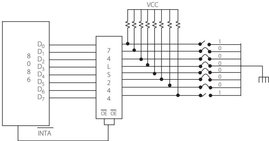
Figure 8.4 | Generation of a type number during the \text{INTA} cycle
