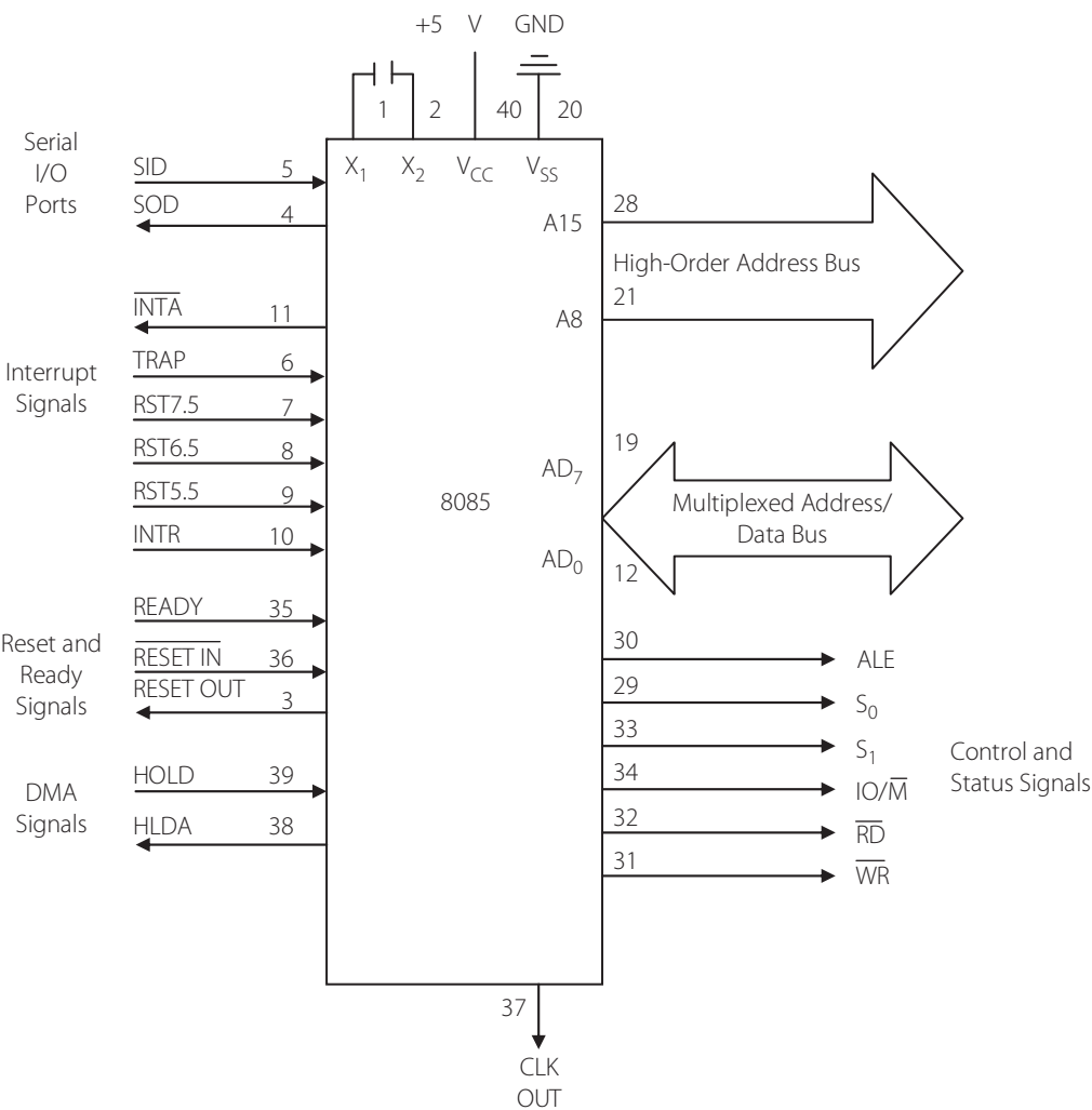
Figure 0.17 | Functional block diagram of 8085
