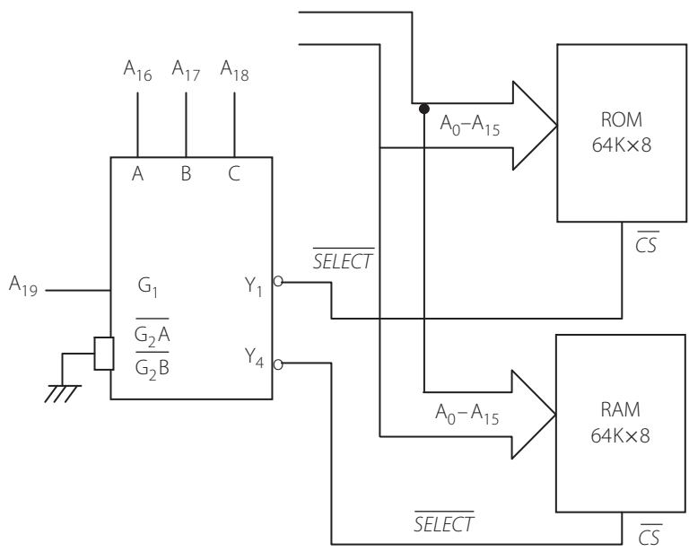
Figure 7.8 | Address decoding of a RAM and ROM using a 3 to 8 decoder
