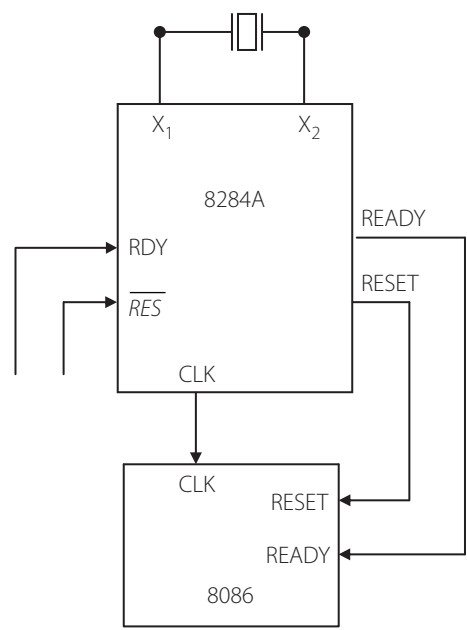
Figure 6.10 | Connections of the clock generator IC to 8086
