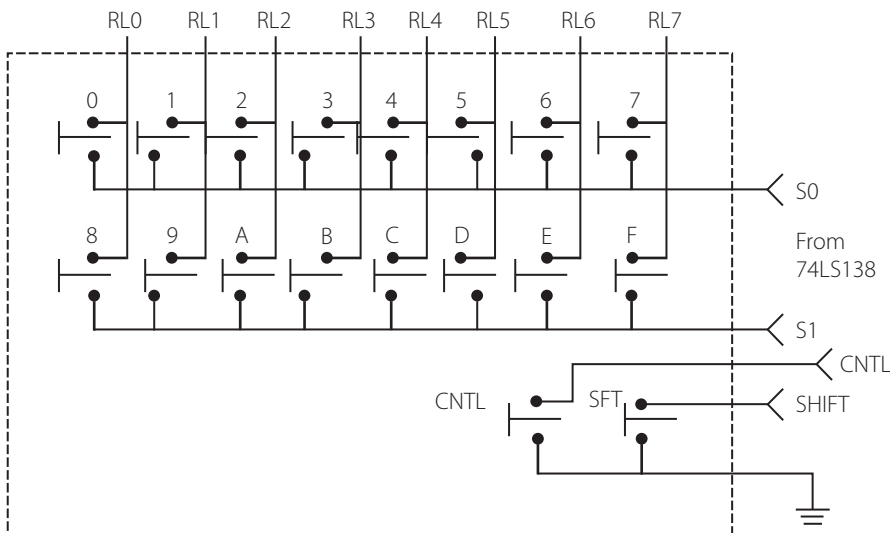
Figure 10.16 | Keyboard section
