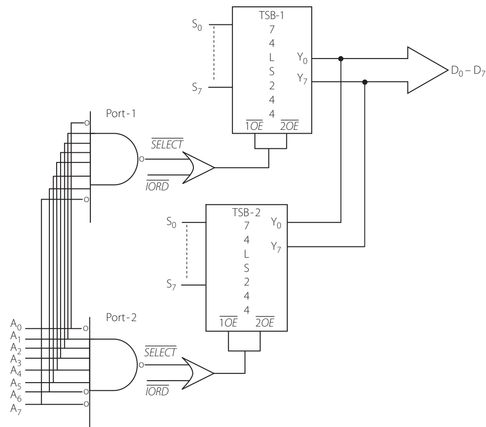
Figure 7.21 | Two sets of switches acting as two 8-bit input ports
