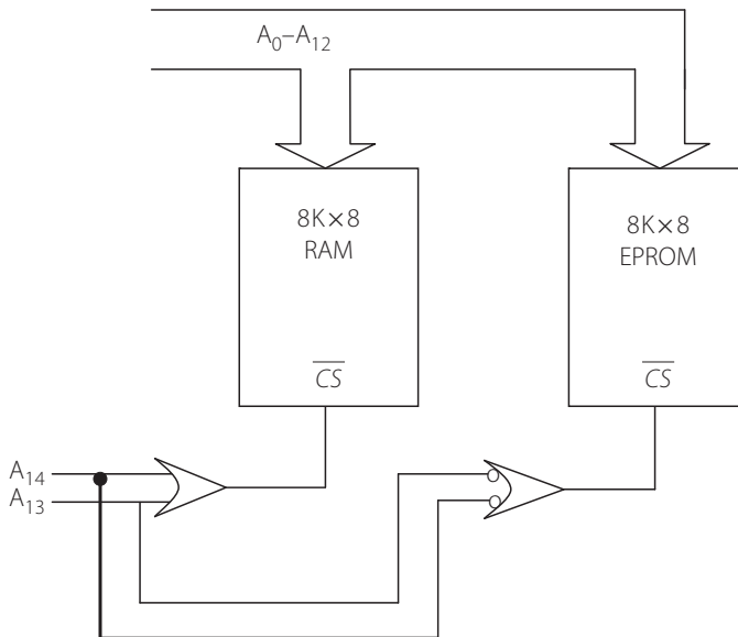
Figure 7.10 | Partial address decoding using two address lines
