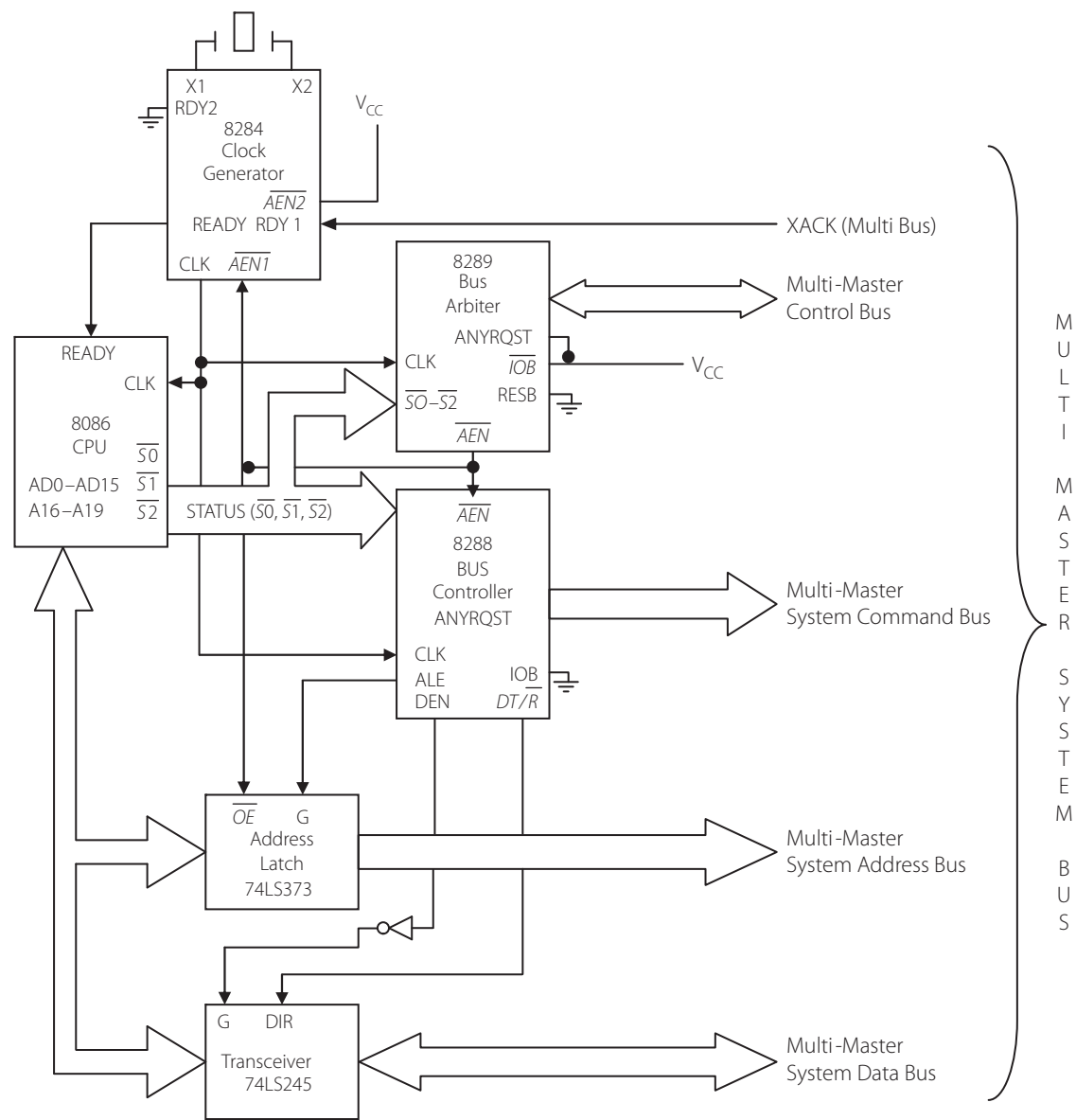
Figure 13.9 | One processing module in a loosely coupled system, shown with the bus arbiter
