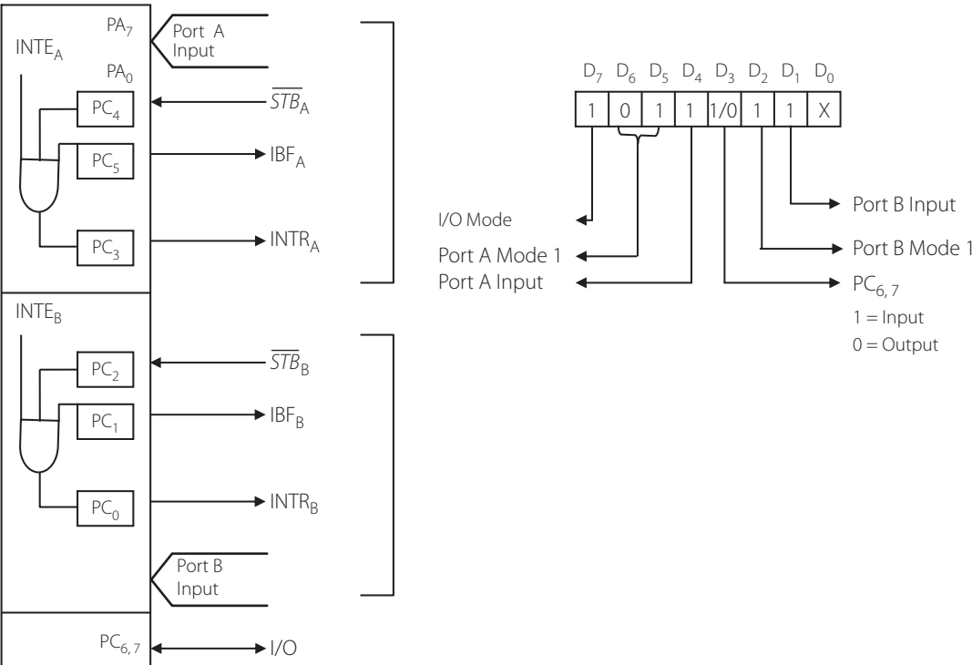
Figure 9.10 | Mode 1: Strobed input – Pin configuration and control word format
