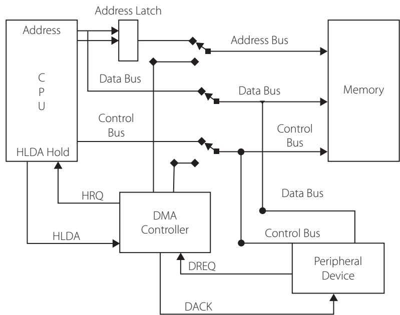
Figure 11.19 | DMA concept
