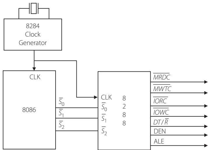
Figure 6.23 | Connection between the 8086 and 8288
