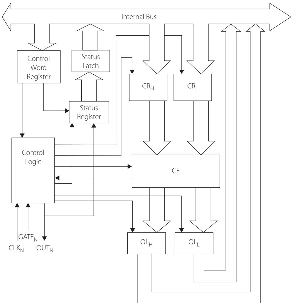
Figure 10.3 | Internal architecture of a counter
