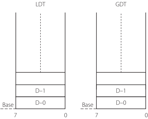
Figure 15.12 | LDT of a task and the GDT of the system
