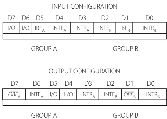
Figure 9.14 | Status of Port C for input and output configurations of Mode 1
