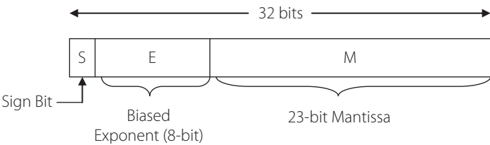
Figure 13.13 | Single precision representation
