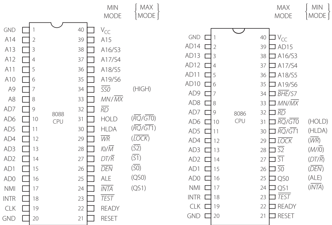
Figure 6.1a | 8088 CPU pin diagram b 8086 CPU pin diagram
