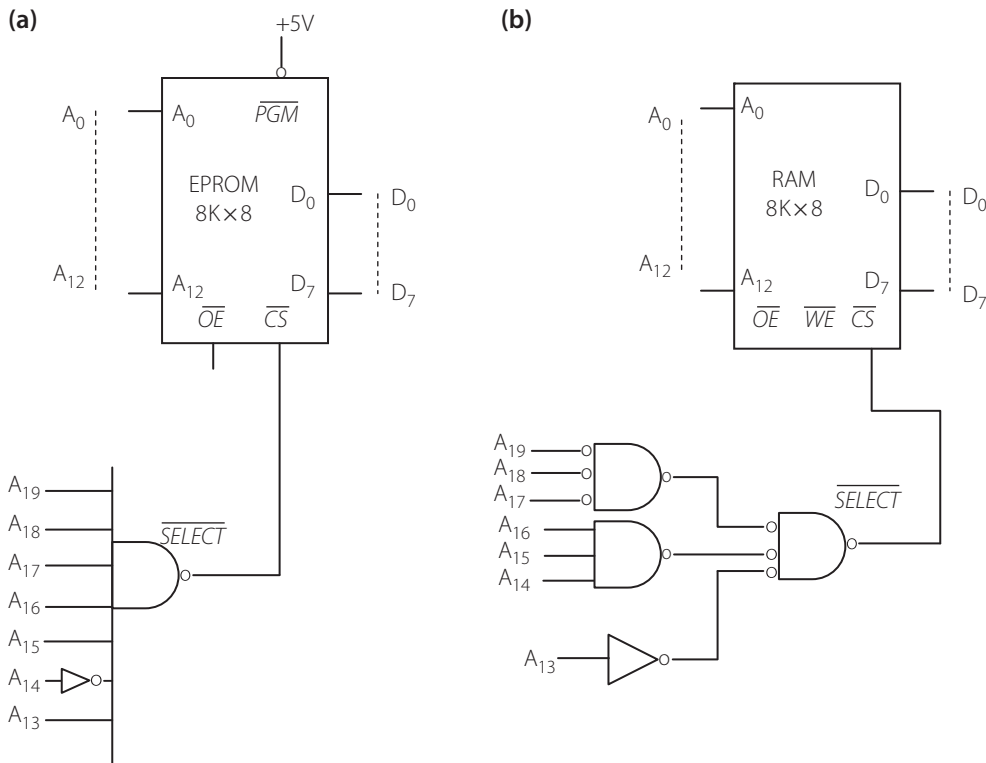
Figure 7.5a | EPROM with address decoder b RAM with address decoder
