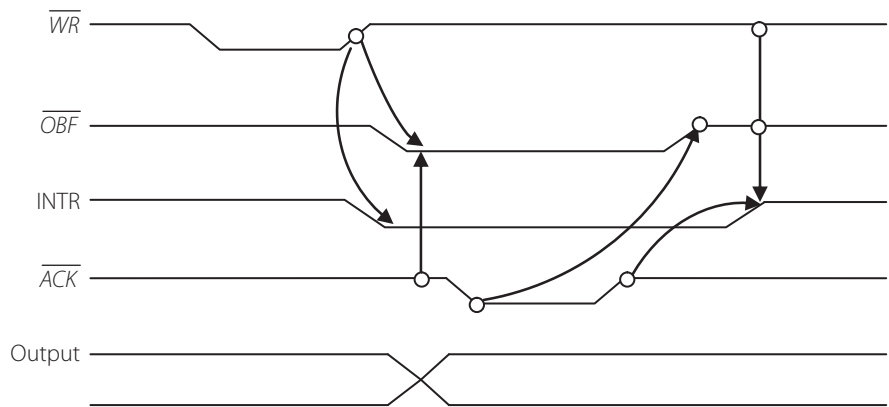
Figure 9.13 | Timing waveform for strobed output mode
