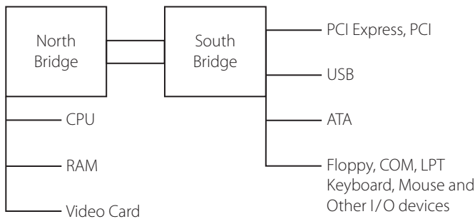
Figure 17.3 | The north bridge and the south bridge
