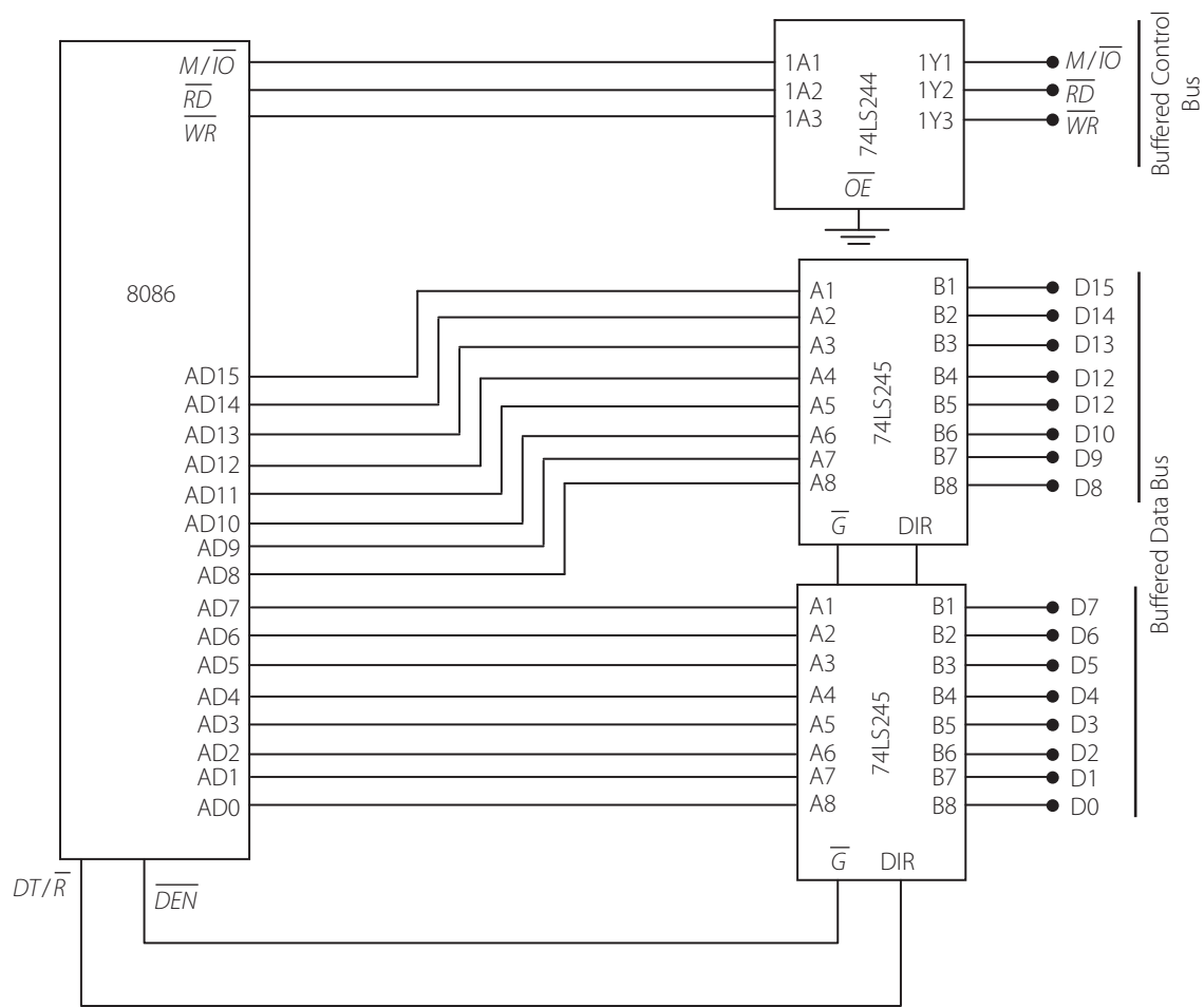
Figure 6.7 | Buffered data bus and control pins
