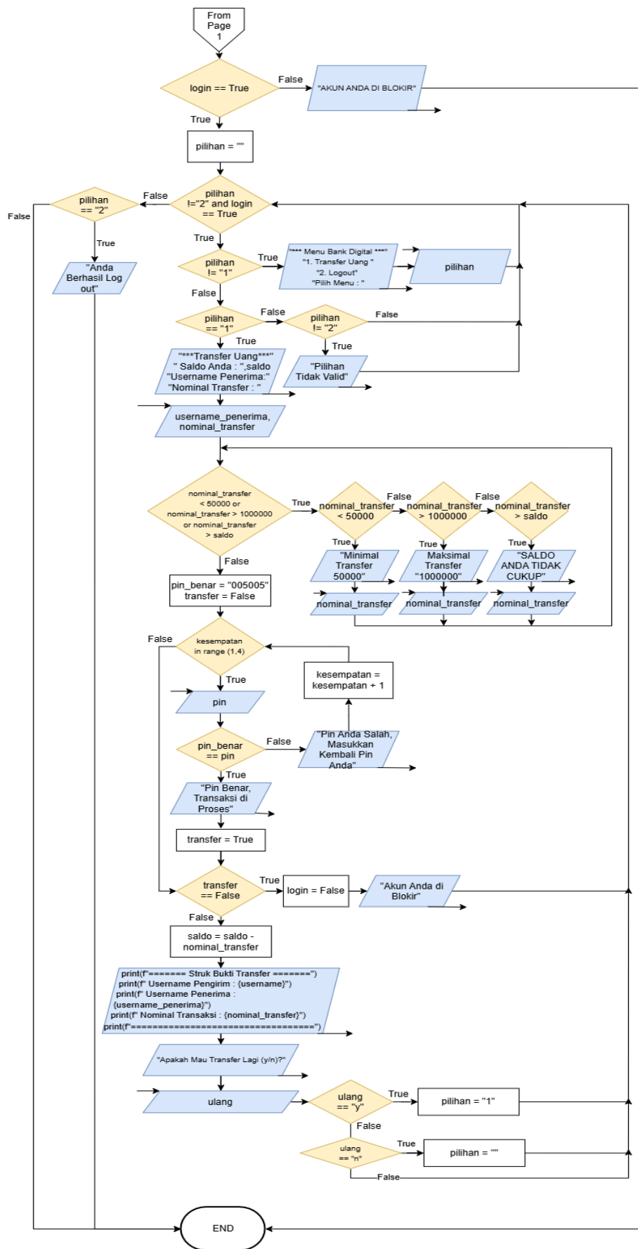
Gambar 1.2 Flowchart Program Page 2
