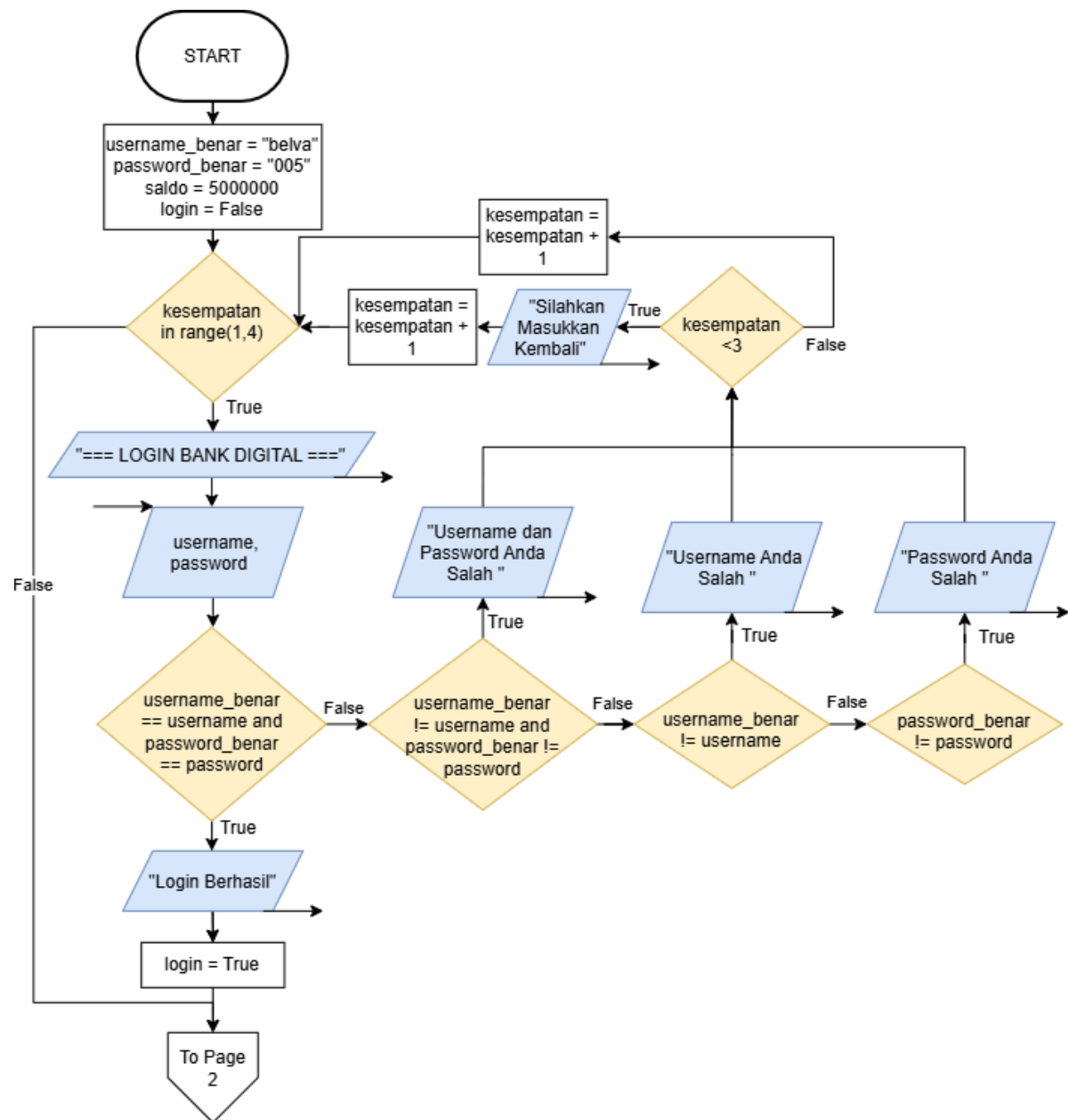
Gambar 1.1 Flowchart Program Page 1
