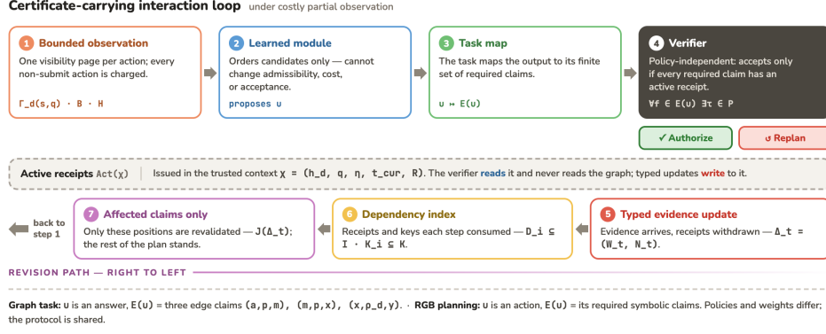
Figure 1: Certificate-carrying interaction loop. Graph and RGB tasks share receipt-backed authorization and dependency-indexed revision, but not policies or task semantics.
