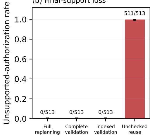
(b) Final-support loss
