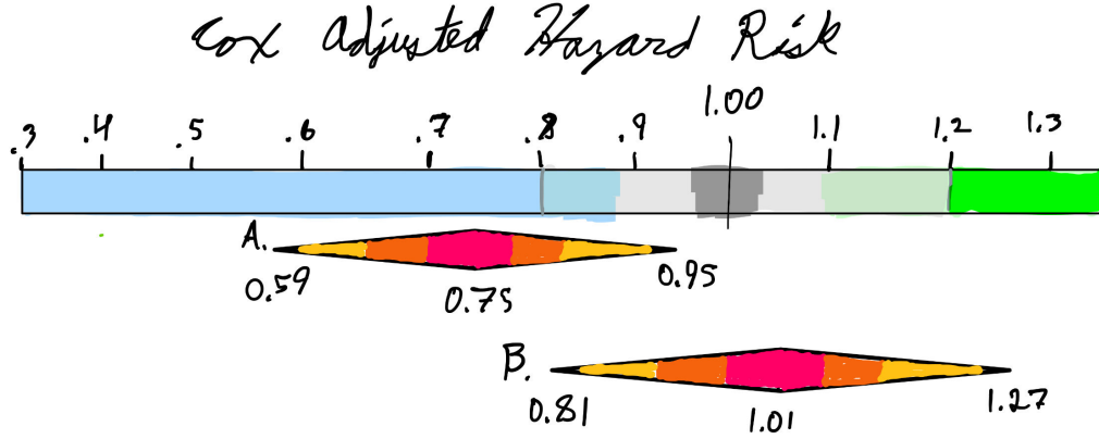
Figure 4: Quantitative backdrop for visualizing the confidence intervals for the adjusted Cox hazard risk model for predicting the likelihood of being diagnosed with AD RD after completing the speed intervention arm with a booster (interval A) and without a booster (interval B) relative to the likelihood of being diagnosed with AD RD with no cognitive intervention after a 20-year long follow-up.
