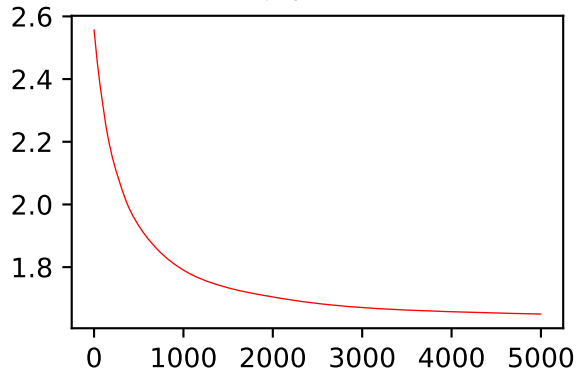
\theta dim 3
