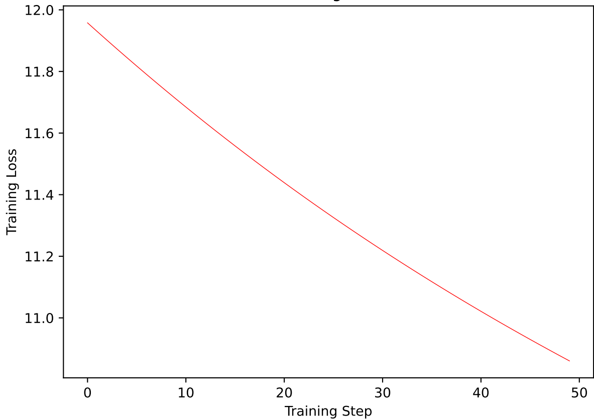
Training loss
