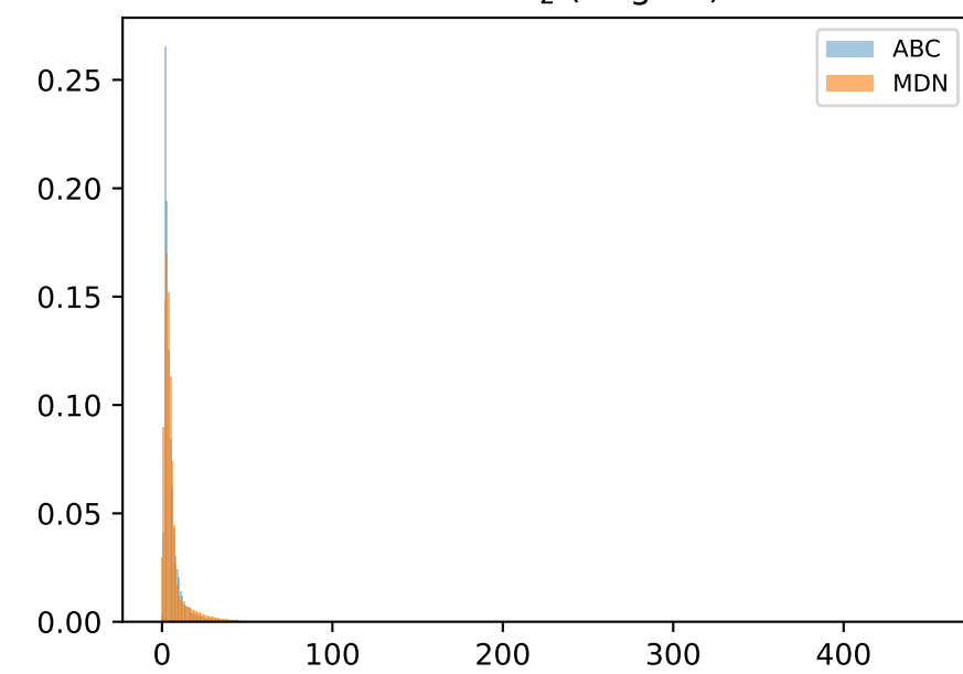
x=0.21 \theta_2 (NegBin)
