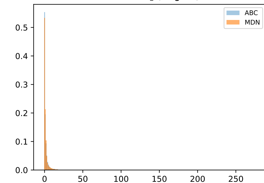
x=0.93 \theta_2 (NegBin)
