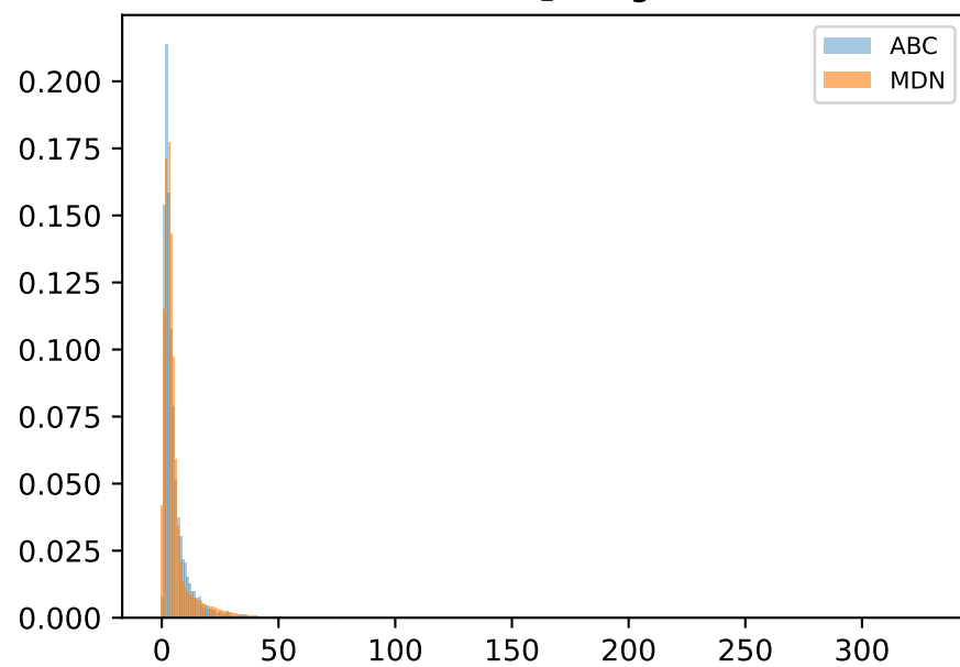
x=-0.73 \theta_2 (NegBin)
