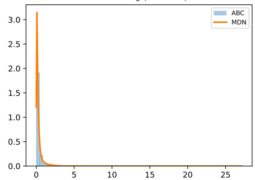
x=0.21 \theta_3 (Gamma)
