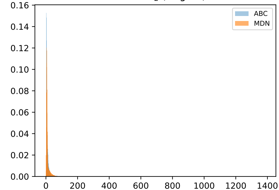
x=0.21 \theta_2 (NegBin)
