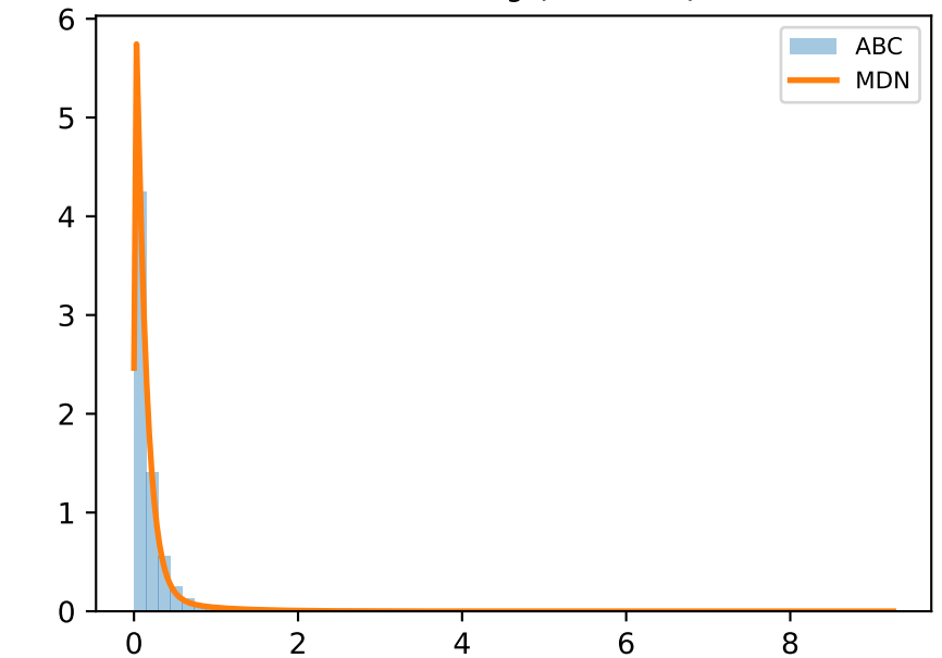
x=0.93 \theta_3 (Gamma)
