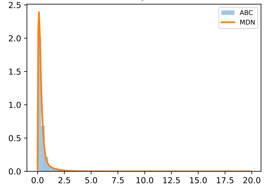
x=-0.73 \theta_3 (Gamma)
