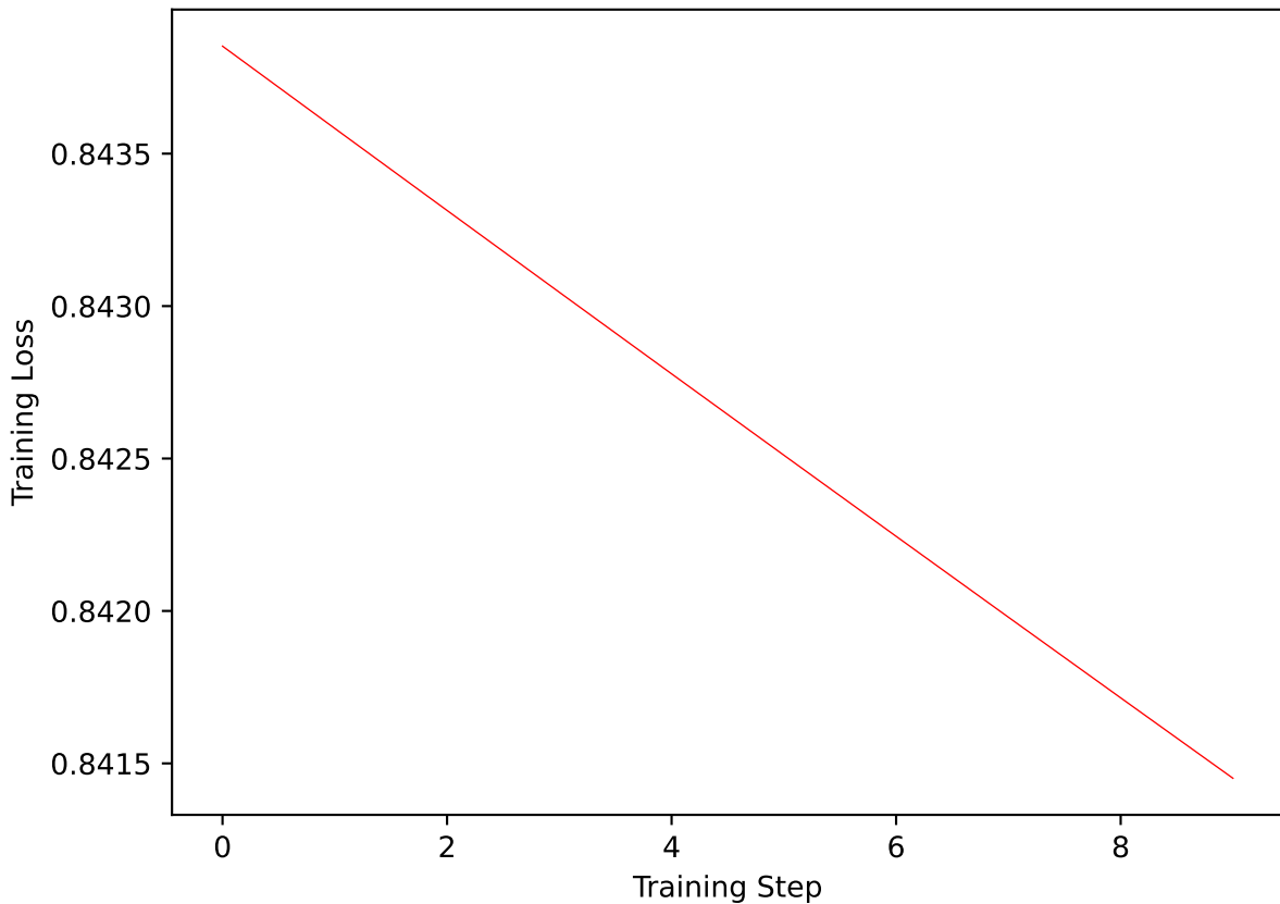
Training loss
