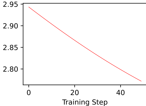
\theta dim 3
