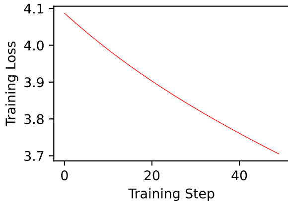
\theta dim 2
