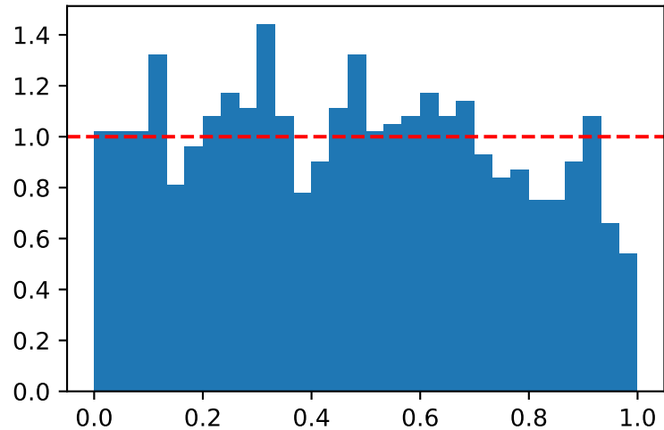
PIT t1 (Gauss)
