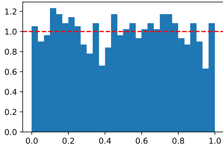
PIT t2 (Gamma)
