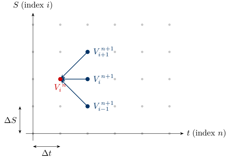
Figure 4: The explicit stencil. The value at an interior node (i, n) is a weighted combination of three nodes at the next time level, (i - 1, n + 1) , (i, n + 1) and (i + 1, n + 1) , with weights a_i , b_i and c_i from (6.2). The scheme marches backwards in time from the payoff.
