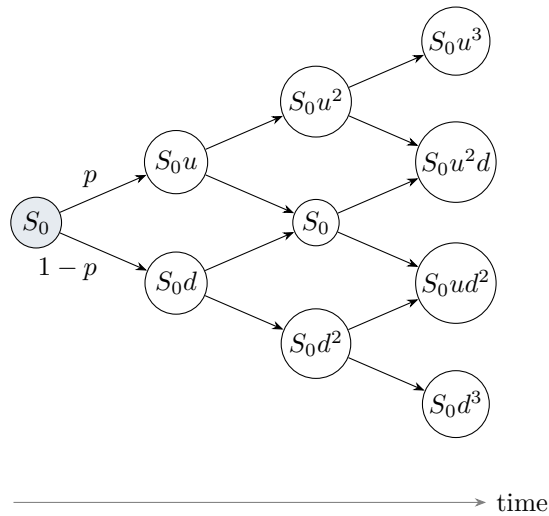
Figure 1: The first three steps of a recombining CRR tree. Each step moves up by a factor u with risk-neutral probability p or down by d with probability 1 - p ; an up move and a down move recombine to the same price.
