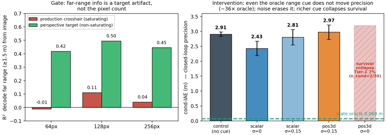
Figure 5. Left (gate): far-range ( \geq 1.5 m) image \rightarrow distance R^2 for three resolutions \times two target renderers. The saturating production crosshair is uninformative at every resolution (raising pixels does nothing); a non-saturating perspective target restores \sim half the far-range information already at 64 px — the loss is a target artifact, not the pixel count. Right (intervention): closed-loop precision (cond-IAE, 3 seeds) when the policy is handed the metric position error the FPV lacks. Even the oracle scalar range ( \sigma=0 ) leaves precision \sim 36\times the state oracle (green dashed, 0.068 m); sensor noise erases the gain; the richer 3-D cue ( \sigma=0 ) collapses survival (hatched; conditional IAE unreliable). Precision is not sensing-gated ; the coverage / teacher-competence hypothesis this points to is built and tested decisively — and also excluded — in §6.4.
