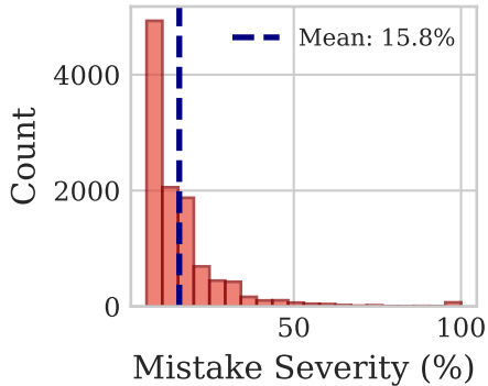
(a) RuleBased Mistake Severity Distribution
