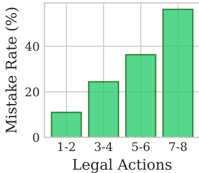
(c) Mistakes by Choice Complexity
