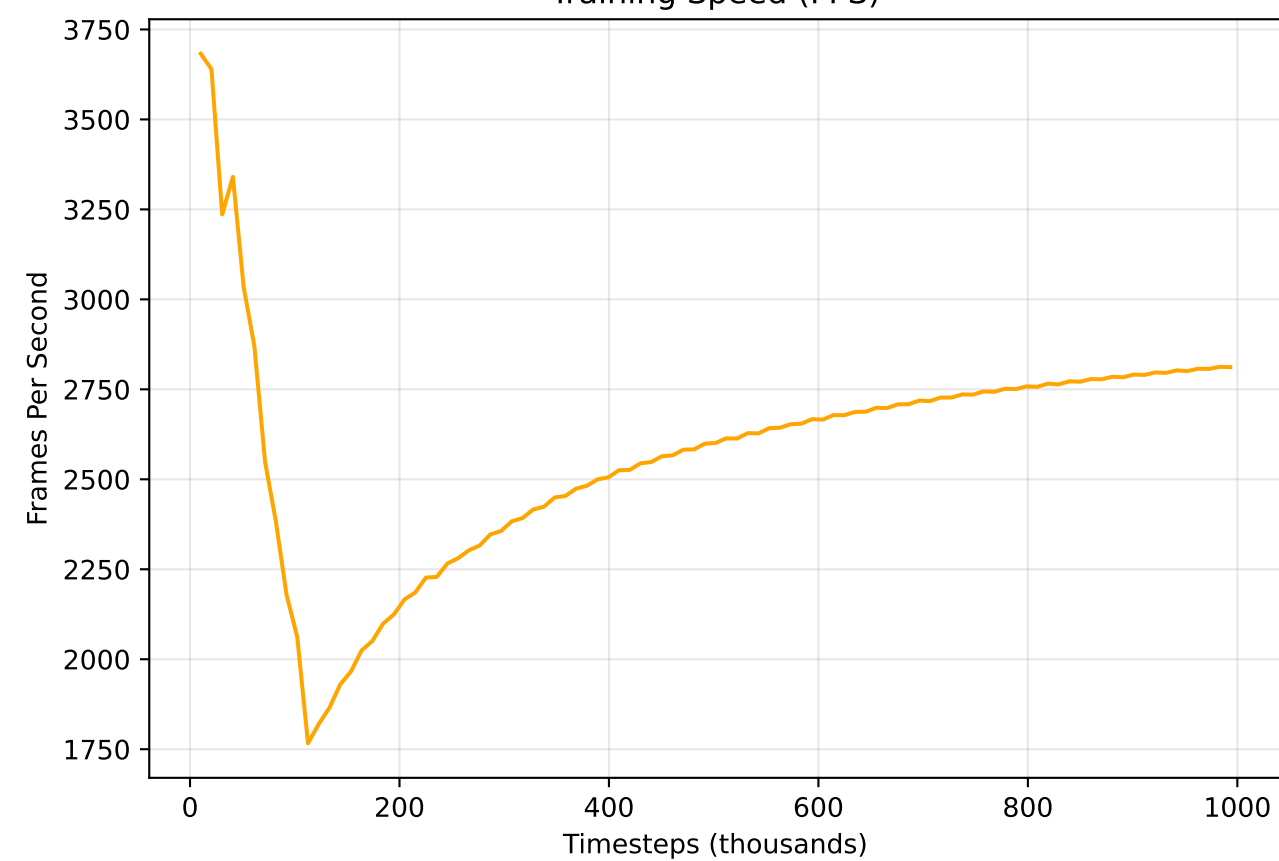
Training Speed (FPS)
