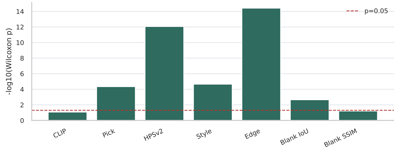
Sample-level significance: Ours vs SDXL+LoRA
